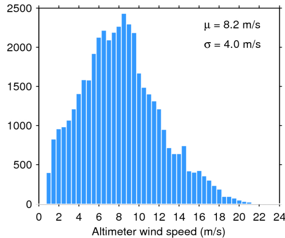
Figure 33. Histogram of flag-valid wind over oceans and lakes for 29/03/2019. The mean ( \mu ) and standard deviation ( \sigma ) are also shown. Note that values larger than 24 m/s are excluded from the histogram for the sake of readability but not from the computation of \mu and \sigma .
