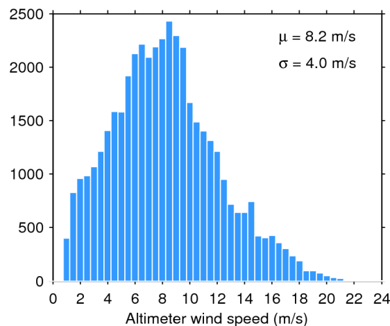
Figure 35. Histogram of science-valid wind over oceans and lakes for 29/03/2019. The mean ( \mu ) and standard deviation ( \sigma ) are also shown. Note that values larger than 24 m/s are excluded from the histogram for the sake of readability but not from the computation of \mu and \sigma .
