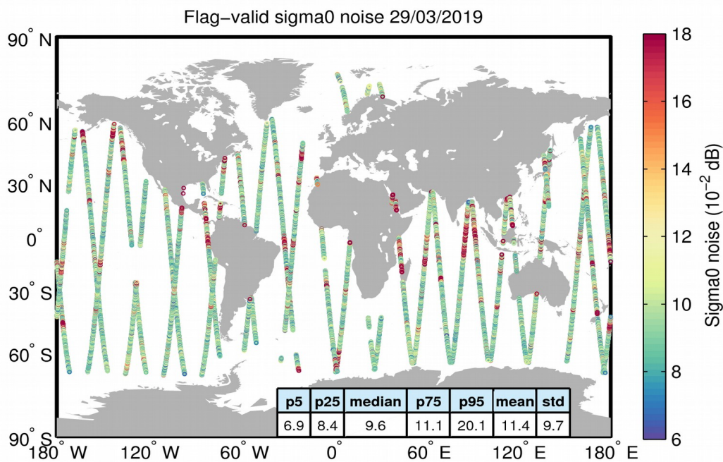
Figure 26. Geographical distribution of flag-valid 20-Hz sigma0 measurement noise over oceans and lakes for 29/03/2019. The statistical values shown in the table refer to the sigma0 noise and are calculated over all measurements shown in the figure.
