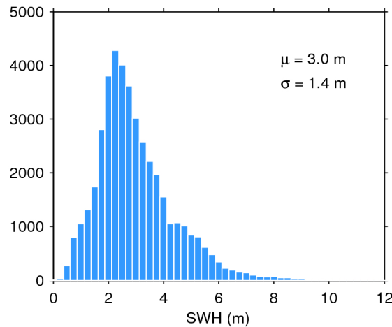
Figure 20. Histogram of science-valid SWH over oceans and lakes for 29/03/2019. The mean ( \mu ) and standard deviation ( \sigma ) are also shown. Note that values larger than 12 m are excluded from the histogram for the sake of readability but not from the computation of \mu and \sigma .
