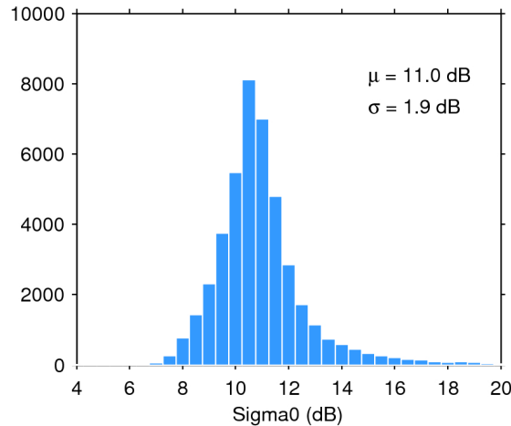
Figure 25. Histogram of flag-valid sigma0 over oceans and lakes for 29/03/2019. The mean ( \mu ) and standard deviation ( \sigma ) are also shown. Note that values outside [4 20] dB are excluded from the histogram for the sake of readability but not from the computation of \mu and \sigma .
