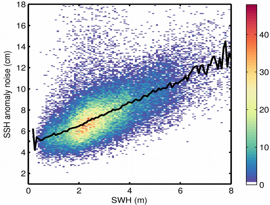
Figure 9. 2D histogram showing flag-valid SSH anomaly noise as a function of SWH for 29/03/2019. The black line denotes the median SSH anomaly noise as a function of SWH.
