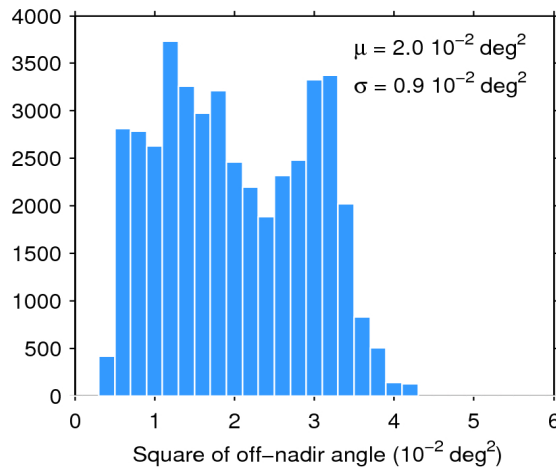
Figure 39. Histogram of flag-valid mispointing over oceans and lakes for 29/03/2019. The mean ( \mu ) and standard deviation ( \sigma ) are also shown. Note that values larger than 6 \cdot 10^{-2} \text{ deg}^2 are excluded from the histogram for the sake of readability but not from the computation of \mu and \sigma .
