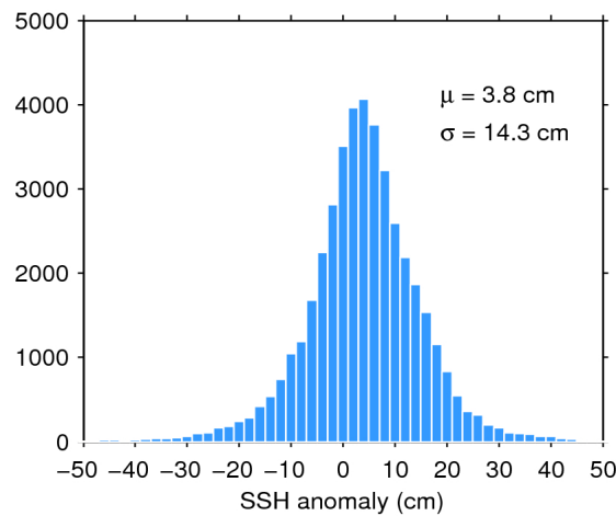
Figure 7. Histogram of flag-valid SSH anomaly over oceans and lakes for 29/03/2019. The mean ( \mu ) and standard deviation ( \sigma ) are also shown. Note that values outside [-50\ 50] cm are excluded from the histogram for the sake of readability but not from the computation of \mu and \sigma .
