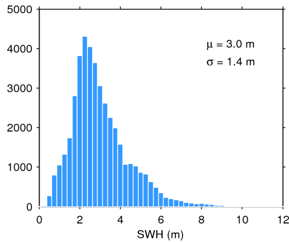
Figure 17. Histogram of flag-valid SWH over oceans and lakes for 29/03/2019. The mean ( \mu ) and standard deviation ( \sigma ) are also shown. Note that values larger than 12 m are excluded from the histogram for the sake of readability but not from the computation of \mu and \sigma .
