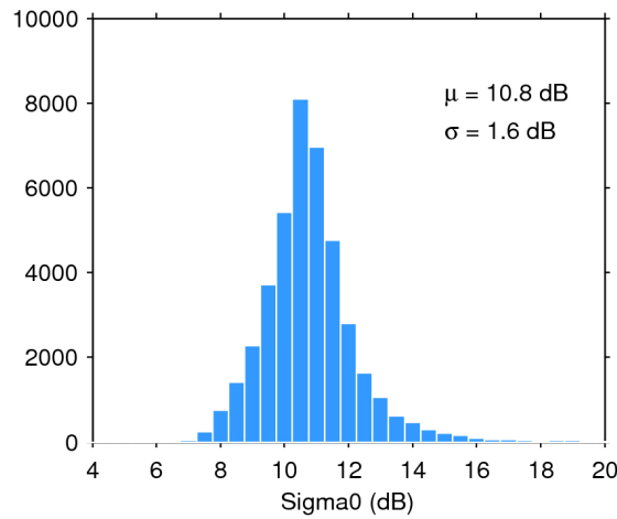
Figure 28. Histogram of science-valid sigma0 over oceans and lakes for 29/03/2019. The mean ( \mu ) and standard deviation ( \sigma ) are also shown. Note that values outside [4 20] dB are excluded from the histogram for the sake of readability but not from the computation of \mu and \sigma .
