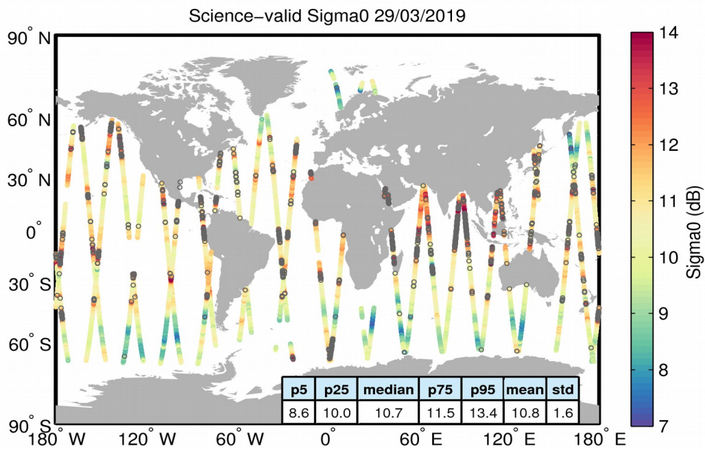
Figure 27. Geographical distribution of science-valid sigma0 data over oceans and lakes for 29/03/2019. The statistical values shown in the table refer to the sigma0 in dB and are calculated over all measurements shown in the figure. Gray circles denote records that have been rejected based on the editing criteria described in Table 4.
