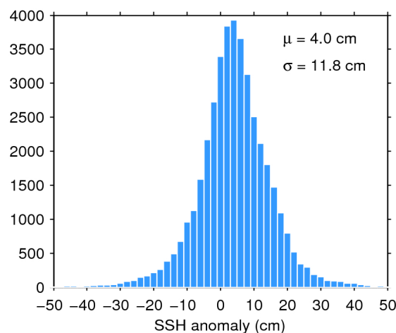
Figure 11. Histogram of science-valid SSH anomaly over oceans and lakes for 29/03/2019. The mean ( \mu ) and standard deviation ( \sigma ) are also shown. Note that values outside [-50 50] cm are excluded from the histogram for the sake of readability but not from the computation of \mu and \sigma .
