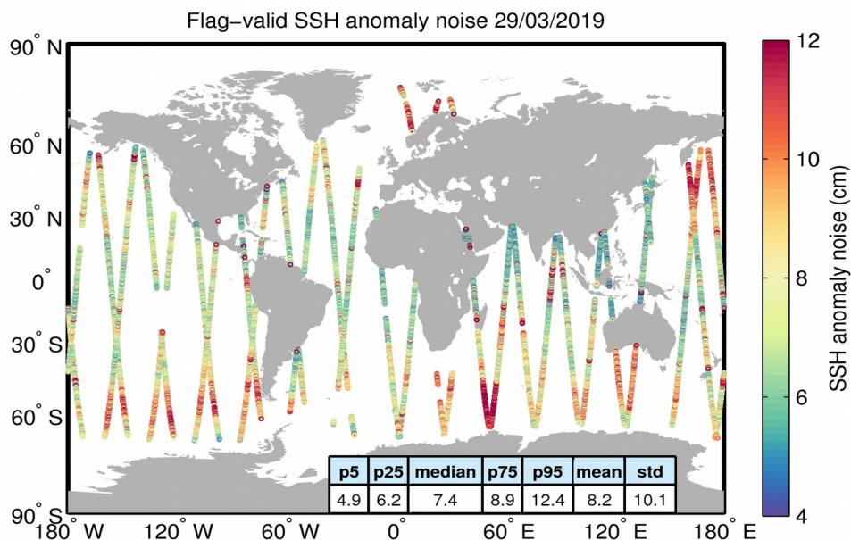
Figure 8. Geographical distribution of flag-valid 20-Hz SSH anomaly measurement noise over oceans and lakes for 29/03/2019. The statistical values shown in the table refer to the SSH anomaly noise and are calculated over all measurements shown in the figure.
