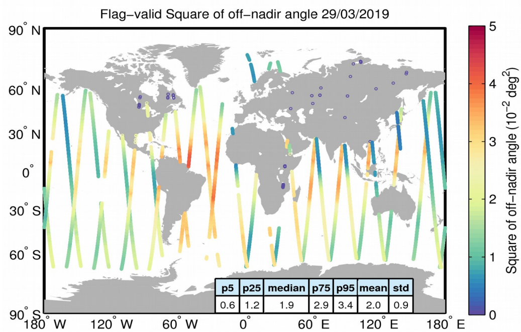
Figure 37. Geographical distribution of flag-valid mispointing data over oceans and lakes for 29/03/2019. The statistical values shown in the table refer to the mispointing in 10^{-2} \text{deg}^2 and are calculated over all measurements shown in the figure.
