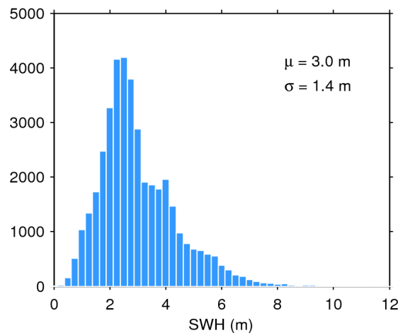
Figure 20. Histogram of science-valid SWH over oceans and lakes for 28/03/2019. The mean ( \mu ) and standard deviation ( \sigma ) are also shown. Note that values larger than 12 m are excluded from the histogram for the sake of readability but not from the computation of \mu and \sigma .
