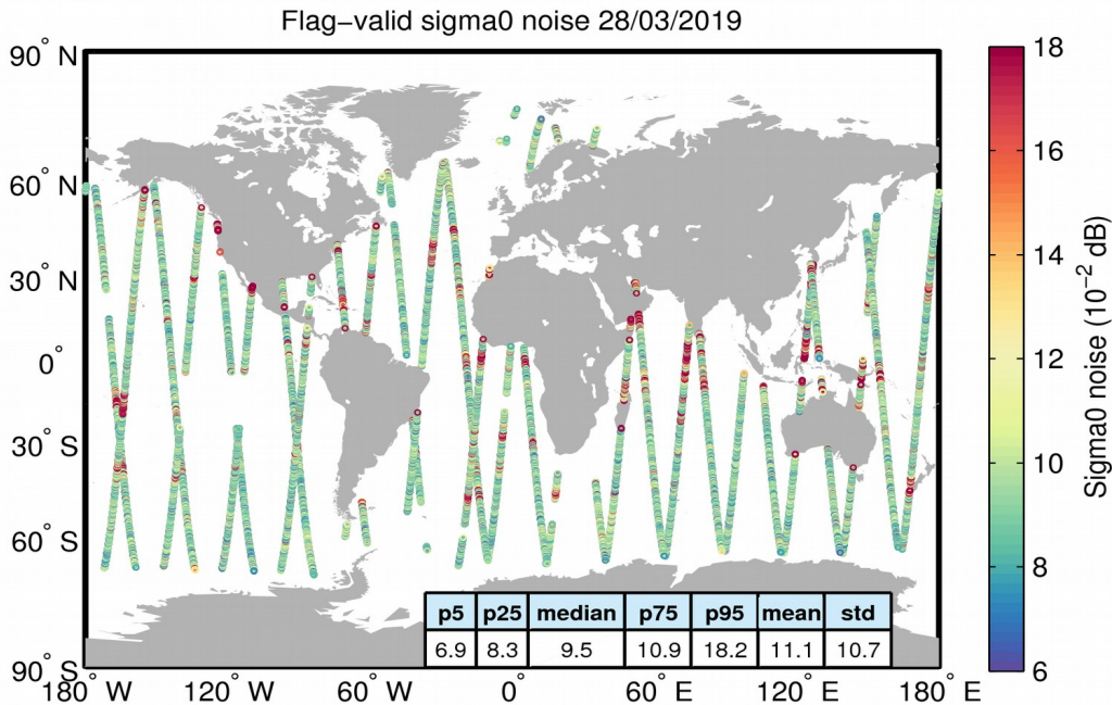
Figure 26. Geographical distribution of flag-valid 20-Hz sigma0 measurement noise over oceans and lakes for 28/03/2019. The statistical values shown in the table refer to the sigma0 noise and are calculated over all measurements shown in the figure.
