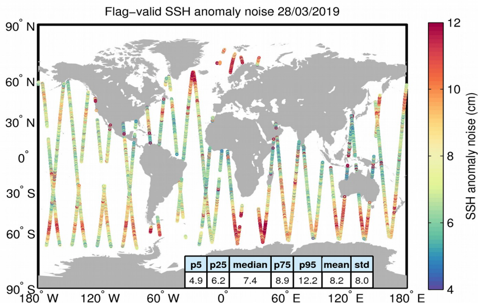
Figure 8. Geographical distribution of flag-valid 20-Hz SSH anomaly measurement noise over oceans and lakes for 28/03/2019. The statistical values shown in the table refer to the SSH anomaly noise and are calculated over all measurements shown in the figure.
