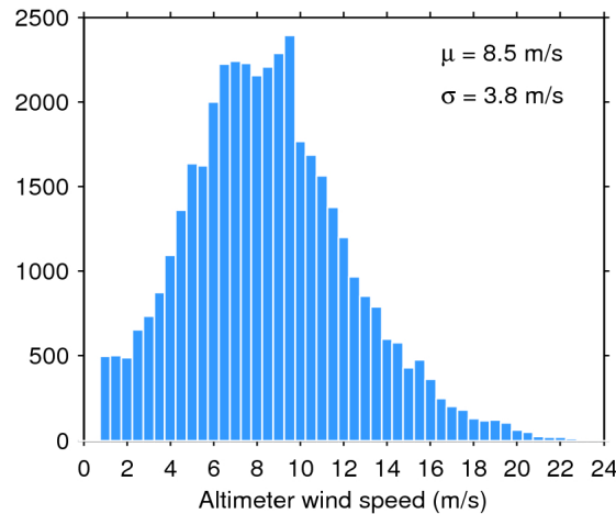
Figure 33. Histogram of flag-valid wind over oceans and lakes for 28/03/2019. The mean ( \mu ) and standard deviation ( \sigma ) are also shown. Note that values larger than 24 m/s are excluded from the histogram for the sake of readability but not from the computation of \mu and \sigma .
