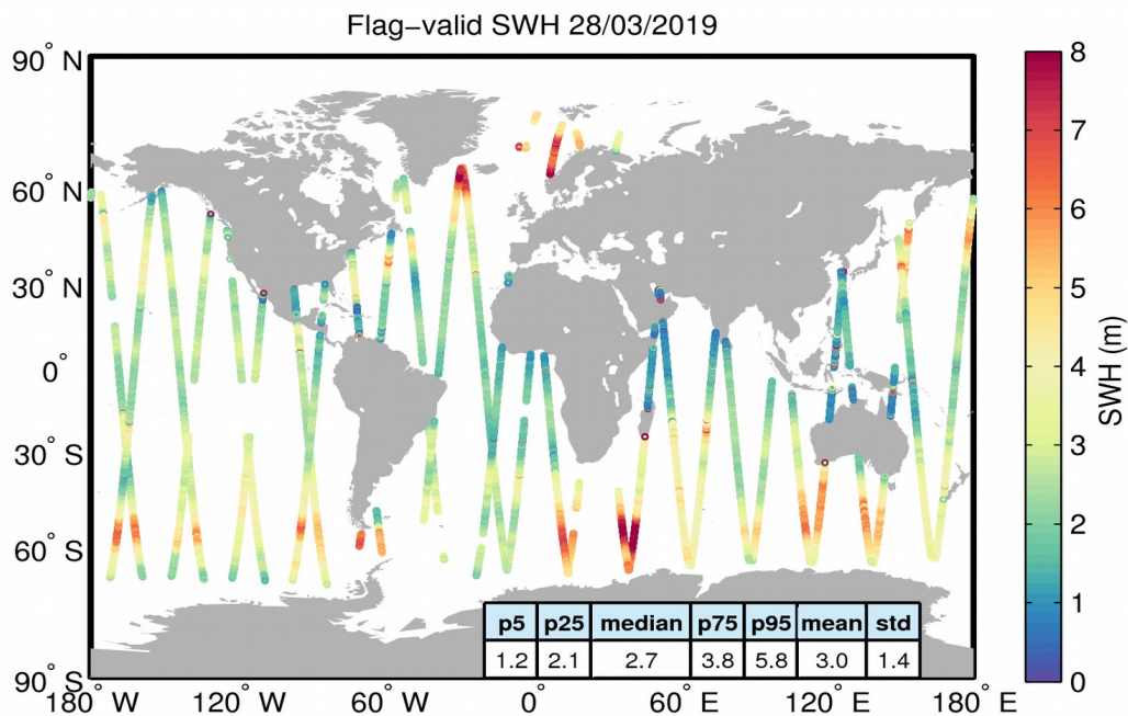
Figure 15. Geographical distribution of flag-valid SWH data over oceans and lakes for 28/03/2019. The statistical values shown in the table refer to the SWH in m and are calculated over all measurements shown in the figure.
