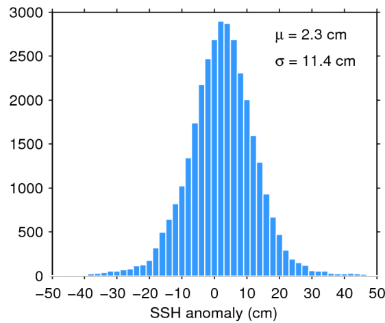
Figure 11. Histogram of science-valid SSH anomaly over oceans and lakes for 28/03/2019. The mean ( \mu ) and standard deviation ( \sigma ) are also shown. Note that values outside [-50 50] cm are excluded from the histogram for the sake of readability but not from the computation of \mu and \sigma .
