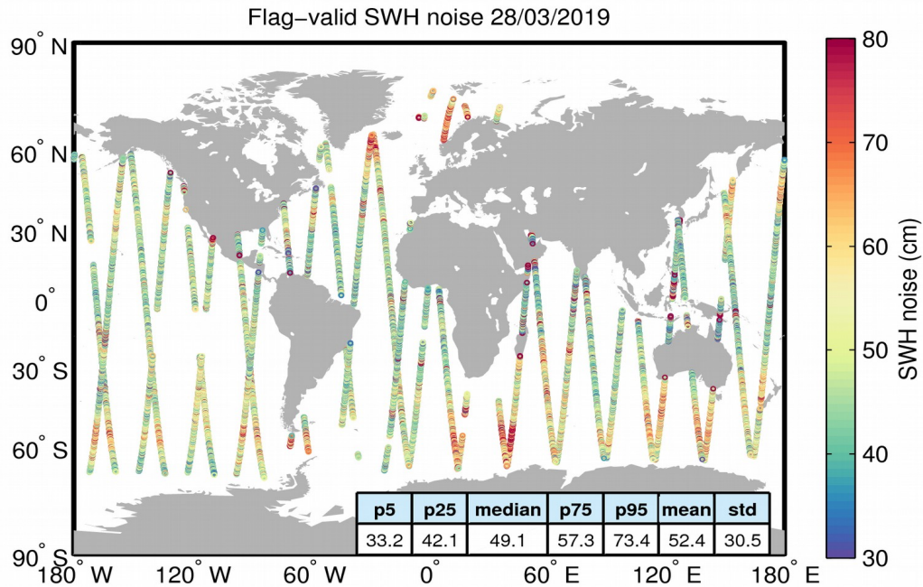
Figure 18. Geographical distribution of flag-valid 20-Hz SWH measurement noise over oceans and lakes for 28/03/2019. The statistical values shown in the figure refer to the SWH noise and are calculated over all measurements shown in the figure.
