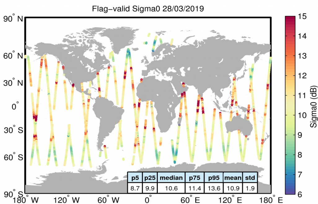
Figure 23. Geographical distribution of flag-valid sigma0 data over oceans and lakes for 28/03/2019. The statistical values shown in the table refer to the sigma0 in dB and are calculated over all measurements shown in the figure.
