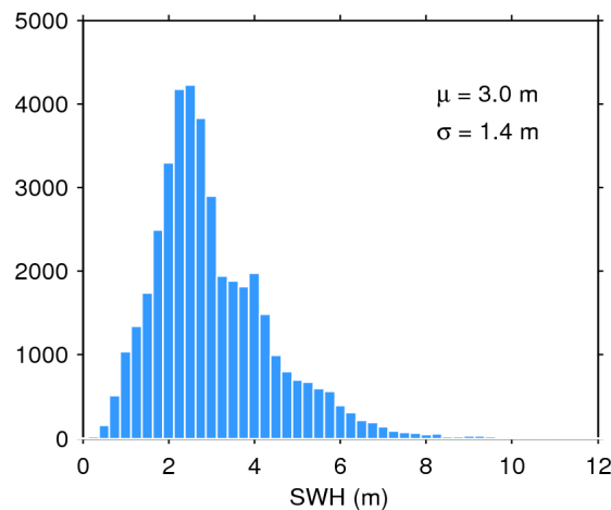
Figure 17. Histogram of flag-valid SWH over oceans and lakes for 28/03/2019. The mean ( \mu ) and standard deviation ( \sigma ) are also shown. Note that values larger than 12 m are excluded from the histogram for the sake of readability but not from the computation of \mu and \sigma .
