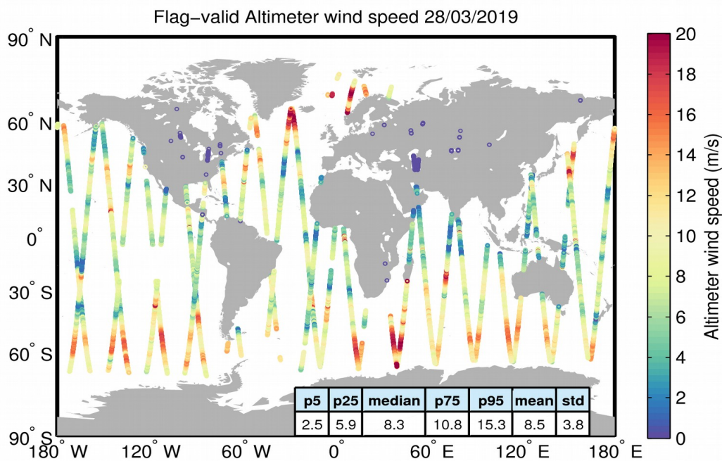
Figure 31. Geographical distribution of flag-valid wind data over oceans and lakes for 28/03/2019. The statistical values shown in the table refer to the wind in m/s and are calculated over all measurements shown in the figure.
