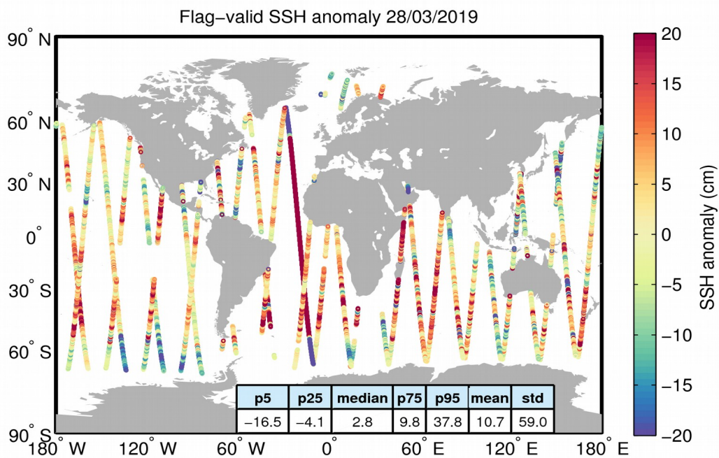
Figure 5. Geographical distribution of flag-valid 1-Hz SSH anomaly data over oceans and lakes for 28/03/2019. The statistical values shown in the table refer to the SSH anomaly in cm and are calculated over all measurements shown in the figure.
