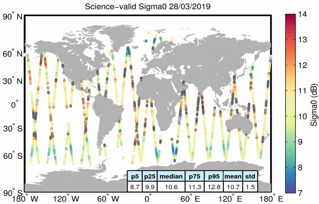
Figure 27. Geographical distribution of science-valid sigma0 data over oceans and lakes for 28/03/2019. The statistical values shown in the table refer to the sigma0 in dB and are calculated over all measurements shown in the figure. Gray circles denote records that have been rejected based on the editing criteria described in Table 4.
