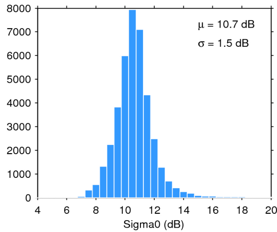
Figure 28. Histogram of science-valid sigma0 over oceans and lakes for 28/03/2019. The mean ( \mu ) and standard deviation ( \sigma ) are also shown. Note that values outside [4 20] dB are excluded from the histogram for the sake of readability but not from the computation of \mu and \sigma .
