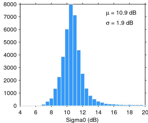
Figure 25. Histogram of flag-valid sigma0 over oceans and lakes for 28/03/2019. The mean ( \mu ) and standard deviation ( \sigma ) are also shown. Note that values outside [4 20] dB are excluded from the histogram for the sake of readability but not from the computation of \mu and \sigma .
