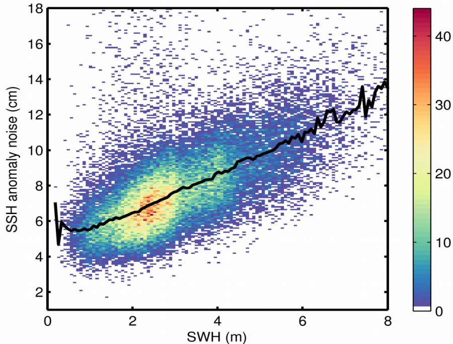
Figure 9. 2D histogram showing flag-valid SSH anomaly noise as a function of SWH for 28/03/2019. The black line denotes the median SSH anomaly noise as a function of SWH.
