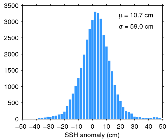
Figure 7. Histogram of flag-valid SSH anomaly over oceans and lakes for 28/03/2019. The mean ( \mu ) and standard deviation ( \sigma ) are also shown. Note that values outside [-50\ 50] cm are excluded from the histogram for the sake of readability but not from the computation of \mu and \sigma .
