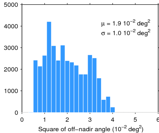
Figure 39. Histogram of flag-valid mispointing over oceans and lakes for 28/03/2019. The mean ( \mu ) and standard deviation ( \sigma ) are also shown. Note that values larger than 6 \cdot 10^{-2} \text{ deg}^2 are excluded from the histogram for the sake of readability but not from the computation of \mu and \sigma .
