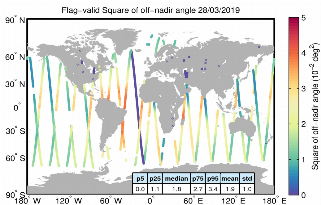
Figure 37. Geographical distribution of flag-valid mispointing data over oceans and lakes for 28/03/2019. The statistical values shown in the table refer to the mispointing in 10^{-2} deg 2 and are calculated over all measurements shown in the figure.
