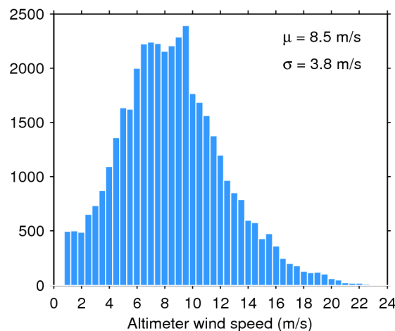
Figure 35. Histogram of science-valid wind over oceans and lakes for 28/03/2019. The mean ( \mu ) and standard deviation ( \sigma ) are also shown. Note that values larger than 24 m/s are excluded from the histogram for the sake of readability but not from the computation of \mu and \sigma .
