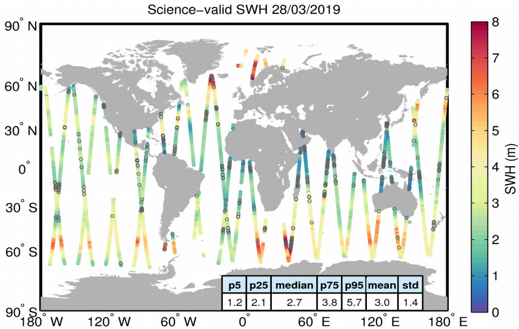
Figure 19. Geographical distribution of science-valid SWH data over oceans and lakes for 28/03/2019. The statistical values shown in the table refer to the SWH in m and are calculated over all measurements shown in the figure. Gray circles denote records that have been rejected based on the editing criteria described in Table 3.
