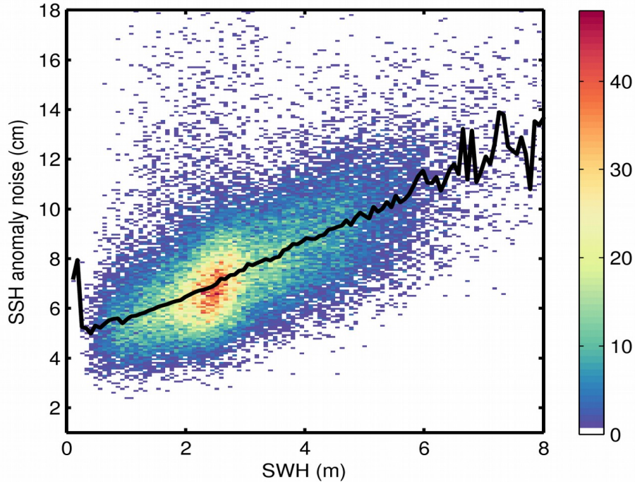
Figure 9. 2D histogram showing flag-valid SSH anomaly noise as a function of SWH for 27/03/2019. The black line denotes the median SSH anomaly noise as a function of SWH.
