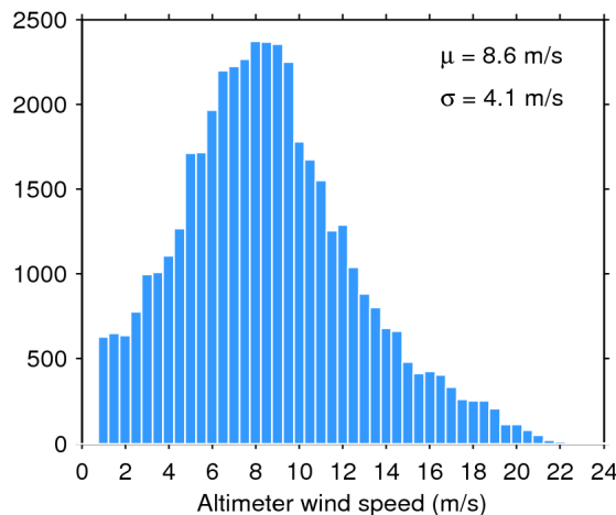
Figure 35. Histogram of science-valid wind over oceans and lakes for 27/03/2019. The mean ( \mu ) and standard deviation ( \sigma ) are also shown. Note that values larger than 24 m/s are excluded from the histogram for the sake of readability but not from the computation of \mu and \sigma .
