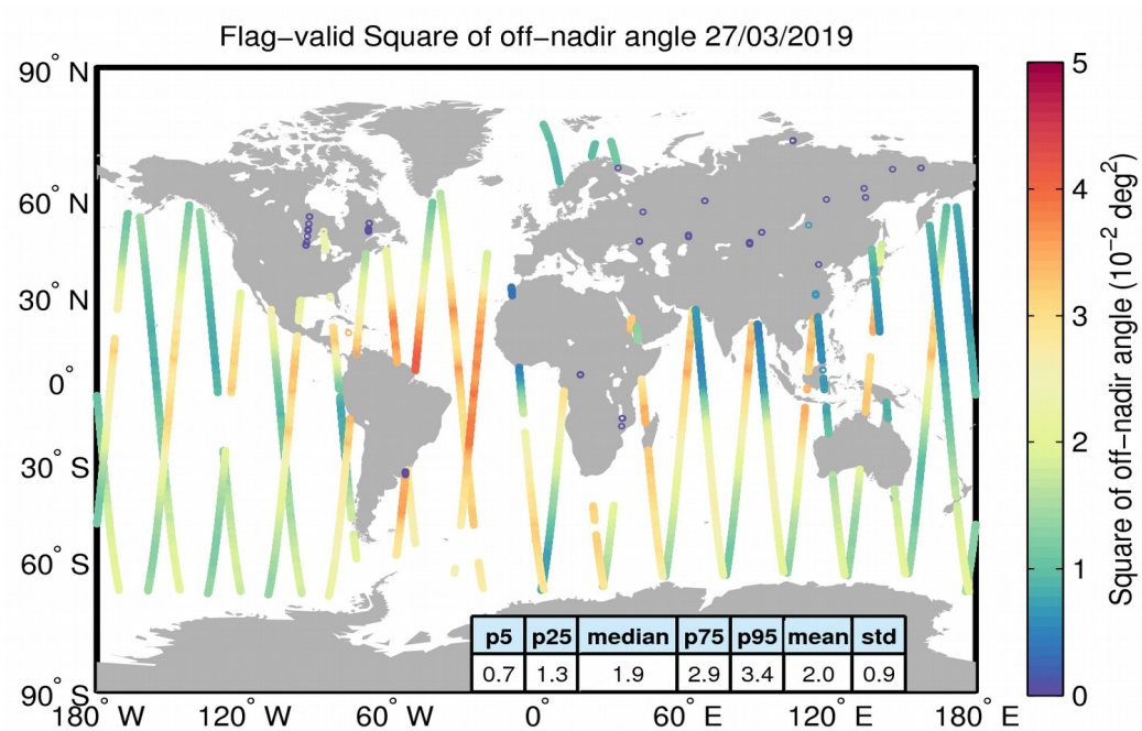
Figure 37. Geographical distribution of flag-valid mispointing data over oceans and lakes for 27/03/2019. The statistical values shown in the table refer to the mispointing in 10^{-2} deg 2 and are calculated over all measurements shown in the figure.
