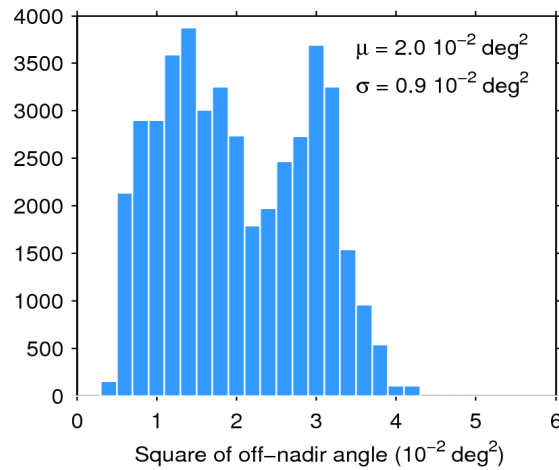
Figure 39. Histogram of flag-valid mispointing over oceans and lakes for 27/03/2019. The mean ( \mu ) and standard deviation ( \sigma ) are also shown. Note that values larger than 6 \cdot 10^{-2} \text{ deg}^2 are excluded from the histogram for the sake of readability but not from the computation of \mu and \sigma .
