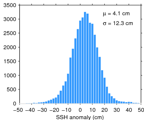
Figure 11. Histogram of science-valid SSH anomaly over oceans and lakes for 27/03/2019. The mean ( \mu ) and standard deviation ( \sigma ) are also shown. Note that values outside [-50 50] cm are excluded from the histogram for the sake of readability but not from the computation of \mu and \sigma .
