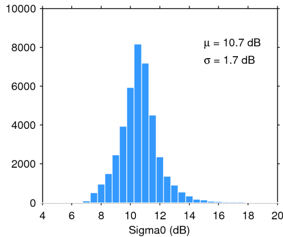
Figure 28. Histogram of science-valid sigma0 over oceans and lakes for 27/03/2019. The mean ( \mu ) and standard deviation ( \sigma ) are also shown. Note that values outside [4 20] dB are excluded from the histogram for the sake of readability but not from the computation of \mu and \sigma .
