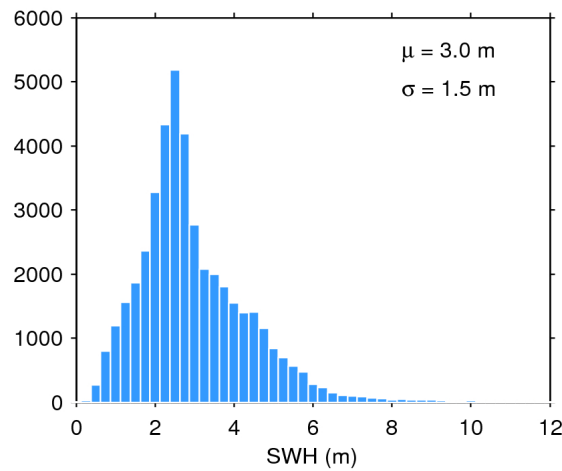
Figure 17. Histogram of flag-valid SWH over oceans and lakes for 27/03/2019. The mean ( \mu ) and standard deviation ( \sigma ) are also shown. Note that values larger than 12 m are excluded from the histogram for the sake of readability but not from the computation of \mu and \sigma .
