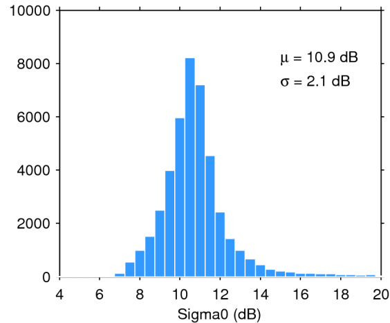
Figure 25. Histogram of flag-valid sigma0 over oceans and lakes for 27/03/2019. The mean ( \mu ) and standard deviation ( \sigma ) are also shown. Note that values outside [4 20] dB are excluded from the histogram for the sake of readability but not from the computation of \mu and \sigma .
