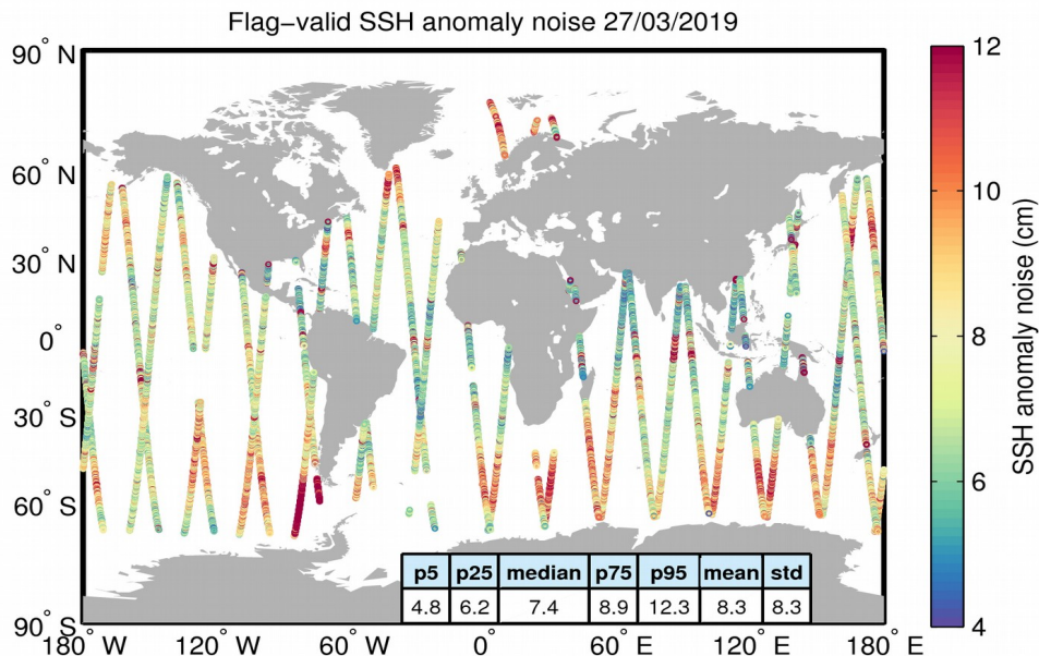
Figure 8. Geographical distribution of flag-valid 20-Hz SSH anomaly measurement noise over oceans and lakes for 27/03/2019. The statistical values shown in the table refer to the SSH anomaly noise and are calculated over all measurements shown in the figure.
