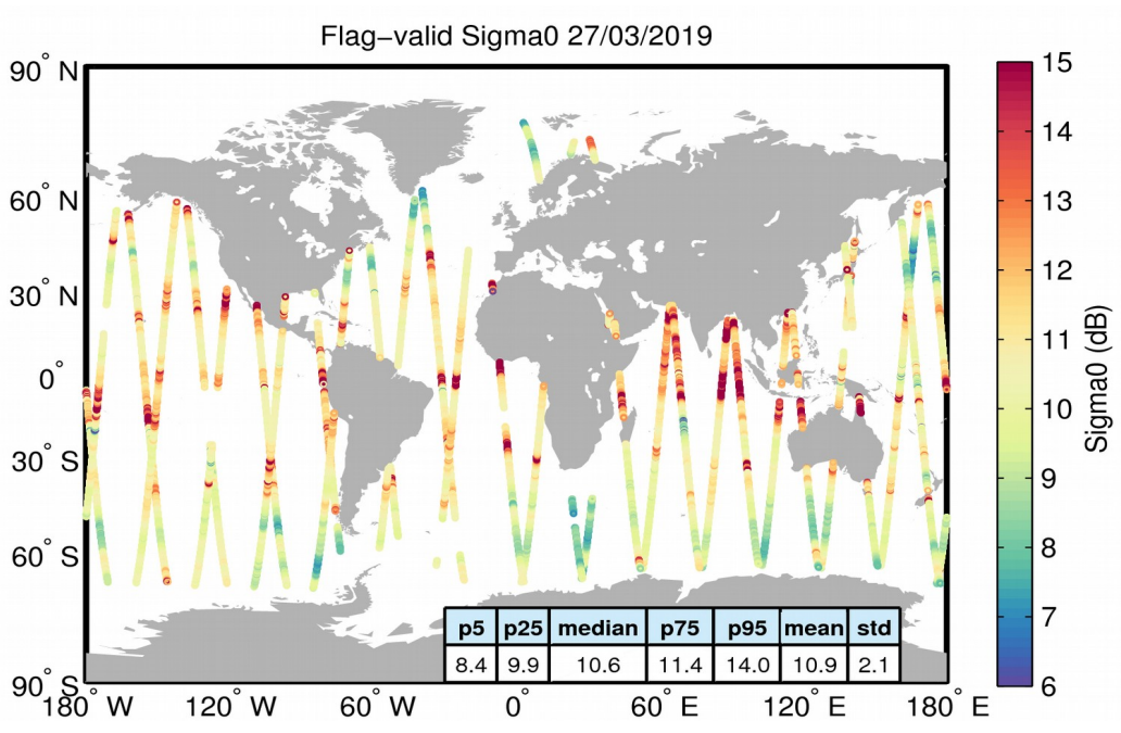
Figure 23. Geographical distribution of flag-valid sigma0 data over oceans and lakes for 27/03/2019. The statistical values shown in the table refer to the sigma0 in dB and are calculated over all measurements shown in the figure.
