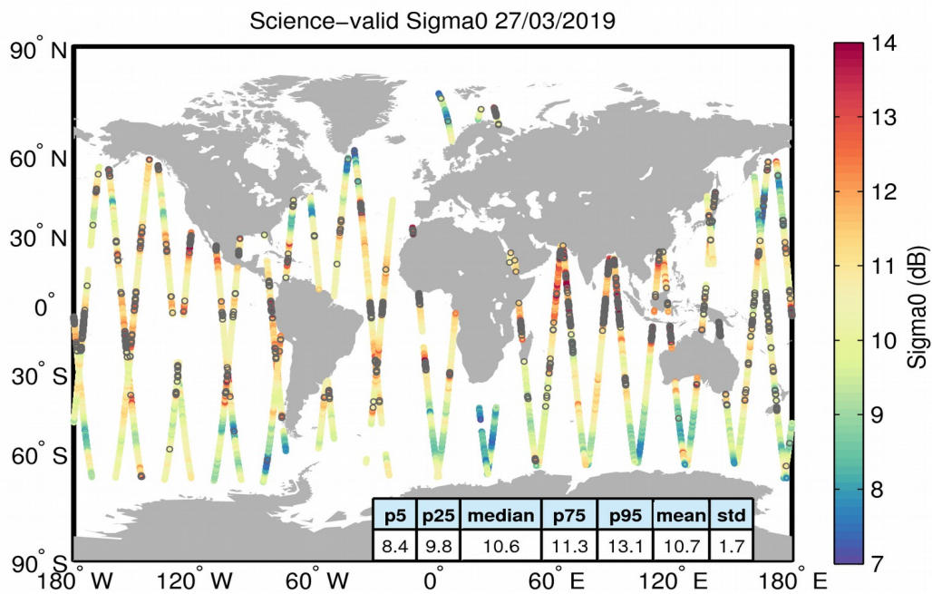
Figure 27. Geographical distribution of science-valid sigma0 data over oceans and lakes for 27/03/2019. The statistical values shown in the table refer to the sigma0 in dB and are calculated over all measurements shown in the figure. Gray circles denote records that have been rejected based on the editing criteria described in Table 4.
