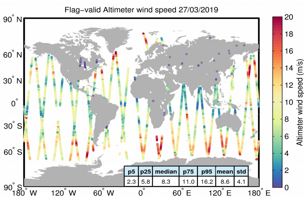
Figure 31. Geographical distribution of flag-valid wind data over oceans and lakes for 27/03/2019. The statistical values shown in the table refer to the wind in m/s and are calculated over all measurements shown in the figure.
