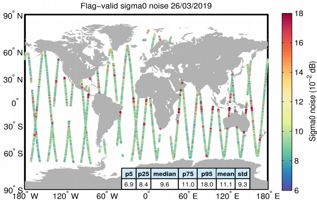
Figure 26. Geographical distribution of flag-valid 20-Hz sigma0 measurement noise over oceans and lakes for 26/03/2019. The statistical values shown in the table refer to the sigma0 noise and are calculated over all measurements shown in the figure.
