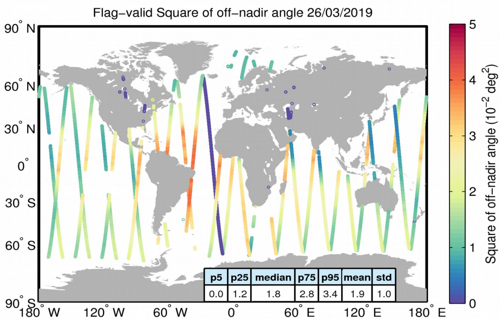
Figure 37. Geographical distribution of flag-valid mispointing data over oceans and lakes for 26/03/2019. The statistical values shown in the table refer to the mispointing in 10^{-2} deg 2 and are calculated over all measurements shown in the figure.
