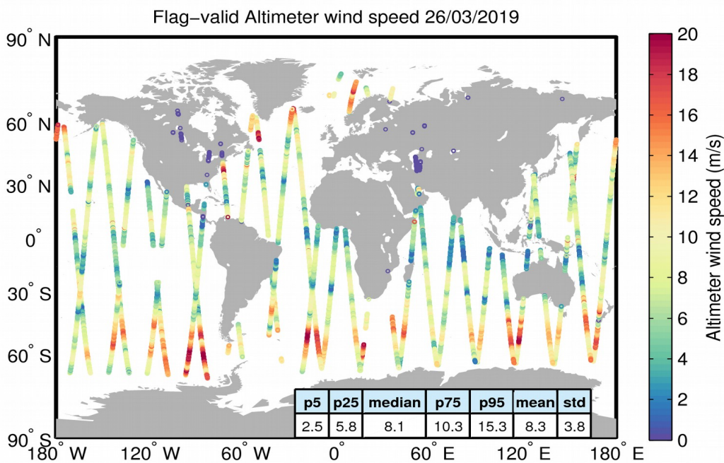
Figure 31. Geographical distribution of flag-valid wind data over oceans and lakes for 26/03/2019. The statistical values shown in the table refer to the wind in m/s and are calculated over all measurements shown in the figure.
