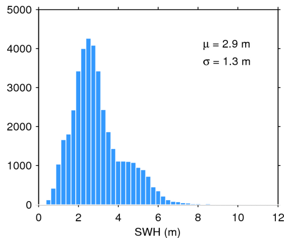
Figure 20. Histogram of science-valid SWH over oceans and lakes for 26/03/2019. The mean ( \mu ) and standard deviation ( \sigma ) are also shown. Note that values larger than 12 m are excluded from the histogram for the sake of readability but not from the computation of \mu and \sigma .
