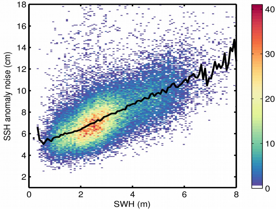
Figure 9. 2D histogram showing flag-valid SSH anomaly noise as a function of SWH for 26/03/2019. The black line denotes the median SSH anomaly noise as a function of SWH.
