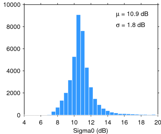
Figure 25. Histogram of flag-valid sigma0 over oceans and lakes for 26/03/2019. The mean ( \mu ) and standard deviation ( \sigma ) are also shown. Note that values outside [4 20] dB are excluded from the histogram for the sake of readability but not from the computation of \mu and \sigma .
