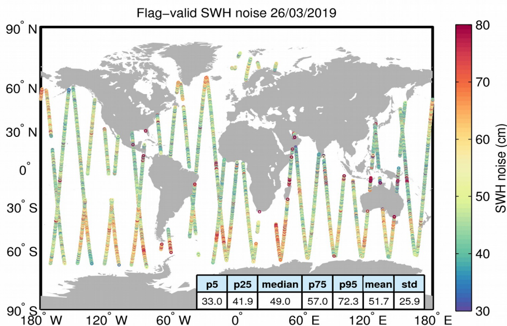
Figure 18. Geographical distribution of flag-valid 20-Hz SWH measurement noise over oceans and lakes for 26/03/2019. The statistical values shown in the table refer to the SWH noise and are calculated over all measurements shown in the figure.
