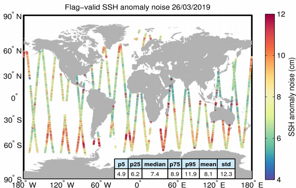
Figure 8. Geographical distribution of flag-valid 20-Hz SSH anomaly measurement noise over oceans and lakes for 26/03/2019. The statistical values shown in the table refer to the SSH anomaly noise and are calculated over all measurements shown in the figure.
