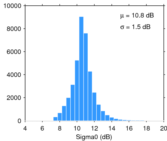
Figure 28. Histogram of science-valid sigma0 over oceans and lakes for 26/03/2019. The mean ( \mu ) and standard deviation ( \sigma ) are also shown. Note that values outside [4 20] dB are excluded from the histogram for the sake of readability but not from the computation of \mu and \sigma .
