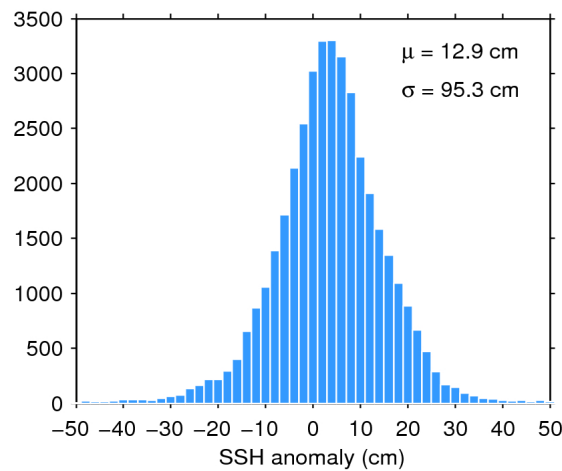
Figure 7. Histogram of flag-valid SSH anomaly over oceans and lakes for 26/03/2019. The mean ( \mu ) and standard deviation ( \sigma ) are also shown. Note that values outside [-50 50] cm are excluded from the histogram for the sake of readability but not from the computation of \mu and \sigma .
