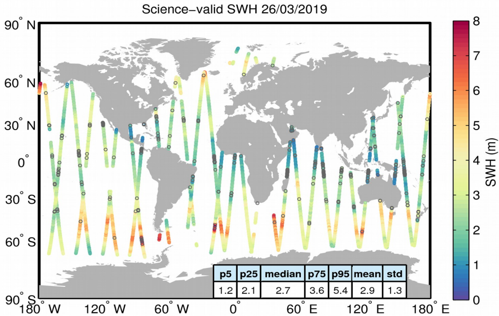
Figure 19. Geographical distribution of science-valid SWH data over oceans and lakes for 26/03/2019. The statistical values shown in the table refer to the SWH in m and are calculated over all measurements shown in the figure. Gray circles denote records that have been rejected based on the editing criteria described in Table 3.
