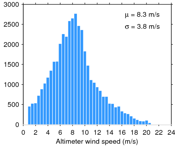
Figure 33. Histogram of flag-valid wind over oceans and lakes for 26/03/2019. The mean ( \mu ) and standard deviation ( \sigma ) are also shown. Note that values larger than 24 m/s are excluded from the histogram for the sake of readability but not from the computation of \mu and \sigma .
