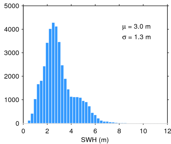
Figure 17. Histogram of flag-valid SWH over oceans and lakes for 26/03/2019. The mean ( \mu ) and standard deviation ( \sigma ) are also shown. Note that values larger than 12 m are excluded from the histogram for the sake of readability but not from the computation of \mu and \sigma .
