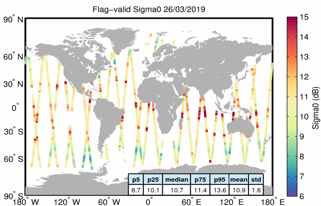
Figure 23. Geographical distribution of flag-valid sigma0 data over oceans and lakes for 26/03/2019. The statistical values shown in the table refer to the sigma0 in dB and are calculated over all measurements shown in the figure.
