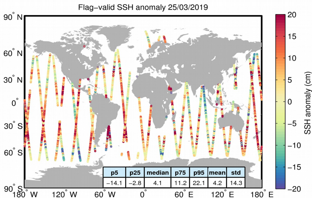
Figure 5. Geographical distribution of flag-valid 1-Hz SSH anomaly data over oceans and lakes for 25/03/2019. The statistical values shown in the table refer to the SSH anomaly in cm and are calculated over all measurements shown in the figure.
