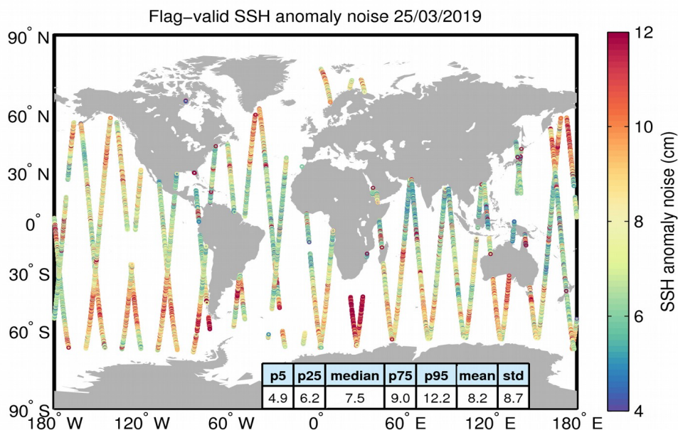
Figure 8. Geographical distribution of flag-valid 20-Hz SSH anomaly measurement noise over oceans and lakes for 25/03/2019. The statistical values shown in the table refer to the SSH anomaly noise and are calculated over all measurements shown in the figure.
