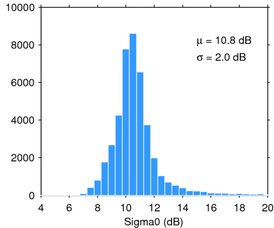
Figure 25. Histogram of flag-valid sigma0 over oceans and lakes for 25/03/2019. The mean ( \mu ) and standard deviation ( \sigma ) are also shown. Note that values outside [4 20] dB are excluded from the histogram for the sake of readability but not from the computation of \mu and \sigma .
