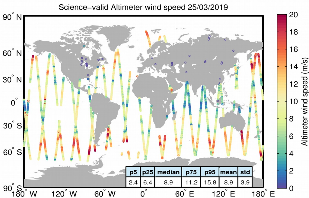
Figure 34. Geographical distribution of science-valid wind data over oceans and lakes for 25/03/2019. The statistical values shown in the table refer to the wind in m/s and are calculated over all measurements shown in the figure. Gray circles denote records that have been rejected based on the editing criteria described in Table 5.
