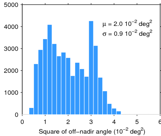
Figure 39. Histogram of flag-valid mispointing over oceans and lakes for 25/03/2019. The mean ( \mu ) and standard deviation ( \sigma ) are also shown. Note that values larger than 6 \cdot 10^{-2} \text{ deg}^2 are excluded from the histogram for the sake of readability but not from the computation of \mu and \sigma .
