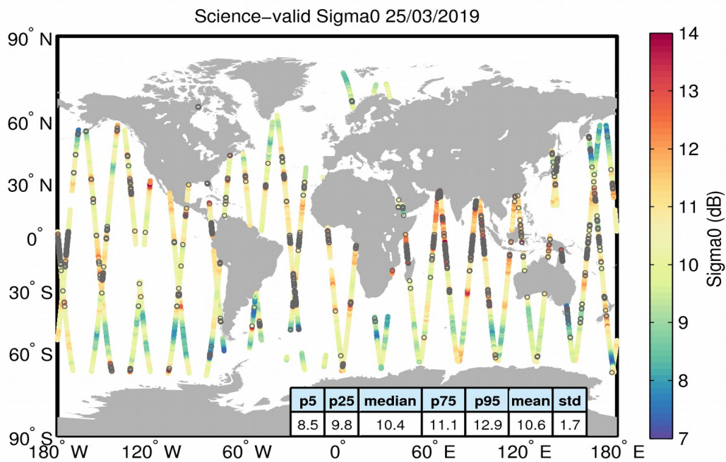
Figure 27. Geographical distribution of science-valid sigma0 data over oceans and lakes for 25/03/2019. The statistical values shown in the table refer to the sigma0 in dB and are calculated over all measurements shown in the figure. Gray circles denote records that have been rejected based on the editing criteria described in Table 4.
