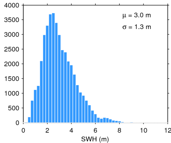
Figure 20. Histogram of science-valid SWH over oceans and lakes for 25/03/2019. The mean ( \mu ) and standard deviation ( \sigma ) are also shown. Note that values larger than 12 m are excluded from the histogram for the sake of readability but not from the computation of \mu and \sigma .
