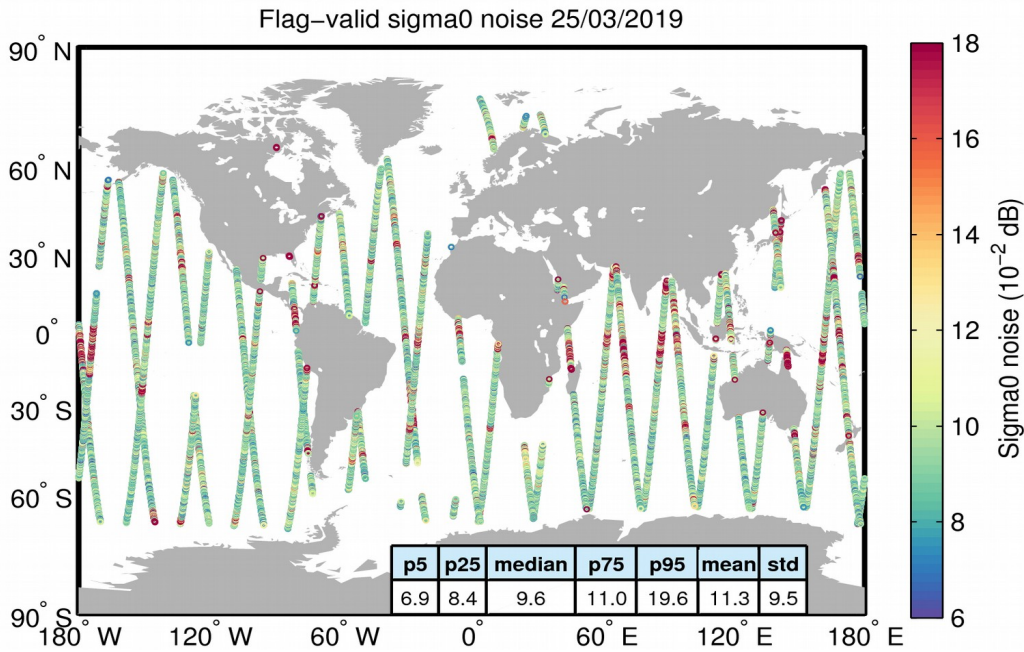
Figure 26. Geographical distribution of flag-valid 20-Hz sigma0 measurement noise over oceans and lakes for 25/03/2019. The statistical values shown in the table refer to the sigma0 noise and are calculated over all measurements shown in the figure.
