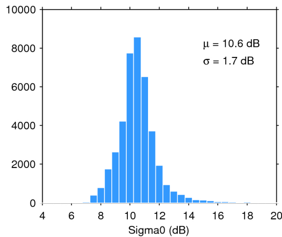
Figure 28. Histogram of science-valid sigma0 over oceans and lakes for 25/03/2019. The mean ( \mu ) and standard deviation ( \sigma ) are also shown. Note that values outside [4 20] dB are excluded from the histogram for the sake of readability but not from the computation of \mu and \sigma .
