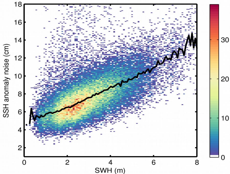
Figure 9. 2D histogram showing flag-valid SSH anomaly noise as a function of SWH for 25/03/2019. The black line denotes the median SSH anomaly noise as a function of SWH.
