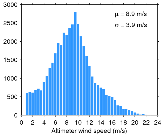
Figure 33. Histogram of flag-valid wind over oceans and lakes for 25/03/2019. The mean ( \mu ) and standard deviation ( \sigma ) are also shown. Note that values larger than 24 m/s are excluded from the histogram for the sake of readability but not from the computation of \mu and \sigma .
