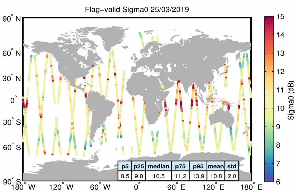
Figure 23. Geographical distribution of flag-valid sigma0 data over oceans and lakes for 25/03/2019. The statistical values shown in the table refer to the sigma0 in dB and are calculated over all measurements shown in the figure.
