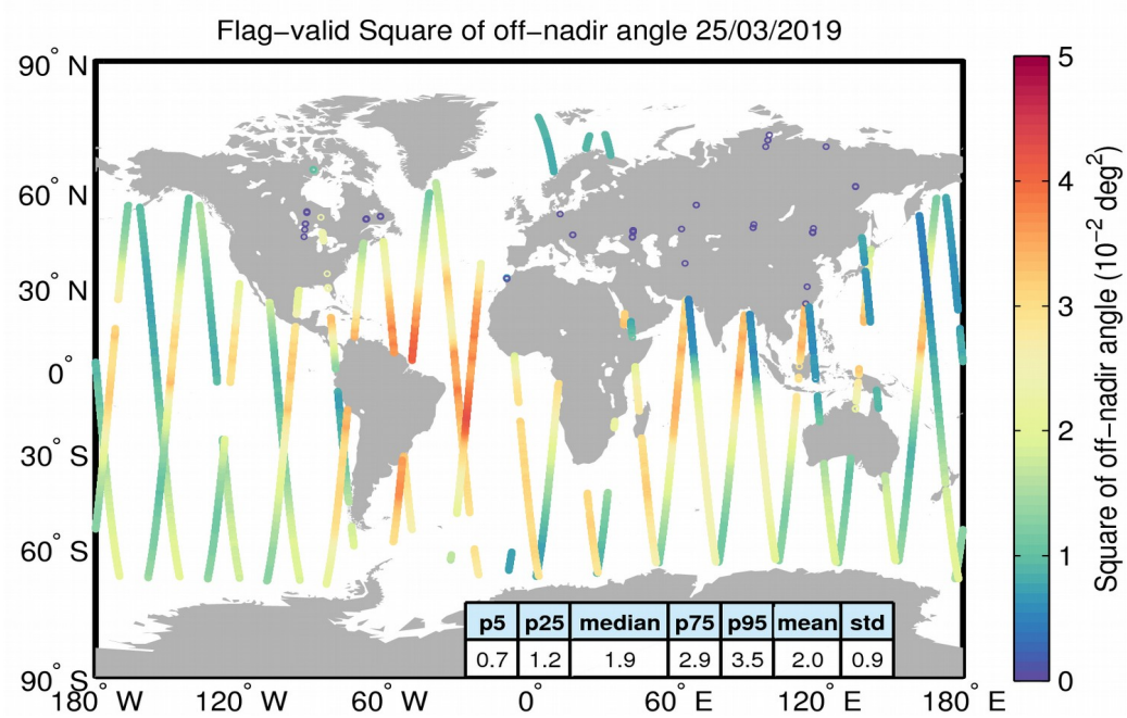
Figure 37. Geographical distribution of flag-valid mispointing data over oceans and lakes for 25/03/2019. The statistical values shown in the table refer to the mispointing in 10^{-2} \text{ deg}^2 and are calculated over all measurements shown in the figure.
