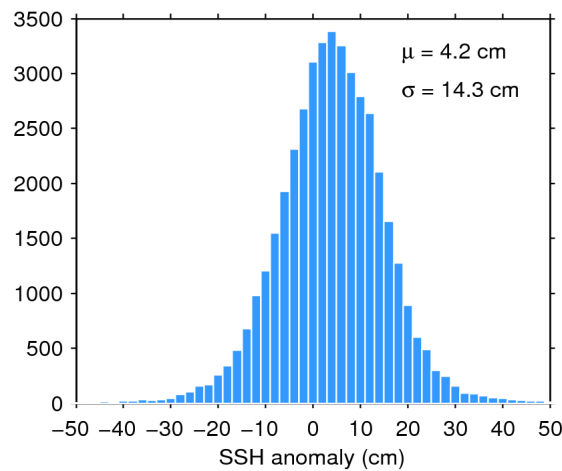
Figure 7. Histogram of flag-valid SSH anomaly over oceans and lakes for 25/03/2019. The mean ( \mu ) and standard deviation ( \sigma ) are also shown. Note that values outside [-50 50] cm are excluded from the histogram for the sake of readability but not from the computation of \mu and \sigma .
