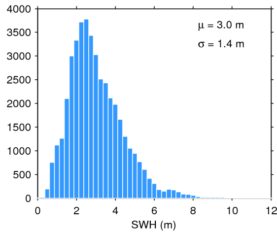
Figure 17. Histogram of flag-valid SWH over oceans and lakes for 25/03/2019. The mean ( \mu ) and standard deviation ( \sigma ) are also shown. Note that values larger than 12 m are excluded from the histogram for the sake of readability but not from the computation of \mu and \sigma .
