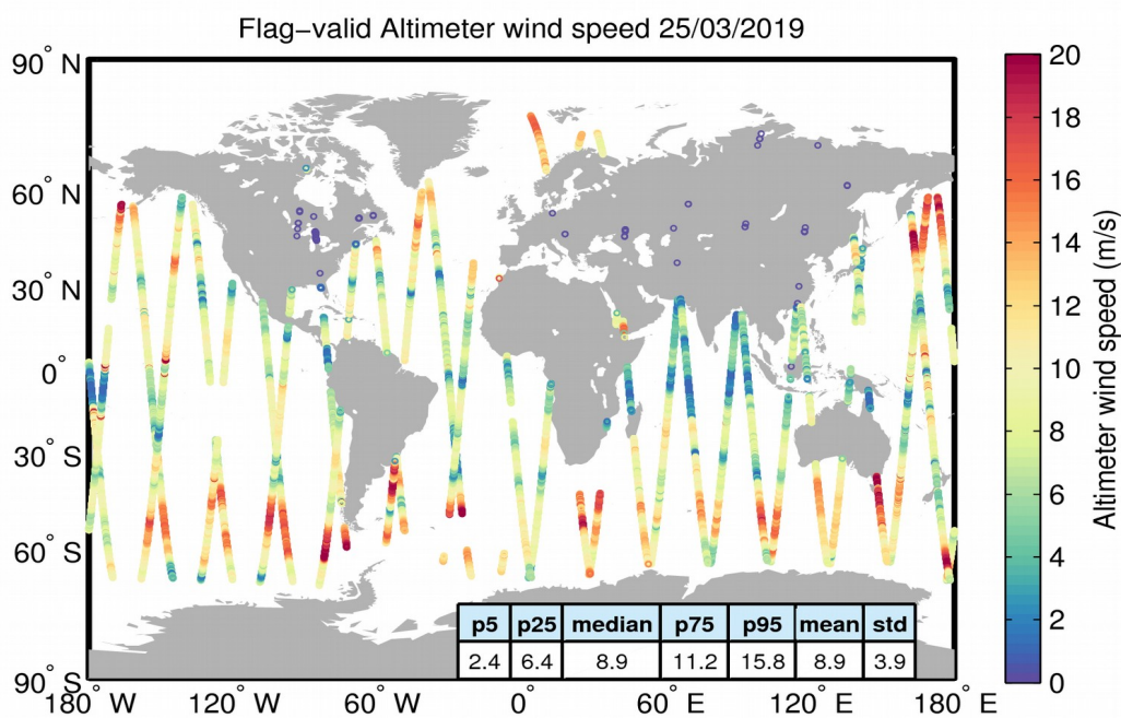
Figure 31. Geographical distribution of flag-valid wind data over oceans and lakes for 25/03/2019. The statistical values shown in the table refer to the wind in m/s and are calculated over all measurements shown in the figure.
