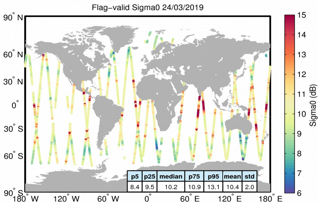
Figure 23. Geographical distribution of flag-valid sigma0 data over oceans and lakes for 24/03/2019. The statistical values shown in the table refer to the sigma0 in dB and are calculated over all measurements shown in the figure.
