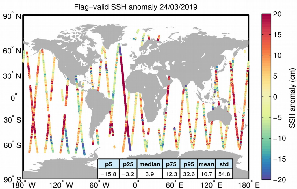
Figure 5. Geographical distribution of flag-valid 1-Hz SSH anomaly data over oceans and lakes for 24/03/2019. The statistical values shown in the table refer to the SSH anomaly in cm and are calculated over all measurements shown in the figure.
