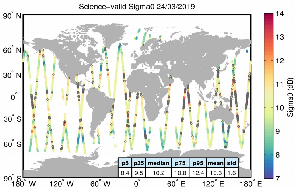
Figure 27. Geographical distribution of science-valid sigma0 data over oceans and lakes for 24/03/2019. The statistical values shown in the table refer to the sigma0 in dB and are calculated over all measurements shown in the figure. Gray circles denote records that have been rejected based on the editing criteria described in Table 4.
