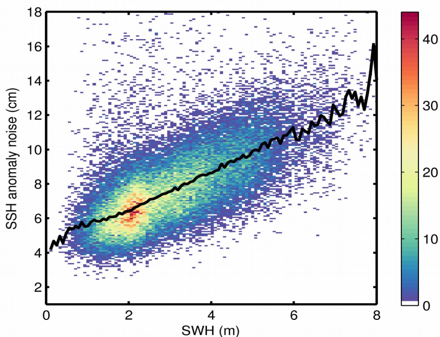
Figure 9. 2D histogram showing flag-valid SSH anomaly noise as a function of SWH for 24/03/2019. The black line denotes the median SSH anomaly noise as a function of SWH.
