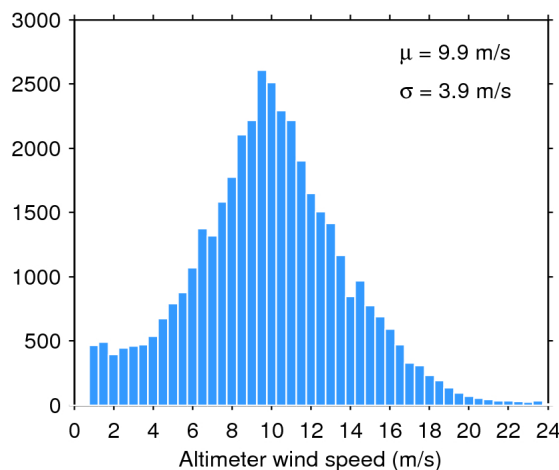
Figure 35. Histogram of science-valid wind over oceans and lakes for 24/03/2019. The mean ( \mu ) and standard deviation ( \sigma ) are also shown. Note that values larger than 24 m/s are excluded from the histogram for the sake of readability but not from the computation of \mu and \sigma .
