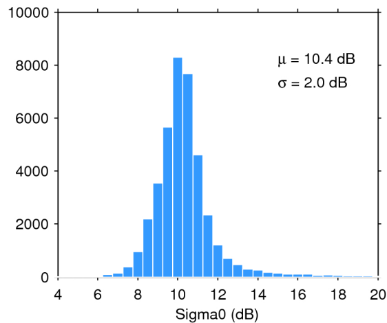
Figure 25. Histogram of flag-valid sigma0 over oceans and lakes for 24/03/2019. The mean ( \mu ) and standard deviation ( \sigma ) are also shown. Note that values outside [4 20] dB are excluded from the histogram for the sake of readability but not from the computation of \mu and \sigma .
