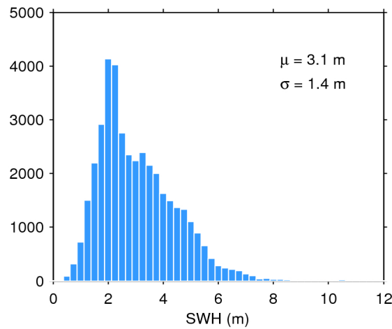
Figure 17. Histogram of flag-valid SWH over oceans and lakes for 24/03/2019. The mean ( \mu ) and standard deviation ( \sigma ) are also shown. Note that values larger than 12 m are excluded from the histogram for the sake of readability but not from the computation of \mu and \sigma .
