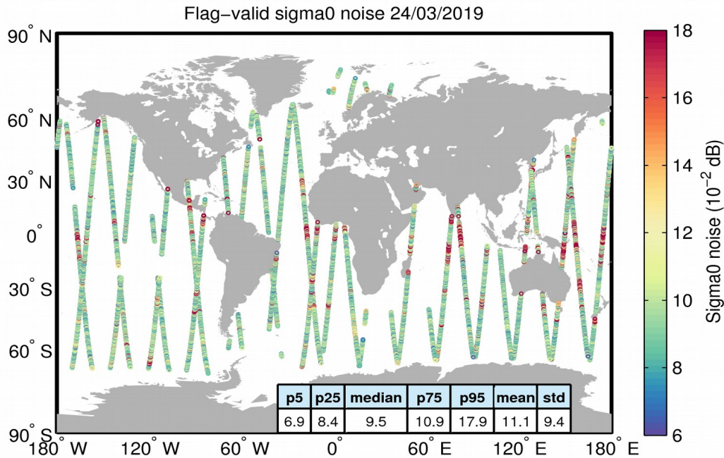
Figure 26. Geographical distribution of flag-valid 20-Hz sigma0 measurement noise over oceans and lakes for 24/03/2019. The statistical values shown in the table refer to the sigma0 noise and are calculated over all measurements shown in the figure.
