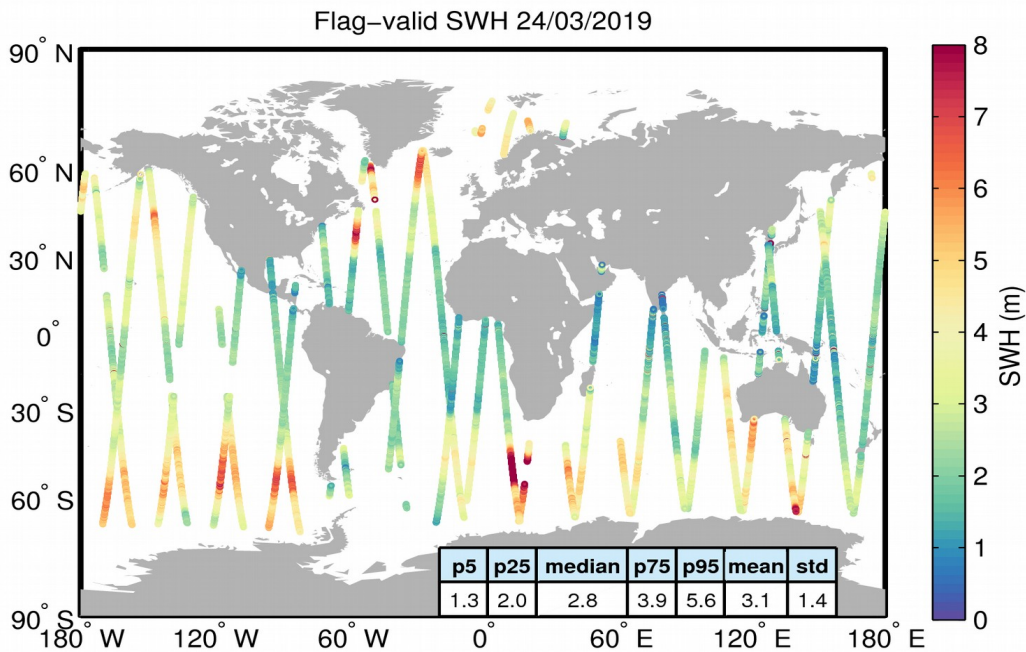
Figure 15. Geographical distribution of flag-valid SWH data over oceans and lakes for 24/03/2019. The statistical values shown in the table refer to the SWH in m and are calculated over all measurements shown in the figure.
