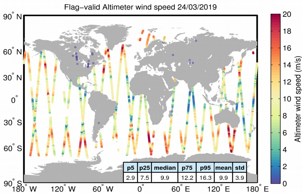
Figure 31. Geographical distribution of flag-valid wind data over oceans and lakes for 24/03/2019. The statistical values shown in the table refer to the wind in m/s and are calculated over all measurements shown in the figure.
