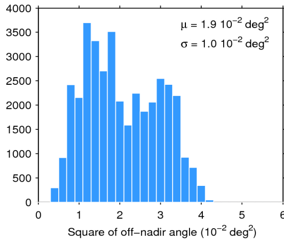
Figure 39. Histogram of flag-valid mispointing over oceans and lakes for 24/03/2019. The mean ( \mu ) and standard deviation ( \sigma ) are also shown. Note that values larger than 6 \cdot 10^{-2} \text{ deg}^2 are excluded from the histogram for the sake of readability but not from the computation of \mu and \sigma .
