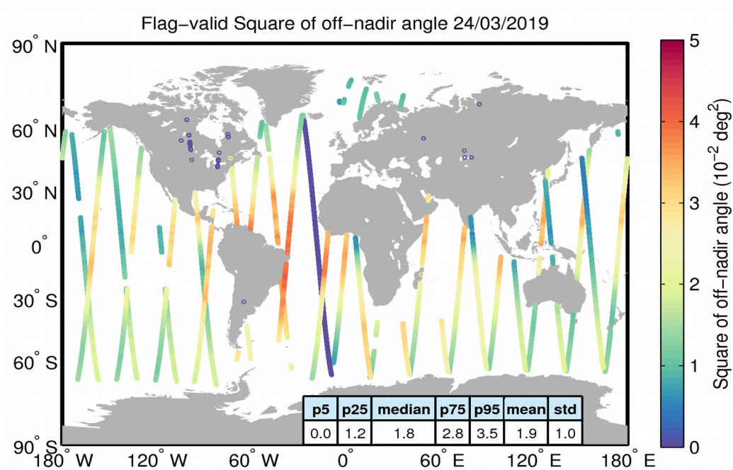
Figure 37. Geographical distribution of flag-valid mispointing data over oceans and lakes for 24/03/2019. The statistical values shown in the table refer to the mispointing in 10^{-2} deg 2 and are calculated over all measurements shown in the figure.
