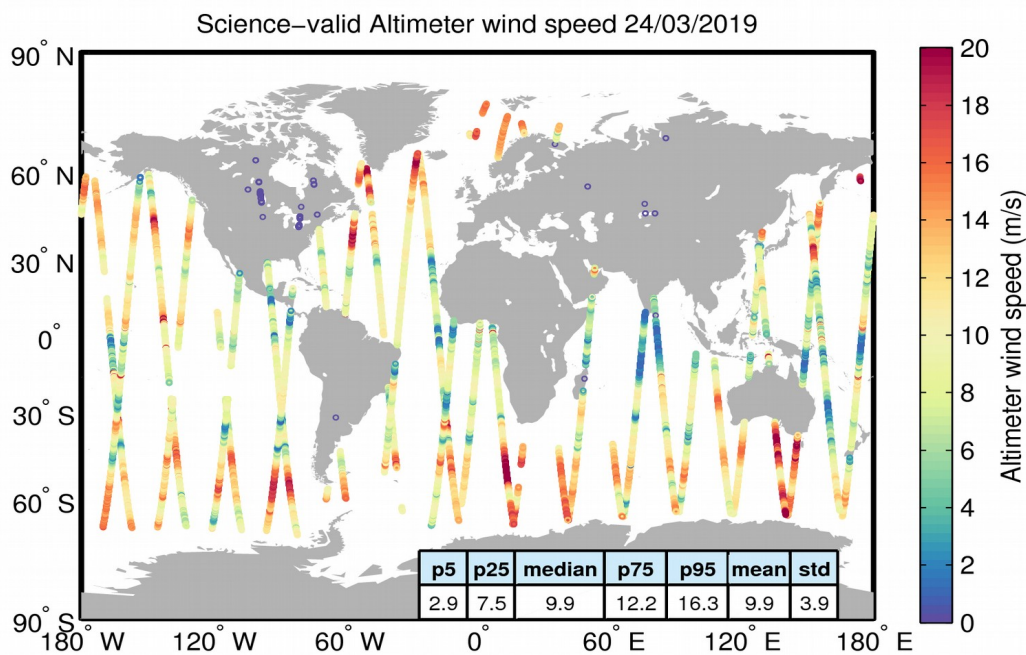
Figure 34. Geographical distribution of science-valid wind data over oceans and lakes for 24/03/2019. The statistical values shown in the table refer to the wind in m/s and are calculated over all measurements shown in the figure. Gray circles denote records that have been rejected based on the editing criteria described in Table 5.
