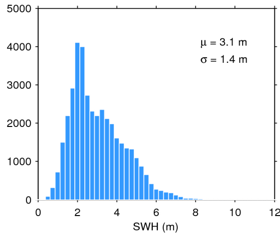
Figure 20. Histogram of science-valid SWH over oceans and lakes for 24/03/2019. The mean ( \mu ) and standard deviation ( \sigma ) are also shown. Note that values larger than 12 m are excluded from the histogram for the sake of readability but not from the computation of \mu and \sigma .
