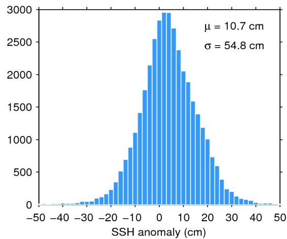
Figure 7. Histogram of flag-valid SSH anomaly over oceans and lakes for 24/03/2019. The mean ( \mu ) and standard deviation ( \sigma ) are also shown. Note that values outside [-50 50] cm are excluded from the histogram for the sake of readability but not from the computation of \mu and \sigma .
