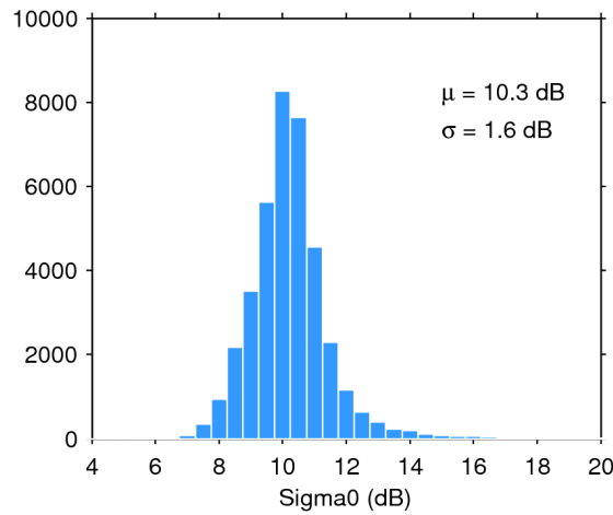
Figure 28. Histogram of science-valid sigma0 over oceans and lakes for 24/03/2019. The mean ( \mu ) and standard deviation ( \sigma ) are also shown. Note that values outside [4 20] dB are excluded from the histogram for the sake of readability but not from the computation of \mu and \sigma .
