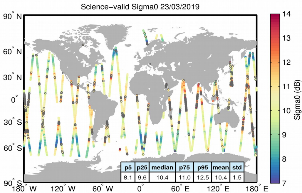
Figure 27. Geographical distribution of science-valid sigma0 data over oceans and lakes for 23/03/2019. The statistical values shown in the table refer to the sigma0 in dB and are calculated over all measurements shown in the figure. Gray circles denote records that have been rejected based on the editing criteria described in Table 4.
