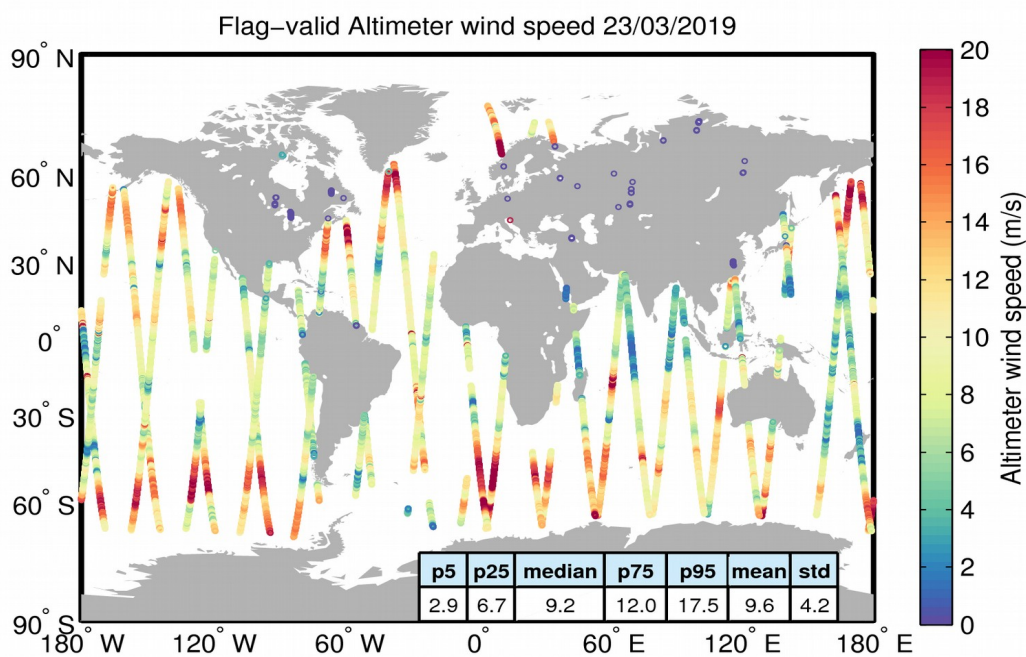
Figure 31. Geographical distribution of flag-valid wind data over oceans and lakes for 23/03/2019. The statistical values shown in the table refer to the wind in m/s and are calculated over all measurements shown in the figure.
