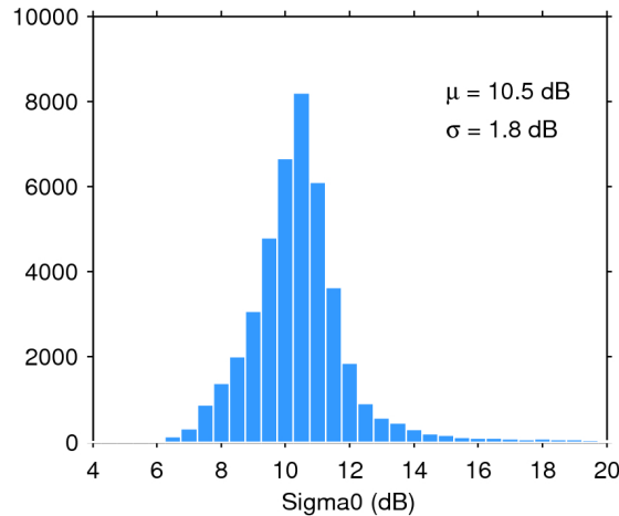
Figure 25. Histogram of flag-valid sigma0 over oceans and lakes for 23/03/2019. The mean ( \mu ) and standard deviation ( \sigma ) are also shown. Note that values outside [4 20] dB are excluded from the histogram for the sake of readability but not from the computation of \mu and \sigma .
