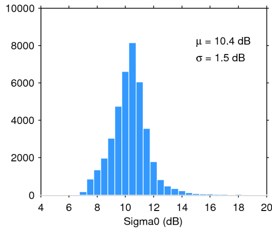
Figure 28. Histogram of science-valid sigma0 over oceans and lakes for 23/03/2019. The mean ( \mu ) and standard deviation ( \sigma ) are also shown. Note that values outside [4 20] dB are excluded from the histogram for the sake of readability but not from the computation of \mu and \sigma .
