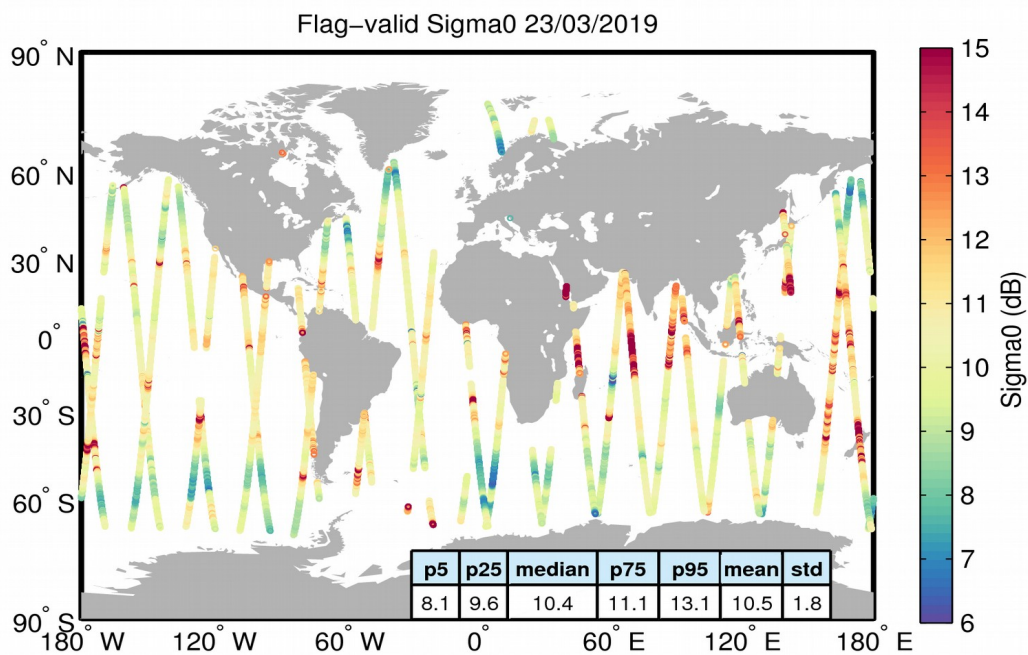
Figure 23. Geographical distribution of flag-valid sigma0 data over oceans and lakes for 23/03/2019. The statistical values shown in the table refer to the sigma0 in dB and are calculated over all measurements shown in the figure.
