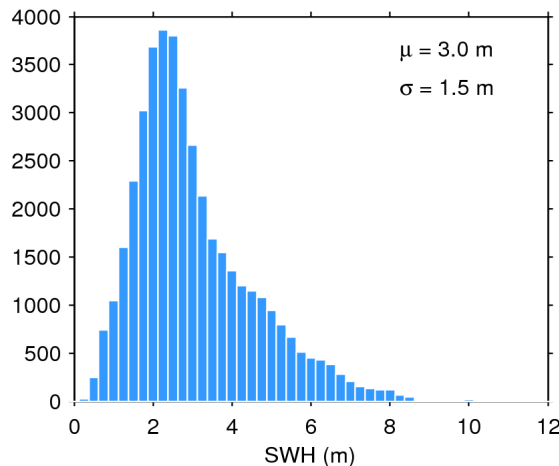
Figure 20. Histogram of science-valid SWH over oceans and lakes for 23/03/2019. The mean ( \mu ) and standard deviation ( \sigma ) are also shown. Note that values larger than 12 m are excluded from the histogram for the sake of readability but not from the computation of \mu and \sigma .
