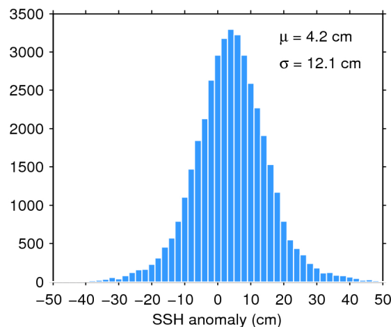
Figure 11. Histogram of science-valid SSH anomaly over oceans and lakes for 23/03/2019. The mean ( \mu ) and standard deviation ( \sigma ) are also shown. Note that values outside [-50 50] cm are excluded from the histogram for the sake of readability but not from the computation of \mu and \sigma .
