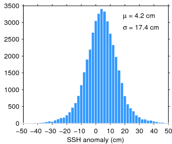
Figure 7. Histogram of flag-valid SSH anomaly over oceans and lakes for 23/03/2019. The mean ( \mu ) and standard deviation ( \sigma ) are also shown. Note that values outside [-50 50] cm are excluded from the histogram for the sake of readability but not from the computation of \mu and \sigma .
