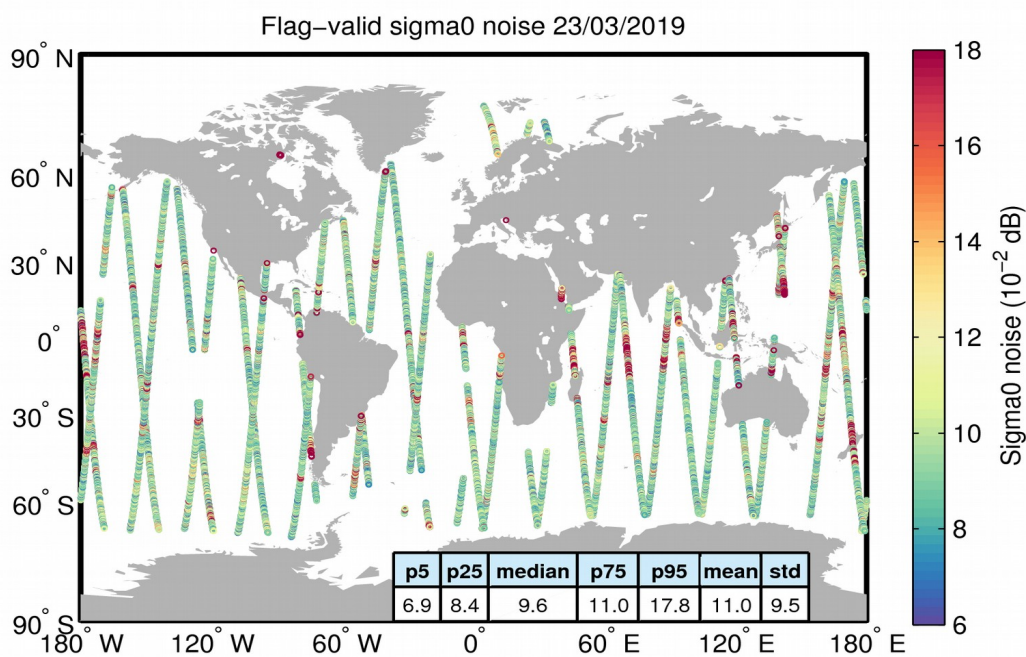
Figure 26. Geographical distribution of flag-valid 20-Hz sigma0 measurement noise over oceans and lakes for 23/03/2019. The statistical values shown in the table refer to the sigma0 noise and are calculated over all measurements shown in the figure.
