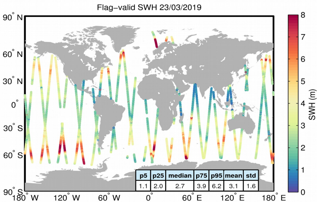
Figure 15. Geographical distribution of flag-valid SWH data over oceans and lakes for 23/03/2019. The statistical values shown in the table refer to the SWH in m and are calculated over all measurements shown in the figure.
