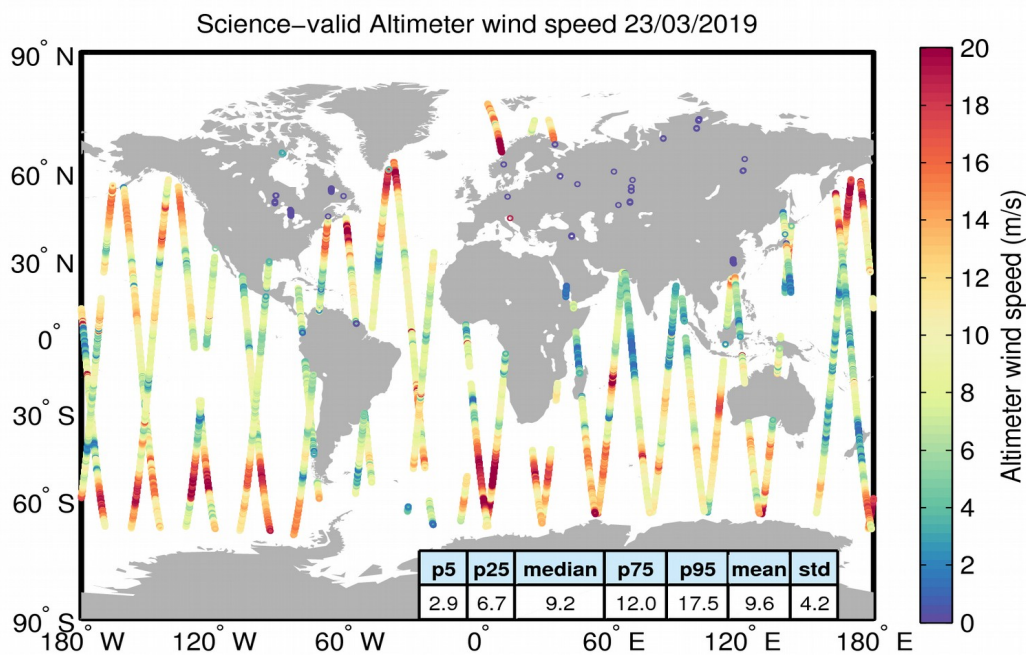
Figure 34. Geographical distribution of science-valid wind data over oceans and lakes for 23/03/2019. The statistical values shown in the table refer to the wind in m/s and are calculated over all measurements shown in the figure. Gray circles denote records that have been rejected based on the editing criteria described in Table 5.
