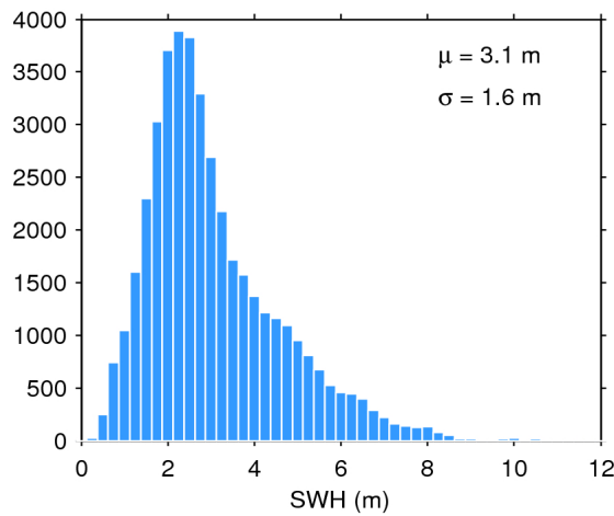
Figure 17. Histogram of flag-valid SWH over oceans and lakes for 23/03/2019. The mean ( \mu ) and standard deviation ( \sigma ) are also shown. Note that values larger than 12 m are excluded from the histogram for the sake of readability but not from the computation of \mu and \sigma .
