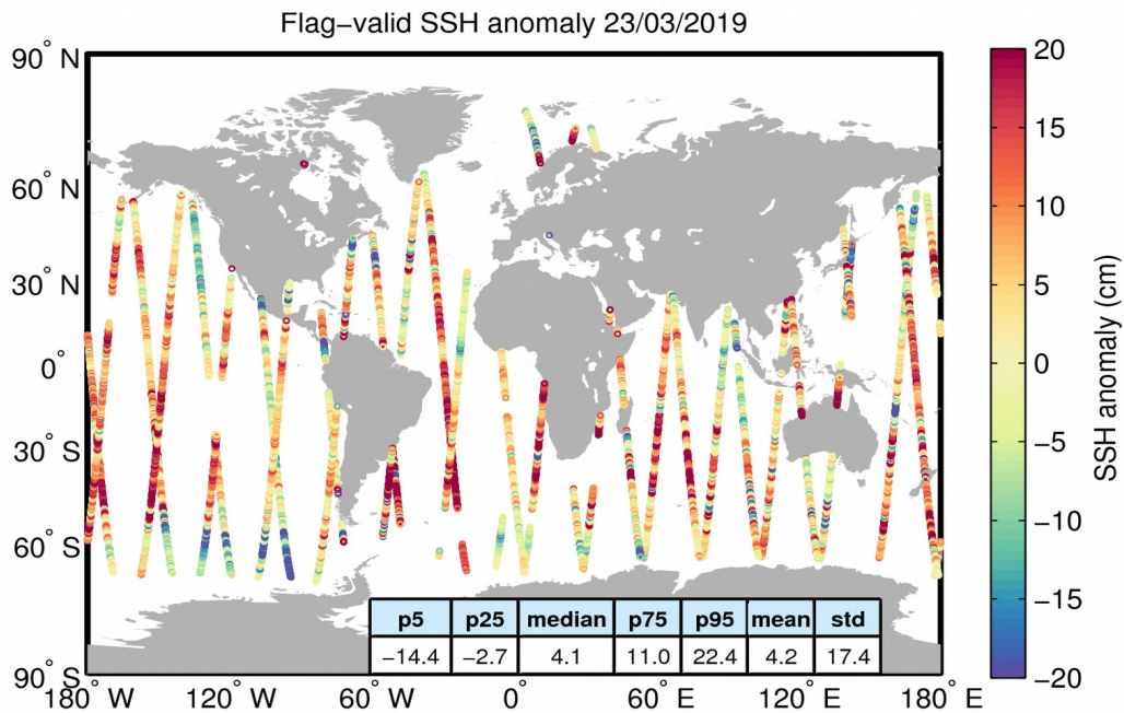
Figure 5. Geographical distribution of flag-valid 1-Hz SSH anomaly data over oceans and lakes for 23/03/2019. The statistical values shown in the table refer to the SSH anomaly in cm and are calculated over all measurements shown in the figure.
