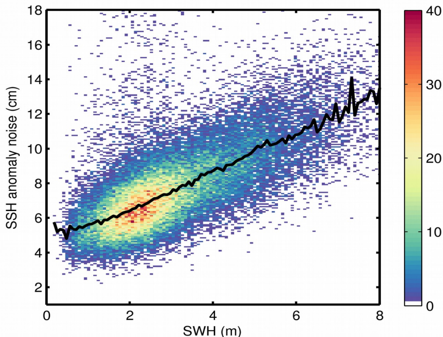
Figure 9. 2D histogram showing flag-valid SSH anomaly noise as a function of SWH for 23/03/2019. The black line denotes the median SSH anomaly noise as a function of SWH.
