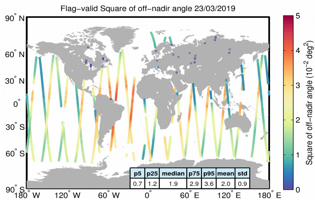
Figure 37. Geographical distribution of flag-valid mispointing data over oceans and lakes for 23/03/2019. The statistical values shown in the table refer to the mispointing in 10^{-2} deg 2 and are calculated over all measurements shown in the figure.
