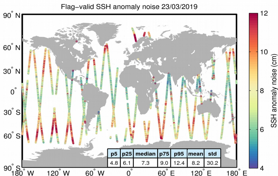
Figure 8. Geographical distribution of flag-valid 20-Hz SSH anomaly measurement noise over oceans and lakes for 23/03/2019. The statistical values shown in the table refer to the SSH anomaly noise and are calculated over all measurements shown in the figure.
