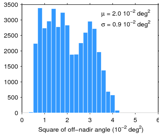
Figure 39. Histogram of flag-valid mispointing over oceans and lakes for 23/03/2019. The mean ( \mu ) and standard deviation ( \sigma ) are also shown. Note that values larger than 6 \cdot 10^{-2} \text{ deg}^2 are excluded from the histogram for the sake of readability but not from the computation of \mu and \sigma .
