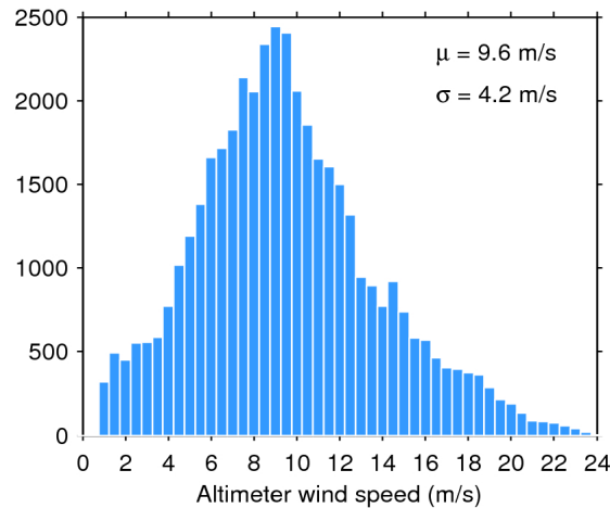
Figure 33. Histogram of flag-valid wind over oceans and lakes for 23/03/2019. The mean ( \mu ) and standard deviation ( \sigma ) are also shown. Note that values larger than 24 m/s are excluded from the histogram for the sake of readability but not from the computation of \mu and \sigma .
