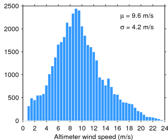
Figure 35. Histogram of science-valid wind over oceans and lakes for 23/03/2019. The mean ( \mu ) and standard deviation ( \sigma ) are also shown. Note that values larger than 24 m/s are excluded from the histogram for the sake of readability but not from the computation of \mu and \sigma .
