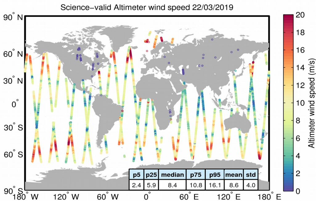
Figure 34. Geographical distribution of science-valid wind data over oceans and lakes for 22/03/2019. The statistical values shown in the table refer to the wind in m/s and are calculated over all measurements shown in the figure. Gray circles denote records that have been rejected based on the editing criteria described in Table 5.
