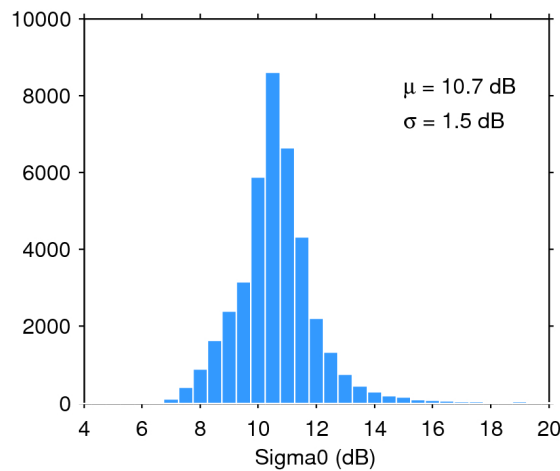
Figure 28. Histogram of science-valid sigma0 over oceans and lakes for 22/03/2019. The mean ( \mu ) and standard deviation ( \sigma ) are also shown. Note that values outside [4 20] dB are excluded from the histogram for the sake of readability but not from the computation of \mu and \sigma .
