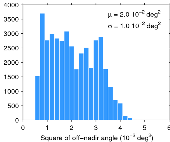
Figure 39. Histogram of flag-valid mispointing over oceans and lakes for 22/03/2019. The mean ( \mu ) and standard deviation ( \sigma ) are also shown. Note that values larger than 6 \cdot 10^{-2} \text{ deg}^2 are excluded from the histogram for the sake of readability but not from the computation of \mu and \sigma .
