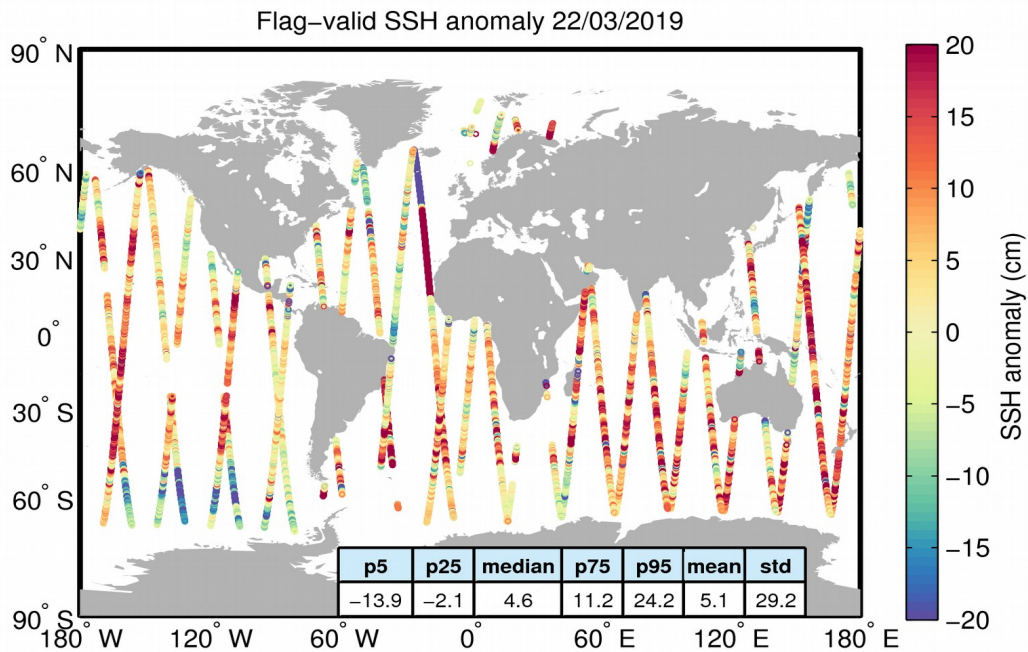
Figure 5. Geographical distribution of flag-valid 1-Hz SSH anomaly data over oceans and lakes for 22/03/2019. The statistical values shown in the table refer to the SSH anomaly in cm and are calculated over all measurements shown in the figure.
