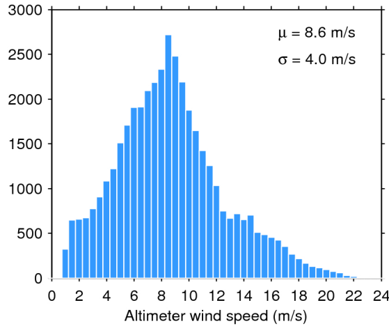
Figure 33. Histogram of flag-valid wind over oceans and lakes for 22/03/2019. The mean ( \mu ) and standard deviation ( \sigma ) are also shown. Note that values larger than 24 m/s are excluded from the histogram for the sake of readability but not from the computation of \mu and \sigma .
