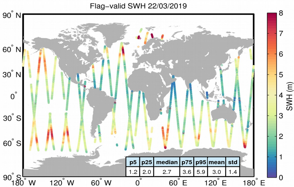
Figure 15. Geographical distribution of flag-valid SWH data over oceans and lakes for 22/03/2019. The statistical values shown in the table refer to the SWH in m and are calculated over all measurements shown in the figure.
