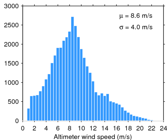
Figure 35. Histogram of science-valid wind over oceans and lakes for 22/03/2019. The mean ( \mu ) and standard deviation ( \sigma ) are also shown. Note that values larger than 24 m/s are excluded from the histogram for the sake of readability but not from the computation of \mu and \sigma .
