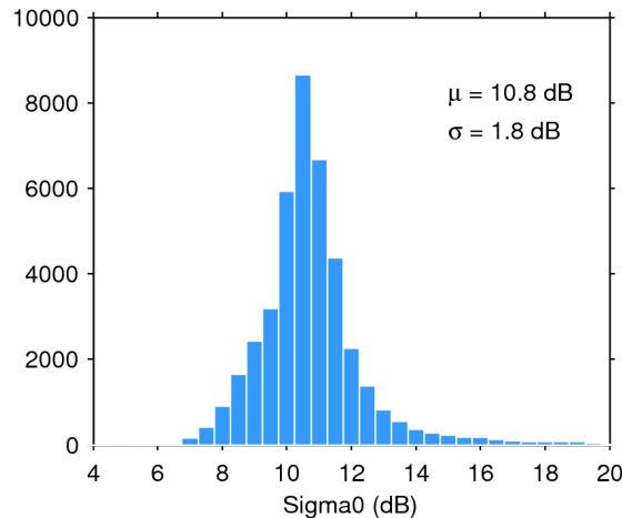
Figure 25. Histogram of flag-valid sigma0 over oceans and lakes for 22/03/2019. The mean ( \mu ) and standard deviation ( \sigma ) are also shown. Note that values outside [4 20] dB are excluded from the histogram for the sake of readability but not from the computation of \mu and \sigma .
