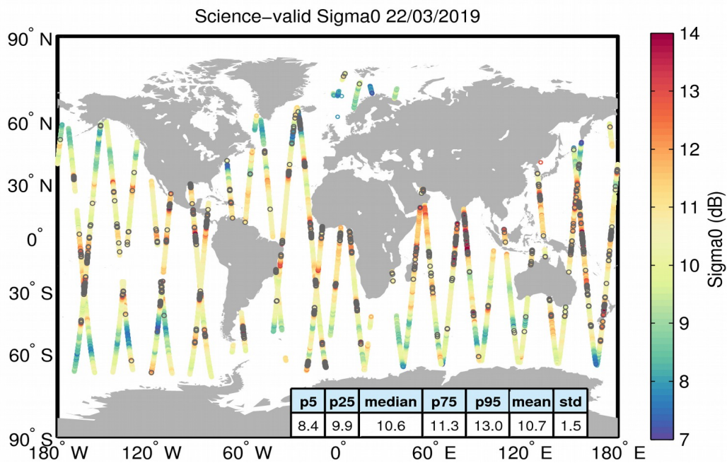
Figure 27. Geographical distribution of science-valid sigma0 data over oceans and lakes for 22/03/2019. The statistical values shown in the table refer to the sigma0 in dB and are calculated over all measurements shown in the figure. Gray circles denote records that have been rejected based on the editing criteria described in Table 4.
