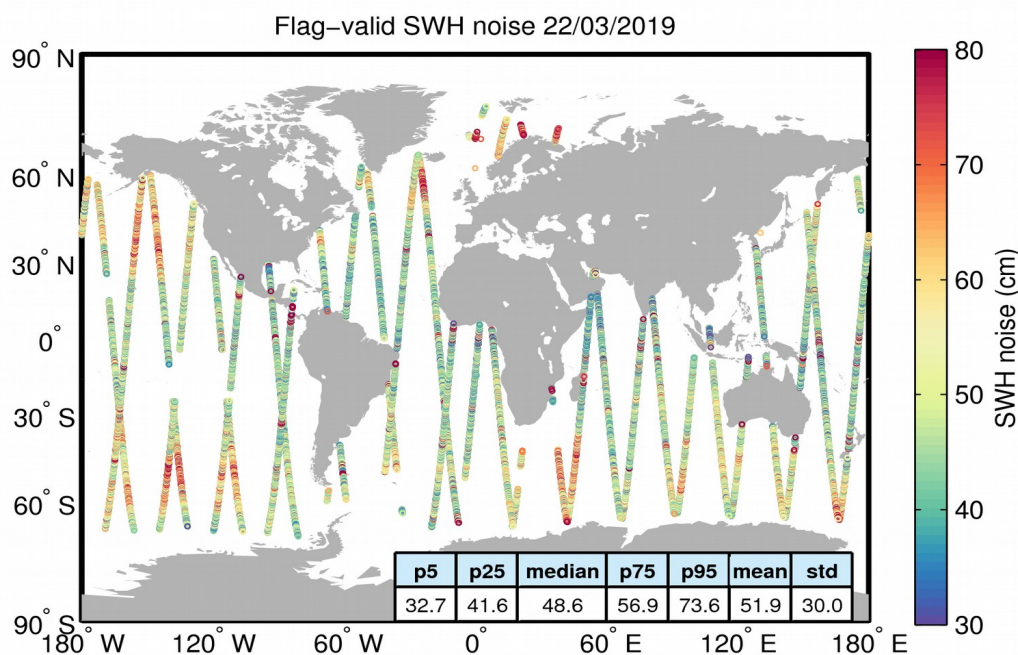
Figure 18. Geographical distribution of flag-valid 20-Hz SWH measurement noise over oceans and lakes for 22/03/2019. The statistical values shown in the figure refer to the SWH noise and are calculated over all measurements shown in the figure.
