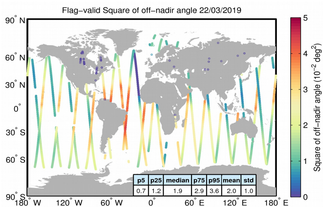
Figure 37. Geographical distribution of flag-valid mispointing data over oceans and lakes for 22/03/2019. The statistical values shown in the table refer to the mispointing in 10^{-2} deg 2 and are calculated over all measurements shown in the figure.
