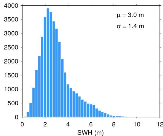
Figure 17. Histogram of flag-valid SWH over oceans and lakes for 22/03/2019. The mean ( \mu ) and standard deviation ( \sigma ) are also shown. Note that values larger than 12 m are excluded from the histogram for the sake of readability but not from the computation of \mu and \sigma .
