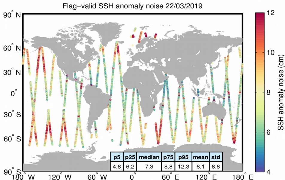
Figure 8. Geographical distribution of flag-valid 20-Hz SSH anomaly measurement noise over oceans and lakes for 22/03/2019. The statistical values shown in the table refer to the SSH anomaly noise and are calculated over all measurements shown in the figure.
