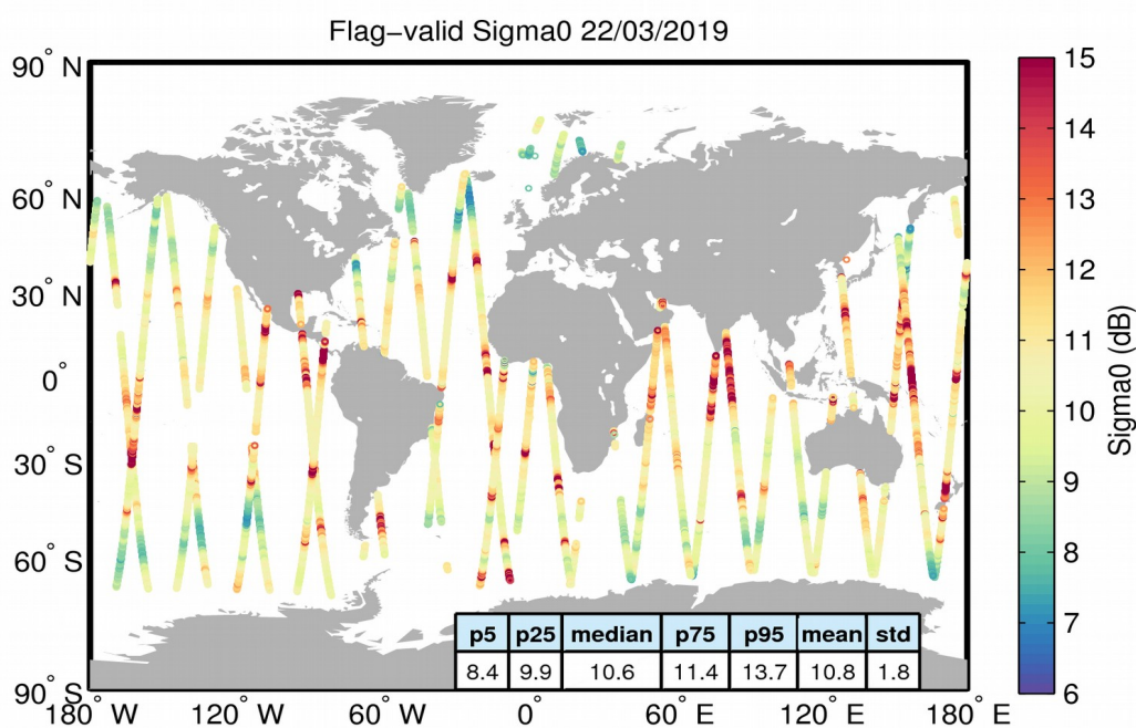
Figure 23. Geographical distribution of flag-valid sigma0 data over oceans and lakes for 22/03/2019. The statistical values shown in the table refer to the sigma0 in dB and are calculated over all measurements shown in the figure.
