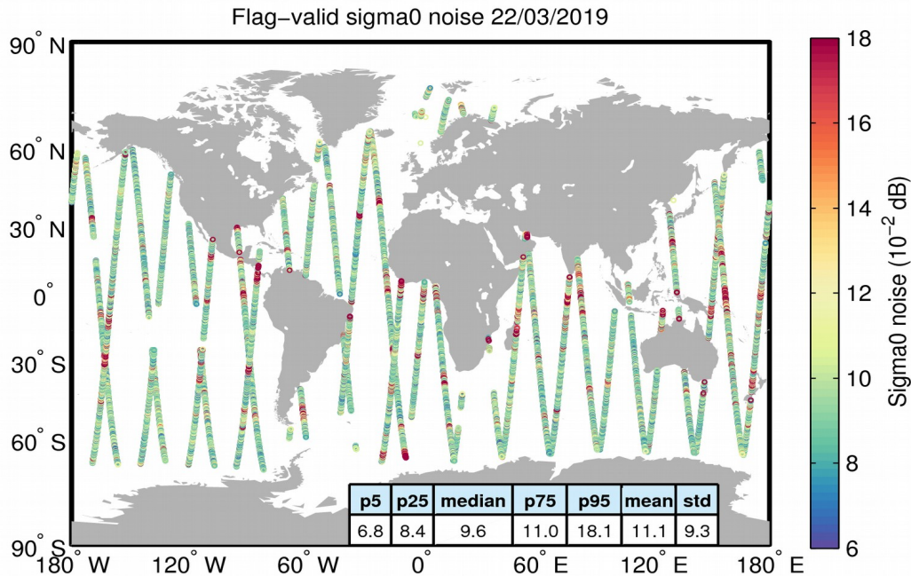
Figure 26. Geographical distribution of flag-valid 20-Hz sigma0 measurement noise over oceans and lakes for 22/03/2019. The statistical values shown in the table refer to the sigma0 noise and are calculated over all measurements shown in the figure.
