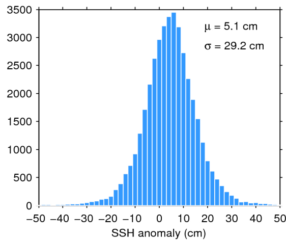
Figure 7. Histogram of flag-valid SSH anomaly over oceans and lakes for 22/03/2019. The mean ( \mu ) and standard deviation ( \sigma ) are also shown. Note that values outside [-50\ 50] cm are excluded from the histogram for the sake of readability but not from the computation of \mu and \sigma .
