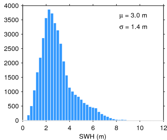
Figure 20. Histogram of science-valid SWH over oceans and lakes for 22/03/2019. The mean ( \mu ) and standard deviation ( \sigma ) are also shown. Note that values larger than 12 m are excluded from the histogram for the sake of readability but not from the computation of \mu and \sigma .
