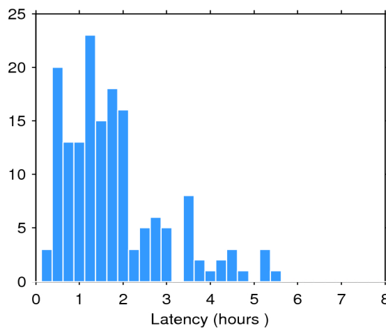
Figure 2. Histogram of the data latency for 22/03/2019. The y-axis denotes the number of files that are made available with a delay of x-hours with respect to the mean time of the records stored in the file.
