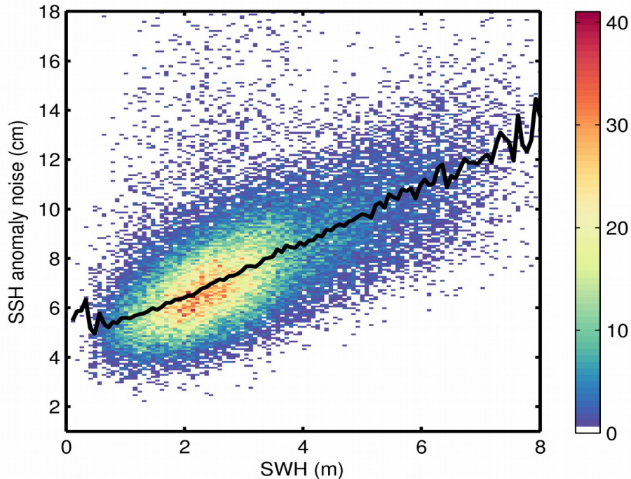
Figure 9. 2D histogram showing flag-valid SSH anomaly noise as a function of SWH for 22/03/2019. The black line denotes the median SSH anomaly noise as a function of SWH.
