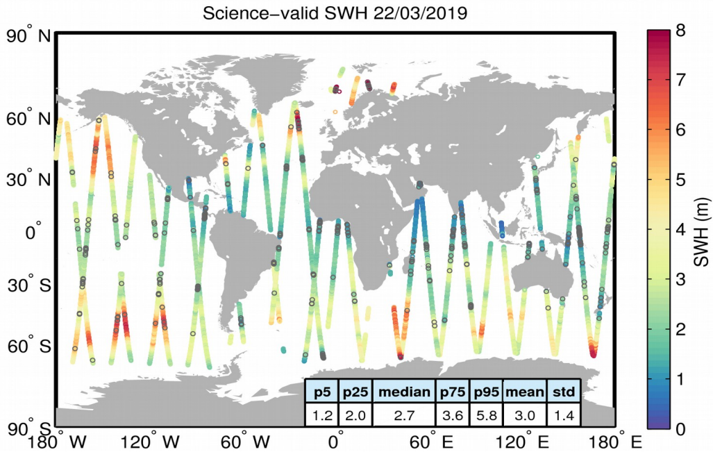
Figure 19. Geographical distribution of science-valid SWH data over oceans and lakes for 22/03/2019. The statistical values shown in the table refer to the SWH in m and are calculated over all measurements shown in the figure. Gray circles denote records that have been rejected based on the editing criteria described in Table 3.
