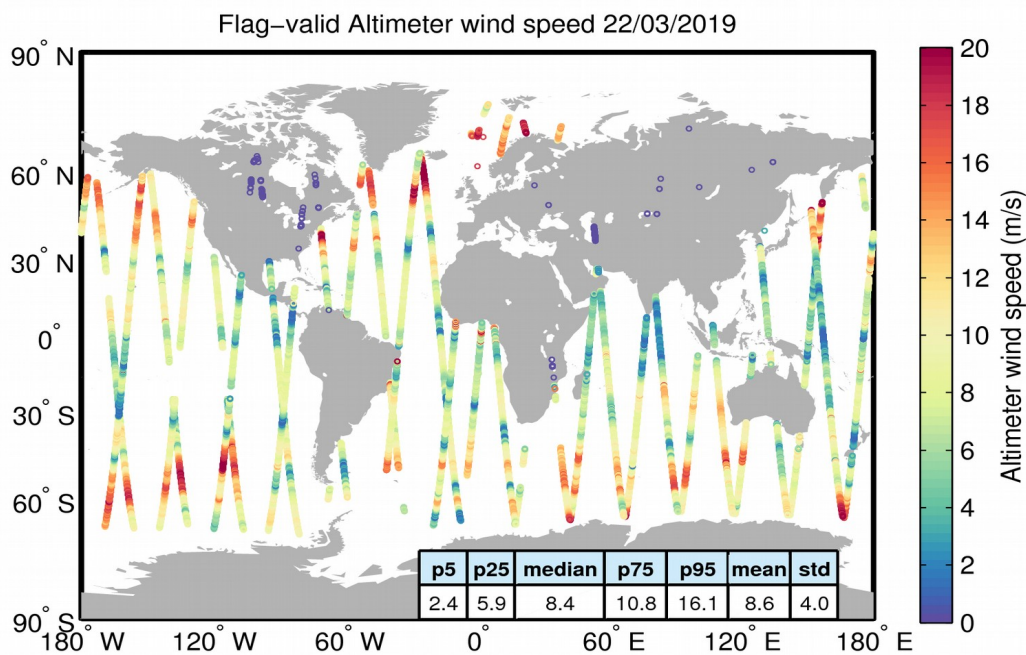
Figure 31. Geographical distribution of flag-valid wind data over oceans and lakes for 22/03/2019. The statistical values shown in the table refer to the wind in m/s and are calculated over all measurements shown in the figure.
