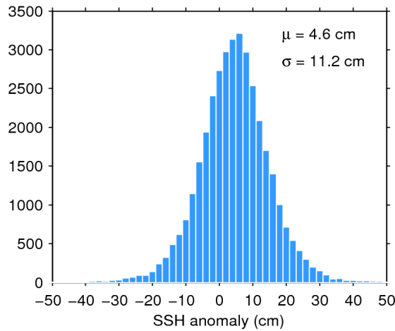
Figure 11. Histogram of science-valid SSH anomaly over oceans and lakes for 22/03/2019. The mean ( \mu ) and standard deviation ( \sigma ) are also shown. Note that values outside [-50 50] cm are excluded from the histogram for the sake of readability but not from the computation of \mu and \sigma .
