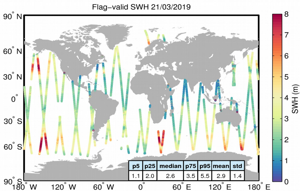
Figure 15. Geographical distribution of flag-valid SWH data over oceans and lakes for 21/03/2019. The statistical values shown in the table refer to the SWH in m and are calculated over all measurements shown in the figure.
