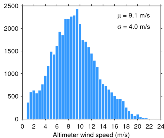
Figure 35. Histogram of science-valid wind over oceans and lakes for 21/03/2019. The mean ( \mu ) and standard deviation ( \sigma ) are also shown. Note that values larger than 24 m/s are excluded from the histogram for the sake of readability but not from the computation of \mu and \sigma .
