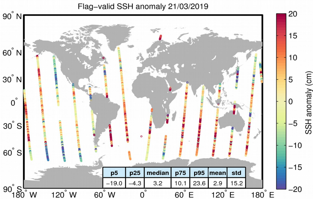
Figure 5. Geographical distribution of flag-valid 1-Hz SSH anomaly data over oceans and lakes for 21/03/2019. The statistical values shown in the table refer to the SSH anomaly in cm and are calculated over all measurements shown in the figure.
