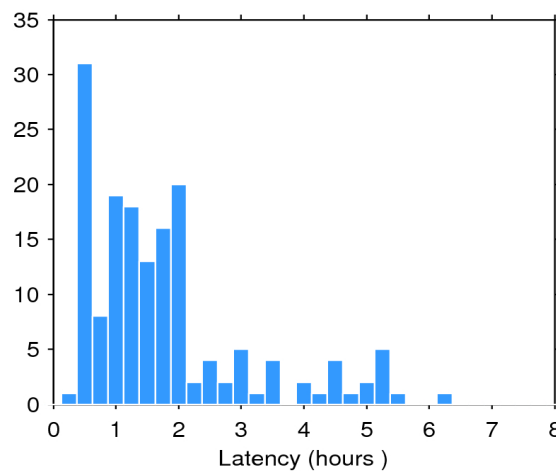
Figure 2. Histogram of the data latency for 21/03/2019. The y-axis denotes the number of files that are made available with a delay of x-hours with respect to the mean time of the records stored in the file.
