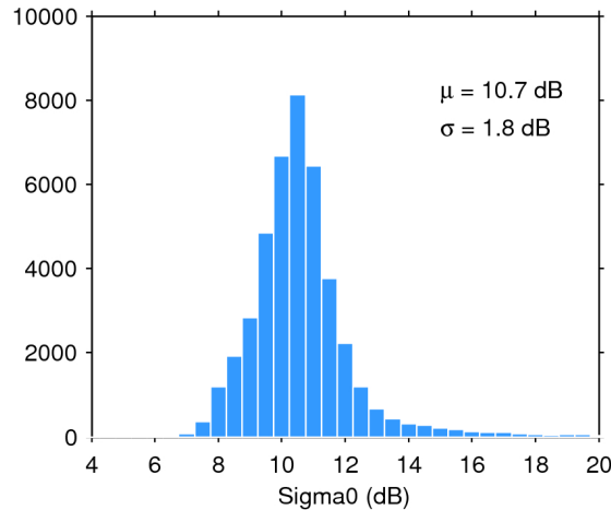
Figure 25. Histogram of flag-valid sigma0 over oceans and lakes for 21/03/2019. The mean ( \mu ) and standard deviation ( \sigma ) are also shown. Note that values outside [4 20] dB are excluded from the histogram for the sake of readability but not from the computation of \mu and \sigma .
