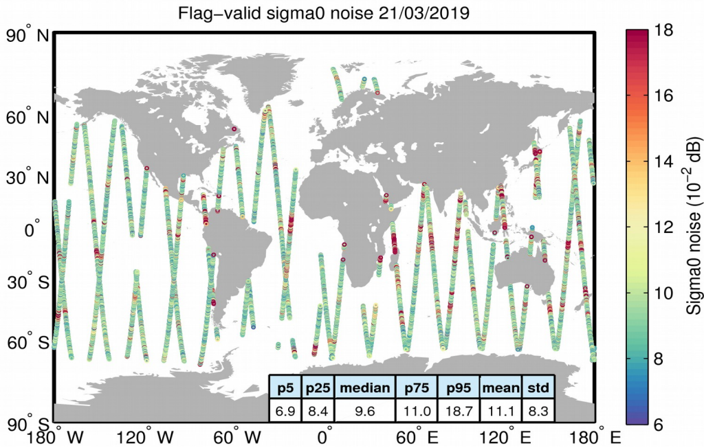
Figure 26. Geographical distribution of flag-valid 20-Hz sigma0 measurement noise over oceans and lakes for 21/03/2019. The statistical values shown in the table refer to the sigma0 noise and are calculated over all measurements shown in the figure.
