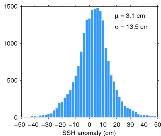
Figure 11. Histogram of science-valid SSH anomaly over oceans and lakes for 21/03/2019. The mean ( \mu ) and standard deviation ( \sigma ) are also shown. Note that values outside [-50 50] cm are excluded from the histogram for the sake of readability but not from the computation of \mu and \sigma .
