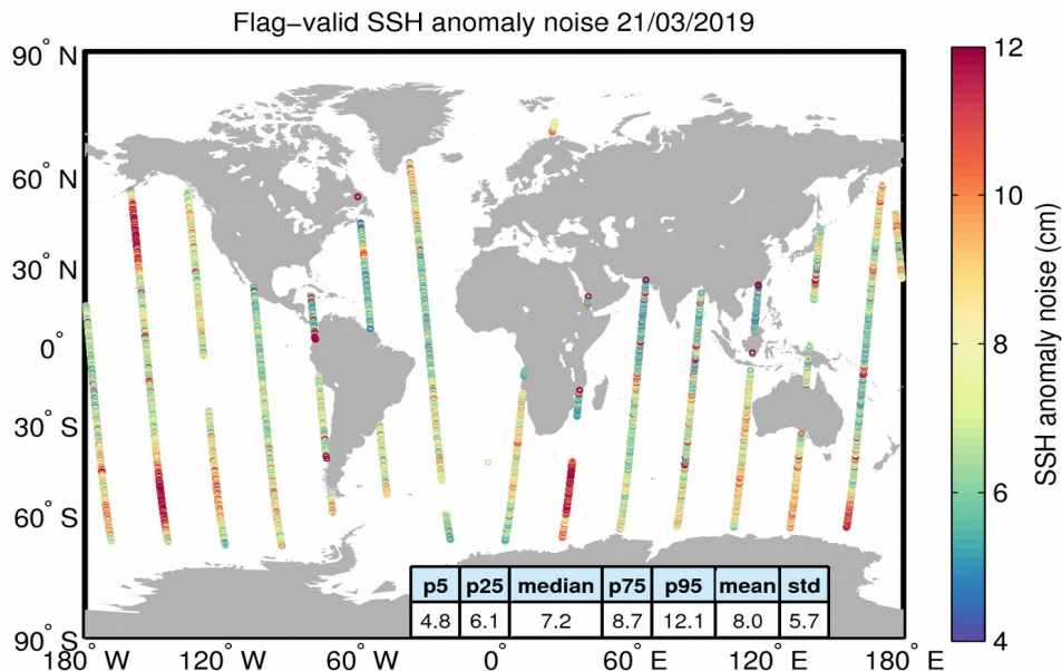
Figure 8. Geographical distribution of flag-valid 20-Hz SSH anomaly measurement noise over oceans and lakes for 21/03/2019. The statistical values shown in the table refer to the SSH anomaly noise and are calculated over all measurements shown in the figure.
