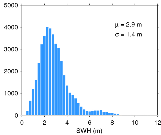
Figure 17. Histogram of flag-valid SWH over oceans and lakes for 21/03/2019. The mean ( \mu ) and standard deviation ( \sigma ) are also shown. Note that values larger than 12 m are excluded from the histogram for the sake of readability but not from the computation of \mu and \sigma .
