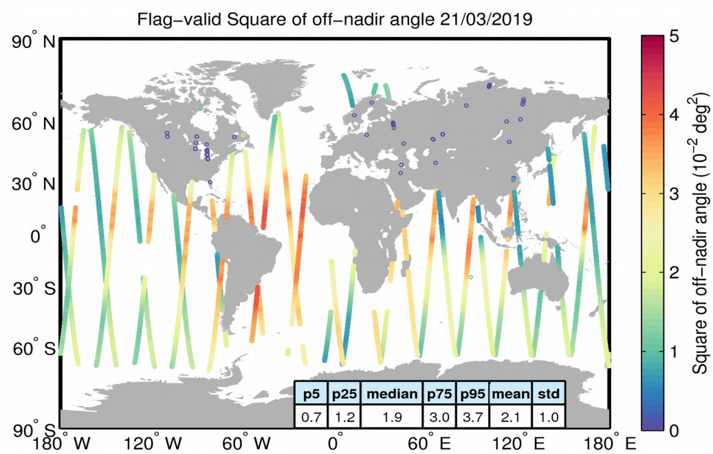
Figure 37. Geographical distribution of flag-valid mispointing data over oceans and lakes for 21/03/2019. The statistical values shown in the table refer to the mispointing in 10^{-2} deg 2 and are calculated over all measurements shown in the figure.
