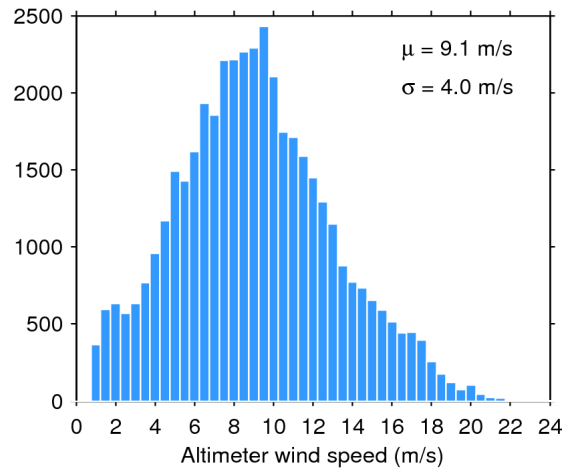
Figure 33. Histogram of flag-valid wind over oceans and lakes for 21/03/2019. The mean ( \mu ) and standard deviation ( \sigma ) are also shown. Note that values larger than 24 m/s are excluded from the histogram for the sake of readability but not from the computation of \mu and \sigma .
