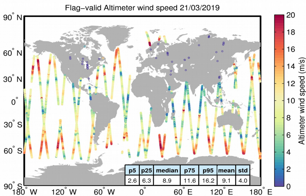
Figure 31. Geographical distribution of flag-valid wind data over oceans and lakes for 21/03/2019. The statistical values shown in the table refer to the wind in m/s and are calculated over all measurements shown in the figure.
