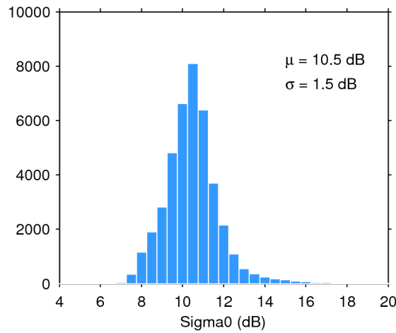
Figure 28. Histogram of science-valid sigma0 over oceans and lakes for 21/03/2019. The mean ( \mu ) and standard deviation ( \sigma ) are also shown. Note that values outside [4 20] dB are excluded from the histogram for the sake of readability but not from the computation of \mu and \sigma .
