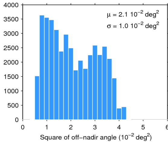
Figure 39. Histogram of flag-valid mispointing over oceans and lakes for 21/03/2019. The mean ( \mu ) and standard deviation ( \sigma ) are also shown. Note that values larger than 6 \cdot 10^{-2} \text{ deg}^2 are excluded from the histogram for the sake of readability but not from the computation of \mu and \sigma .
