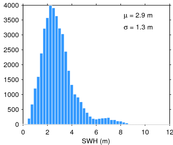
Figure 20. Histogram of science-valid SWH over oceans and lakes for 21/03/2019. The mean ( \mu ) and standard deviation ( \sigma ) are also shown. Note that values larger than 12 m are excluded from the histogram for the sake of readability but not from the computation of \mu and \sigma .
