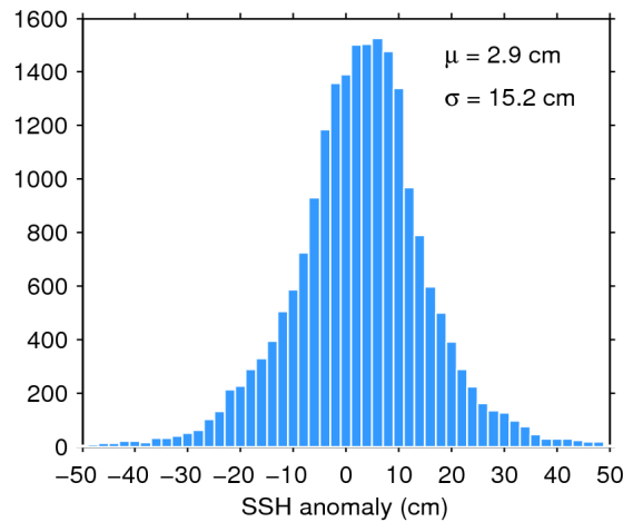
Figure 7. Histogram of flag-valid SSH anomaly over oceans and lakes for 21/03/2019. The mean ( \mu ) and standard deviation ( \sigma ) are also shown. Note that values outside [-50 50] cm are excluded from the histogram for the sake of readability but not from the computation of \mu and \sigma .
