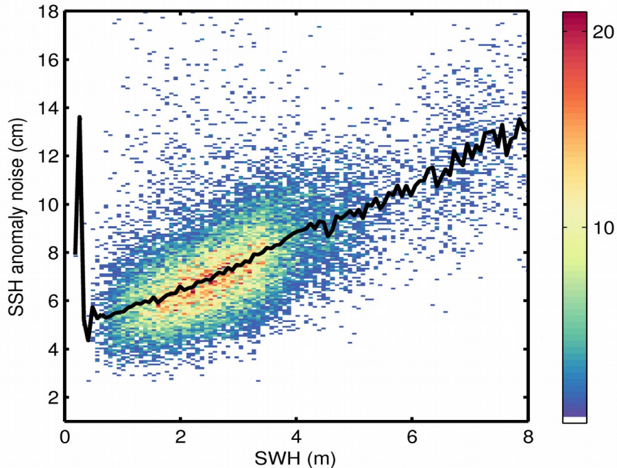
Figure 9. 2D histogram showing flag-valid SSH anomaly noise as a function of SWH for 21/03/2019. The black line denotes the median SSH anomaly noise as a function of SWH.
