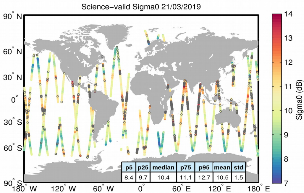
Figure 27. Geographical distribution of science-valid sigma0 data over oceans and lakes for 21/03/2019. The statistical values shown in the table refer to the sigma0 in dB and are calculated over all measurements shown in the figure. Gray circles denote records that have been rejected based on the editing criteria described in Table 4.
