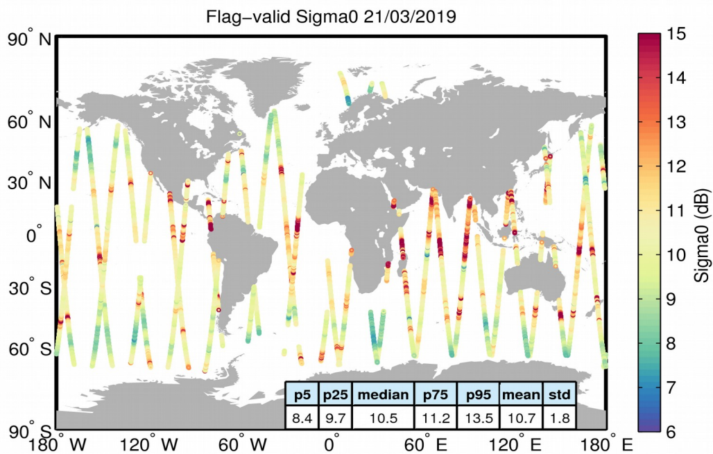
Figure 23. Geographical distribution of flag-valid sigma0 data over oceans and lakes for 21/03/2019. The statistical values shown in the table refer to the sigma0 in dB and are calculated over all measurements shown in the figure.
