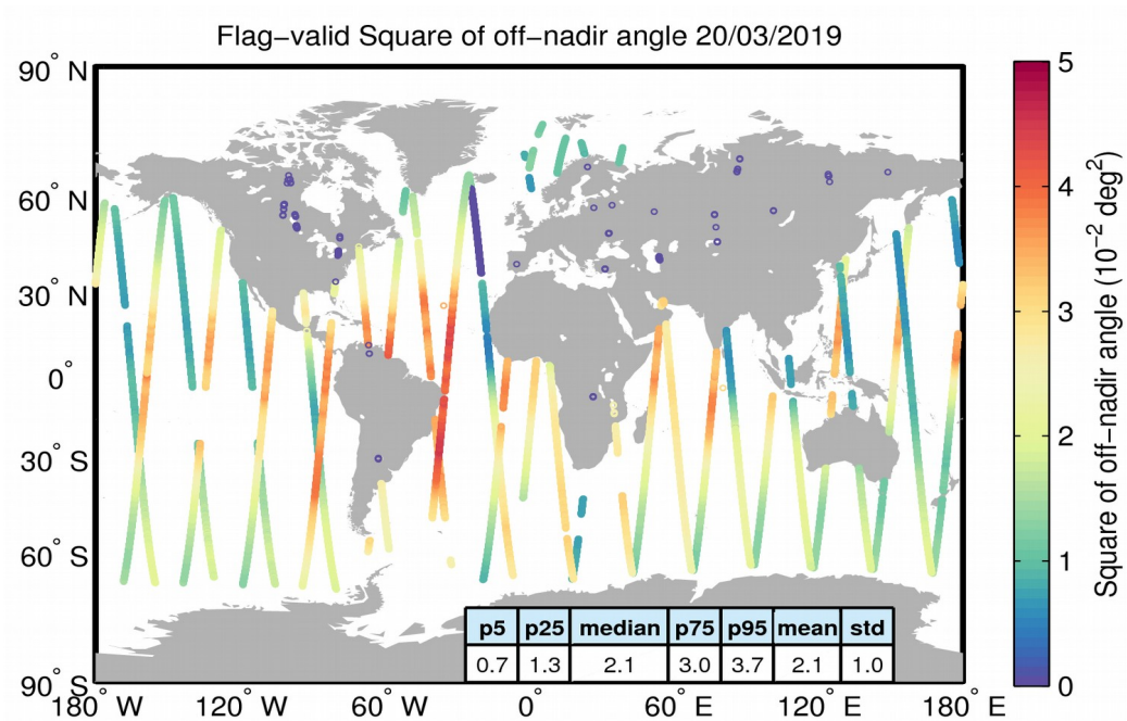
Figure 37. Geographical distribution of flag-valid mispointing data over oceans and lakes for 20/03/2019. The statistical values shown in the table refer to the mispointing in 10^{-2} \text{ deg}^2 and are calculated over all measurements shown in the figure.
