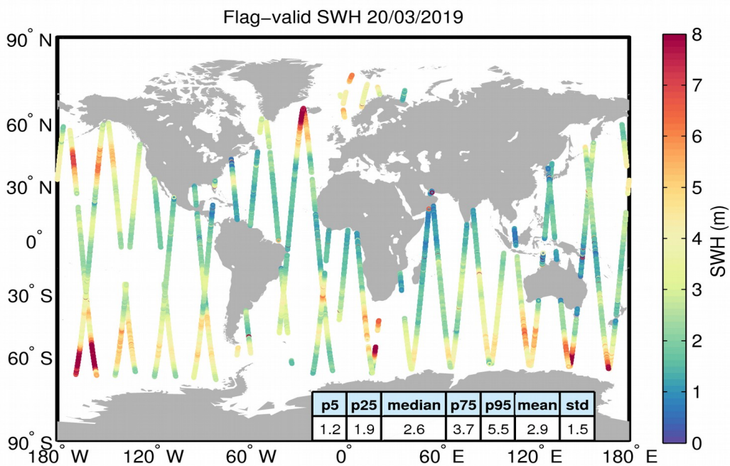
Figure 15. Geographical distribution of flag-valid SWH data over oceans and lakes for 20/03/2019. The statistical values shown in the table refer to the SWH in m and are calculated over all measurements shown in the figure.
