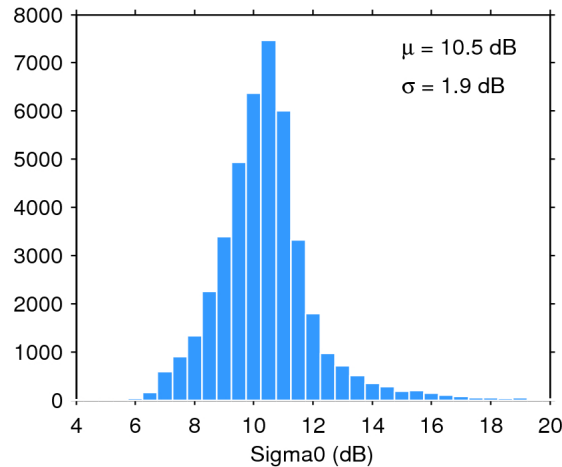
Figure 25. Histogram of flag-valid sigma0 over oceans and lakes for 20/03/2019. The mean ( \mu ) and standard deviation ( \sigma ) are also shown. Note that values outside [4 20] dB are excluded from the histogram for the sake of readability but not from the computation of \mu and \sigma .
