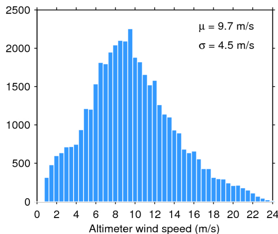
Figure 35. Histogram of science-valid wind over oceans and lakes for 20/03/2019. The mean ( \mu ) and standard deviation ( \sigma ) are also shown. Note that values larger than 24 m/s are excluded from the histogram for the sake of readability but not from the computation of \mu and \sigma .
