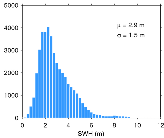
Figure 17. Histogram of flag-valid SWH over oceans and lakes for 20/03/2019. The mean ( \mu ) and standard deviation ( \sigma ) are also shown. Note that values larger than 12 m are excluded from the histogram for the sake of readability but not from the computation of \mu and \sigma .
