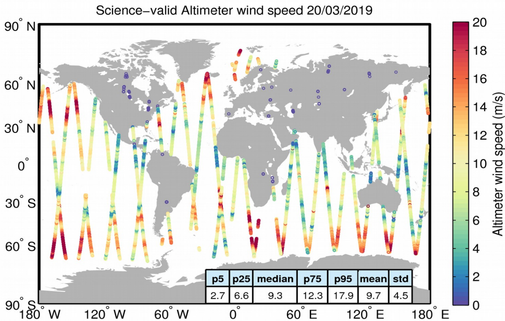
Figure 34. Geographical distribution of science-valid wind data over oceans and lakes for 20/03/2019. The statistical values shown in the table refer to the wind in m/s and are calculated over all measurements shown in the figure. Gray circles denote records that have been rejected based on the editing criteria described in Table 5.
