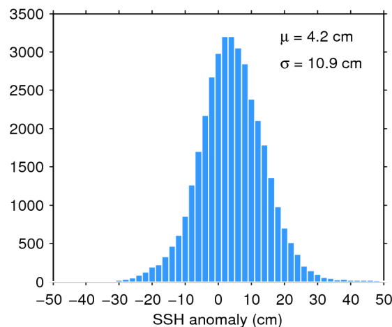
Figure 11. Histogram of science-valid SSH anomaly over oceans and lakes for 20/03/2019. The mean ( \mu ) and standard deviation ( \sigma ) are also shown. Note that values outside [-50 50] cm are excluded from the histogram for the sake of readability but not from the computation of \mu and \sigma .
