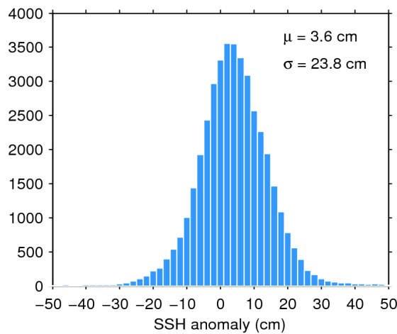
Figure 7. Histogram of flag-valid SSH anomaly over oceans and lakes for 20/03/2019. The mean ( \mu ) and standard deviation ( \sigma ) are also shown. Note that values outside [-50\ 50] cm are excluded from the histogram for the sake of readability but not from the computation of \mu and \sigma .
