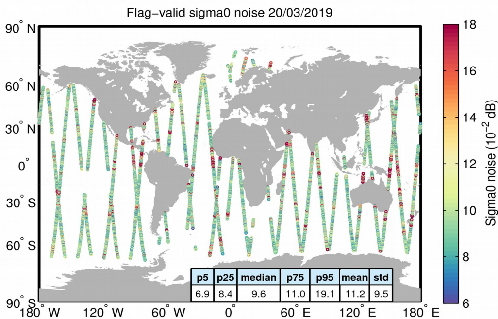
Figure 26. Geographical distribution of flag-valid 20-Hz sigma0 measurement noise over oceans and lakes for 20/03/2019. The statistical values shown in the table refer to the sigma0 noise and are calculated over all measurements shown in the figure.
