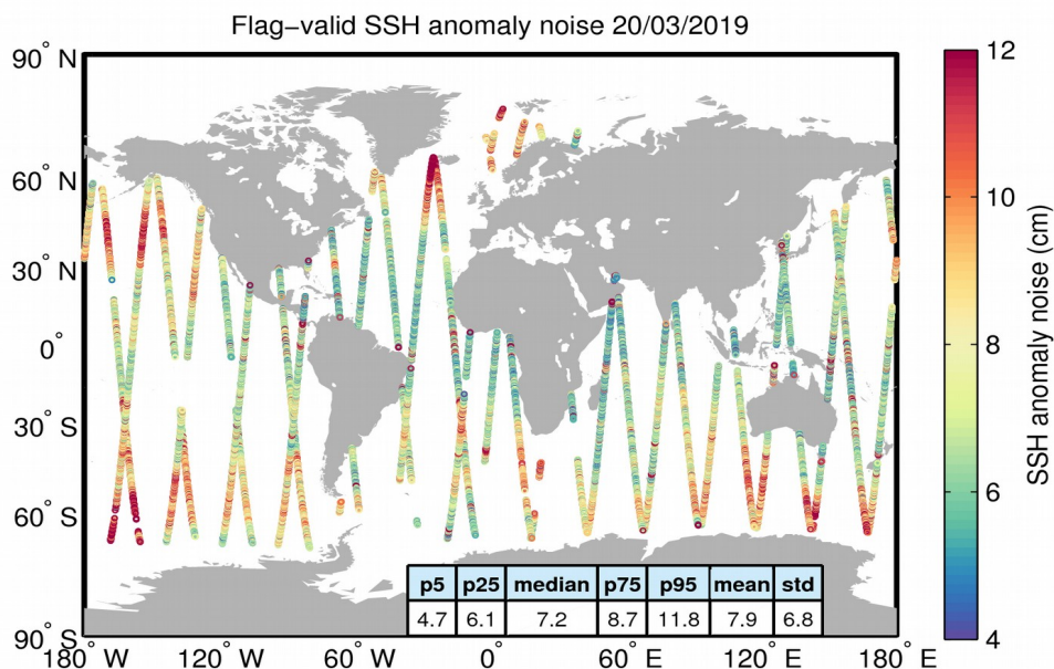
Figure 8. Geographical distribution of flag-valid 20-Hz SSH anomaly measurement noise over oceans and lakes for 20/03/2019. The statistical values shown in the table refer to the SSH anomaly noise and are calculated over all measurements shown in the figure.
