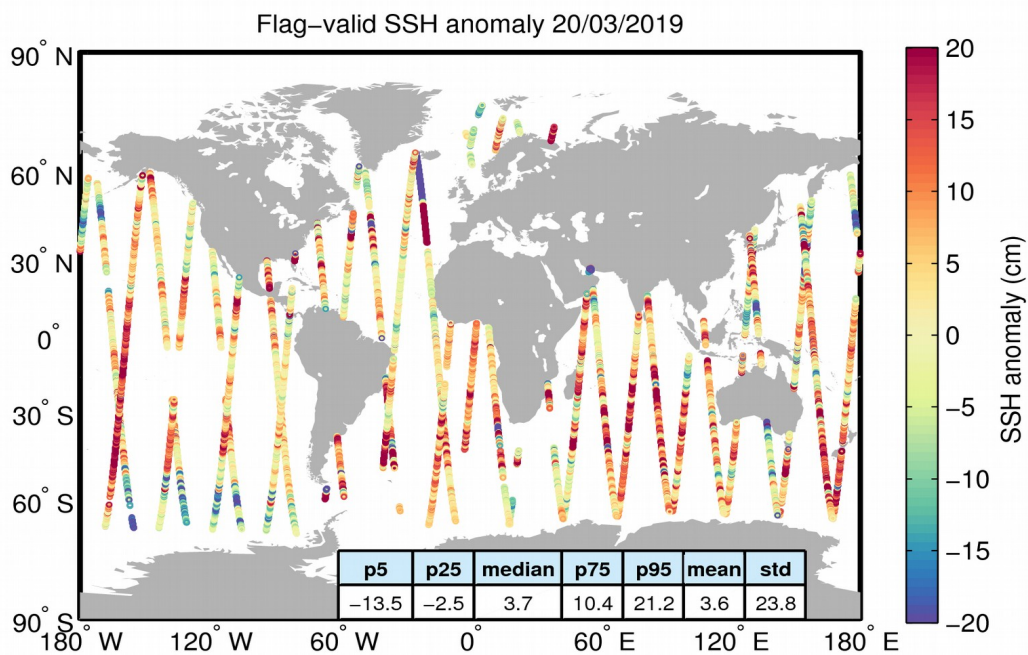
Figure 5. Geographical distribution of flag-valid 1-Hz SSH anomaly data over oceans and lakes for 20/03/2019. The statistical values shown in the table refer to the SSH anomaly in cm and are calculated over all measurements shown in the figure.
