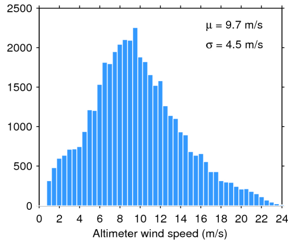
Figure 33. Histogram of flag-valid wind over oceans and lakes for 20/03/2019. The mean ( \mu ) and standard deviation ( \sigma ) are also shown. Note that values larger than 24 m/s are excluded from the histogram for the sake of readability but not from the computation of \mu and \sigma .
