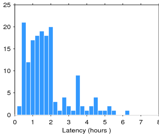
Figure 2. Histogram of the data latency for 20/03/2019. The y-axis denotes the number of files that are made available with a delay of x-hours with respect to the mean time of the records stored in the file.
