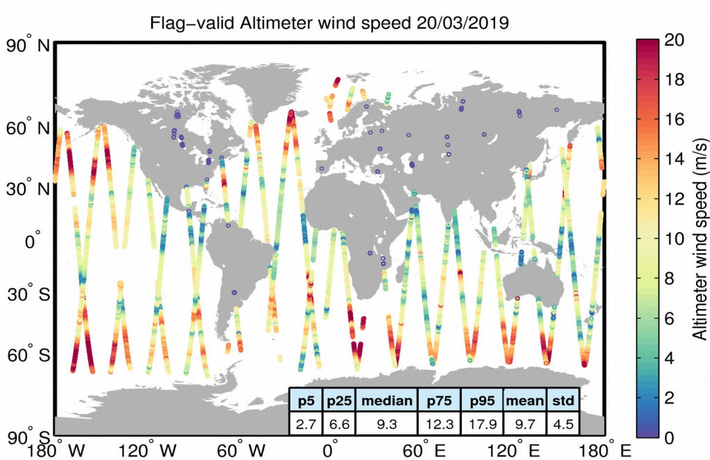
Figure 31. Geographical distribution of flag-valid wind data over oceans and lakes for 20/03/2019. The statistical values shown in the table refer to the wind in m/s and are calculated over all measurements shown in the figure.
