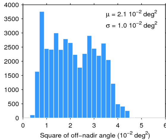
Figure 39. Histogram of flag-valid mispointing over oceans and lakes for 20/03/2019. The mean ( \mu ) and standard deviation ( \sigma ) are also shown. Note that values larger than 6 \cdot 10^{-2} \text{ deg}^2 are excluded from the histogram for the sake of readability but not from the computation of \mu and \sigma .
