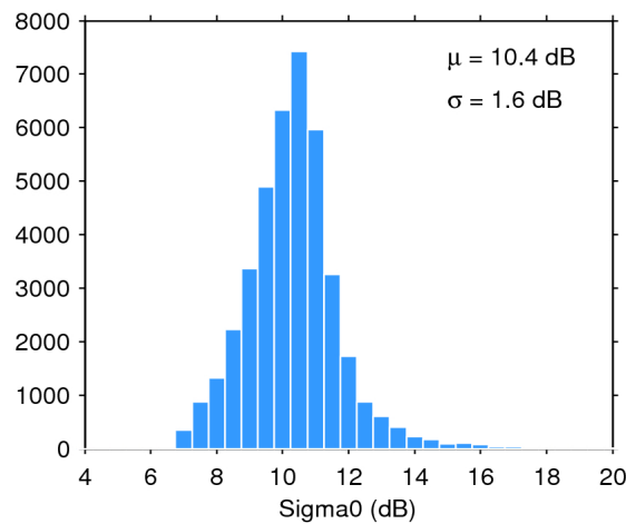
Figure 28. Histogram of science-valid sigma0 over oceans and lakes for 20/03/2019. The mean ( \mu ) and standard deviation ( \sigma ) are also shown. Note that values outside [4 20] dB are excluded from the histogram for the sake of readability but not from the computation of \mu and \sigma .
