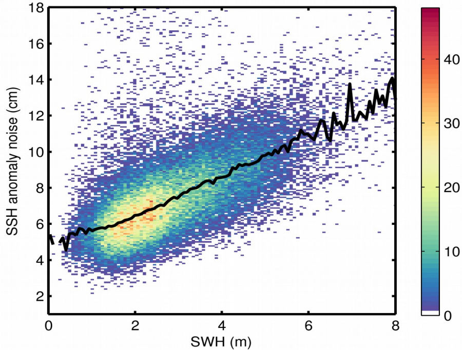
Figure 9. 2D histogram showing flag-valid SSH anomaly noise as a function of SWH for 20/03/2019. The black line denotes the median SSH anomaly noise as a function of SWH.
