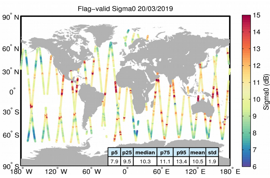
Figure 23. Geographical distribution of flag-valid sigma0 data over oceans and lakes for 20/03/2019. The statistical values shown in the table refer to the sigma0 in dB and are calculated over all measurements shown in the figure.
