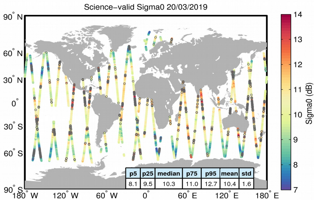
Figure 27. Geographical distribution of science-valid sigma0 data over oceans and lakes for 20/03/2019. The statistical values shown in the table refer to the sigma0 in dB and are calculated over all measurements shown in the figure. Gray circles denote records that have been rejected based on the editing criteria described in Table 4.
