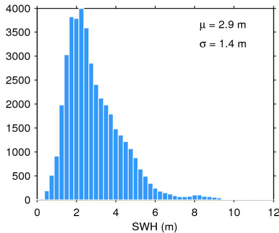
Figure 20. Histogram of science-valid SWH over oceans and lakes for 20/03/2019. The mean ( \mu ) and standard deviation ( \sigma ) are also shown. Note that values larger than 12 m are excluded from the histogram for the sake of readability but not from the computation of \mu and \sigma .
