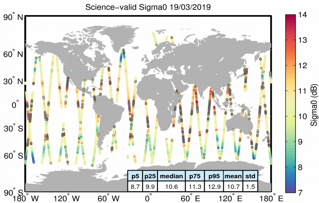
Figure 27. Geographical distribution of science-valid sigma0 data over oceans and lakes for 19/03/2019. The statistical values shown in the table refer to the sigma0 in dB and are calculated over all measurements shown in the figure. Gray circles denote records that have been rejected based on the editing criteria described in Table 4.
