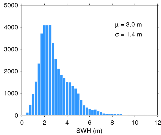
Figure 17. Histogram of flag-valid SWH over oceans and lakes for 19/03/2019. The mean ( \mu ) and standard deviation ( \sigma ) are also shown. Note that values larger than 12 m are excluded from the histogram for the sake of readability but not from the computation of \mu and \sigma .
