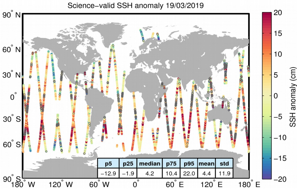
Figure 10. Geographical distribution of science-valid SSH anomaly data over oceans and lakes for 19/03/2019. The statistical values shown in the table refer to the SSH anomaly in cm and are calculated over all measurements shown in the figure. Gray circles denote records that have been rejected based on the editing criteria described in Table 2.
