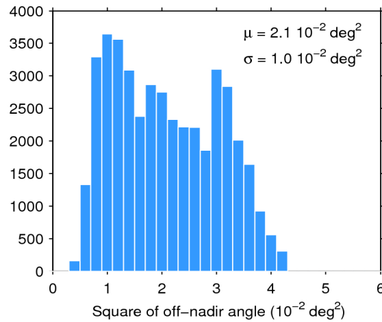
Figure 39. Histogram of flag-valid mispointing over oceans and lakes for 19/03/2019. The mean ( \mu ) and standard deviation ( \sigma ) are also shown. Note that values larger than 6 \cdot 10^{-2} \text{ deg}^2 are excluded from the histogram for the sake of readability but not from the computation of \mu and \sigma .
