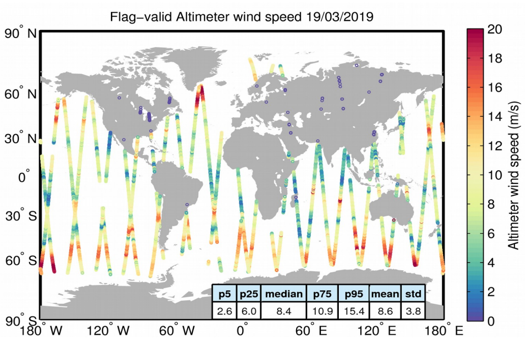
Figure 31. Geographical distribution of flag-valid wind data over oceans and lakes for 19/03/2019. The statistical values shown in the table refer to the wind in m/s and are calculated over all measurements shown in the figure.
