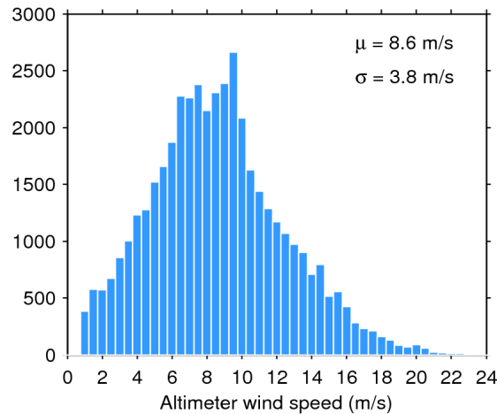
Figure 33. Histogram of flag-valid wind over oceans and lakes for 19/03/2019. The mean ( \mu ) and standard deviation ( \sigma ) are also shown. Note that values larger than 24 m/s are excluded from the histogram for the sake of readability but not from the computation of \mu and \sigma .
