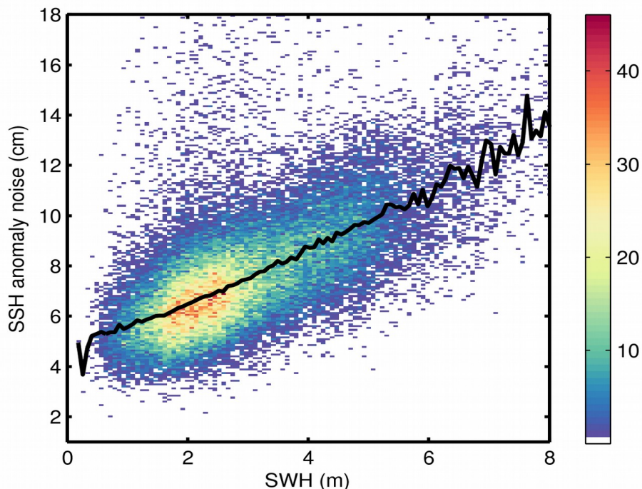
Figure 9. 2D histogram showing flag-valid SSH anomaly noise as a function of SWH for 19/03/2019. The black line denotes the median SSH anomaly noise as a function of SWH.
