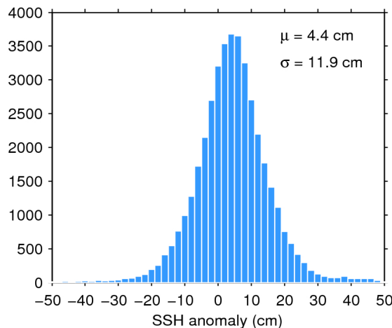
Figure 11. Histogram of science-valid SSH anomaly over oceans and lakes for 19/03/2019. The mean ( \mu ) and standard deviation ( \sigma ) are also shown. Note that values outside [-50 50] cm are excluded from the histogram for the sake of readability but not from the computation of \mu and \sigma .
