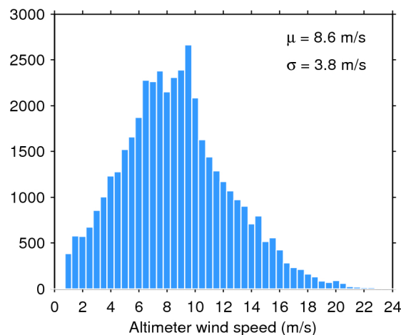
Figure 35. Histogram of science-valid wind over oceans and lakes for 19/03/2019. The mean ( \mu ) and standard deviation ( \sigma ) are also shown. Note that values larger than 24 m/s are excluded from the histogram for the sake of readability but not from the computation of \mu and \sigma .
