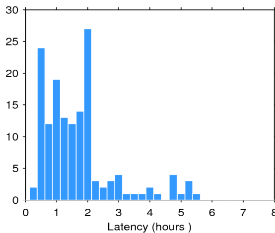
Figure 2. Histogram of the data latency for 19/03/2019. The y-axis denotes the number of files that are made available with a delay of x-hours with respect to the mean time of the records stored in the file.
