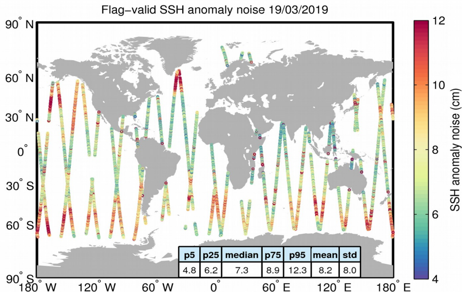
Figure 8. Geographical distribution of flag-valid 20-Hz SSH anomaly measurement noise over oceans and lakes for 19/03/2019. The statistical values shown in the table refer to the SSH anomaly noise and are calculated over all measurements shown in the figure.
