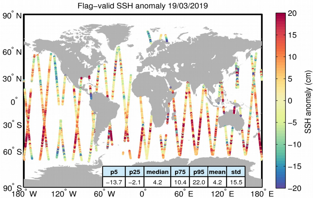
Figure 5. Geographical distribution of flag-valid 1-Hz SSH anomaly data over oceans and lakes for 19/03/2019. The statistical values shown in the table refer to the SSH anomaly in cm and are calculated over all measurements shown in the figure.
