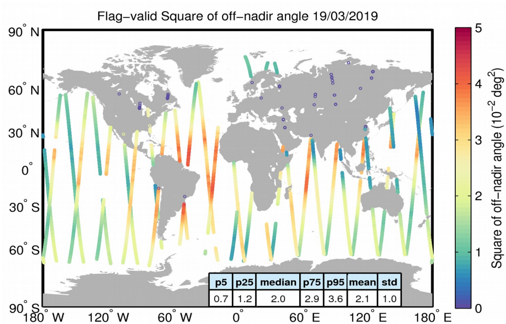
Figure 37. Geographical distribution of flag-valid mispointing data over oceans and lakes for 19/03/2019. The statistical values shown in the table refer to the mispointing in 10^{-2} deg 2 and are calculated over all measurements shown in the figure.
