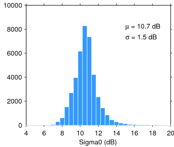
Figure 28. Histogram of science-valid sigma0 over oceans and lakes for 19/03/2019. The mean ( \mu ) and standard deviation ( \sigma ) are also shown. Note that values outside [4 20] dB are excluded from the histogram for the sake of readability but not from the computation of \mu and \sigma .
