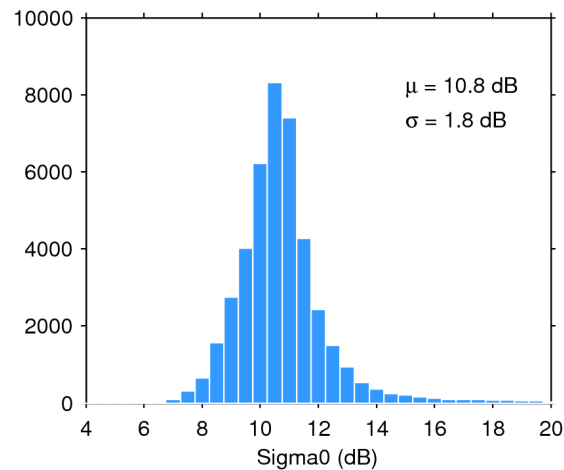
Figure 25. Histogram of flag-valid sigma0 over oceans and lakes for 19/03/2019. The mean ( \mu ) and standard deviation ( \sigma ) are also shown. Note that values outside [4 20] dB are excluded from the histogram for the sake of readability but not from the computation of \mu and \sigma .
