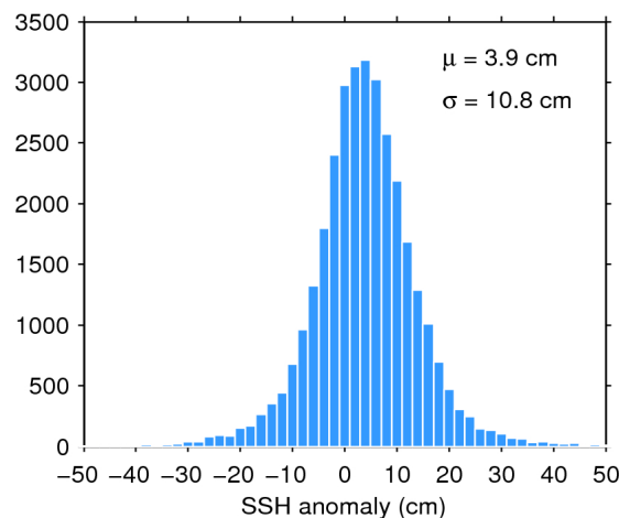
Figure 11. Histogram of science-valid SSH anomaly over oceans and lakes for 18/03/2019. The mean ( \mu ) and standard deviation ( \sigma ) are also shown. Note that values outside [-50 50] cm are excluded from the histogram for the sake of readability but not from the computation of \mu and \sigma .
