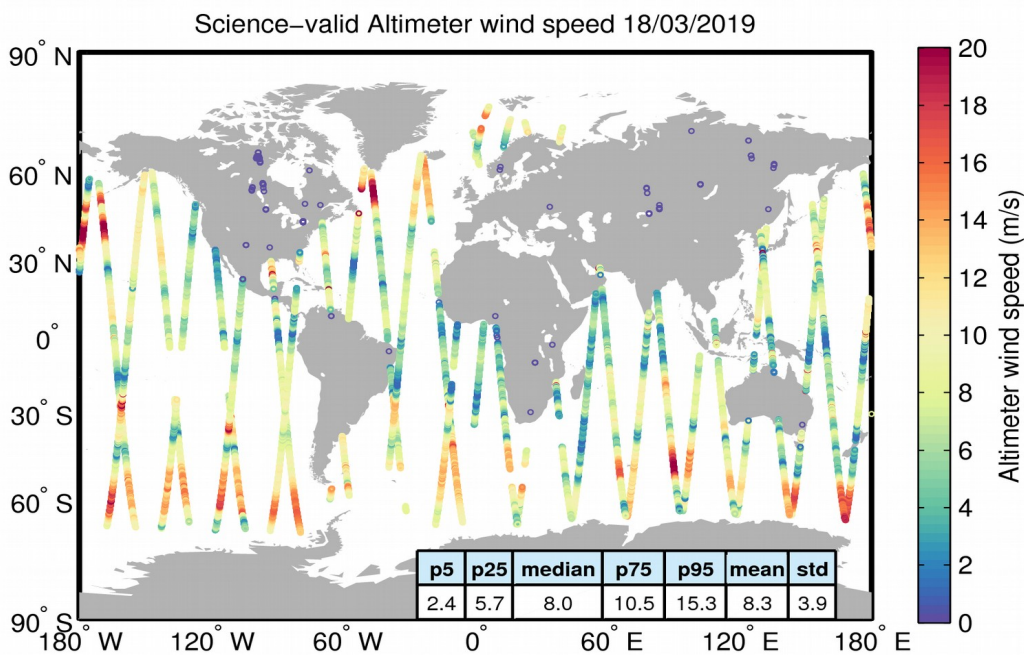
Figure 34. Geographical distribution of science-valid wind data over oceans and lakes for 18/03/2019. The statistical values shown in the table refer to the wind in m/s and are calculated over all measurements shown in the figure. Gray circles denote records that have been rejected based on the editing criteria described in Table 5.
