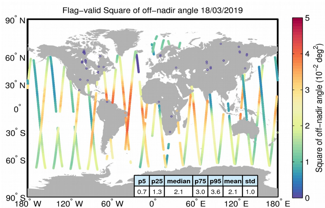
Figure 37. Geographical distribution of flag-valid mispointing data over oceans and lakes for 18/03/2019. The statistical values shown in the table refer to the mispointing in 10^{-2} deg 2 and are calculated over all measurements shown in the figure.
