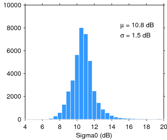
Figure 28. Histogram of science-valid sigma0 over oceans and lakes for 18/03/2019. The mean ( \mu ) and standard deviation ( \sigma ) are also shown. Note that values outside [4 20] dB are excluded from the histogram for the sake of readability but not from the computation of \mu and \sigma .
