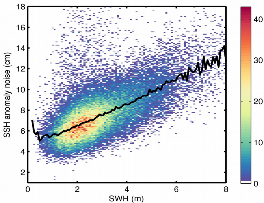
Figure 9. 2D histogram showing flag-valid SSH anomaly noise as a function of SWH for 18/03/2019. The black line denotes the median SSH anomaly noise as a function of SWH.
