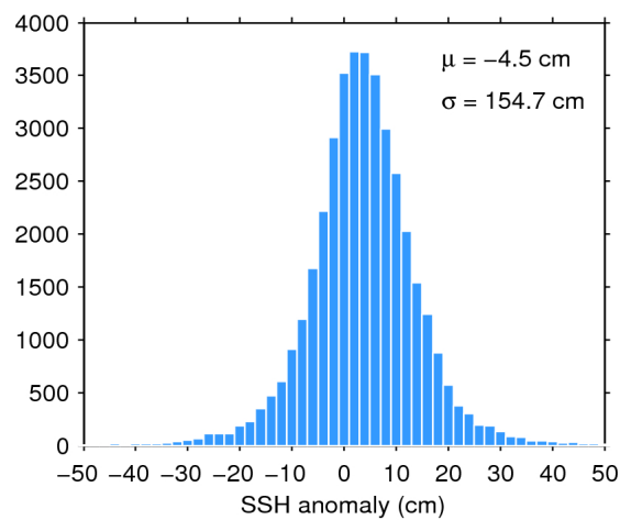
Figure 7. Histogram of flag-valid SSH anomaly over oceans and lakes for 18/03/2019. The mean ( \mu ) and standard deviation ( \sigma ) are also shown. Note that values outside [-50 50] cm are excluded from the histogram for the sake of readability but not from the computation of \mu and \sigma .
