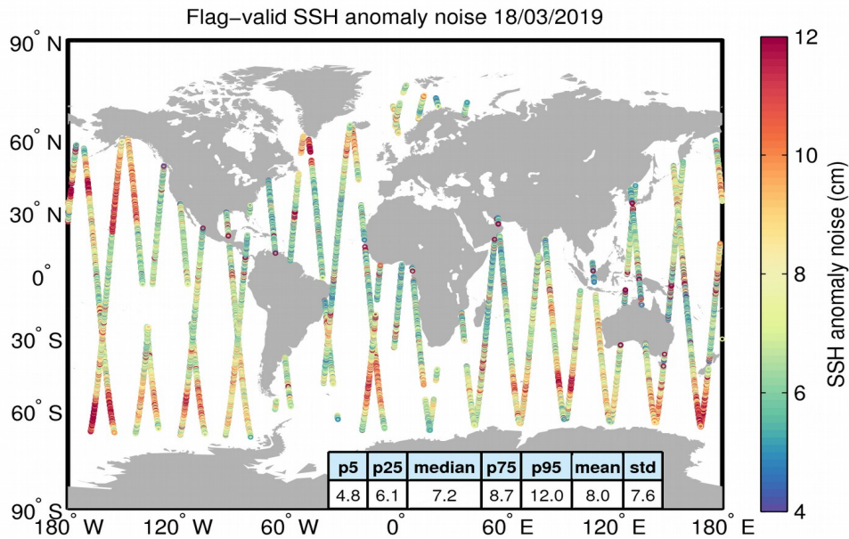
Figure 8. Geographical distribution of flag-valid 20-Hz SSH anomaly measurement noise over oceans and lakes for 18/03/2019. The statistical values shown in the table refer to the SSH anomaly noise and are calculated over all measurements shown in the figure.
