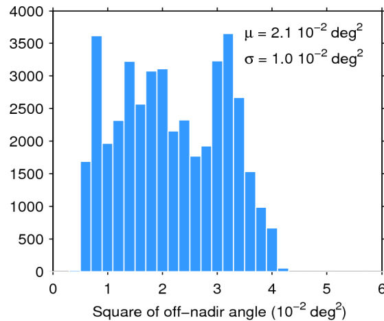
Figure 39. Histogram of flag-valid mispointing over oceans and lakes for 18/03/2019. The mean ( \mu ) and standard deviation ( \sigma ) are also shown. Note that values larger than 6 \cdot 10^{-2} \text{ deg}^2 are excluded from the histogram for the sake of readability but not from the computation of \mu and \sigma .
