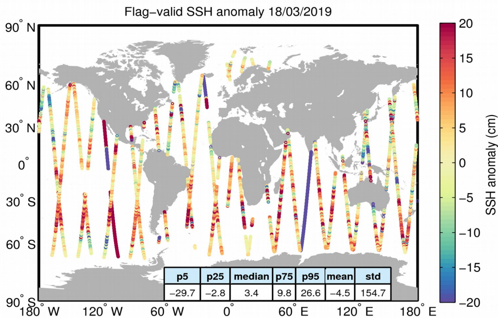
Figure 5. Geographical distribution of flag-valid 1-Hz SSH anomaly data over oceans and lakes for 18/03/2019. The statistical values shown in the table refer to the SSH anomaly in cm and are calculated over all measurements shown in the figure.
