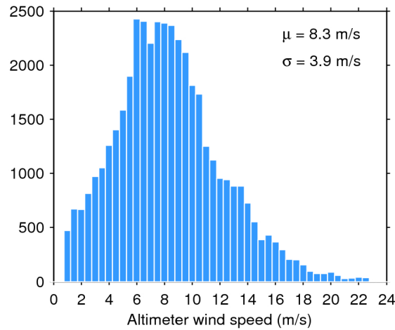
Figure 33. Histogram of flag-valid wind over oceans and lakes for 18/03/2019. The mean ( \mu ) and standard deviation ( \sigma ) are also shown. Note that values larger than 24 m/s are excluded from the histogram for the sake of readability but not from the computation of \mu and \sigma .
