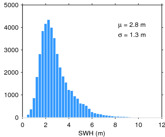
Figure 20. Histogram of science-valid SWH over oceans and lakes for 18/03/2019. The mean ( \mu ) and standard deviation ( \sigma ) are also shown. Note that values larger than 12 m are excluded from the histogram for the sake of readability but not from the computation of \mu and \sigma .
