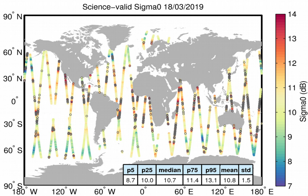
Figure 27. Geographical distribution of science-valid sigma0 data over oceans and lakes for 18/03/2019. The statistical values shown in the table refer to the sigma0 in dB and are calculated over all measurements shown in the figure. Gray circles denote records that have been rejected based on the editing criteria described in Table 4.
