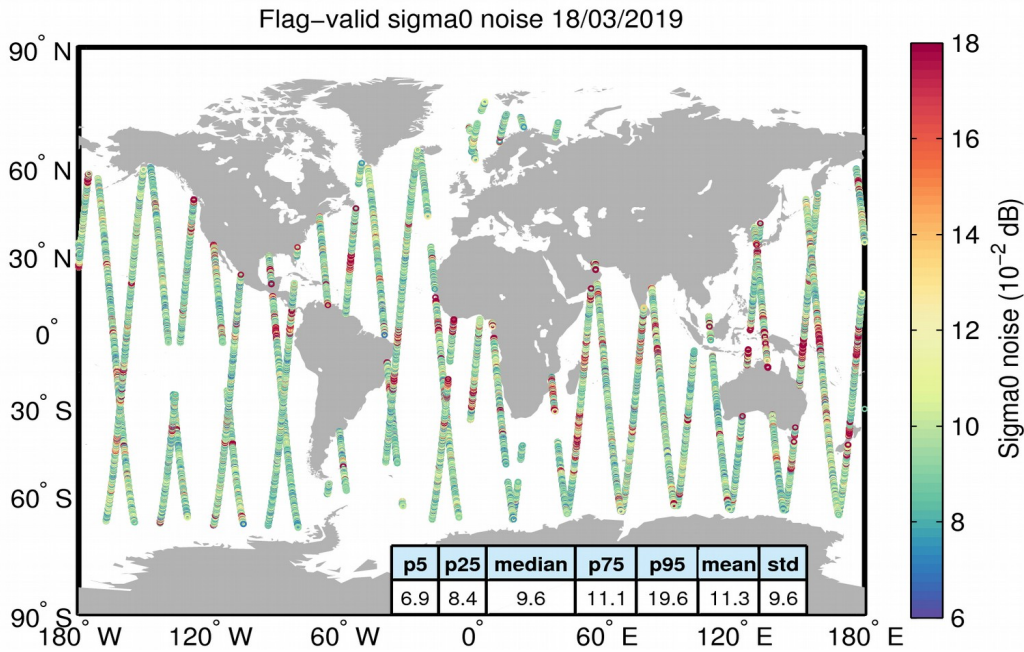
Figure 26. Geographical distribution of flag-valid 20-Hz sigma0 measurement noise over oceans and lakes for 18/03/2019. The statistical values shown in the table refer to the sigma0 noise and are calculated over all measurements shown in the figure.
