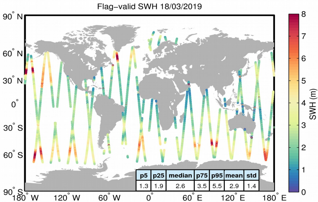
Figure 15. Geographical distribution of flag-valid SWH data over oceans and lakes for 18/03/2019. The statistical values shown in the table refer to the SWH in m and are calculated over all measurements shown in the figure.
