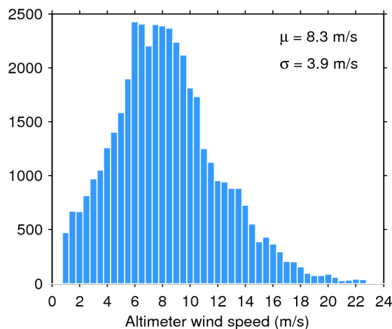
Figure 35. Histogram of science-valid wind over oceans and lakes for 18/03/2019. The mean ( \mu ) and standard deviation ( \sigma ) are also shown. Note that values larger than 24 m/s are excluded from the histogram for the sake of readability but not from the computation of \mu and \sigma .
