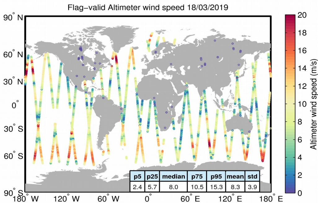
Figure 31. Geographical distribution of flag-valid wind data over oceans and lakes for 18/03/2019. The statistical values shown in the table refer to the wind in m/s and are calculated over all measurements shown in the figure.
