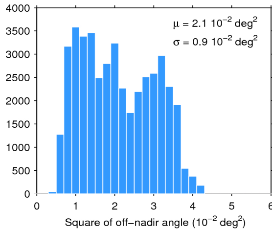
Figure 39. Histogram of flag-valid mispointing over oceans and lakes for 17/03/2019. The mean ( \mu ) and standard deviation ( \sigma ) are also shown. Note that values larger than 6 \cdot 10^{-2} \text{ deg}^2 are excluded from the histogram for the sake of readability but not from the computation of \mu and \sigma .
