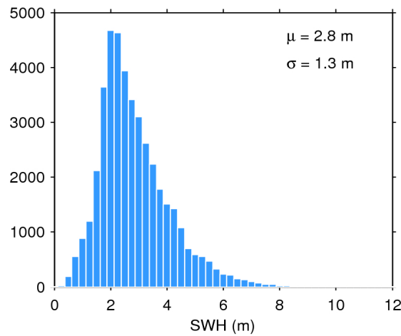
Figure 17. Histogram of flag-valid SWH over oceans and lakes for 17/03/2019. The mean ( \mu ) and standard deviation ( \sigma ) are also shown. Note that values larger than 12 m are excluded from the histogram for the sake of readability but not from the computation of \mu and \sigma .
