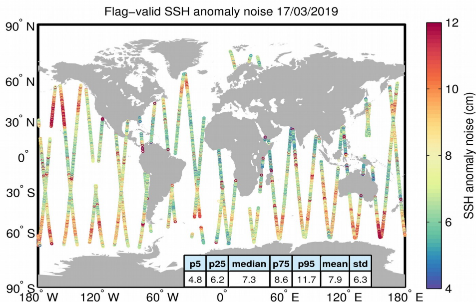
Figure 8. Geographical distribution of flag-valid 20-Hz SSH anomaly measurement noise over oceans and lakes for 17/03/2019. The statistical values shown in the table refer to the SSH anomaly noise and are calculated over all measurements shown in the figure.
