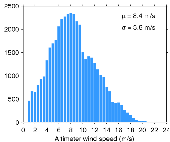
Figure 35. Histogram of science-valid wind over oceans and lakes for 17/03/2019. The mean ( \mu ) and standard deviation ( \sigma ) are also shown. Note that values larger than 24 m/s are excluded from the histogram for the sake of readability but not from the computation of \mu and \sigma .
