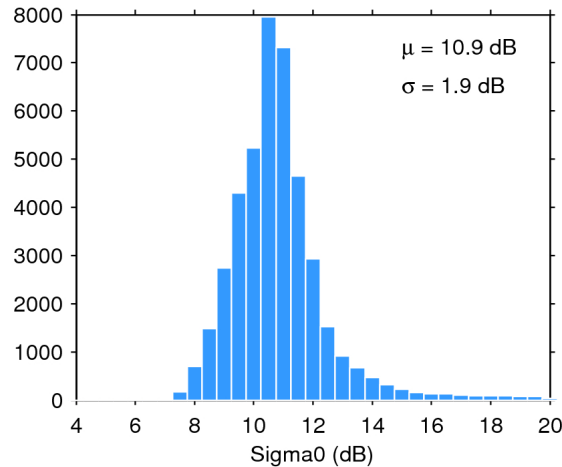
Figure 25. Histogram of flag-valid sigma0 over oceans and lakes for 17/03/2019. The mean ( \mu ) and standard deviation ( \sigma ) are also shown. Note that values outside [4 20] dB are excluded from the histogram for the sake of readability but not from the computation of \mu and \sigma .
