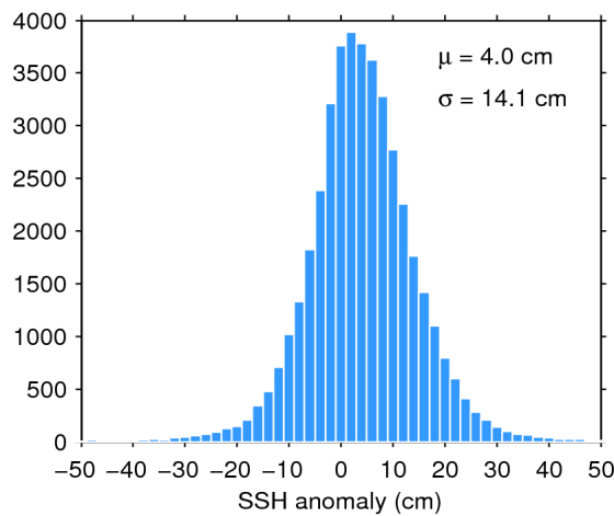
Figure 7. Histogram of flag-valid SSH anomaly over oceans and lakes for 17/03/2019. The mean ( \mu ) and standard deviation ( \sigma ) are also shown. Note that values outside [-50 50] cm are excluded from the histogram for the sake of readability but not from the computation of \mu and \sigma .
