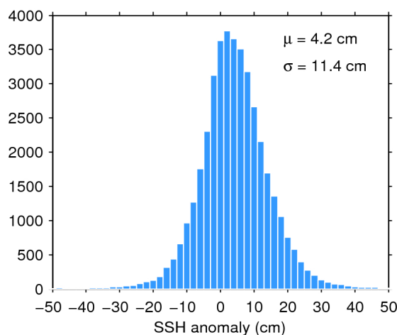
Figure 11. Histogram of science-valid SSH anomaly over oceans and lakes for 17/03/2019. The mean ( \mu ) and standard deviation ( \sigma ) are also shown. Note that values outside [-50 \text{ } 50] cm are excluded from the histogram for the sake of readability but not from the computation of \mu and \sigma .
