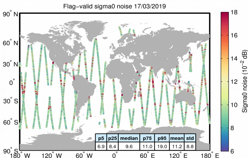
Figure 26. Geographical distribution of flag-valid 20-Hz sigma0 measurement noise over oceans and lakes for 17/03/2019. The statistical values shown in the table refer to the sigma0 noise and are calculated over all measurements shown in the figure.
