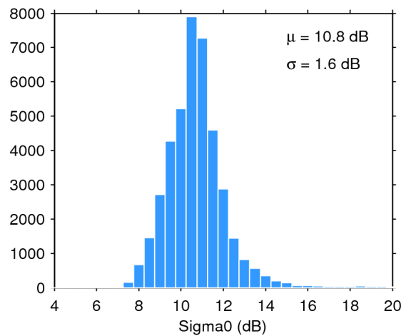
Figure 28. Histogram of science-valid sigma0 over oceans and lakes for 17/03/2019. The mean ( \mu ) and standard deviation ( \sigma ) are also shown. Note that values outside [4 20] dB are excluded from the histogram for the sake of readability but not from the computation of \mu and \sigma .
