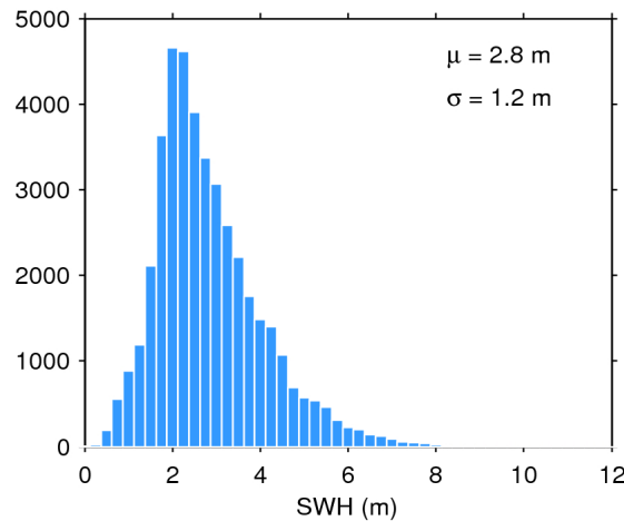
Figure 20. Histogram of science-valid SWH over oceans and lakes for 17/03/2019. The mean ( \mu ) and standard deviation ( \sigma ) are also shown. Note that values larger than 12 m are excluded from the histogram for the sake of readability but not from the computation of \mu and \sigma .
