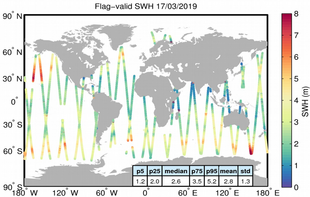
Figure 15. Geographical distribution of flag-valid SWH data over oceans and lakes for 17/03/2019. The statistical values shown in the table refer to the SWH in m and are calculated over all measurements shown in the figure.
