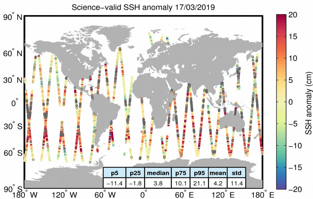
Figure 10. Geographical distribution of science-valid SSH anomaly data over oceans and lakes for 17/03/2019. The statistical values shown in the table refer to the SSH anomaly in cm and are calculated over all measurements shown in the figure. Gray circles denote records that have been rejected based on the editing criteria described in Table 2.
