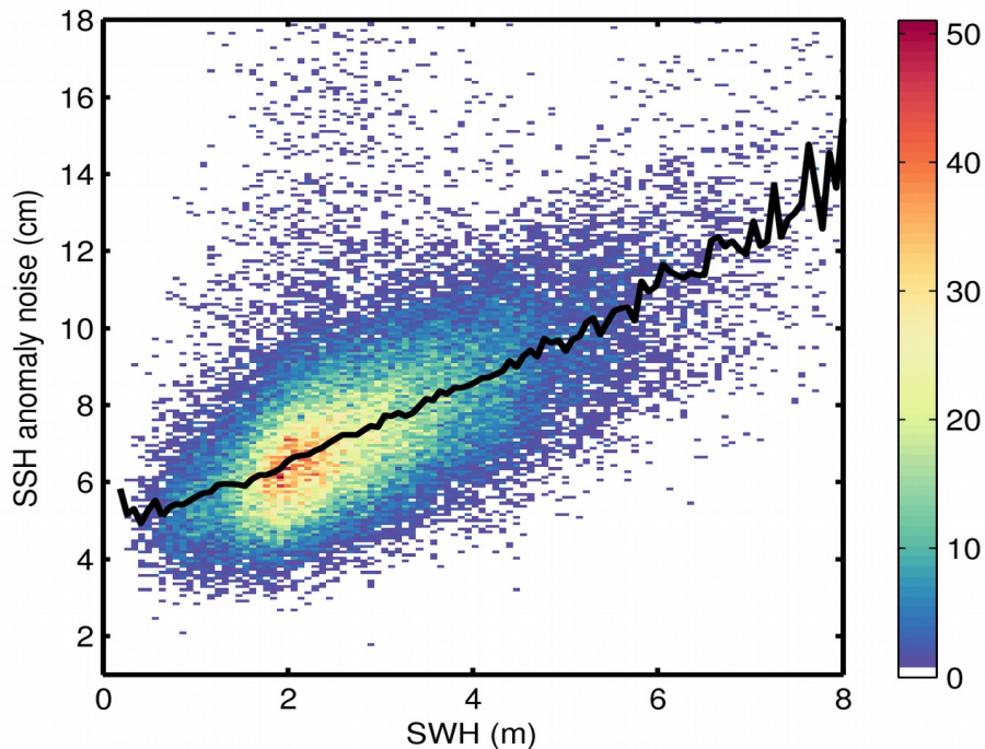
Figure 9. 2D histogram showing flag-valid SSH anomaly noise as a function of SWH for 17/03/2019. The black line denotes the median SSH anomaly noise as a function of SWH.
