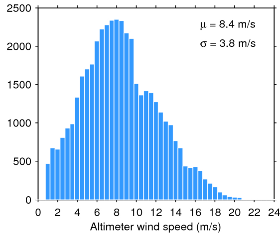
Figure 33. Histogram of flag-valid wind over oceans and lakes for 17/03/2019. The mean ( \mu ) and standard deviation ( \sigma ) are also shown. Note that values larger than 24 m/s are excluded from the histogram for the sake of readability but not from the computation of \mu and \sigma .
