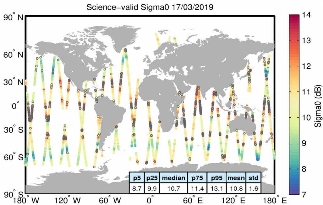
Figure 27. Geographical distribution of science-valid sigma0 data over oceans and lakes for 17/03/2019. The statistical values shown in the table refer to the sigma0 in dB and are calculated over all measurements shown in the figure. Gray circles denote records that have been rejected based on the editing criteria described in Table 4.
