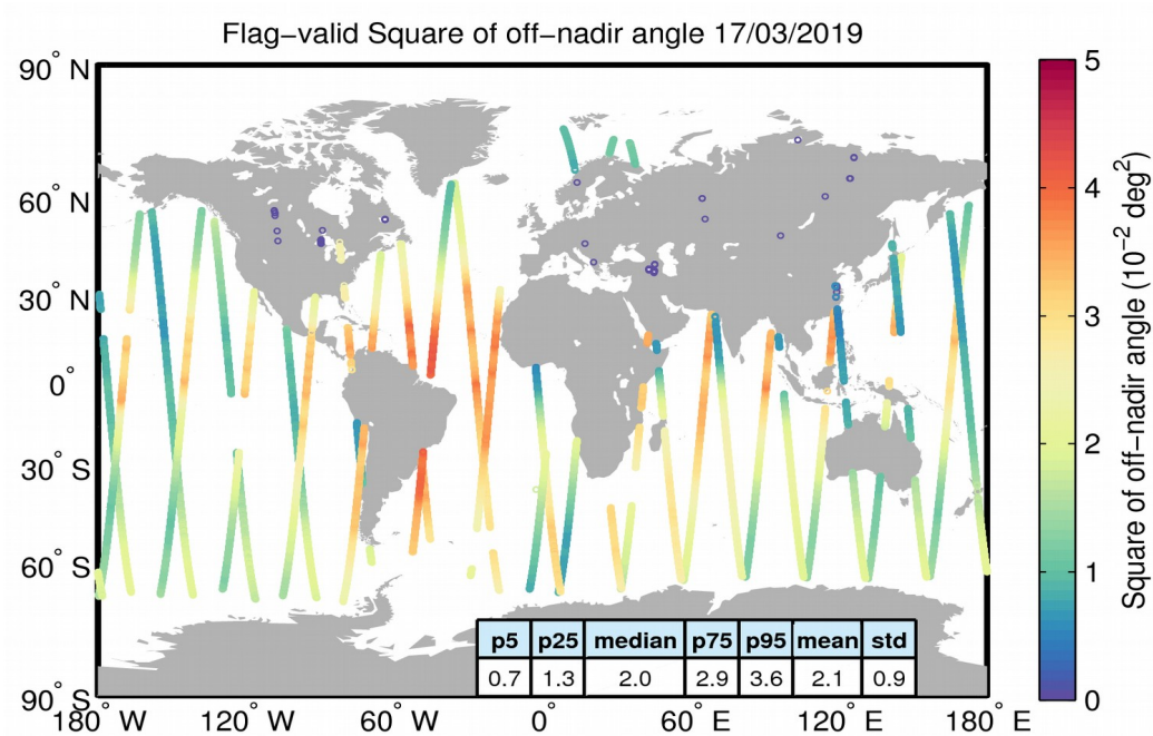
Figure 37. Geographical distribution of flag-valid mispointing data over oceans and lakes for 17/03/2019. The statistical values shown in the table refer to the mispointing in 10^{-2} \text{ deg}^2 and are calculated over all measurements shown in the figure.
