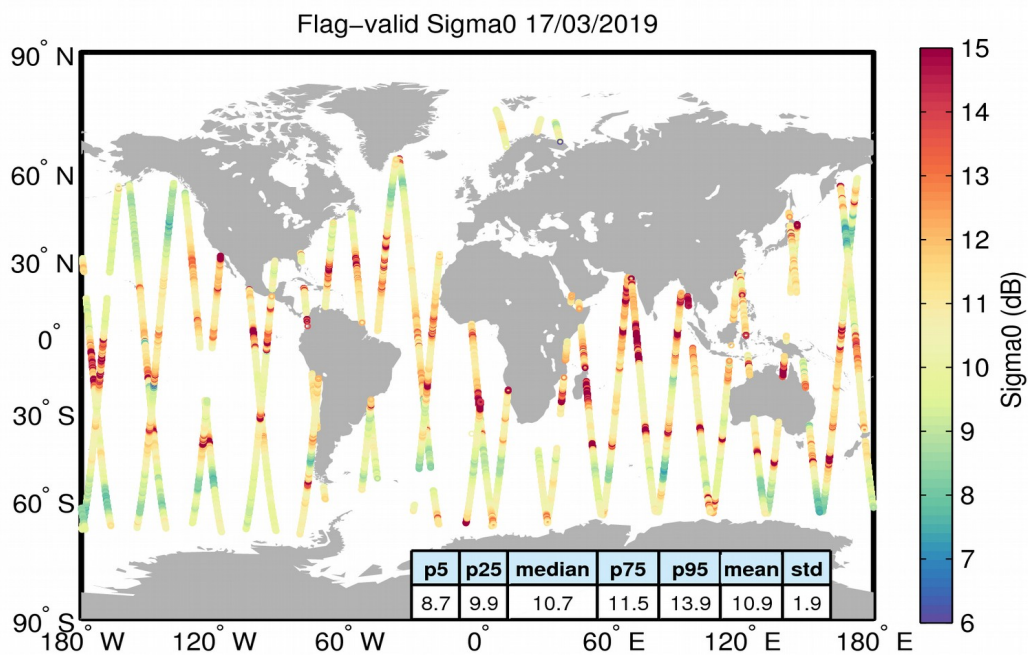
Figure 23. Geographical distribution of flag-valid sigma0 data over oceans and lakes for 17/03/2019. The statistical values shown in the table refer to the sigma0 in dB and are calculated over all measurements shown in the figure.
