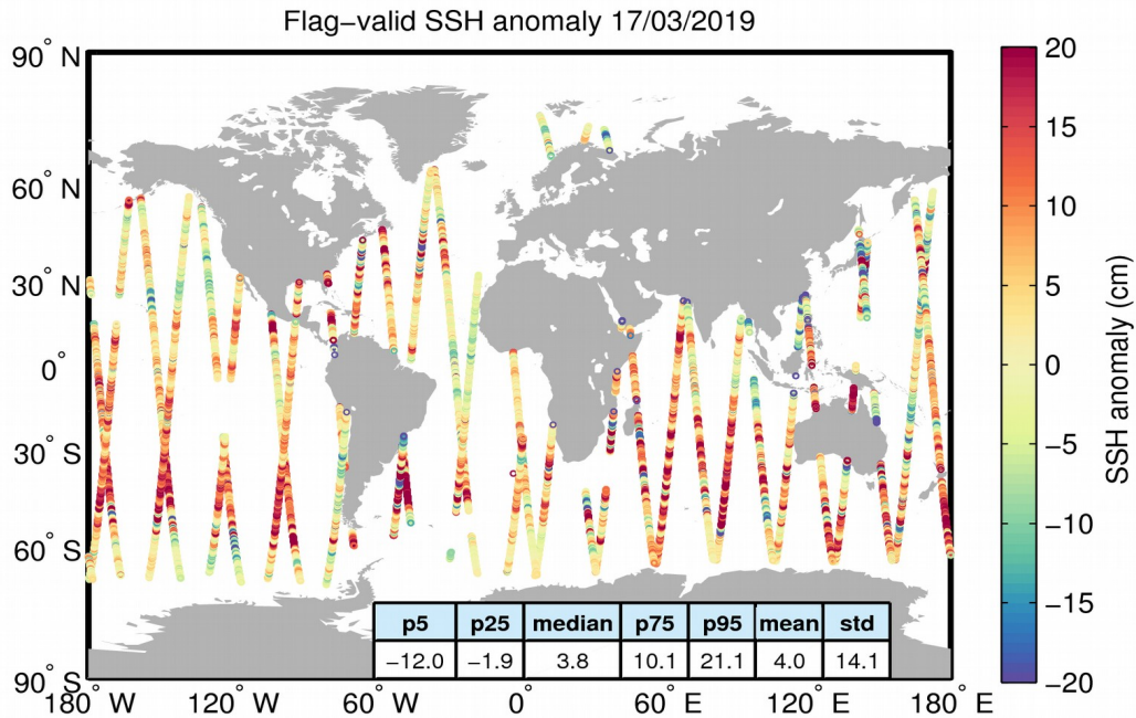
Figure 5. Geographical distribution of flag-valid 1-Hz SSH anomaly data over oceans and lakes for 17/03/2019. The statistical values shown in the table refer to the SSH anomaly in cm and are calculated over all measurements shown in the figure.
