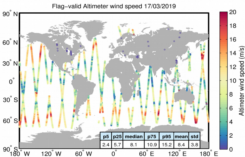
Figure 31. Geographical distribution of flag-valid wind data over oceans and lakes for 17/03/2019. The statistical values shown in the table refer to the wind in m/s and are calculated over all measurements shown in the figure.
