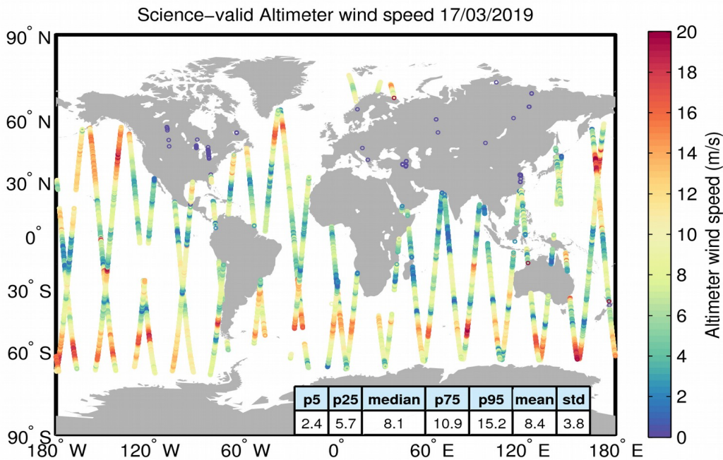
Figure 34. Geographical distribution of science-valid wind data over oceans and lakes for 17/03/2019. The statistical values shown in the table refer to the wind in m/s and are calculated over all measurements shown in the figure. Gray circles denote records that have been rejected based on the editing criteria described in Table 5.
