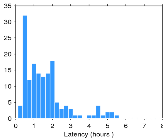
Figure 2. Histogram of the data latency for 17/03/2019. The y-axis denotes the number of files that are made available with a delay of x-hours with respect to the mean time of the records stored in the file.
