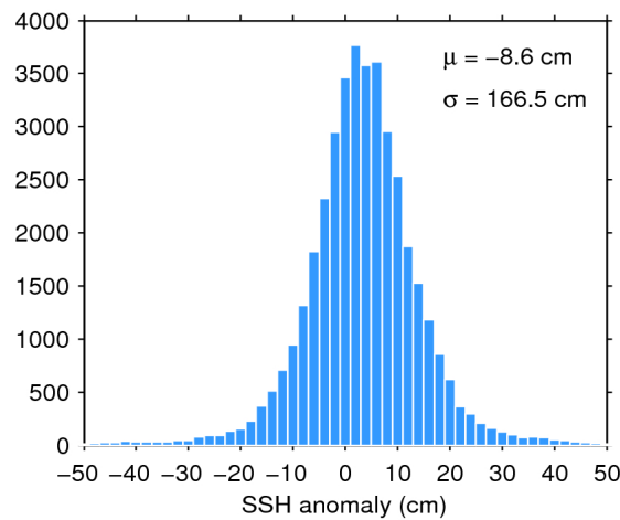
Figure 7. Histogram of flag-valid SSH anomaly over oceans and lakes for 16/03/2019. The mean ( \mu ) and standard deviation ( \sigma ) are also shown. Note that values outside [-50 50] cm are excluded from the histogram for the sake of readability but not from the computation of \mu and \sigma .
