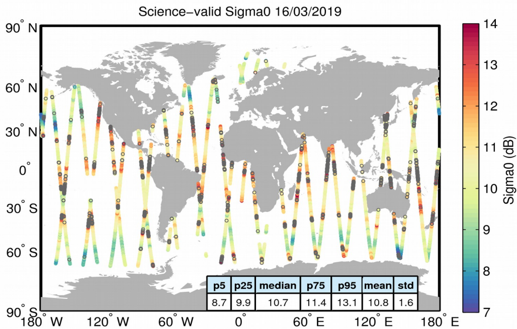
Figure 27. Geographical distribution of science-valid sigma0 data over oceans and lakes for 16/03/2019. The statistical values shown in the table refer to the sigma0 in dB and are calculated over all measurements shown in the figure. Gray circles denote records that have been rejected based on the editing criteria described in Table 4.
