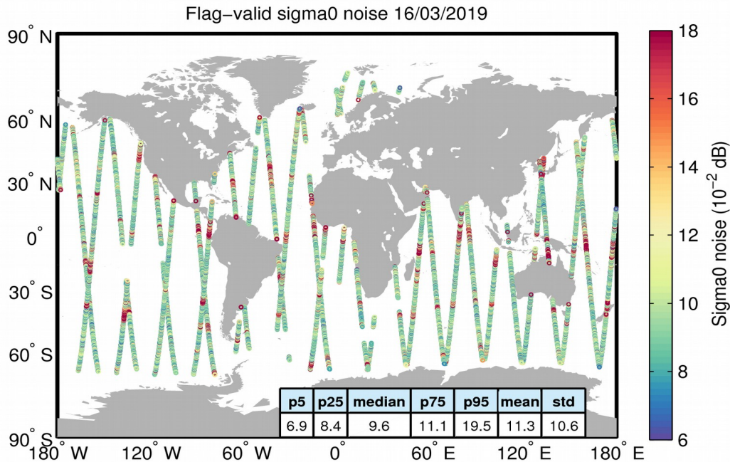
Figure 26. Geographical distribution of flag-valid 20-Hz sigma0 measurement noise over oceans and lakes for 16/03/2019. The statistical values shown in the table refer to the sigma0 noise and are calculated over all measurements shown in the figure.
