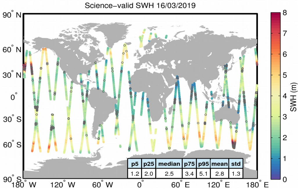
Figure 19. Geographical distribution of science-valid SWH data over oceans and lakes for 16/03/2019. The statistical values shown in the table refer to the SWH in m and are calculated over all measurements shown in the figure. Gray circles denote records that have been rejected based on the editing criteria described in Table 3.
