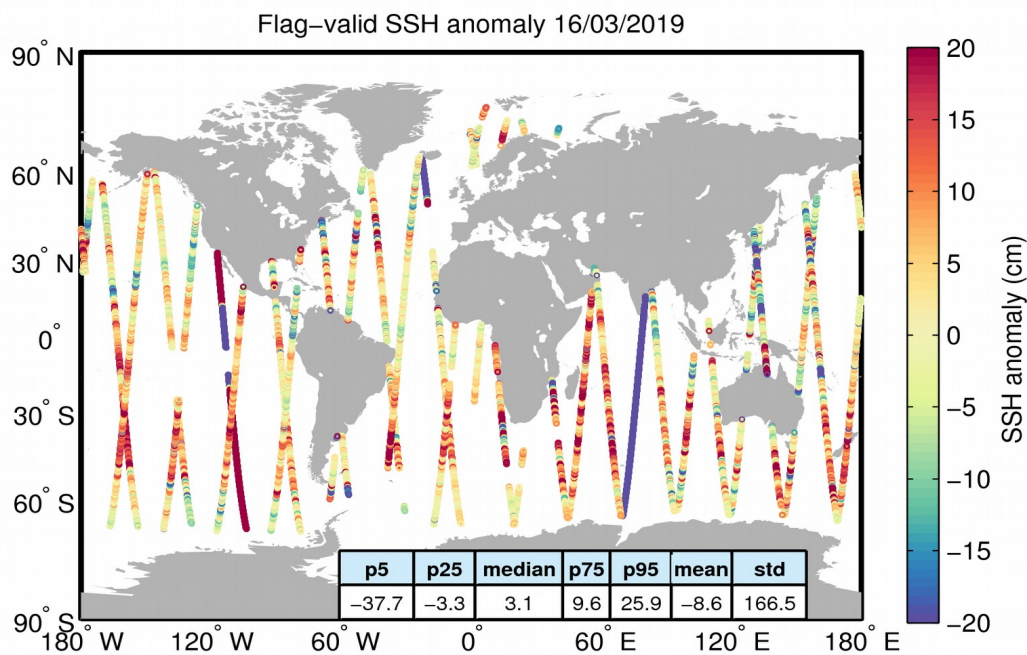
Figure 5. Geographical distribution of flag-valid 1-Hz SSH anomaly data over oceans and lakes for 16/03/2019. The statistical values shown in the table refer to the SSH anomaly in cm and are calculated over all measurements shown in the figure.
