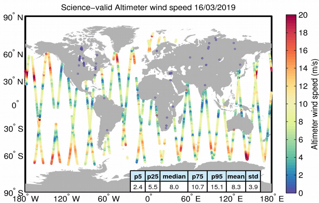
Figure 34. Geographical distribution of science-valid wind data over oceans and lakes for 16/03/2019. The statistical values shown in the table refer to the wind in m/s and are calculated over all measurements shown in the figure. Gray circles denote records that have been rejected based on the editing criteria described in Table 5.
