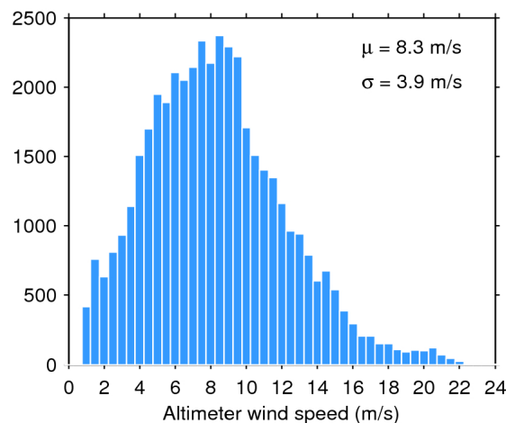
Figure 35. Histogram of science-valid wind over oceans and lakes for 16/03/2019. The mean ( \mu ) and standard deviation ( \sigma ) are also shown. Note that values larger than 24 m/s are excluded from the histogram for the sake of readability but not from the computation of \mu and \sigma .
