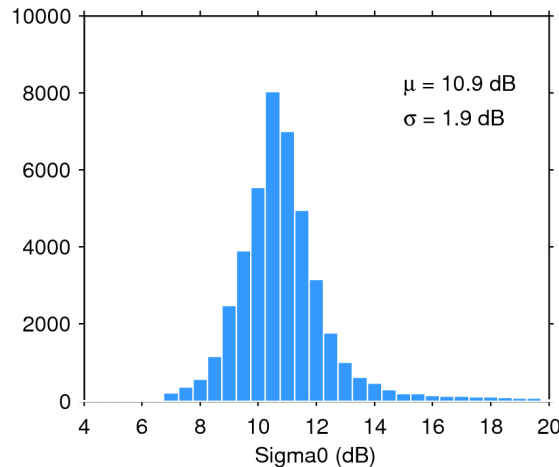
Figure 25. Histogram of flag-valid sigma0 over oceans and lakes for 16/03/2019. The mean ( \mu ) and standard deviation ( \sigma ) are also shown. Note that values outside [4 20] dB are excluded from the histogram for the sake of readability but not from the computation of \mu and \sigma .
