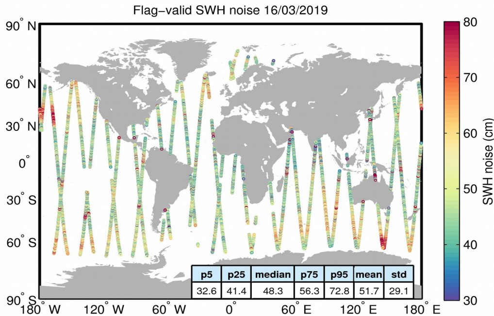
Figure 18. Geographical distribution of flag-valid 20-Hz SWH measurement noise over oceans and lakes for 16/03/2019. The statistical values shown in the table refer to the SWH noise and are calculated over all measurements shown in the figure.
