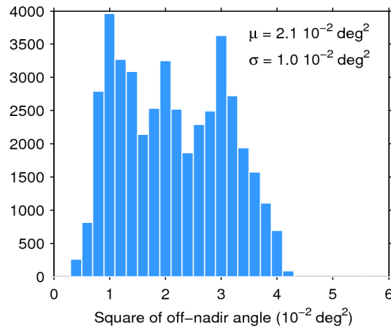
Figure 39. Histogram of flag-valid mispointing over oceans and lakes for 16/03/2019. The mean ( \mu ) and standard deviation ( \sigma ) are also shown. Note that values larger than 6 \cdot 10^{-2} \text{ deg}^2 are excluded from the histogram for the sake of readability but not from the computation of \mu and \sigma .
