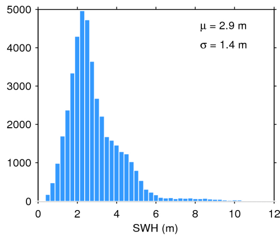
Figure 17. Histogram of flag-valid SWH over oceans and lakes for 16/03/2019. The mean ( \mu ) and standard deviation ( \sigma ) are also shown. Note that values larger than 12 m are excluded from the histogram for the sake of readability but not from the computation of \mu and \sigma .
