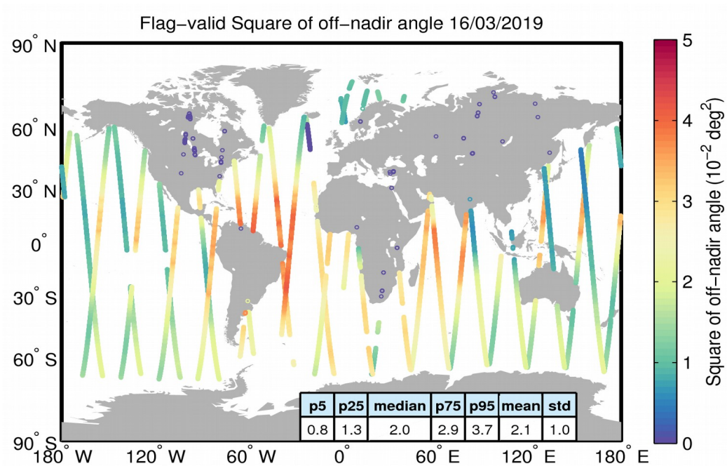
Figure 37. Geographical distribution of flag-valid mispointing data over oceans and lakes for 16/03/2019. The statistical values shown in the table refer to the mispointing in 10^{-2} \text{ deg}^2 and are calculated over all measurements shown in the figure.
