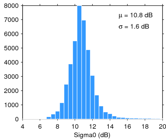
Figure 28. Histogram of science-valid sigma0 over oceans and lakes for 16/03/2019. The mean ( \mu ) and standard deviation ( \sigma ) are also shown. Note that values outside [4 20] dB are excluded from the histogram for the sake of readability but not from the computation of \mu and \sigma .
