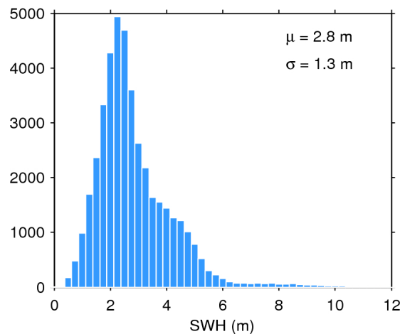
Figure 20. Histogram of science-valid SWH over oceans and lakes for 16/03/2019. The mean ( \mu ) and standard deviation ( \sigma ) are also shown. Note that values larger than 12 m are excluded from the histogram for the sake of readability but not from the computation of \mu and \sigma .
