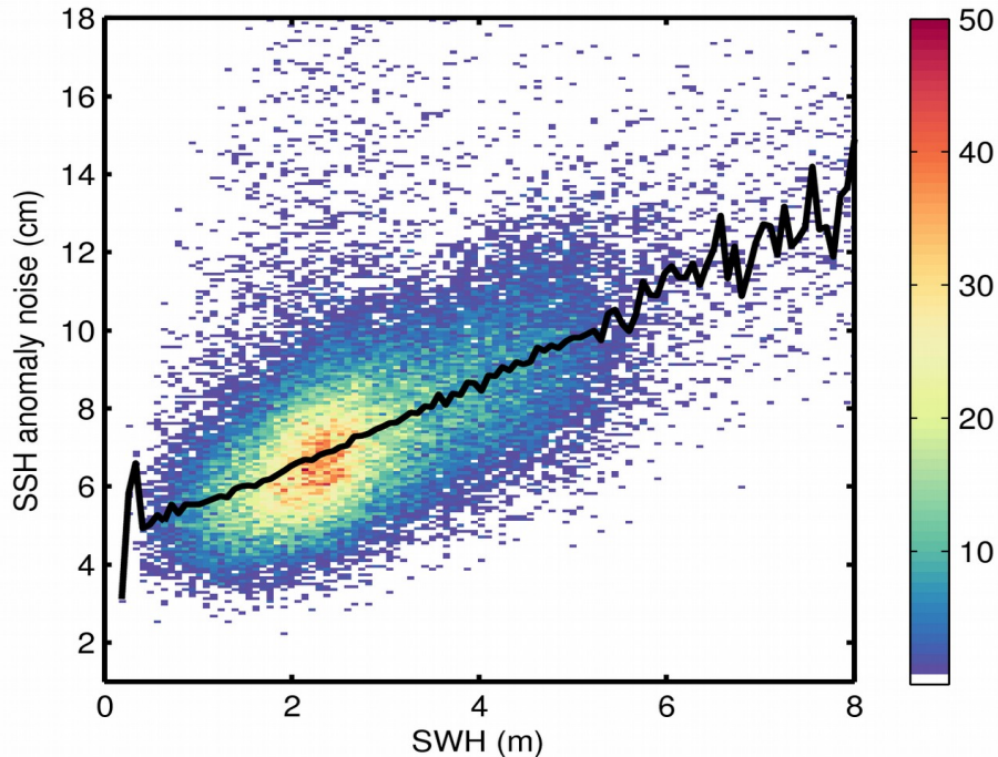
Figure 9. 2D histogram showing flag-valid SSH anomaly noise as a function of SWH for 16/03/2019. The black line denotes the median SSH anomaly noise as a function of SWH.
