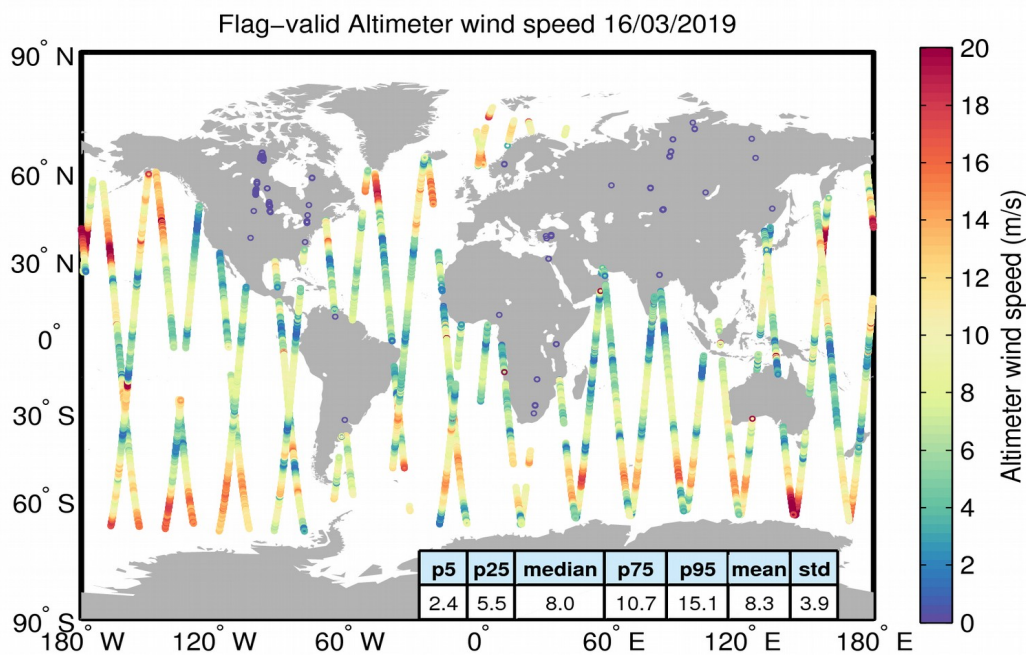
Figure 31. Geographical distribution of flag-valid wind data over oceans and lakes for 16/03/2019. The statistical values shown in the table refer to the wind in m/s and are calculated over all measurements shown in the figure.
