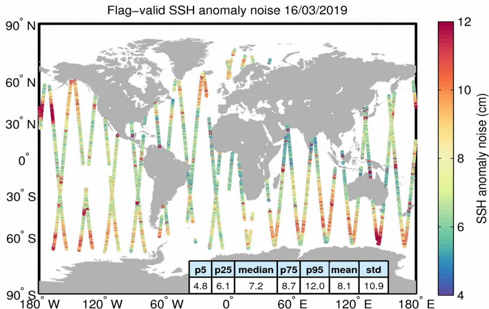
Figure 8. Geographical distribution of flag-valid 20-Hz SSH anomaly measurement noise over oceans and lakes for 16/03/2019. The statistical values shown in the table refer to the SSH anomaly noise and are calculated over all measurements shown in the figure.
