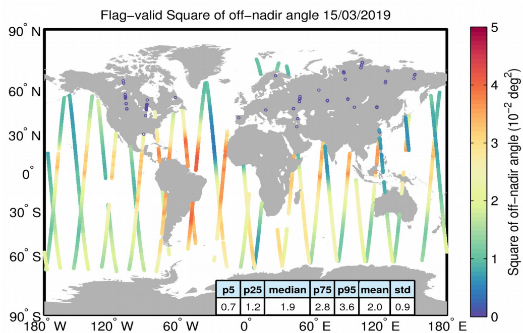
Figure 37. Geographical distribution of flag-valid mispointing data over oceans and lakes for 15/03/2019. The statistical values shown in the table refer to the mispointing in 10^{-2} \text{ deg}^2 and are calculated over all measurements shown in the figure.
