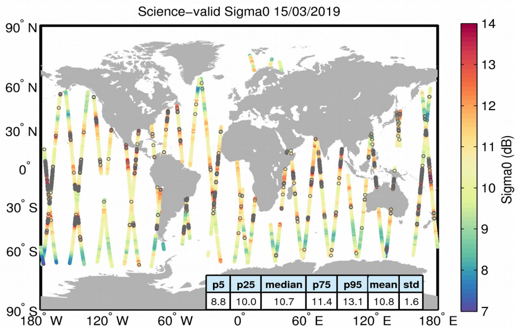
Figure 27. Geographical distribution of science-valid sigma0 data over oceans and lakes for 15/03/2019. The statistical values shown in the table refer to the sigma0 in dB and are calculated over all measurements shown in the figure. Gray circles denote records that have been rejected based on the editing criteria described in Table 4.
