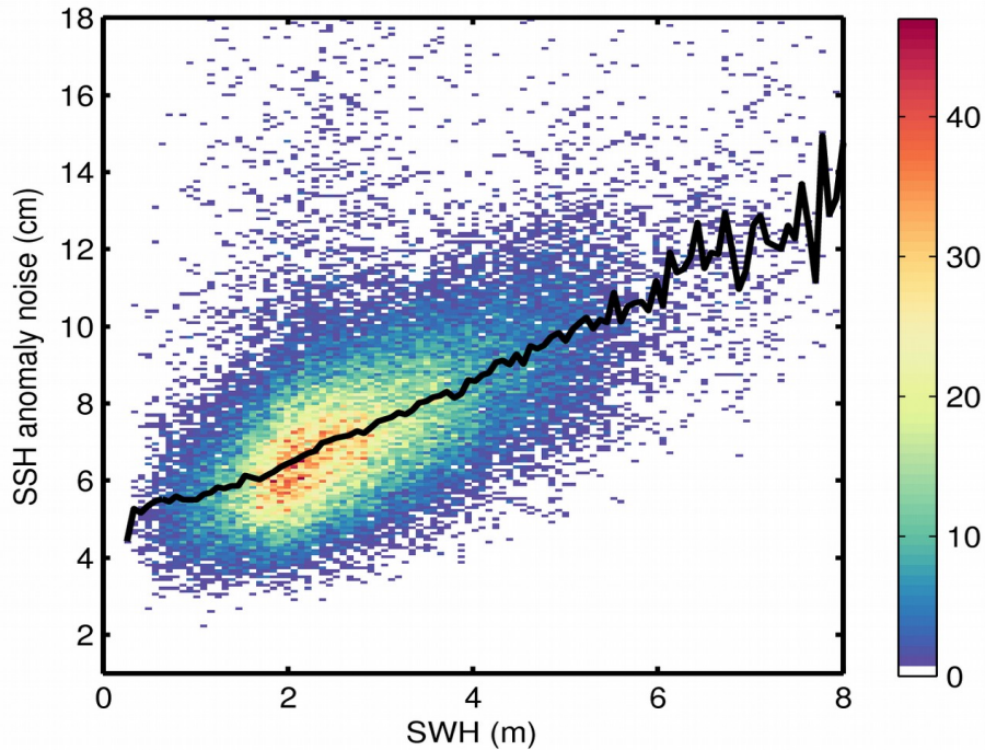
Figure 9. 2D histogram showing flag-valid SSH anomaly noise as a function of SWH for 15/03/2019. The black line denotes the median SSH anomaly noise as a function of SWH.
