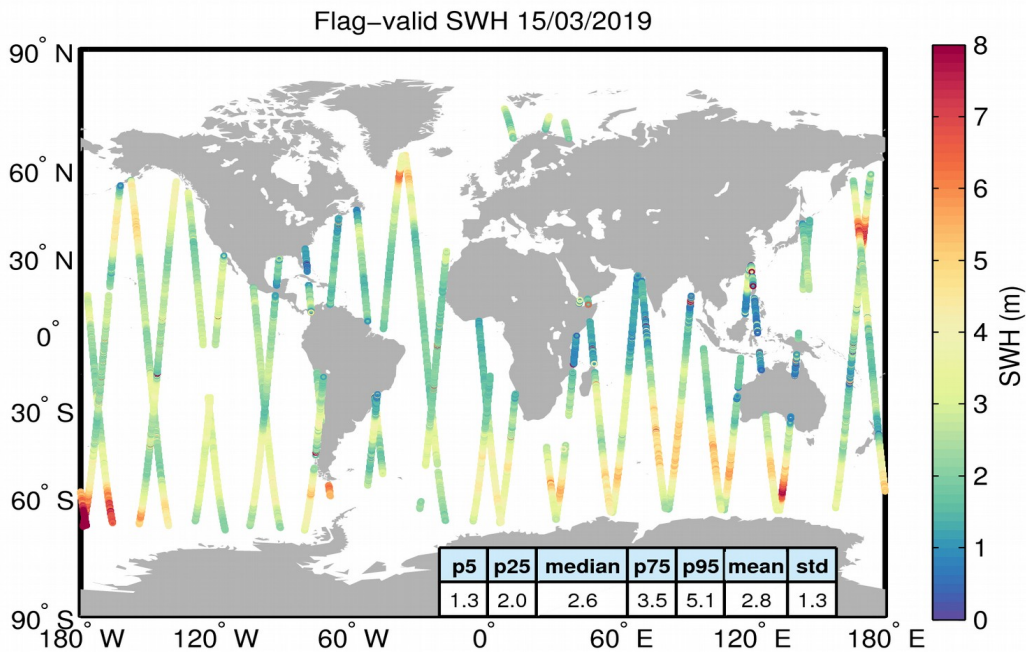
Figure 15. Geographical distribution of flag-valid SWH data over oceans and lakes for 15/03/2019. The statistical values shown in the table refer to the SWH in m and are calculated over all measurements shown in the figure.
