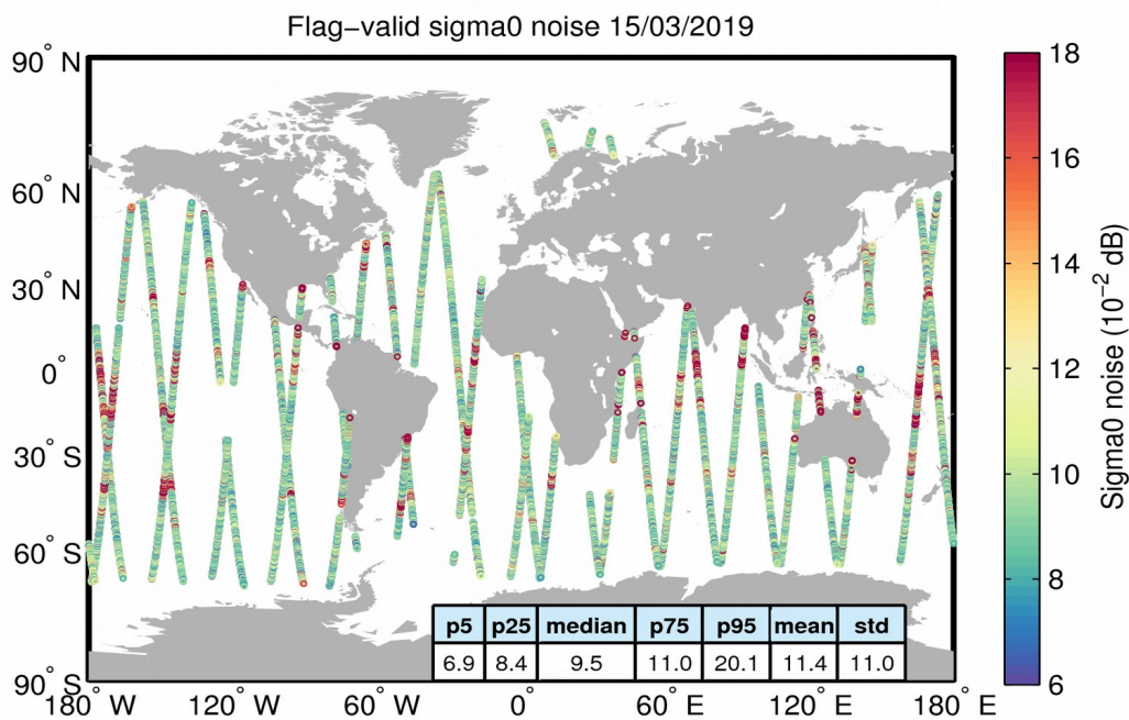
Figure 26. Geographical distribution of flag-valid 20-Hz sigma0 measurement noise over oceans and lakes for 15/03/2019. The statistical values shown in the table refer to the sigma0 noise and are calculated over all measurements shown in the figure.
