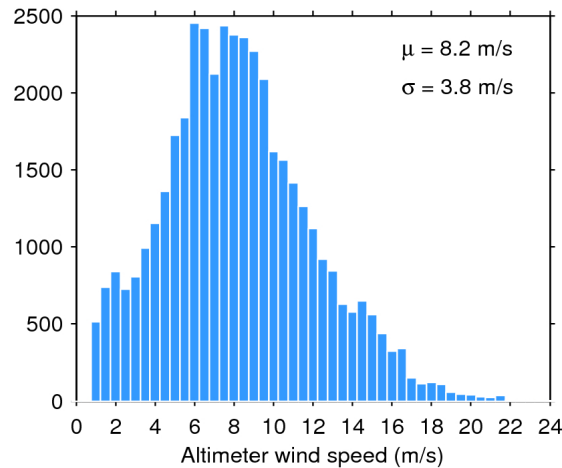
Figure 33. Histogram of flag-valid wind over oceans and lakes for 15/03/2019. The mean ( \mu ) and standard deviation ( \sigma ) are also shown. Note that values larger than 24 m/s are excluded from the histogram for the sake of readability but not from the computation of \mu and \sigma .
