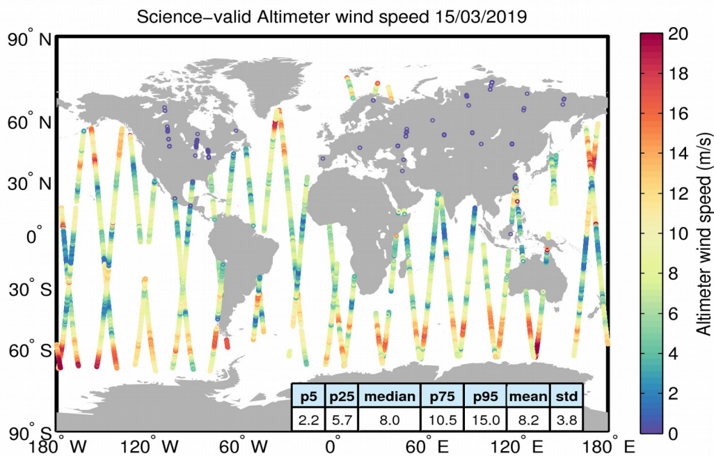
Figure 34. Geographical distribution of science-valid wind data over oceans and lakes for 15/03/2019. The statistical values shown in the table refer to the wind in m/s and are calculated over all measurements shown in the figure. Gray circles denote records that have been rejected based on the editing criteria described in Table 5.
