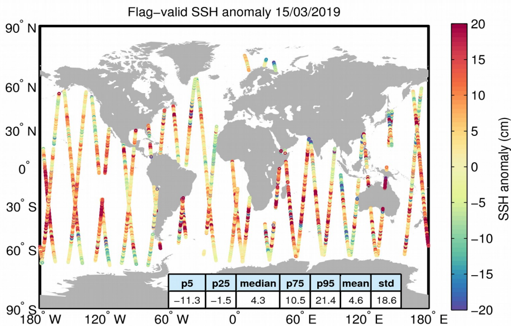
Figure 5. Geographical distribution of flag-valid 1-Hz SSH anomaly data over oceans and lakes for 15/03/2019. The statistical values shown in the table refer to the SSH anomaly in cm and are calculated over all measurements shown in the figure.
