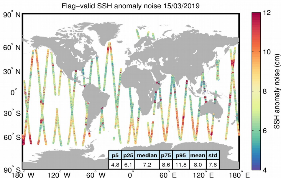
Figure 8. Geographical distribution of flag-valid 20-Hz SSH anomaly measurement noise over oceans and lakes for 15/03/2019. The statistical values shown in the table refer to the SSH anomaly noise and are calculated over all measurements shown in the figure.
