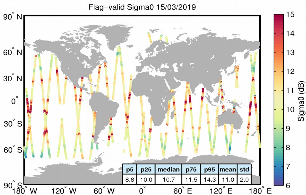
Figure 23. Geographical distribution of flag-valid sigma0 data over oceans and lakes for 15/03/2019. The statistical values shown in the table refer to the sigma0 in dB and are calculated over all measurements shown in the figure.
