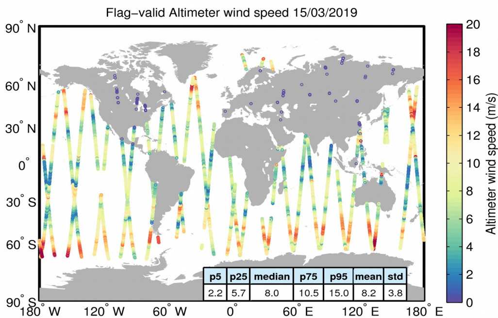
Figure 31. Geographical distribution of flag-valid wind data over oceans and lakes for 15/03/2019. The statistical values shown in the table refer to the wind in m/s and are calculated over all measurements shown in the figure.
