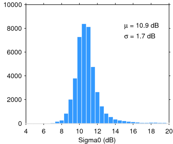
Figure 25. Histogram of flag-valid sigma0 over oceans and lakes for 14/03/2019. The mean ( \mu ) and standard deviation ( \sigma ) are also shown. Note that values outside [4 20] dB are excluded from the histogram for the sake of readability but not from the computation of \mu and \sigma .
