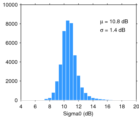
Figure 28. Histogram of science-valid sigma0 over oceans and lakes for 14/03/2019. The mean ( \mu ) and standard deviation ( \sigma ) are also shown. Note that values outside [4 20] dB are excluded from the histogram for the sake of readability but not from the computation of \mu and \sigma .
