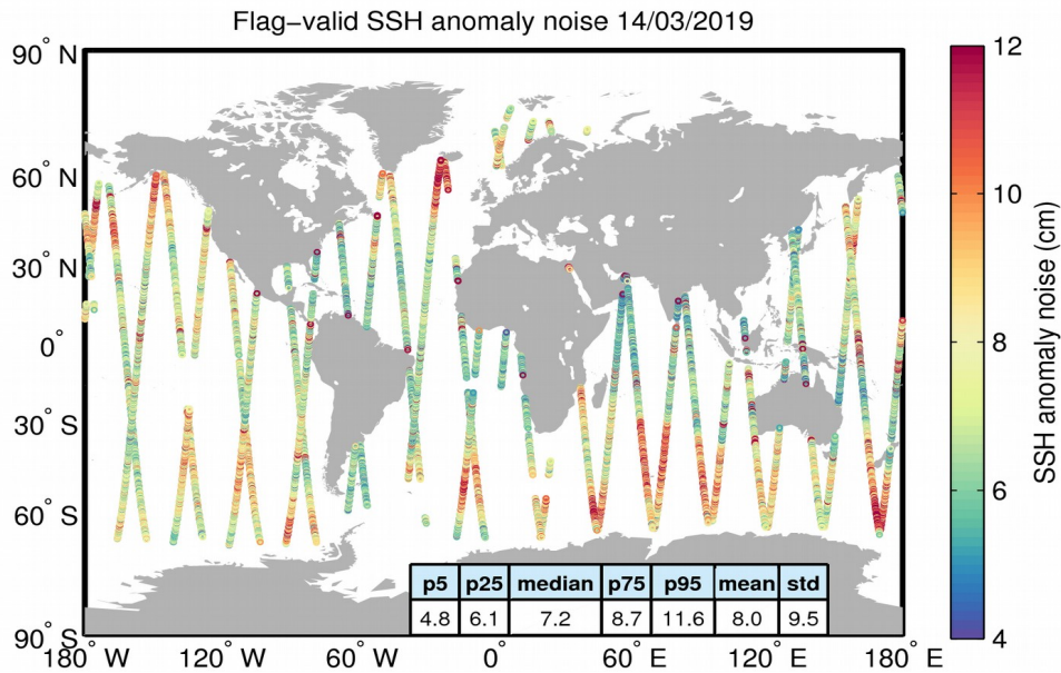
Figure 8. Geographical distribution of flag-valid 20-Hz SSH anomaly measurement noise over oceans and lakes for 14/03/2019. The statistical values shown in the table refer to the SSH anomaly noise and are calculated over all measurements shown in the figure.
