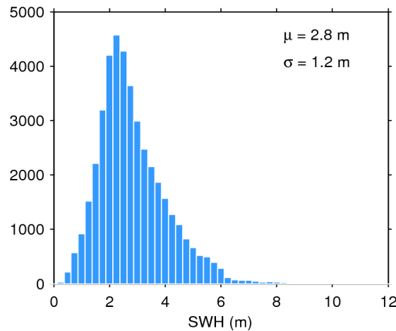
Figure 20. Histogram of science-valid SWH over oceans and lakes for 14/03/2019. The mean ( \mu ) and standard deviation ( \sigma ) are also shown. Note that values larger than 12 m are excluded from the histogram for the sake of readability but not from the computation of \mu and \sigma .
