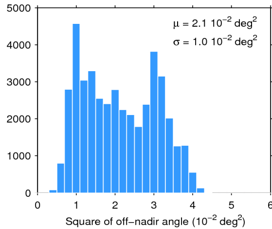
Figure 39. Histogram of flag-valid mispointing over oceans and lakes for 14/03/2019. The mean ( \mu ) and standard deviation ( \sigma ) are also shown. Note that values larger than 6 \cdot 10^{-2} \text{ deg}^2 are excluded from the histogram for the sake of readability but not from the computation of \mu and \sigma .
