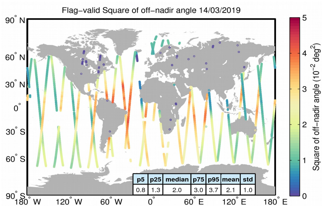
Figure 37. Geographical distribution of flag-valid mispointing data over oceans and lakes for 14/03/2019. The statistical values shown in the table refer to the mispointing in 10^{-2} deg 2 and are calculated over all measurements shown in the figure.
