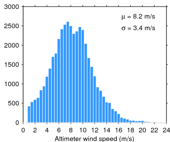
Figure 35. Histogram of science-valid wind over oceans and lakes for 14/03/2019. The mean ( \mu ) and standard deviation ( \sigma ) are also shown. Note that values larger than 24 m/s are excluded from the histogram for the sake of readability but not from the computation of \mu and \sigma .
