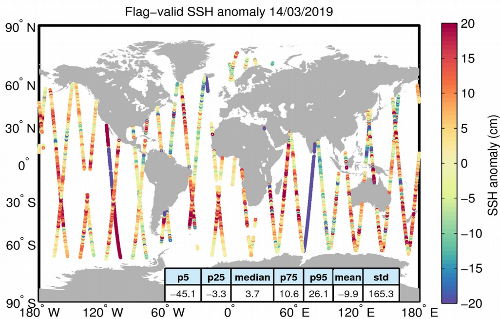
Figure 5. Geographical distribution of flag-valid 1-Hz SSH anomaly data over oceans and lakes for 14/03/2019. The statistical values shown in the table refer to the SSH anomaly in cm and are calculated over all measurements shown in the figure.
