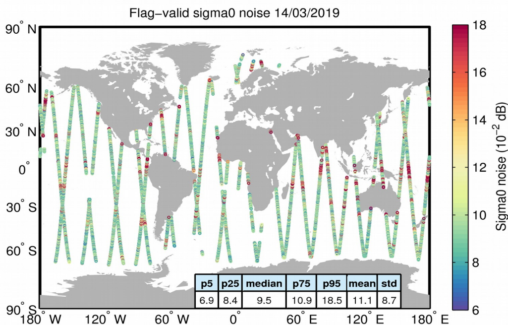
Figure 26. Geographical distribution of flag-valid 20-Hz sigma0 measurement noise over oceans and lakes for 14/03/2019. The statistical values shown in the table refer to the sigma0 noise and are calculated over all measurements shown in the figure.
