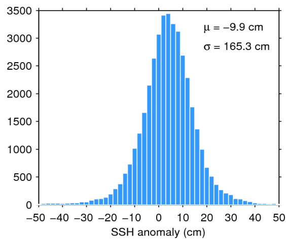
Figure 7. Histogram of flag-valid SSH anomaly over oceans and lakes for 14/03/2019. The mean ( \mu ) and standard deviation ( \sigma ) are also shown. Note that values outside [-50 50] cm are excluded from the histogram for the sake of readability but not from the computation of \mu and \sigma .
