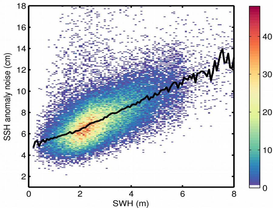
Figure 9. 2D histogram showing flag-valid SSH anomaly noise as a function of SWH for 14/03/2019. The black line denotes the median SSH anomaly noise as a function of SWH.
