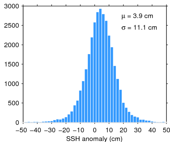
Figure 11. Histogram of science-valid SSH anomaly over oceans and lakes for 14/03/2019. The mean ( \mu ) and standard deviation ( \sigma ) are also shown. Note that values outside [-50 50] cm are excluded from the histogram for the sake of readability but not from the computation of \mu and \sigma .
