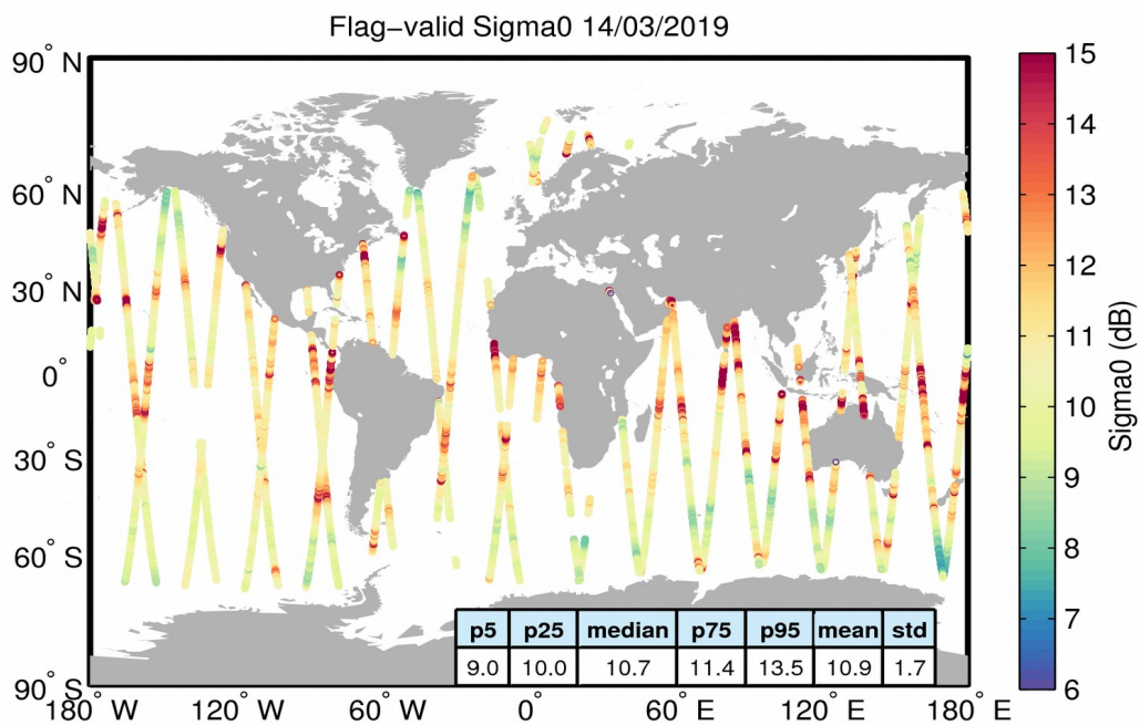
Figure 23. Geographical distribution of flag-valid sigma0 data over oceans and lakes for 14/03/2019. The statistical values shown in the table refer to the sigma0 in dB and are calculated over all measurements shown in the figure.
