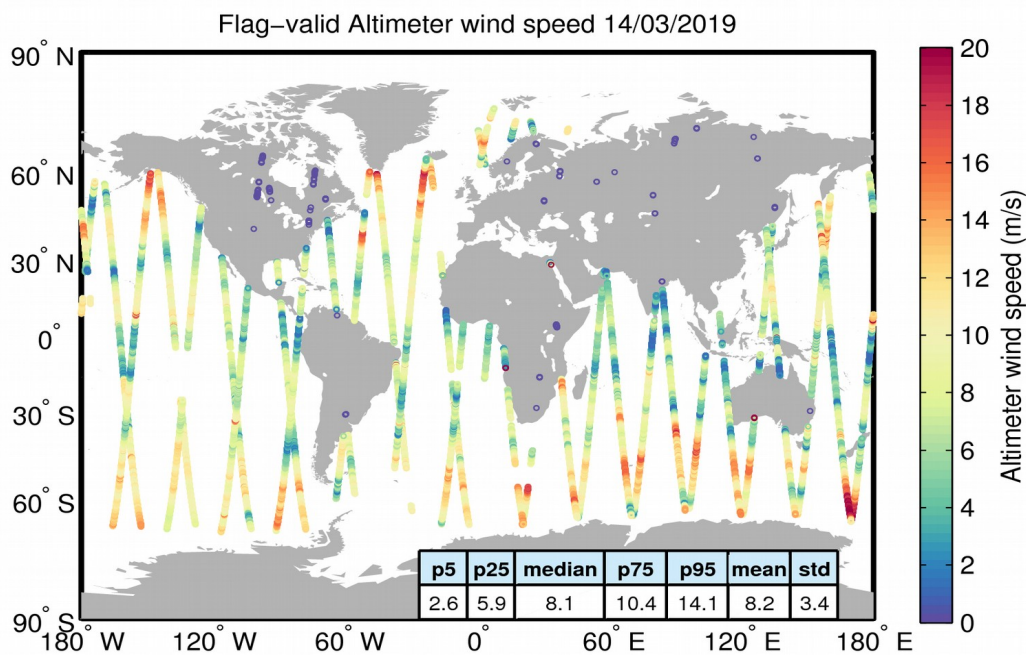
Figure 31. Geographical distribution of flag-valid wind data over oceans and lakes for 14/03/2019. The statistical values shown in the table refer to the wind in m/s and are calculated over all measurements shown in the figure.
