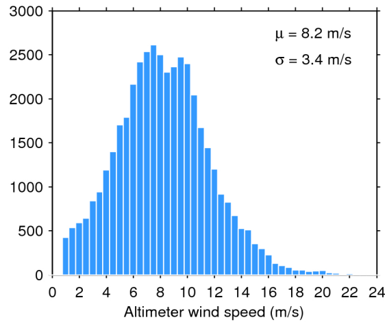
Figure 33. Histogram of flag-valid wind over oceans and lakes for 14/03/2019. The mean ( \mu ) and standard deviation ( \sigma ) are also shown. Note that values larger than 24 m/s are excluded from the histogram for the sake of readability but not from the computation of \mu and \sigma .
