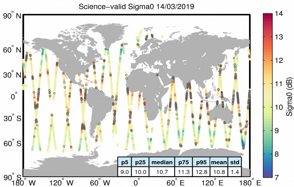
Figure 27. Geographical distribution of science-valid sigma0 data over oceans and lakes for 14/03/2019. The statistical values shown in the table refer to the sigma0 in dB and are calculated over all measurements shown in the figure. Gray circles denote records that have been rejected based on the editing criteria described in Table 4.
