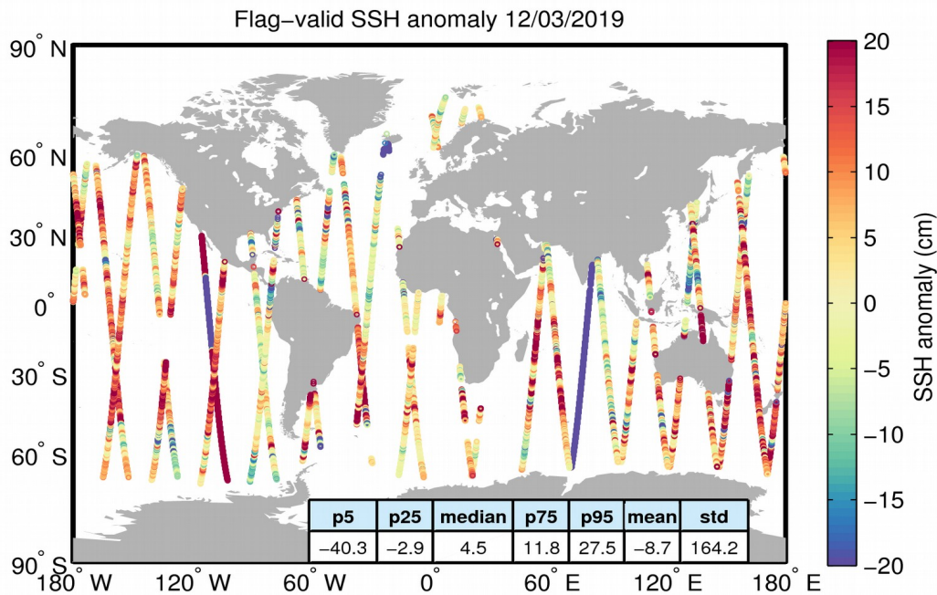
Figure 5. Geographical distribution of flag-valid 1-Hz SSH anomaly data over oceans and lakes for 12/03/2019. The statistical values shown in the table refer to the SSH anomaly in cm and are calculated over all measurements shown in the figure.
