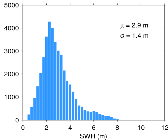
Figure 20. Histogram of science-valid SWH over oceans and lakes for 12/03/2019. The mean ( \mu ) and standard deviation ( \sigma ) are also shown. Note that values larger than 12 m are excluded from the histogram for the sake of readability but not from the computation of \mu and \sigma .
