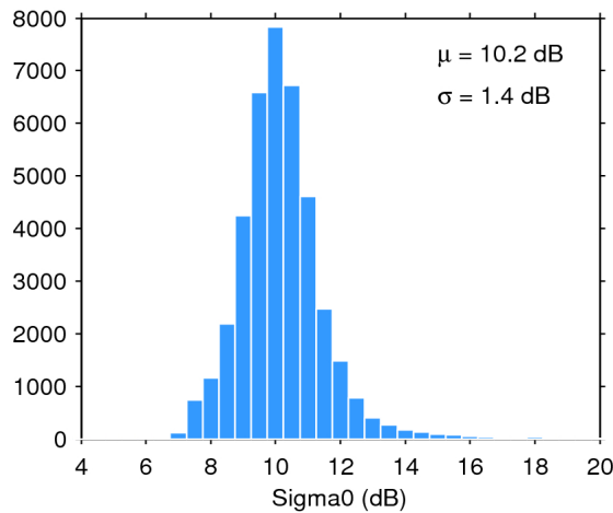
Figure 28. Histogram of science-valid sigma0 over oceans and lakes for 12/03/2019. The mean ( \mu ) and standard deviation ( \sigma ) are also shown. Note that values outside [4 20] dB are excluded from the histogram for the sake of readability but not from the computation of \mu and \sigma .
