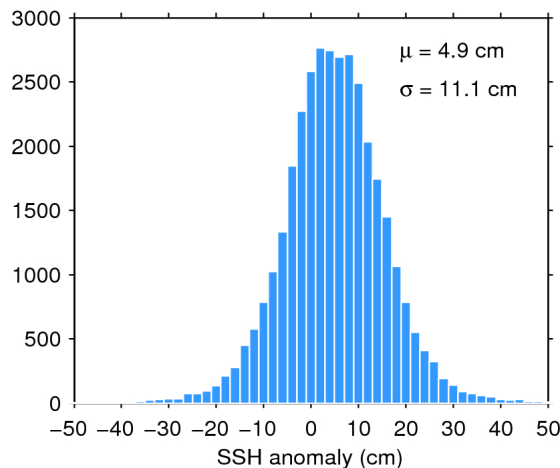
Figure 11. Histogram of science-valid SSH anomaly over oceans and lakes for 12/03/2019. The mean ( \mu ) and standard deviation ( \sigma ) are also shown. Note that values outside [-50 50] cm are excluded from the histogram for the sake of readability but not from the computation of \mu and \sigma .
