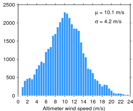
Figure 35. Histogram of science-valid wind over oceans and lakes for 12/03/2019. The mean ( \mu ) and standard deviation ( \sigma ) are also shown. Note that values larger than 24 m/s are excluded from the histogram for the sake of readability but not from the computation of \mu and \sigma .
