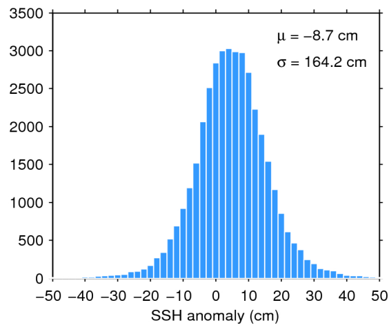
Figure 7. Histogram of flag-valid SSH anomaly over oceans and lakes for 12/03/2019. The mean ( \mu ) and standard deviation ( \sigma ) are also shown. Note that values outside [-50 50] cm are excluded from the histogram for the sake of readability but not from the computation of \mu and \sigma .
