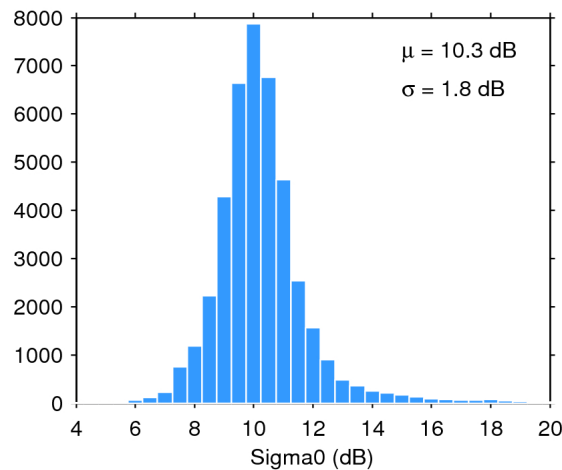
Figure 25. Histogram of flag-valid sigma0 over oceans and lakes for 12/03/2019. The mean ( \mu ) and standard deviation ( \sigma ) are also shown. Note that values outside [4 20] dB are excluded from the histogram for the sake of readability but not from the computation of \mu and \sigma .
