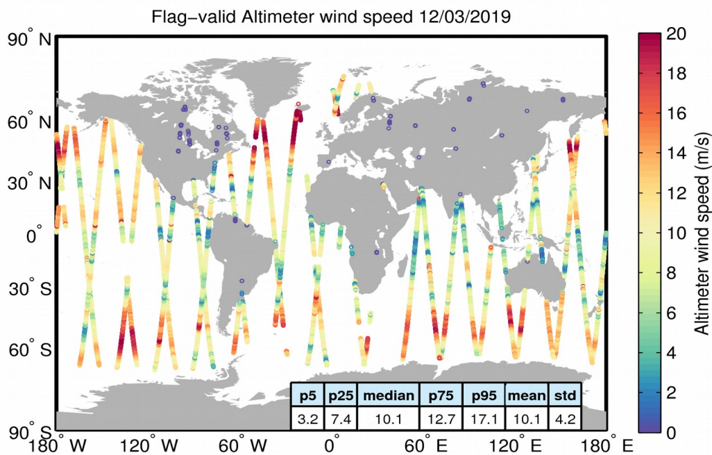
Figure 31. Geographical distribution of flag-valid wind data over oceans and lakes for 12/03/2019. The statistical values shown in the table refer to the wind in m/s and are calculated over all measurements shown in the figure.
