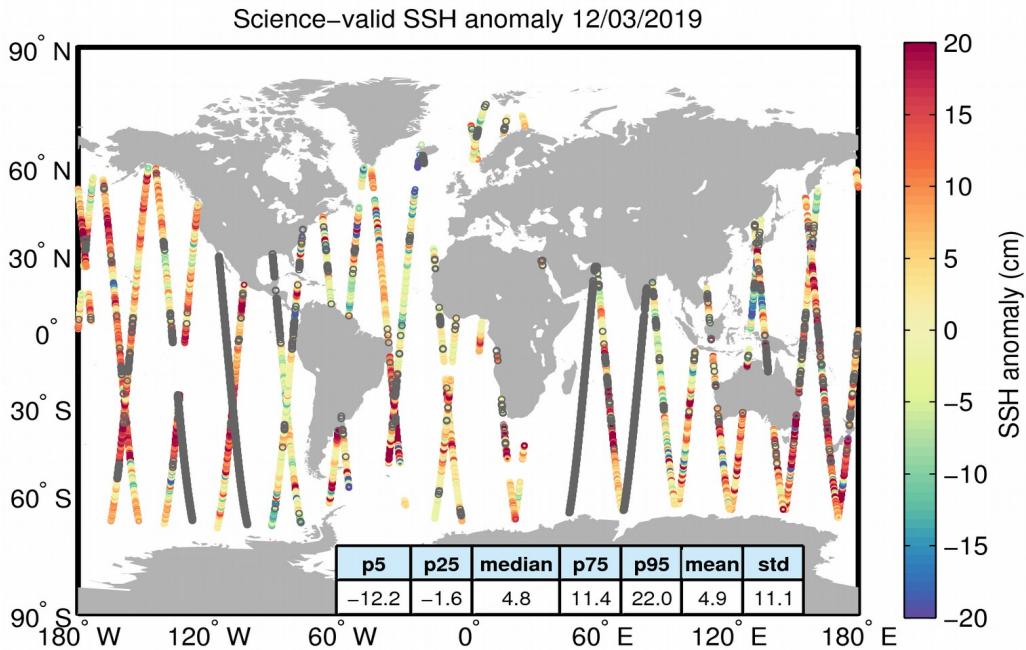
Figure 10. Geographical distribution of science-valid SSH anomaly data over oceans and lakes for 12/03/2019. The statistical values shown in the table refer to the SSH anomaly in cm and are calculated over all measurements shown in the figure. Gray circles denote records that have been rejected based on the editing criteria described in Table 2.
