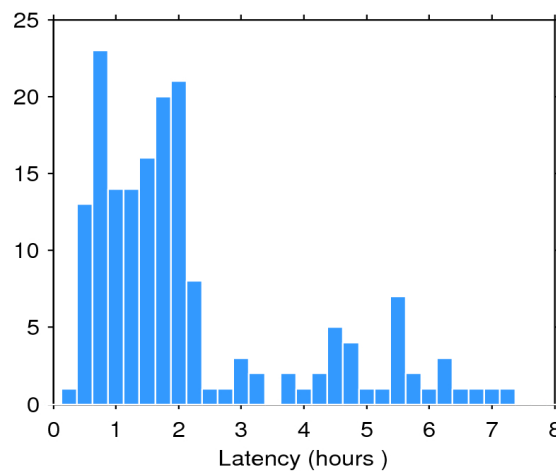
Figure 2. Histogram of the data latency for 12/03/2019. The y-axis denotes the number of files that are made available with a delay of x-hours with respect to the mean time of the records stored in the file.
