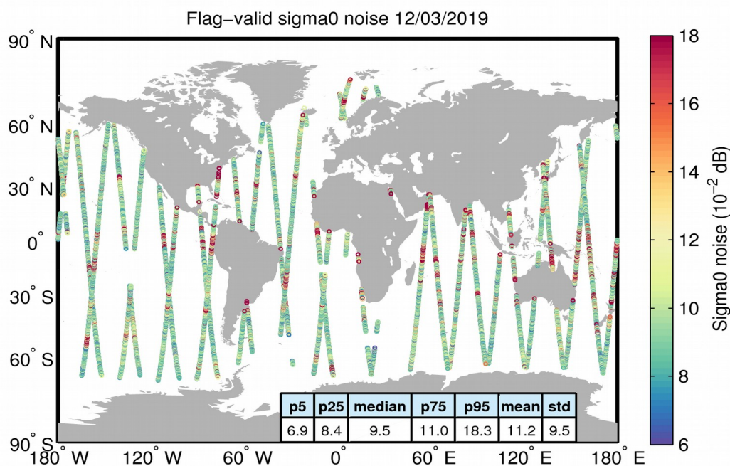
Figure 26. Geographical distribution of flag-valid 20-Hz sigma0 measurement noise over oceans and lakes for 12/03/2019. The statistical values shown in the table refer to the sigma0 noise and are calculated over all measurements shown in the figure.
