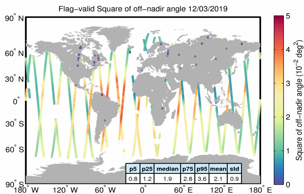
Figure 37. Geographical distribution of flag-valid mispointing data over oceans and lakes for 12/03/2019. The statistical values shown in the table refer to the mispointing in 10^{-2} deg 2 and are calculated over all measurements shown in the figure.
