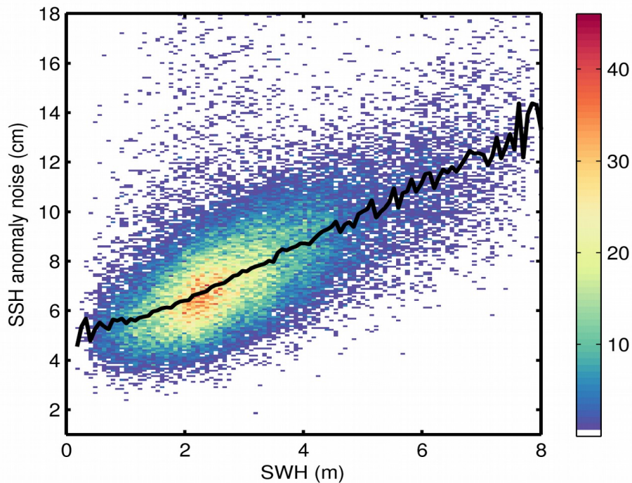
Figure 9. 2D histogram showing flag-valid SSH anomaly noise as a function of SWH for 12/03/2019. The black line denotes the median SSH anomaly noise as a function of SWH.
