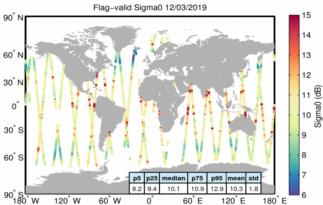
Figure 23. Geographical distribution of flag-valid sigma0 data over oceans and lakes for 12/03/2019. The statistical values shown in the table refer to the sigma0 in dB and are calculated over all measurements shown in the figure.
