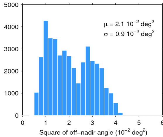
Figure 39. Histogram of flag-valid mispointing over oceans and lakes for 12/03/2019. The mean ( \mu ) and standard deviation ( \sigma ) are also shown. Note that values larger than 6 \cdot 10^{-2} \text{ deg}^2 are excluded from the histogram for the sake of readability but not from the computation of \mu and \sigma .
