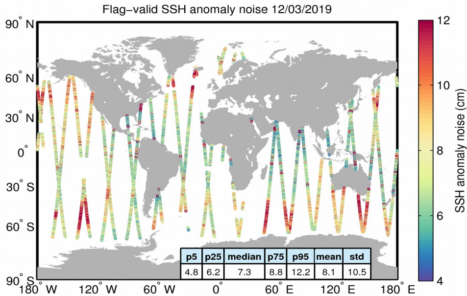
Figure 8. Geographical distribution of flag-valid 20-Hz SSH anomaly measurement noise over oceans and lakes for 12/03/2019. The statistical values shown in the table refer to the SSH anomaly noise and are calculated over all measurements shown in the figure.
