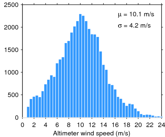
Figure 33. Histogram of flag-valid wind over oceans and lakes for 12/03/2019. The mean ( \mu ) and standard deviation ( \sigma ) are also shown. Note that values larger than 24 m/s are excluded from the histogram for the sake of readability but not from the computation of \mu and \sigma .
