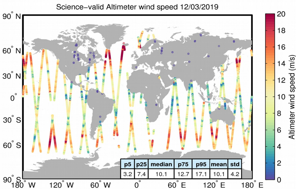
Figure 34. Geographical distribution of science-valid wind data over oceans and lakes for 12/03/2019. The statistical values shown in the table refer to the wind in m/s and are calculated over all measurements shown in the figure. Gray circles denote records that have been rejected based on the editing criteria described in Table 5.
