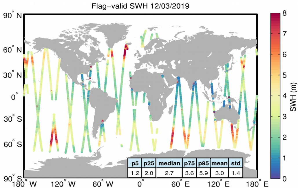
Figure 15. Geographical distribution of flag-valid SWH data over oceans and lakes for 12/03/2019. The statistical values shown in the table refer to the SWH in m and are calculated over all measurements shown in the figure.
