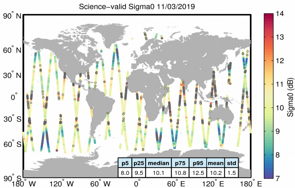
Figure 27. Geographical distribution of science-valid sigma0 data over oceans and lakes for 11/03/2019. The statistical values shown in the table refer to the sigma0 in dB and are calculated over all measurements shown in the figure. Gray circles denote records that have been rejected based on the editing criteria described in Table 4.
