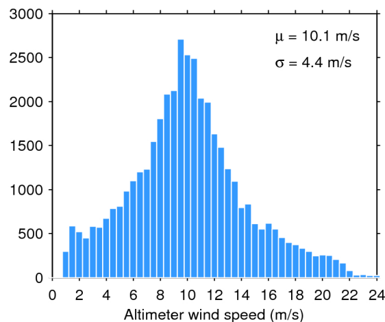
Figure 35. Histogram of science-valid wind over oceans and lakes for 11/03/2019. The mean ( \mu ) and standard deviation ( \sigma ) are also shown. Note that values larger than 24 m/s are excluded from the histogram for the sake of readability but not from the computation of \mu and \sigma .
