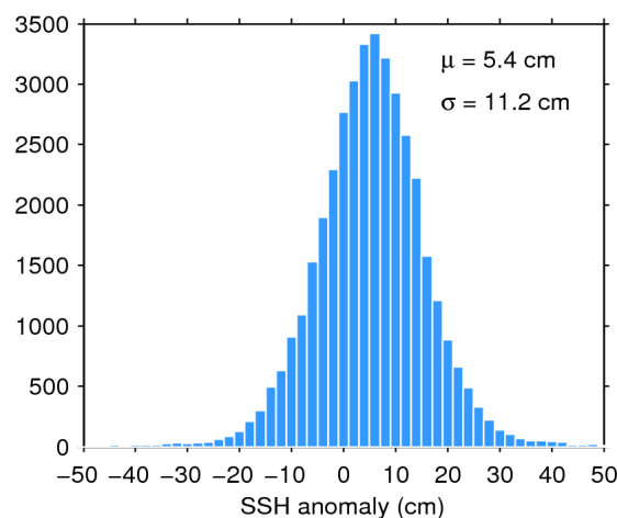
Figure 11. Histogram of science-valid SSH anomaly over oceans and lakes for 11/03/2019. The mean ( \mu ) and standard deviation ( \sigma ) are also shown. Note that values outside [-50 50] cm are excluded from the histogram for the sake of readability but not from the computation of \mu and \sigma .
