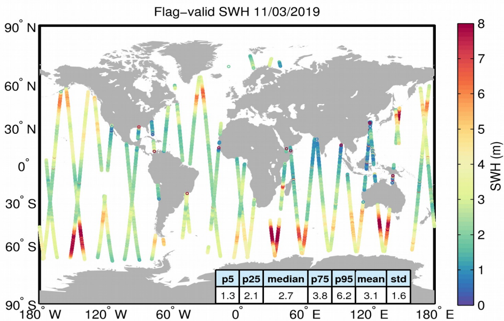
Figure 15. Geographical distribution of flag-valid SWH data over oceans and lakes for 11/03/2019. The statistical values shown in the table refer to the SWH in m and are calculated over all measurements shown in the figure.
