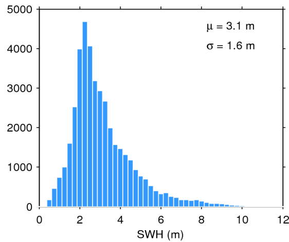
Figure 17. Histogram of flag-valid SWH over oceans and lakes for 11/03/2019. The mean ( \mu ) and standard deviation ( \sigma ) are also shown. Note that values larger than 12 m are excluded from the histogram for the sake of readability but not from the computation of \mu and \sigma .
