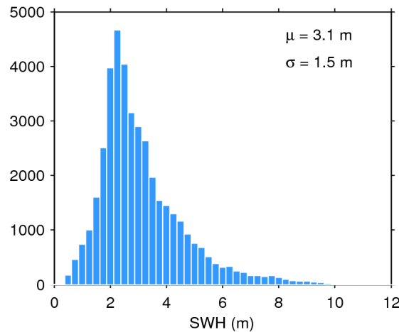
Figure 20. Histogram of science-valid SWH over oceans and lakes for 11/03/2019. The mean ( \mu ) and standard deviation ( \sigma ) are also shown. Note that values larger than 12 m are excluded from the histogram for the sake of readability but not from the computation of \mu and \sigma .
