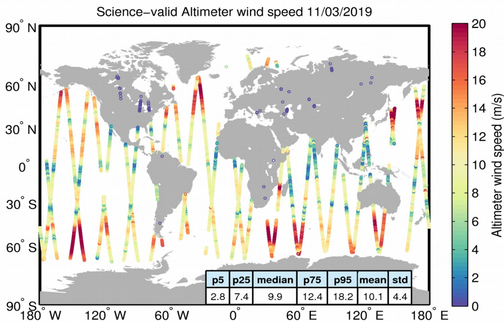
Figure 34. Geographical distribution of science-valid wind data over oceans and lakes for 11/03/2019. The statistical values shown in the table refer to the wind in m/s and are calculated over all measurements shown in the figure. Gray circles denote records that have been rejected based on the editing criteria described in Table 5.
