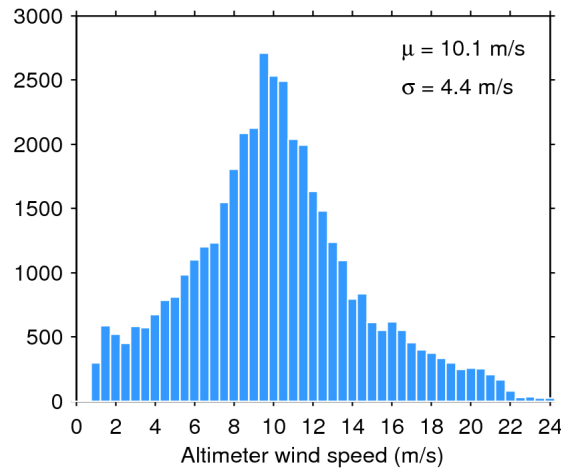
Figure 33. Histogram of flag-valid wind over oceans and lakes for 11/03/2019. The mean ( \mu ) and standard deviation ( \sigma ) are also shown. Note that values larger than 24 m/s are excluded from the histogram for the sake of readability but not from the computation of \mu and \sigma .
