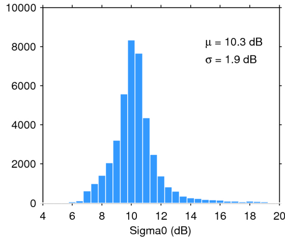
Figure 25. Histogram of flag-valid sigma0 over oceans and lakes for 11/03/2019. The mean ( \mu ) and standard deviation ( \sigma ) are also shown. Note that values outside [4 20] dB are excluded from the histogram for the sake of readability but not from the computation of \mu and \sigma .
