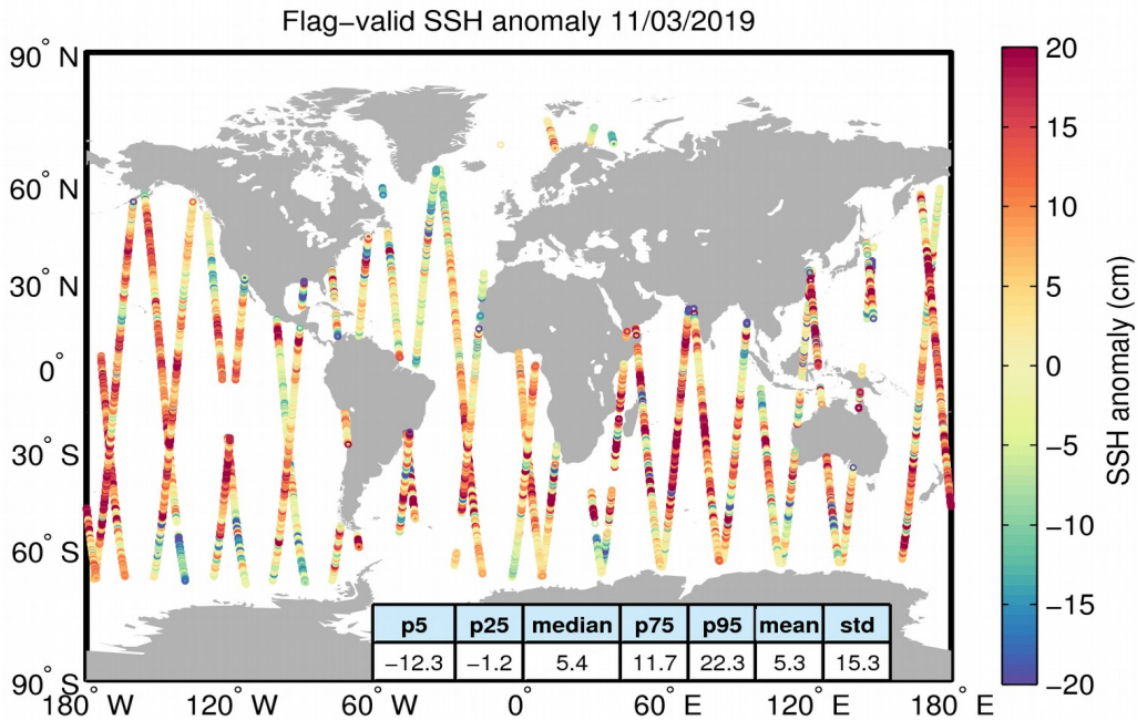
Figure 5. Geographical distribution of flag-valid 1-Hz SSH anomaly data over oceans and lakes for 11/03/2019. The statistical values shown in the table refer to the SSH anomaly in cm and are calculated over all measurements shown in the figure.
