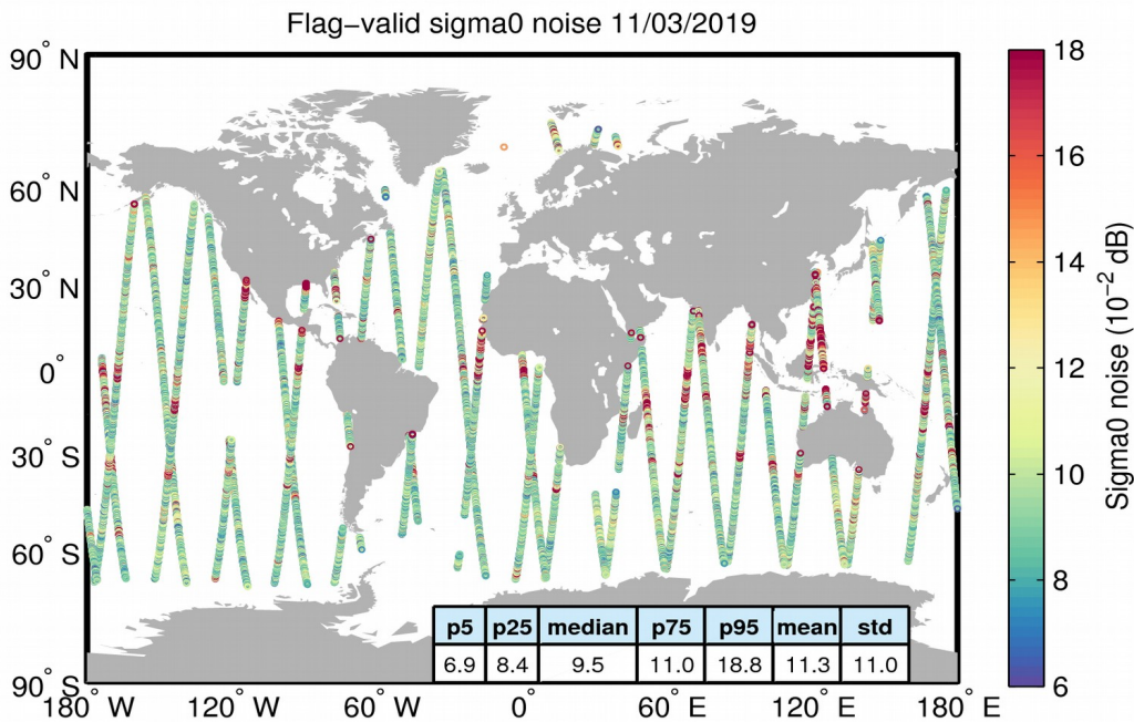
Figure 26. Geographical distribution of flag-valid 20-Hz sigma0 measurement noise over oceans and lakes for 11/03/2019. The statistical values shown in the table refer to the sigma0 noise and are calculated over all measurements shown in the figure.
