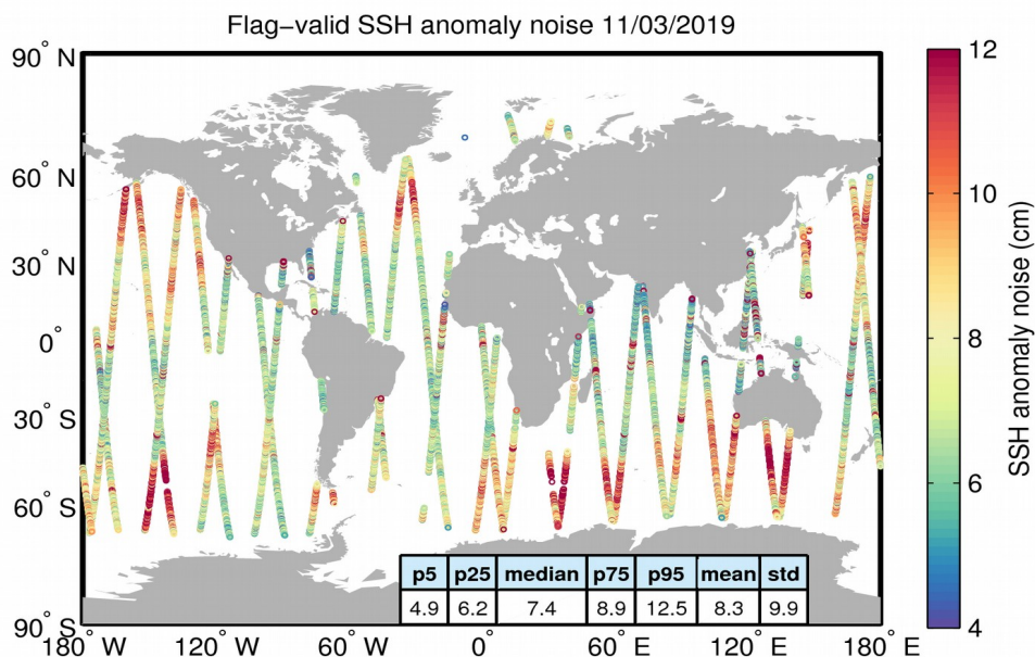
Figure 8. Geographical distribution of flag-valid 20-Hz SSH anomaly measurement noise over oceans and lakes for 11/03/2019. The statistical values shown in the table refer to the SSH anomaly noise and are calculated over all measurements shown in the figure.
