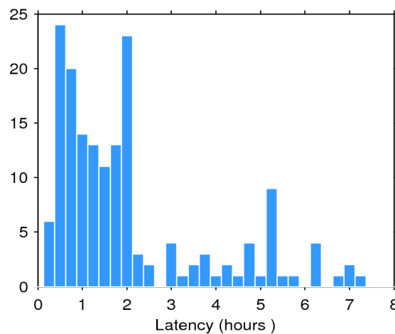
Figure 2. Histogram of the data latency for 08/03/2019. The y-axis denotes the number of files that are made available with a delay of x-hours with respect to the mean time of the records stored in the file.
