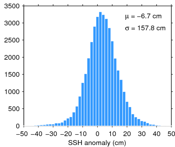
Figure 7. Histogram of flag-valid SSH anomaly over oceans and lakes for 08/03/2019. The mean ( \mu ) and standard deviation ( \sigma ) are also shown. Note that values outside [-50 50] cm are excluded from the histogram for the sake of readability but not from the computation of \mu and \sigma .
