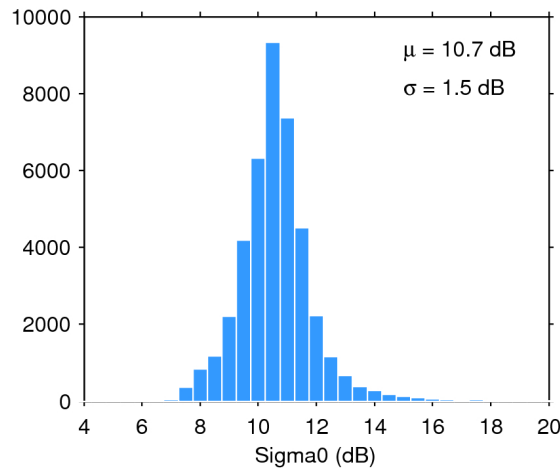
Figure 28. Histogram of science-valid sigma0 over oceans and lakes for 08/03/2019. The mean ( \mu ) and standard deviation ( \sigma ) are also shown. Note that values outside [4 20] dB are excluded from the histogram for the sake of readability but not from the computation of \mu and \sigma .
