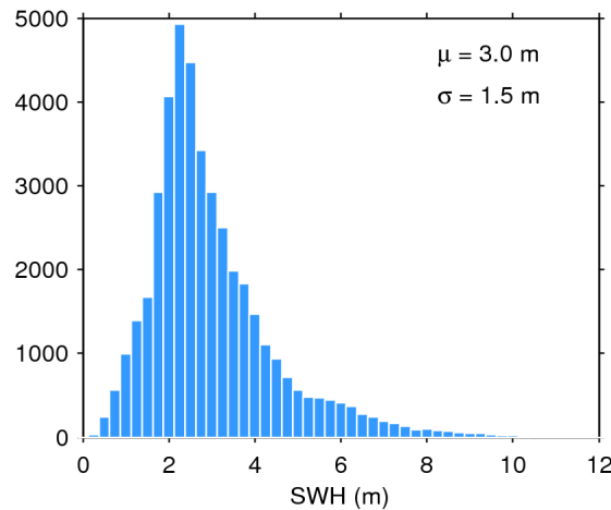
Figure 20. Histogram of science-valid SWH over oceans and lakes for 08/03/2019. The mean ( \mu ) and standard deviation ( \sigma ) are also shown. Note that values larger than 12 m are excluded from the histogram for the sake of readability but not from the computation of \mu and \sigma .
