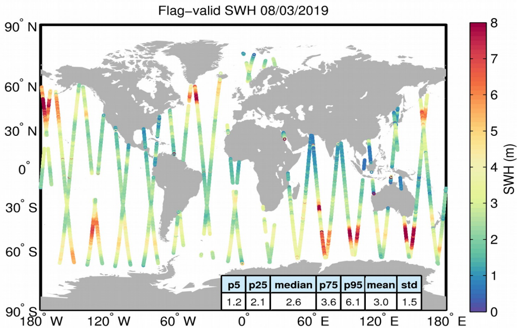
Figure 15. Geographical distribution of flag-valid SWH data over oceans and lakes for 08/03/2019. The statistical values shown in the table refer to the SWH in m and are calculated over all measurements shown in the figure.
