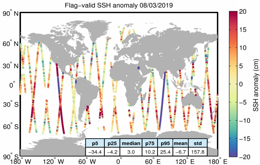
Figure 5. Geographical distribution of flag-valid 1-Hz SSH anomaly data over oceans and lakes for 08/03/2019. The statistical values shown in the table refer to the SSH anomaly in cm and are calculated over all measurements shown in the figure.
