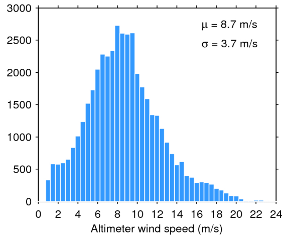
Figure 33. Histogram of flag-valid wind over oceans and lakes for 08/03/2019. The mean ( \mu ) and standard deviation ( \sigma ) are also shown. Note that values larger than 24 m/s are excluded from the histogram for the sake of readability but not from the computation of \mu and \sigma .
