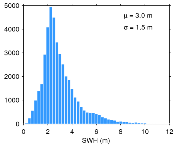
Figure 17. Histogram of flag-valid SWH over oceans and lakes for 08/03/2019. The mean ( \mu ) and standard deviation ( \sigma ) are also shown. Note that values larger than 12 m are excluded from the histogram for the sake of readability but not from the computation of \mu and \sigma .
