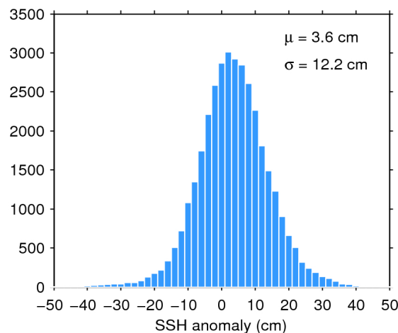
Figure 11. Histogram of science-valid SSH anomaly over oceans and lakes for 08/03/2019. The mean ( \mu ) and standard deviation ( \sigma ) are also shown. Note that values outside [-50 50] cm are excluded from the histogram for the sake of readability but not from the computation of \mu and \sigma .
