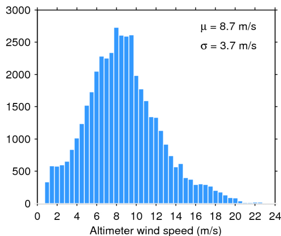
Figure 35. Histogram of science-valid wind over oceans and lakes for 08/03/2019. The mean ( \mu ) and standard deviation ( \sigma ) are also shown. Note that values larger than 24 m/s are excluded from the histogram for the sake of readability but not from the computation of \mu and \sigma .
