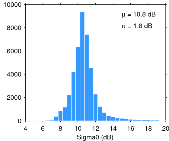
Figure 25. Histogram of flag-valid sigma0 over oceans and lakes for 08/03/2019. The mean ( \mu ) and standard deviation ( \sigma ) are also shown. Note that values outside [4 20] dB are excluded from the histogram for the sake of readability but not from the computation of \mu and \sigma .
