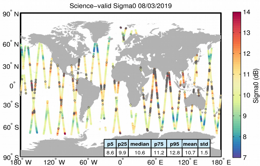
Figure 27. Geographical distribution of science-valid sigma0 data over oceans and lakes for 08/03/2019. The statistical values shown in the table refer to the sigma0 in dB and are calculated over all measurements shown in the figure. Gray circles denote records that have been rejected based on the editing criteria described in Table 4.
