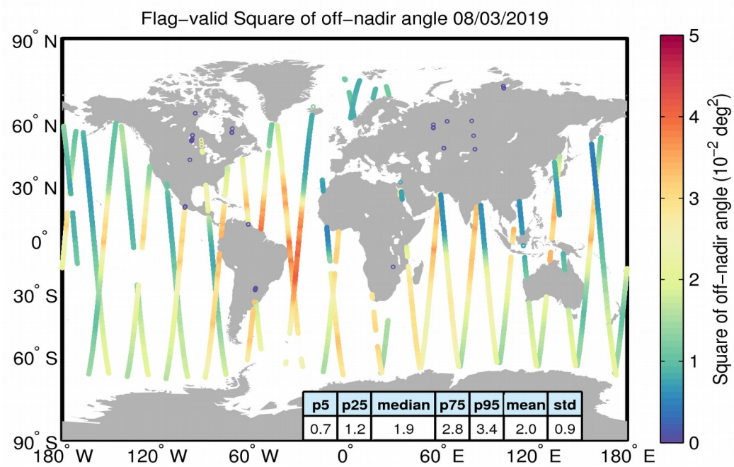
Figure 37. Geographical distribution of flag-valid mispointing data over oceans and lakes for 08/03/2019. The statistical values shown in the table refer to the mispointing in 10^{-2} \text{deg}^2 and are calculated over all measurements shown in the figure.
