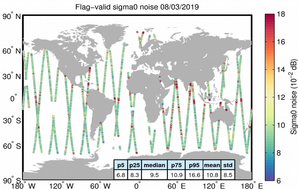
Figure 26. Geographical distribution of flag-valid 20-Hz sigma0 measurement noise over oceans and lakes for 08/03/2019. The statistical values shown in the table refer to the sigma0 noise and are calculated over all measurements shown in the figure.
