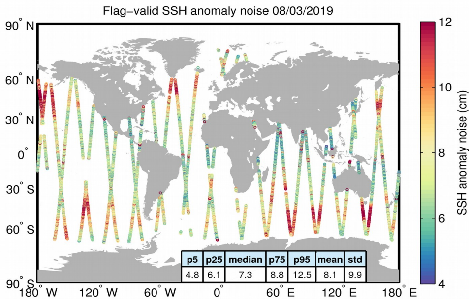
Figure 8. Geographical distribution of flag-valid 20-Hz SSH anomaly measurement noise over oceans and lakes for 08/03/2019. The statistical values shown in the table refer to the SSH anomaly noise and are calculated over all measurements shown in the figure.
