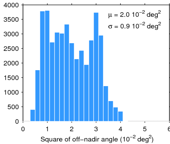
Figure 39. Histogram of flag-valid mispointing over oceans and lakes for 08/03/2019. The mean ( \mu ) and standard deviation ( \sigma ) are also shown. Note that values larger than 6 \cdot 10^{-2} \text{ deg}^2 are excluded from the histogram for the sake of readability but not from the computation of \mu and \sigma .
