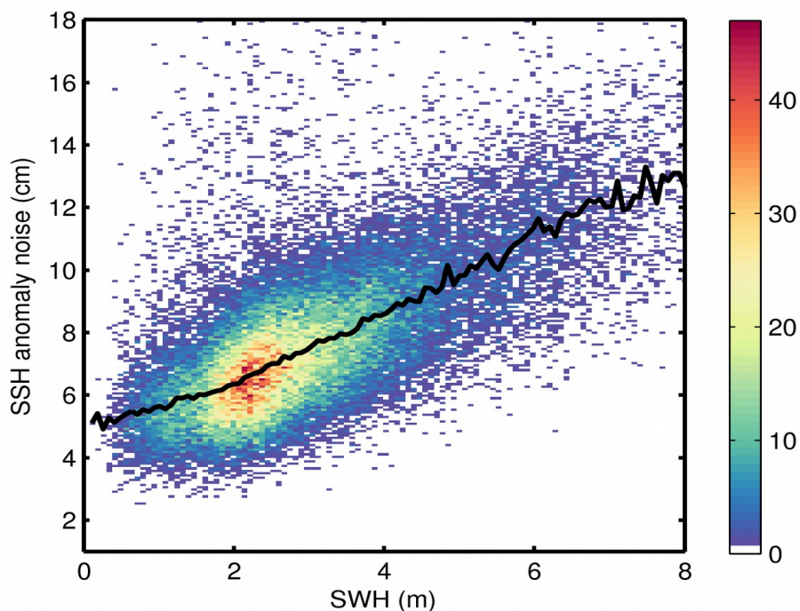
Figure 9. 2D histogram showing flag-valid SSH anomaly noise as a function of SWH for 08/03/2019. The black line denotes the median SSH anomaly noise as a function of SWH.
