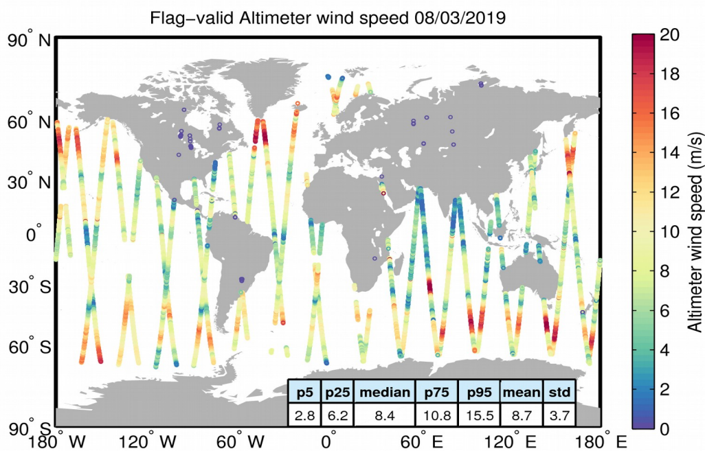
Figure 31. Geographical distribution of flag-valid wind data over oceans and lakes for 08/03/2019. The statistical values shown in the table refer to the wind in m/s and are calculated over all measurements shown in the figure.
