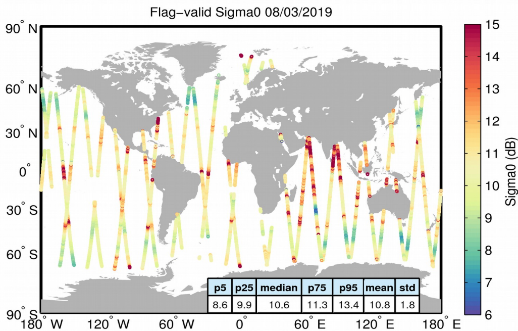
Figure 23. Geographical distribution of flag-valid sigma0 data over oceans and lakes for 08/03/2019. The statistical values shown in the table refer to the sigma0 in dB and are calculated over all measurements shown in the figure.
