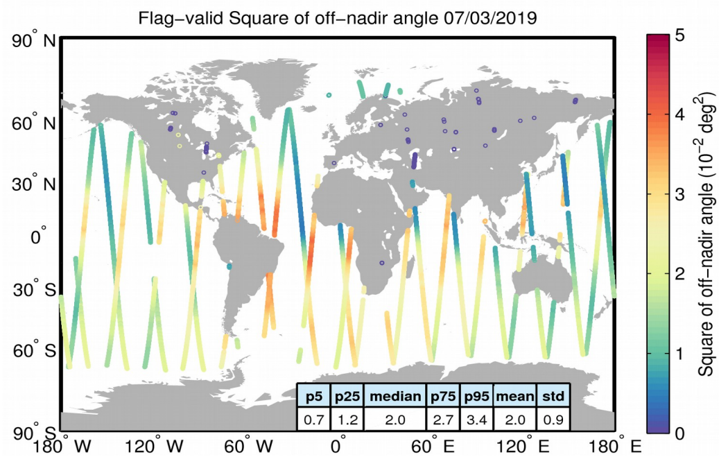
Figure 37. Geographical distribution of flag-valid mispointing data over oceans and lakes for 07/03/2019. The statistical values shown in the table refer to the mispointing in 10^{-2} \text{ deg}^2 and are calculated over all measurements shown in the figure.
