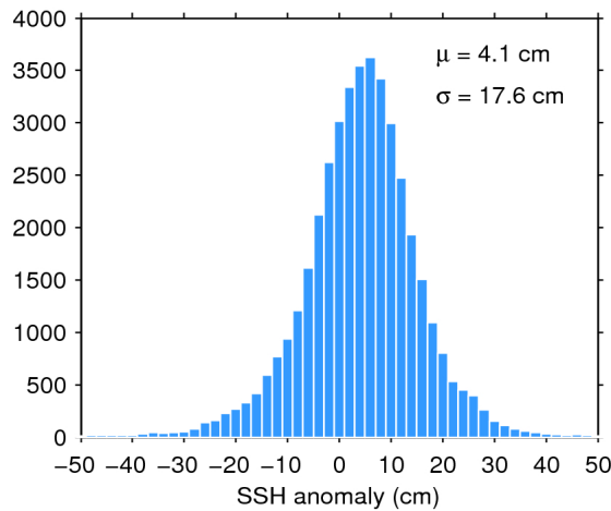
Figure 7. Histogram of flag-valid SSH anomaly over oceans and lakes for 07/03/2019. The mean ( \mu ) and standard deviation ( \sigma ) are also shown. Note that values outside [-50\ 50] cm are excluded from the histogram for the sake of readability but not from the computation of \mu and \sigma .
