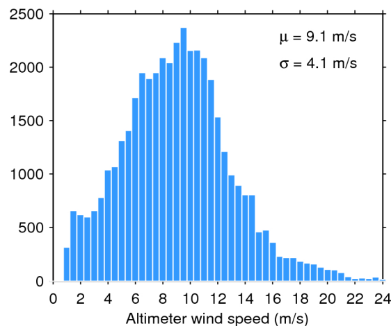
Figure 35. Histogram of science-valid wind over oceans and lakes for 07/03/2019. The mean ( \mu ) and standard deviation ( \sigma ) are also shown. Note that values larger than 24 m/s are excluded from the histogram for the sake of readability but not from the computation of \mu and \sigma .
