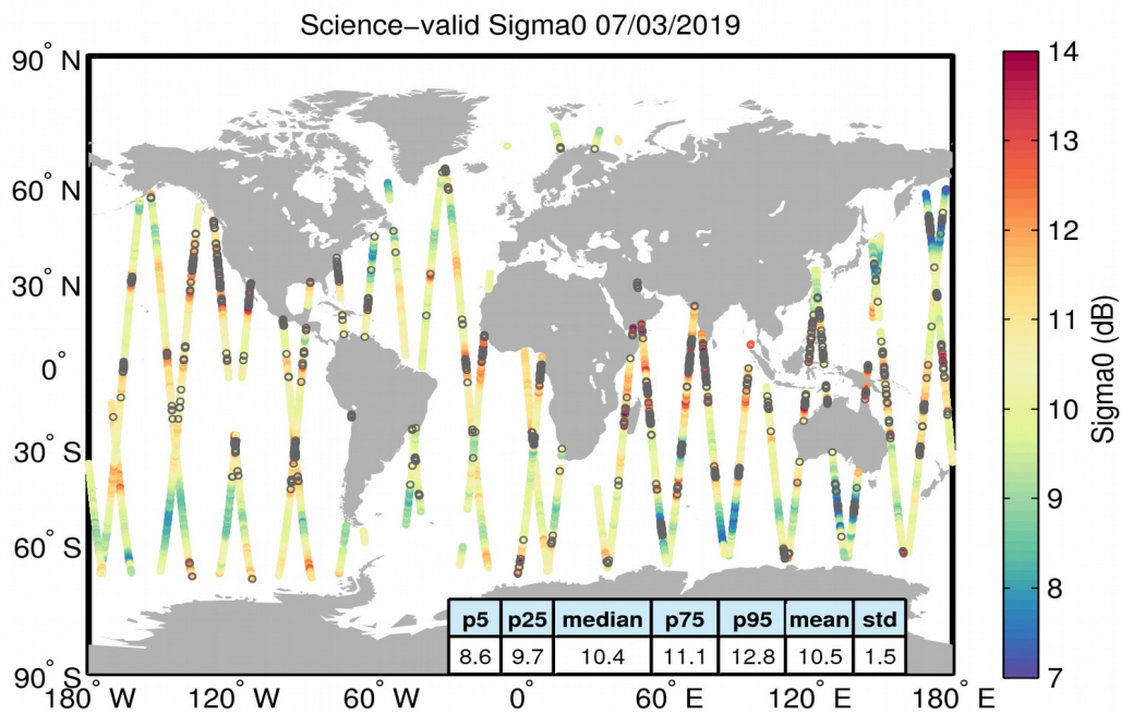
Figure 27. Geographical distribution of science-valid sigma0 data over oceans and lakes for 07/03/2019. The statistical values shown in the table refer to the sigma0 in dB and are calculated over all measurements shown in the figure. Gray circles denote records that have been rejected based on the editing criteria described in Table 4.
