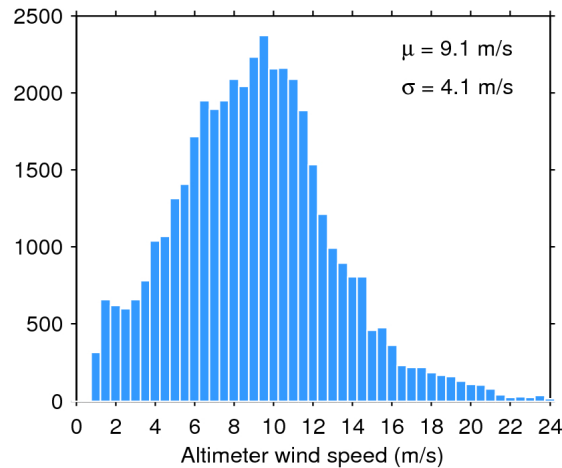
Figure 33. Histogram of flag-valid wind over oceans and lakes for 07/03/2019. The mean ( \mu ) and standard deviation ( \sigma ) are also shown. Note that values larger than 24 m/s are excluded from the histogram for the sake of readability but not from the computation of \mu and \sigma .
