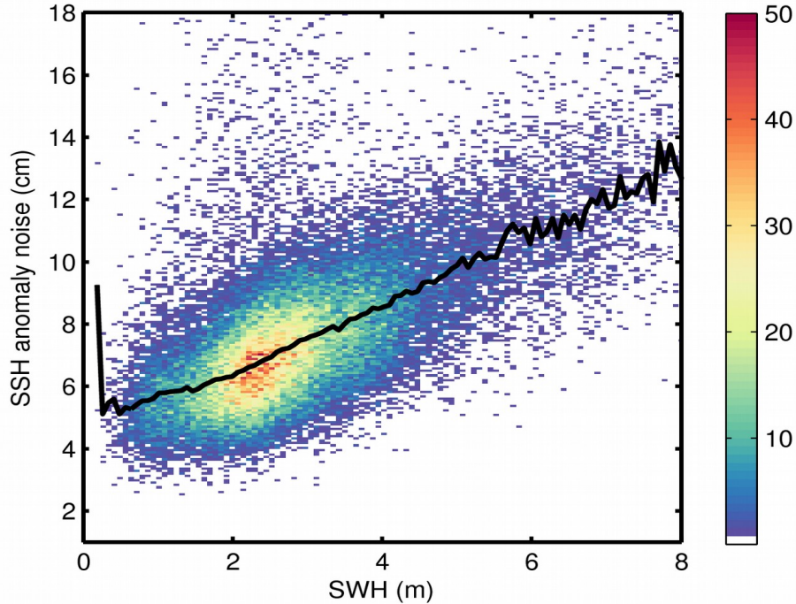
Figure 9. 2D histogram showing flag-valid SSH anomaly noise as a function of SWH for 07/03/2019. The black line denotes the median SSH anomaly noise as a function of SWH.
