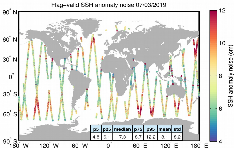
Figure 8. Geographical distribution of flag-valid 20-Hz SSH anomaly measurement noise over oceans and lakes for 07/03/2019. The statistical values shown in the table refer to the SSH anomaly noise and are calculated over all measurements shown in the figure.
