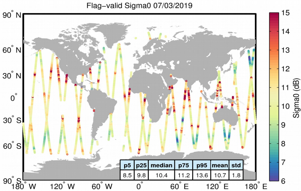
Figure 23. Geographical distribution of flag-valid sigma0 data over oceans and lakes for 07/03/2019. The statistical values shown in the table refer to the sigma0 in dB and are calculated over all measurements shown in the figure.
