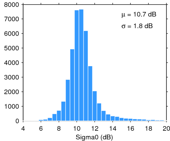
Figure 25. Histogram of flag-valid sigma0 over oceans and lakes for 07/03/2019. The mean ( \mu ) and standard deviation ( \sigma ) are also shown. Note that values outside [4 20] dB are excluded from the histogram for the sake of readability but not from the computation of \mu and \sigma .
