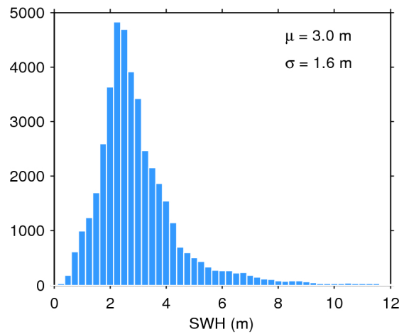
Figure 17. Histogram of flag-valid SWH over oceans and lakes for 07/03/2019. The mean ( \mu ) and standard deviation ( \sigma ) are also shown. Note that values larger than 12 m are excluded from the histogram for the sake of readability but not from the computation of \mu and \sigma .
