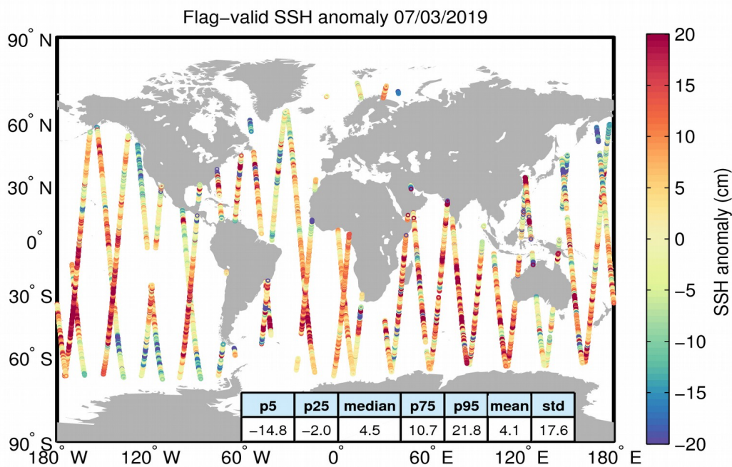
Figure 5. Geographical distribution of flag-valid 1-Hz SSH anomaly data over oceans and lakes for 07/03/2019. The statistical values shown in the table refer to the SSH anomaly in cm and are calculated over all measurements shown in the figure.
