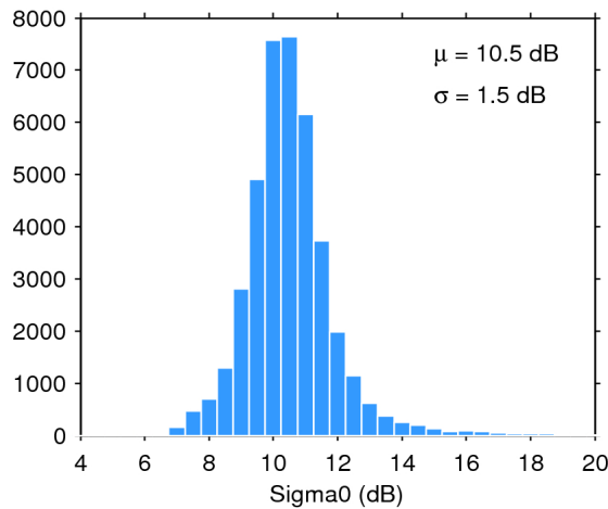
Figure 28. Histogram of science-valid sigma0 over oceans and lakes for 07/03/2019. The mean ( \mu ) and standard deviation ( \sigma ) are also shown. Note that values outside [4 20] dB are excluded from the histogram for the sake of readability but not from the computation of \mu and \sigma .
