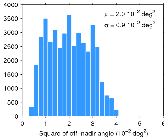
Figure 39. Histogram of flag-valid mispointing over oceans and lakes for 07/03/2019. The mean ( \mu ) and standard deviation ( \sigma ) are also shown. Note that values larger than 6 \cdot 10^{-2} \text{ deg}^2 are excluded from the histogram for the sake of readability but not from the computation of \mu and \sigma .
