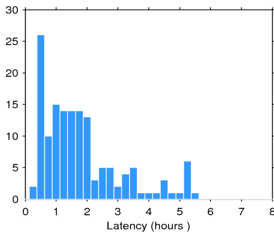
Figure 2. Histogram of the data latency for 07/03/2019. The y-axis denotes the number of files that are made available with a delay of x-hours with respect to the mean time of the records stored in the file.
