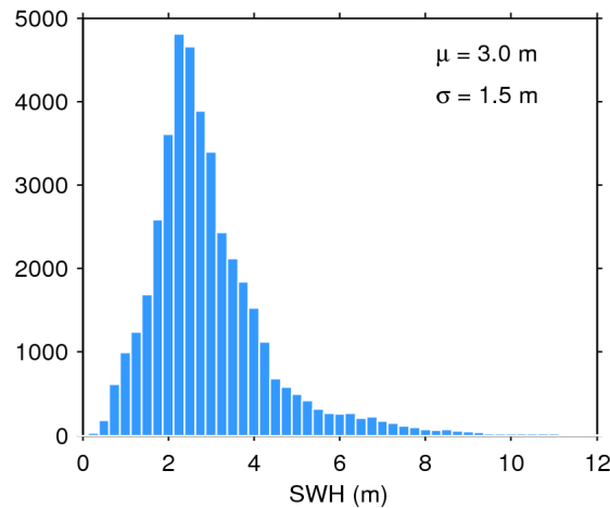
Figure 20. Histogram of science-valid SWH over oceans and lakes for 07/03/2019. The mean ( \mu ) and standard deviation ( \sigma ) are also shown. Note that values larger than 12 m are excluded from the histogram for the sake of readability but not from the computation of \mu and \sigma .
