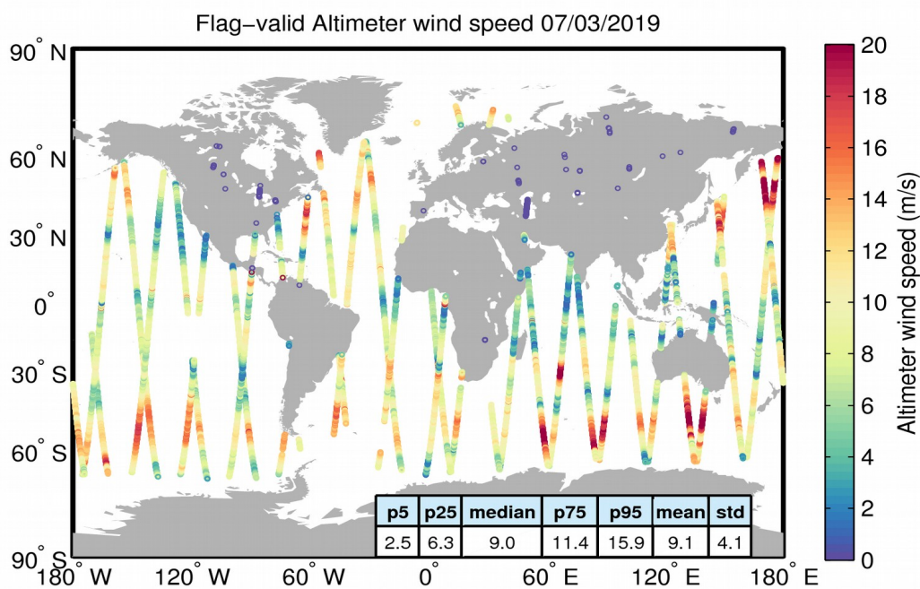
Figure 31. Geographical distribution of flag-valid wind data over oceans and lakes for 07/03/2019. The statistical values shown in the table refer to the wind in m/s and are calculated over all measurements shown in the figure.
