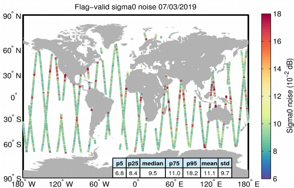
Figure 26. Geographical distribution of flag-valid 20-Hz sigma0 measurement noise over oceans and lakes for 07/03/2019. The statistical values shown in the table refer to the sigma0 noise and are calculated over all measurements shown in the figure.
