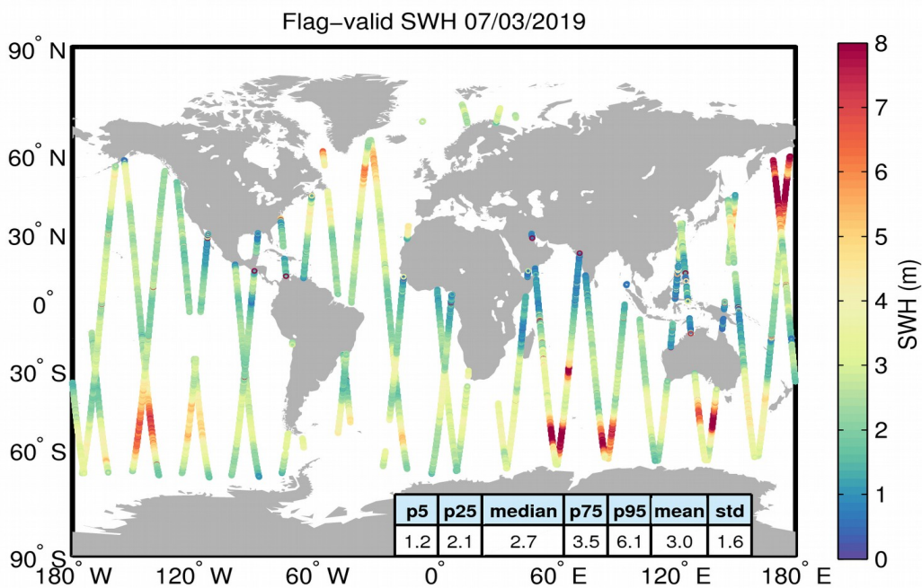
Figure 15. Geographical distribution of flag-valid SWH data over oceans and lakes for 07/03/2019. The statistical values shown in the table refer to the SWH in m and are calculated over all measurements shown in the figure.
