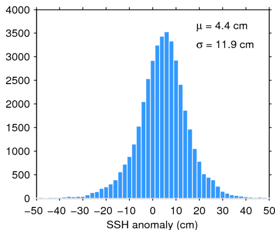
Figure 11. Histogram of science-valid SSH anomaly over oceans and lakes for 07/03/2019. The mean ( \mu ) and standard deviation ( \sigma ) are also shown. Note that values outside [-50 50] cm are excluded from the histogram for the sake of readability but not from the computation of \mu and \sigma .
