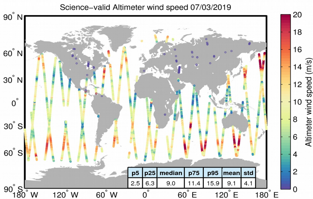
Figure 34. Geographical distribution of science-valid wind data over oceans and lakes for 07/03/2019. The statistical values shown in the table refer to the wind in m/s and are calculated over all measurements shown in the figure. Gray circles denote records that have been rejected based on the editing criteria described in Table 5.
