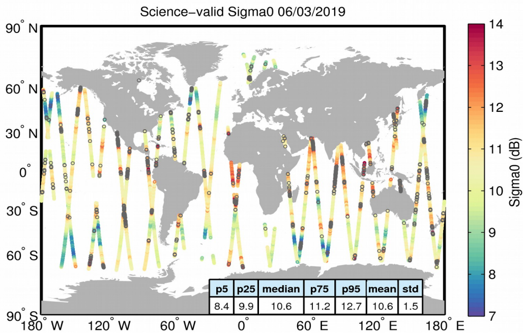
Figure 27. Geographical distribution of science-valid sigma0 data over oceans and lakes for 06/03/2019. The statistical values shown in the table refer to the sigma0 in dB and are calculated over all measurements shown in the figure. Gray circles denote records that have been rejected based on the editing criteria described in Table 4.
