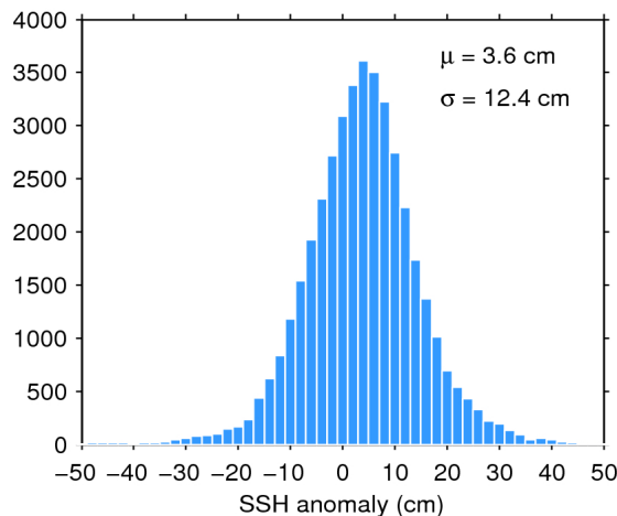
Figure 11. Histogram of science-valid SSH anomaly over oceans and lakes for 06/03/2019. The mean ( \mu ) and standard deviation ( \sigma ) are also shown. Note that values outside [-50 50] cm are excluded from the histogram for the sake of readability but not from the computation of \mu and \sigma .
