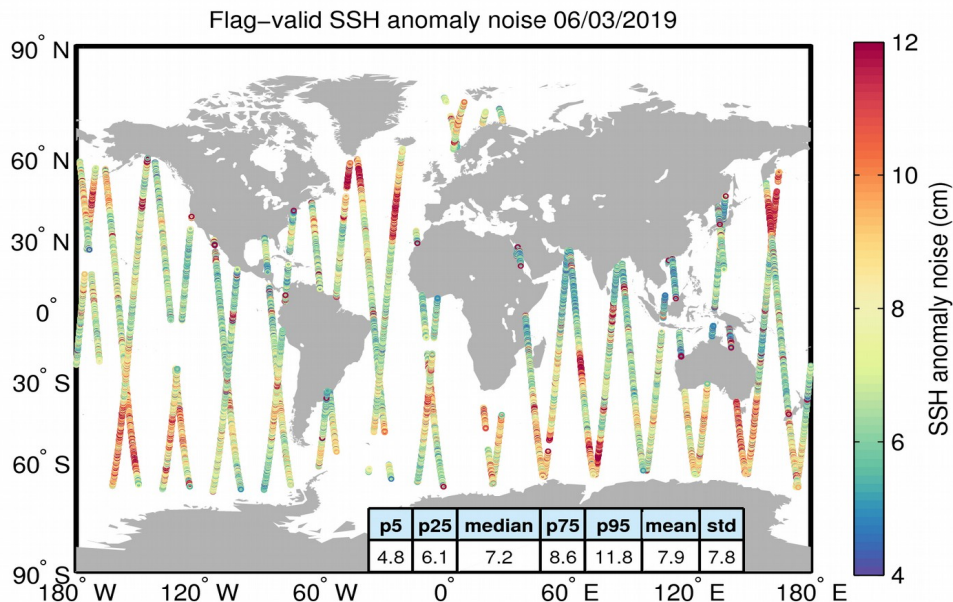
Figure 8. Geographical distribution of flag-valid 20-Hz SSH anomaly measurement noise over oceans and lakes for 06/03/2019. The statistical values shown in the table refer to the SSH anomaly noise and are calculated over all measurements shown in the figure.
