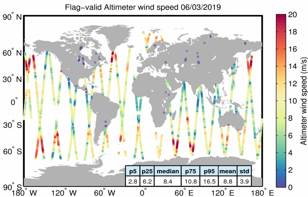
Figure 31. Geographical distribution of flag-valid wind data over oceans and lakes for 06/03/2019. The statistical values shown in the table refer to the wind in m/s and are calculated over all measurements shown in the figure.
