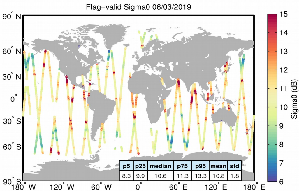
Figure 23. Geographical distribution of flag-valid sigma0 data over oceans and lakes for 06/03/2019. The statistical values shown in the table refer to the sigma0 in dB and are calculated over all measurements shown in the figure.
