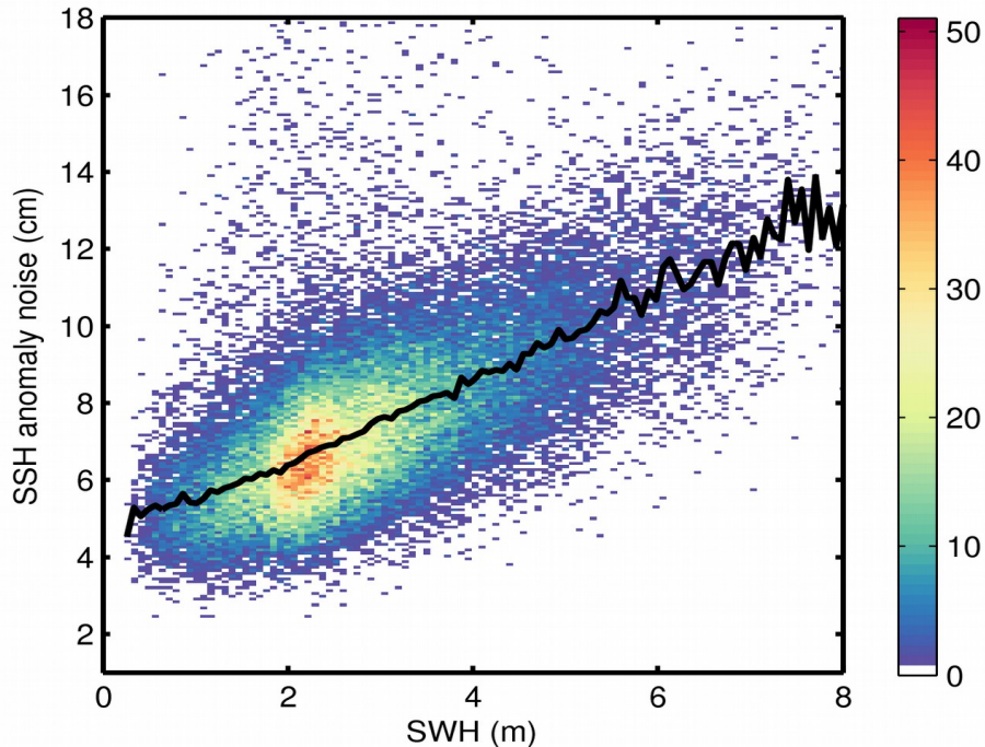
Figure 9. 2D histogram showing flag-valid SSH anomaly noise as a function of SWH for 06/03/2019. The black line denotes the median SSH anomaly noise as a function of SWH.
