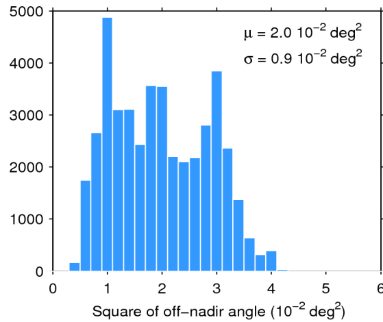
Figure 39. Histogram of flag-valid mispointing over oceans and lakes for 06/03/2019. The mean ( \mu ) and standard deviation ( \sigma ) are also shown. Note that values larger than 6 \cdot 10^{-2} \text{ deg}^2 are excluded from the histogram for the sake of readability but not from the computation of \mu and \sigma .
