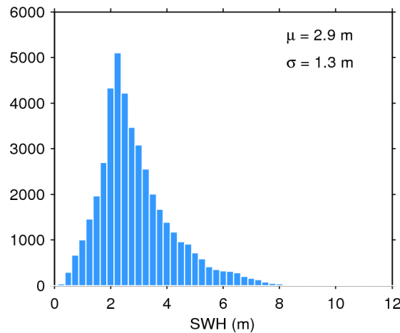
Figure 20. Histogram of science-valid SWH over oceans and lakes for 06/03/2019. The mean ( \mu ) and standard deviation ( \sigma ) are also shown. Note that values larger than 12 m are excluded from the histogram for the sake of readability but not from the computation of \mu and \sigma .
