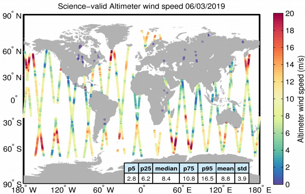
Figure 34. Geographical distribution of science-valid wind data over oceans and lakes for 06/03/2019. The statistical values shown in the table refer to the wind in m/s and are calculated over all measurements shown in the figure. Gray circles denote records that have been rejected based on the editing criteria described in Table 5.
