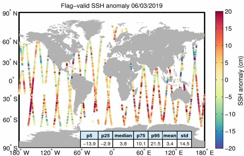
Figure 5. Geographical distribution of flag-valid 1-Hz SSH anomaly data over oceans and lakes for 06/03/2019. The statistical values shown in the table refer to the SSH anomaly in cm and are calculated over all measurements shown in the figure.
