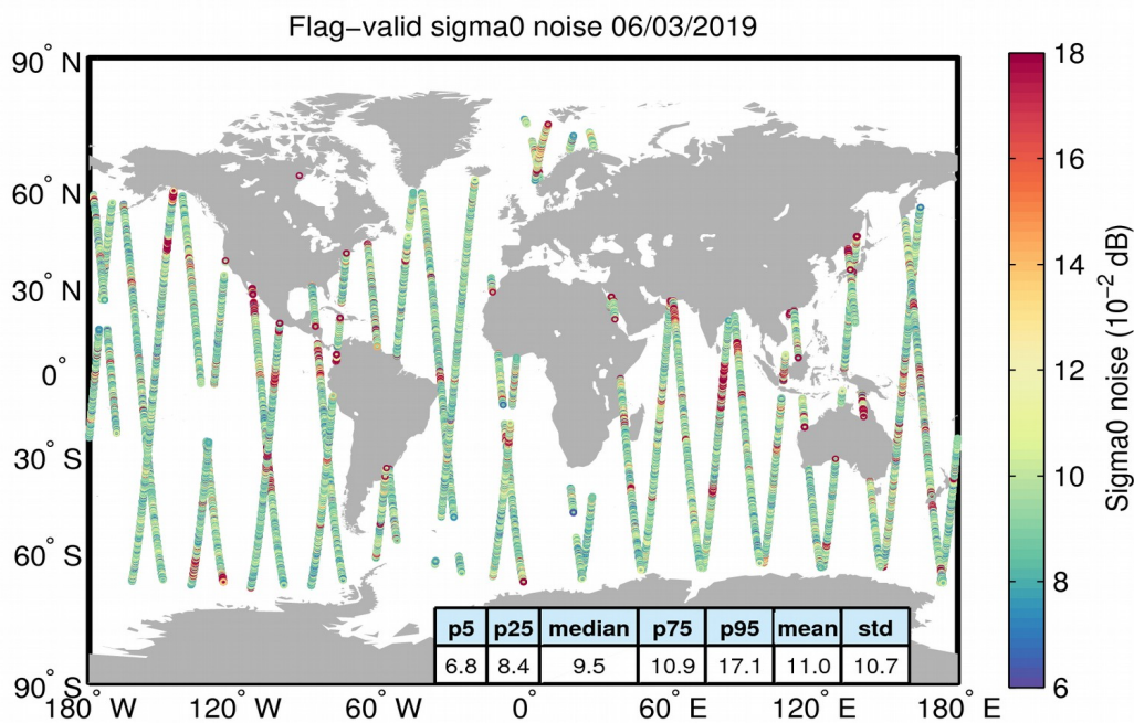
Figure 26. Geographical distribution of flag-valid 20-Hz sigma0 measurement noise over oceans and lakes for 06/03/2019. The statistical values shown in the table refer to the sigma0 noise and are calculated over all measurements shown in the figure.
