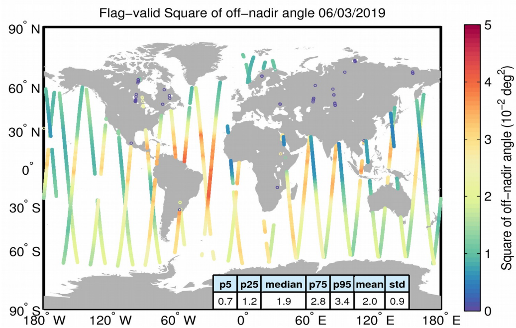
Figure 37. Geographical distribution of flag-valid mispointing data over oceans and lakes for 06/03/2019. The statistical values shown in the table refer to the mispointing in 10^{-2} deg 2 and are calculated over all measurements shown in the figure.
