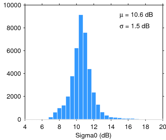
Figure 28. Histogram of science-valid sigma0 over oceans and lakes for 06/03/2019. The mean ( \mu ) and standard deviation ( \sigma ) are also shown. Note that values outside [4 20] dB are excluded from the histogram for the sake of readability but not from the computation of \mu and \sigma .
