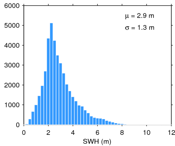
Figure 17. Histogram of flag-valid SWH over oceans and lakes for 06/03/2019. The mean ( \mu ) and standard deviation ( \sigma ) are also shown. Note that values larger than 12 m are excluded from the histogram for the sake of readability but not from the computation of \mu and \sigma .
