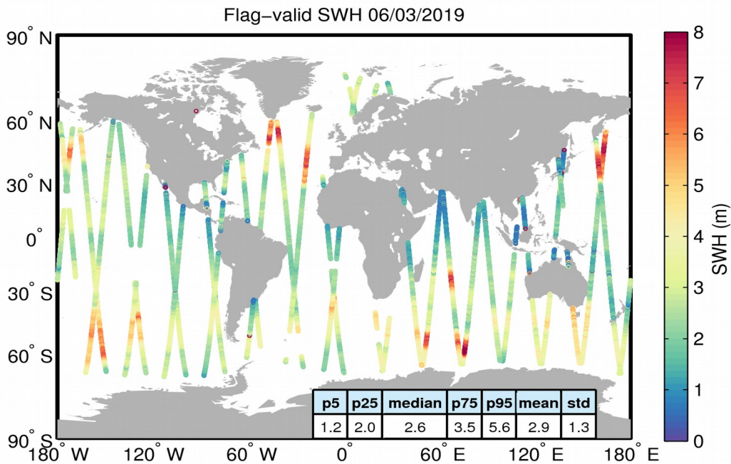
Figure 15. Geographical distribution of flag-valid SWH data over oceans and lakes for 06/03/2019. The statistical values shown in the table refer to the SWH in m and are calculated over all measurements shown in the figure.
