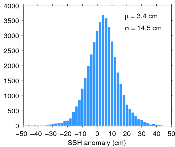
Figure 7. Histogram of flag-valid SSH anomaly over oceans and lakes for 06/03/2019. The mean ( \mu ) and standard deviation ( \sigma ) are also shown. Note that values outside [-50\ 50] cm are excluded from the histogram for the sake of readability but not from the computation of \mu and \sigma .
