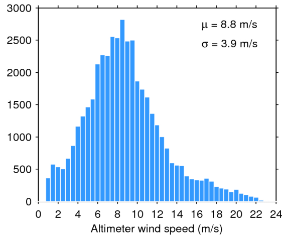
Figure 33. Histogram of flag-valid wind over oceans and lakes for 06/03/2019. The mean ( \mu ) and standard deviation ( \sigma ) are also shown. Note that values larger than 24 m/s are excluded from the histogram for the sake of readability but not from the computation of \mu and \sigma .
