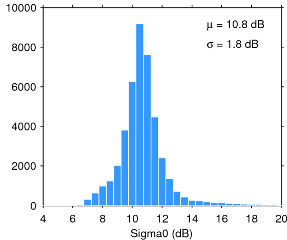
Figure 25. Histogram of flag-valid sigma0 over oceans and lakes for 06/03/2019. The mean ( \mu ) and standard deviation ( \sigma ) are also shown. Note that values outside [4 20] dB are excluded from the histogram for the sake of readability but not from the computation of \mu and \sigma .
