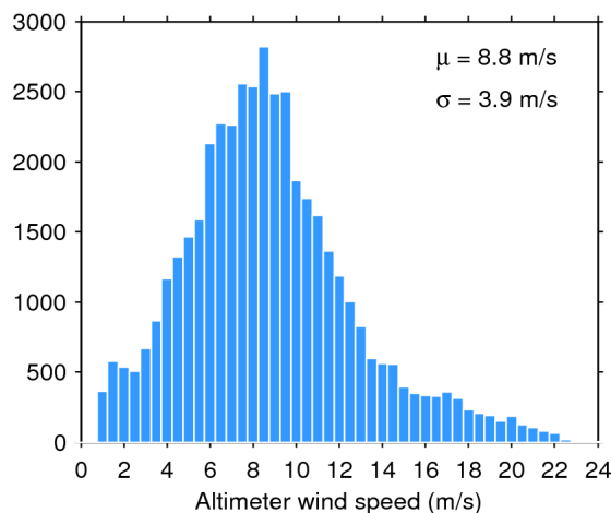
Figure 35. Histogram of science-valid wind over oceans and lakes for 06/03/2019. The mean ( \mu ) and standard deviation ( \sigma ) are also shown. Note that values larger than 24 m/s are excluded from the histogram for the sake of readability but not from the computation of \mu and \sigma .
