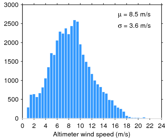
Figure 33. Histogram of flag-valid wind over oceans and lakes for 05/03/2019. The mean ( \mu ) and standard deviation ( \sigma ) are also shown. Note that values larger than 24 m/s are excluded from the histogram for the sake of readability but not from the computation of \mu and \sigma .
