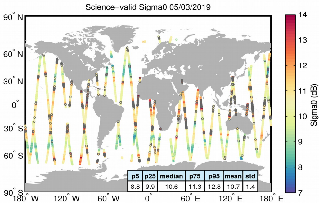
Figure 27. Geographical distribution of science-valid sigma0 data over oceans and lakes for 05/03/2019. The statistical values shown in the table refer to the sigma0 in dB and are calculated over all measurements shown in the figure. Gray circles denote records that have been rejected based on the editing criteria described in Table 4.
