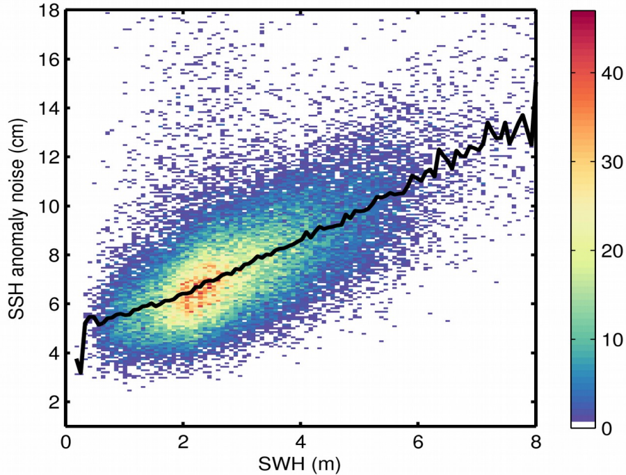
Figure 9. 2D histogram showing flag-valid SSH anomaly noise as a function of SWH for 05/03/2019. The black line denotes the median SSH anomaly noise as a function of SWH.
