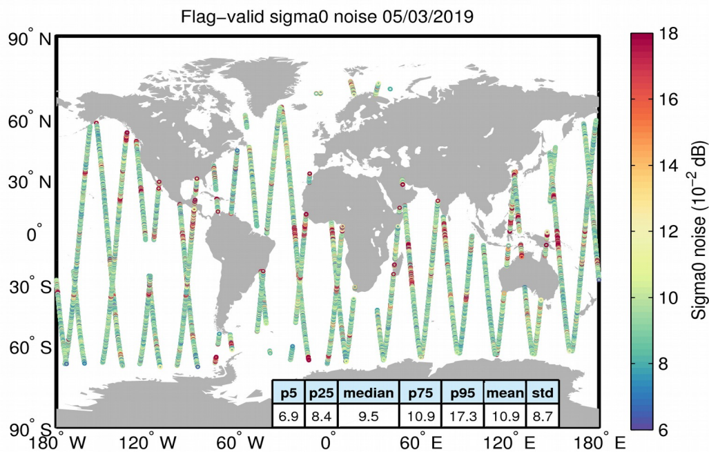
Figure 26. Geographical distribution of flag-valid 20-Hz sigma0 measurement noise over oceans and lakes for 05/03/2019. The statistical values shown in the table refer to the sigma0 noise and are calculated over all measurements shown in the figure.
