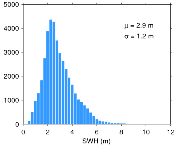
Figure 20. Histogram of science-valid SWH over oceans and lakes for 05/03/2019. The mean ( \mu ) and standard deviation ( \sigma ) are also shown. Note that values larger than 12 m are excluded from the histogram for the sake of readability but not from the computation of \mu and \sigma .
