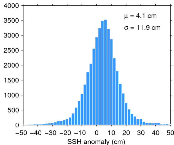
Figure 11. Histogram of science-valid SSH anomaly over oceans and lakes for 05/03/2019. The mean ( \mu ) and standard deviation ( \sigma ) are also shown. Note that values outside [-50 50] cm are excluded from the histogram for the sake of readability but not from the computation of \mu and \sigma .
