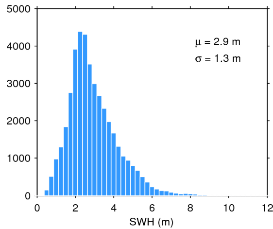
Figure 17. Histogram of flag-valid SWH over oceans and lakes for 05/03/2019. The mean ( \mu ) and standard deviation ( \sigma ) are also shown. Note that values larger than 12 m are excluded from the histogram for the sake of readability but not from the computation of \mu and \sigma .
