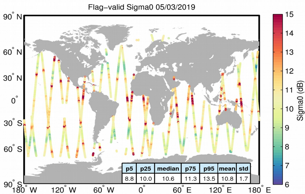
Figure 23. Geographical distribution of flag-valid sigma0 data over oceans and lakes for 05/03/2019. The statistical values shown in the table refer to the sigma0 in dB and are calculated over all measurements shown in the figure.
