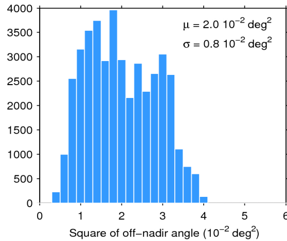
Figure 39. Histogram of flag-valid mispointing over oceans and lakes for 05/03/2019. The mean ( \mu ) and standard deviation ( \sigma ) are also shown. Note that values larger than 6 \cdot 10^{-2} \text{ deg}^2 are excluded from the histogram for the sake of readability but not from the computation of \mu and \sigma .
