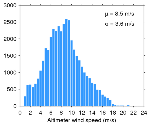
Figure 35. Histogram of science-valid wind over oceans and lakes for 05/03/2019. The mean ( \mu ) and standard deviation ( \sigma ) are also shown. Note that values larger than 24 m/s are excluded from the histogram for the sake of readability but not from the computation of \mu and \sigma .
