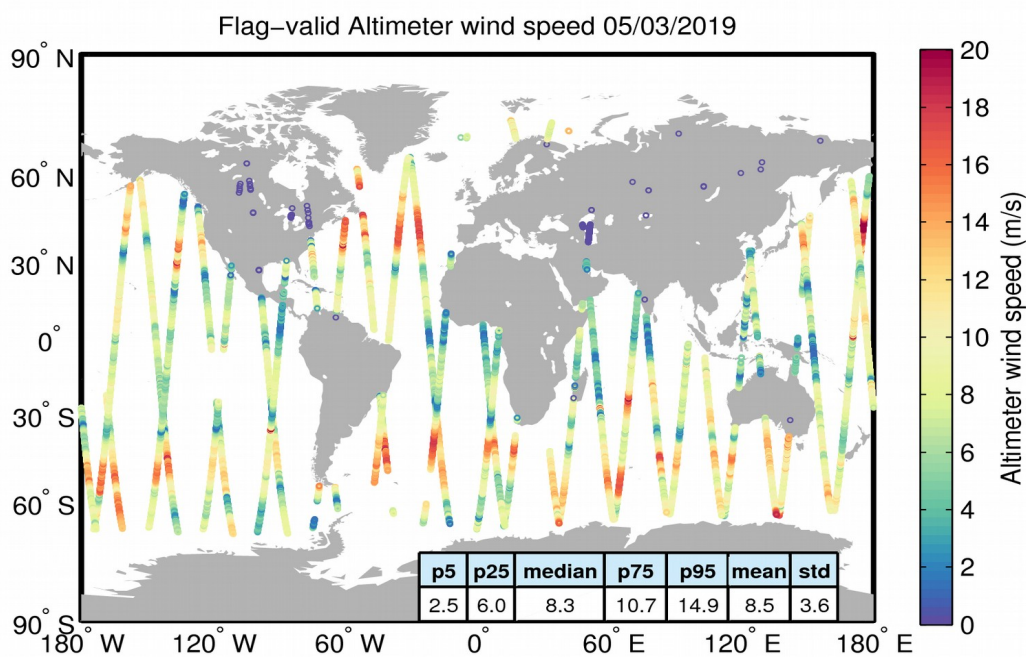
Figure 31. Geographical distribution of flag-valid wind data over oceans and lakes for 05/03/2019. The statistical values shown in the table refer to the wind in m/s and are calculated over all measurements shown in the figure.
