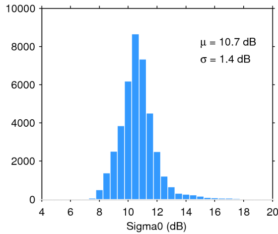
Figure 28. Histogram of science-valid sigma0 over oceans and lakes for 05/03/2019. The mean ( \mu ) and standard deviation ( \sigma ) are also shown. Note that values outside [4 20] dB are excluded from the histogram for the sake of readability but not from the computation of \mu and \sigma .
