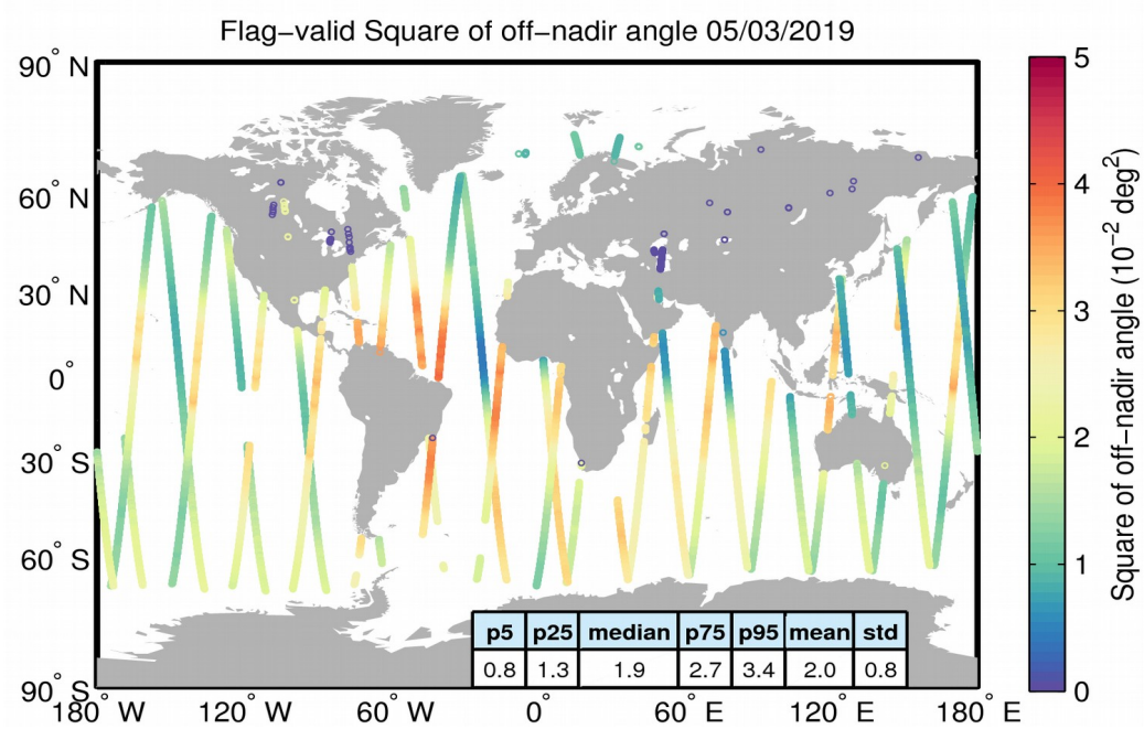
Figure 37. Geographical distribution of flag-valid mispointing data over oceans and lakes for 05/03/2019. The statistical values shown in the table refer to the mispointing in 10^{-2} deg 2 and are calculated over all measurements shown in the figure.
