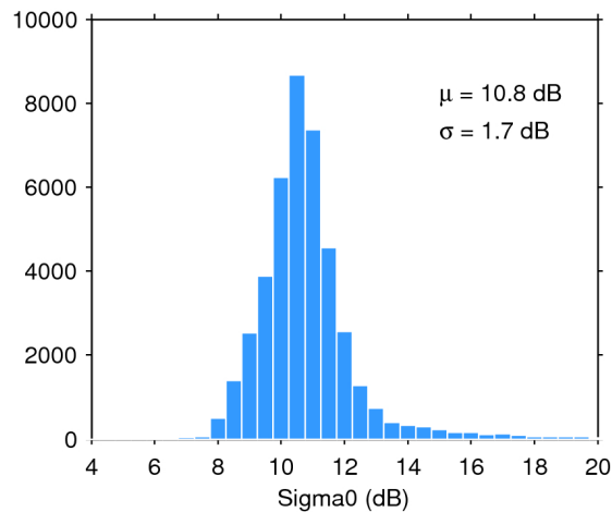
Figure 25. Histogram of flag-valid sigma0 over oceans and lakes for 05/03/2019. The mean ( \mu ) and standard deviation ( \sigma ) are also shown. Note that values outside [4 20] dB are excluded from the histogram for the sake of readability but not from the computation of \mu and \sigma .
