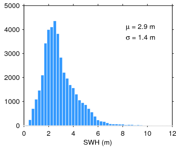
Figure 17. Histogram of flag-valid SWH over oceans and lakes for 04/03/2019. The mean ( \mu ) and standard deviation ( \sigma ) are also shown. Note that values larger than 12 m are excluded from the histogram for the sake of readability but not from the computation of \mu and \sigma .
