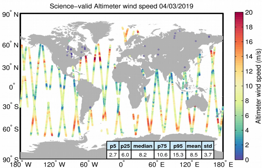
Figure 34. Geographical distribution of science-valid wind data over oceans and lakes for 04/03/2019. The statistical values shown in the table refer to the wind in m/s and are calculated over all measurements shown in the figure. Gray circles denote records that have been rejected based on the editing criteria described in Table 5.
