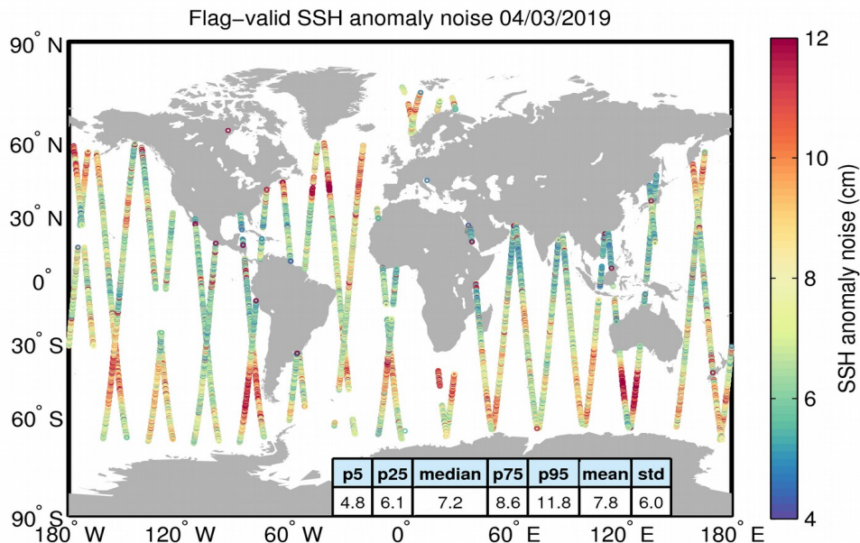
Figure 8. Geographical distribution of flag-valid 20-Hz SSH anomaly measurement noise over oceans and lakes for 04/03/2019. The statistical values shown in the table refer to the SSH anomaly noise and are calculated over all measurements shown in the figure.
