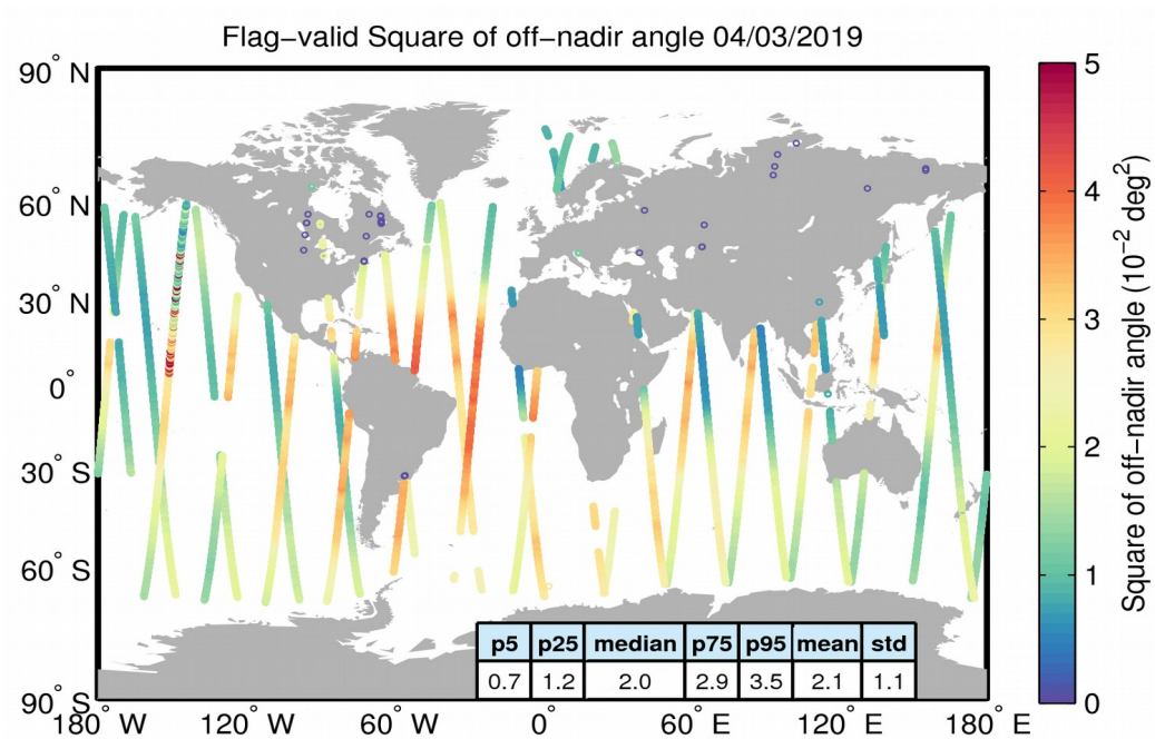
Figure 37. Geographical distribution of flag-valid mispointing data over oceans and lakes for 04/03/2019. The statistical values shown in the table refer to the mispointing in 10^{-2} \text{ deg}^2 and are calculated over all measurements shown in the figure.
