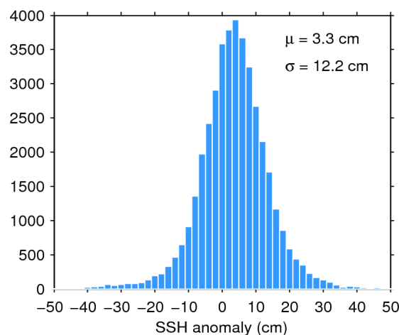
Figure 11. Histogram of science-valid SSH anomaly over oceans and lakes for 04/03/2019. The mean ( \mu ) and standard deviation ( \sigma ) are also shown. Note that values outside [-50 50] cm are excluded from the histogram for the sake of readability but not from the computation of \mu and \sigma .
