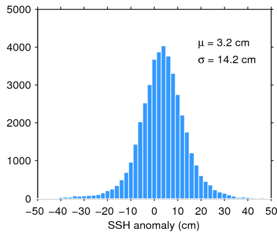
Figure 7. Histogram of flag-valid SSH anomaly over oceans and lakes for 04/03/2019. The mean ( \mu ) and standard deviation ( \sigma ) are also shown. Note that values outside [-50 50] cm are excluded from the histogram for the sake of readability but not from the computation of \mu and \sigma .
