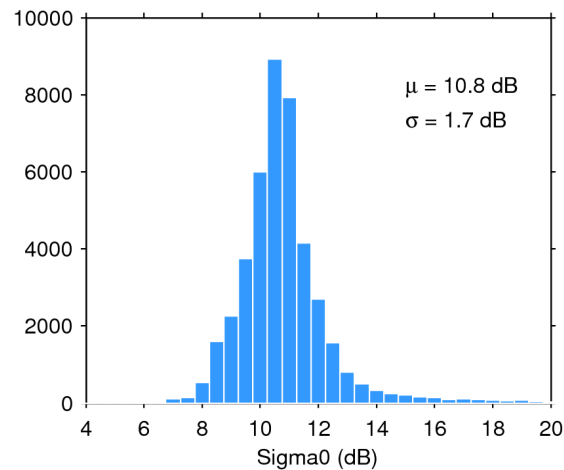
Figure 25. Histogram of flag-valid sigma0 over oceans and lakes for 04/03/2019. The mean ( \mu ) and standard deviation ( \sigma ) are also shown. Note that values outside [4 20] dB are excluded from the histogram for the sake of readability but not from the computation of \mu and \sigma .
