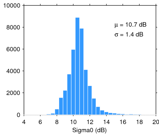
Figure 28. Histogram of science-valid sigma0 over oceans and lakes for 04/03/2019. The mean ( \mu ) and standard deviation ( \sigma ) are also shown. Note that values outside [4 20] dB are excluded from the histogram for the sake of readability but not from the computation of \mu and \sigma .
