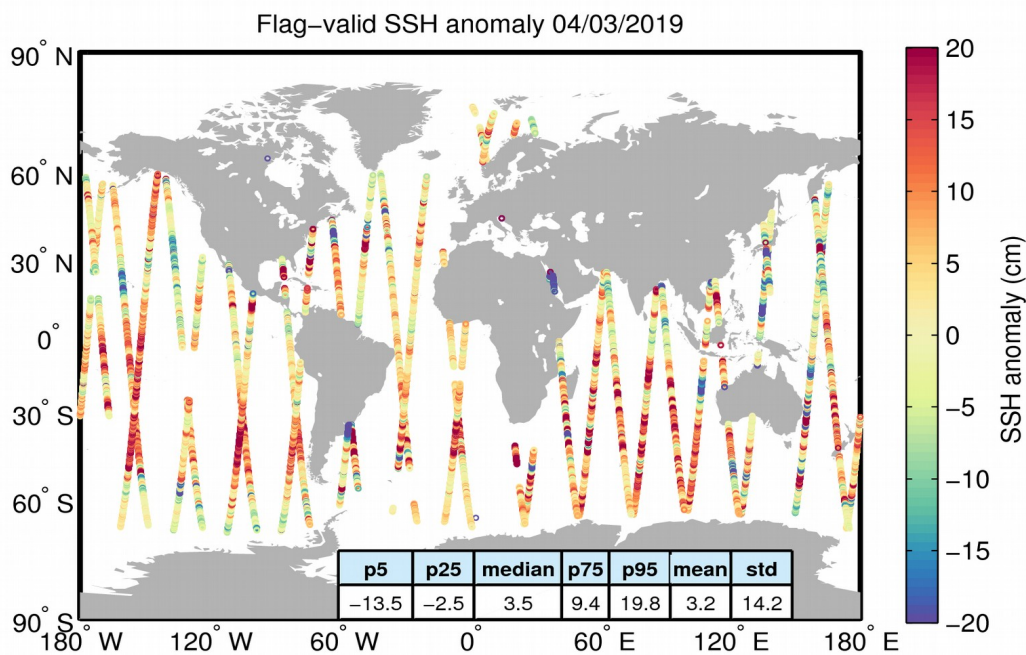
Figure 5. Geographical distribution of flag-valid 1-Hz SSH anomaly data over oceans and lakes for 04/03/2019. The statistical values shown in the table refer to the SSH anomaly in cm and are calculated over all measurements shown in the figure.
