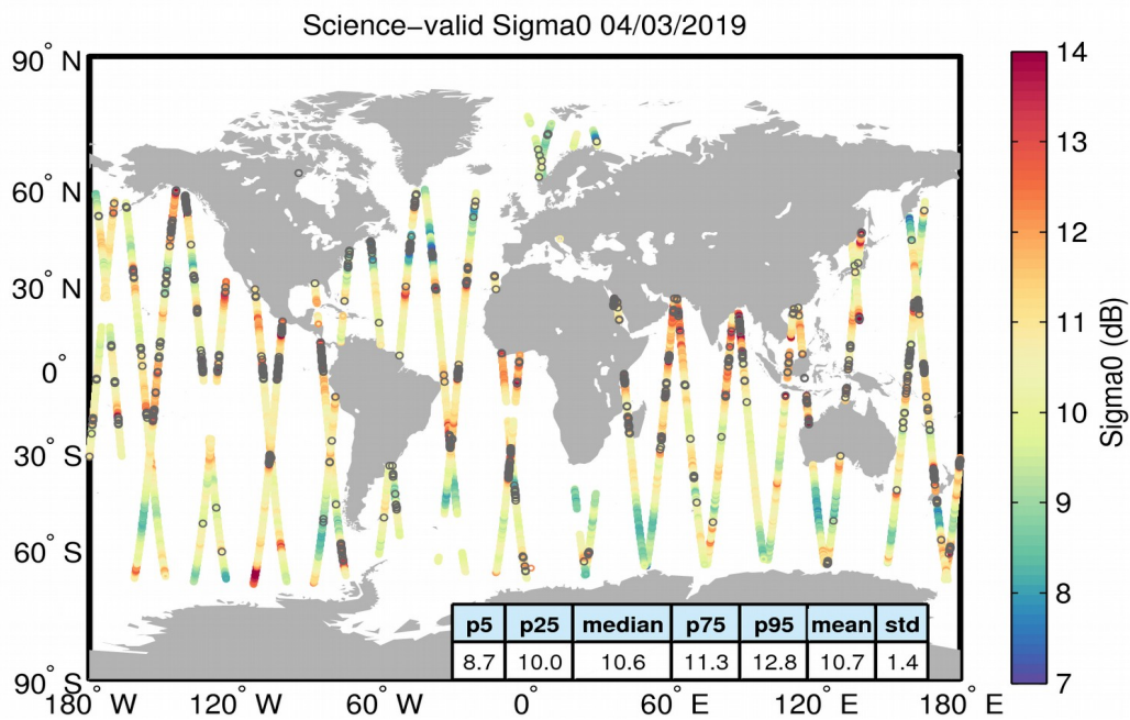
Figure 27. Geographical distribution of science-valid sigma0 data over oceans and lakes for 04/03/2019. The statistical values shown in the table refer to the sigma0 in dB and are calculated over all measurements shown in the figure. Gray circles denote records that have been rejected based on the editing criteria described in Table 4.
