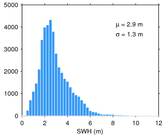
Figure 20. Histogram of science-valid SWH over oceans and lakes for 04/03/2019. The mean ( \mu ) and standard deviation ( \sigma ) are also shown. Note that values larger than 12 m are excluded from the histogram for the sake of readability but not from the computation of \mu and \sigma .
