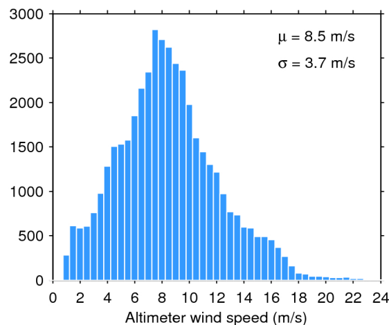
Figure 35. Histogram of science-valid wind over oceans and lakes for 04/03/2019. The mean ( \mu ) and standard deviation ( \sigma ) are also shown. Note that values larger than 24 m/s are excluded from the histogram for the sake of readability but not from the computation of \mu and \sigma .
