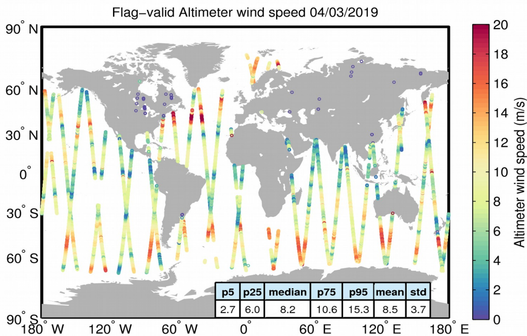
Figure 31. Geographical distribution of flag-valid wind data over oceans and lakes for 04/03/2019. The statistical values shown in the table refer to the wind in m/s and are calculated over all measurements shown in the figure.
