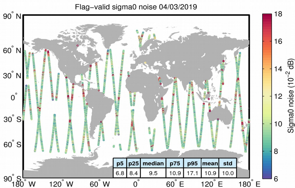
Figure 26. Geographical distribution of flag-valid 20-Hz sigma0 measurement noise over oceans and lakes for 04/03/2019. The statistical values shown in the table refer to the sigma0 noise and are calculated over all measurements shown in the figure.
