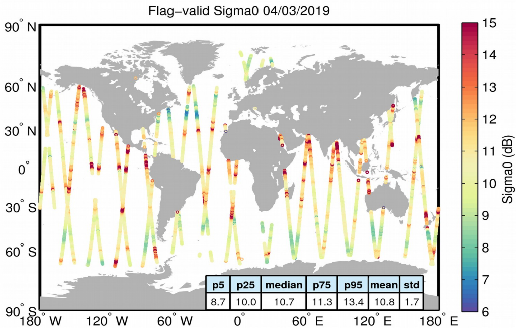
Figure 23. Geographical distribution of flag-valid sigma0 data over oceans and lakes for 04/03/2019. The statistical values shown in the table refer to the sigma0 in dB and are calculated over all measurements shown in the figure.
