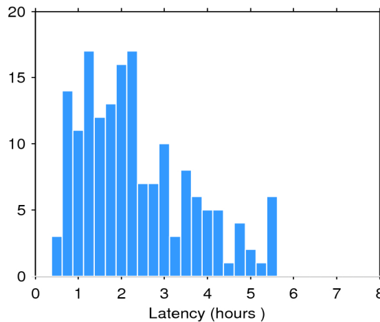
Figure 2. Histogram of the data latency for 04/03/2019. The y-axis denotes the number of files that are made available with a delay of x-hours with respect to the mean time of the records stored in the file.
