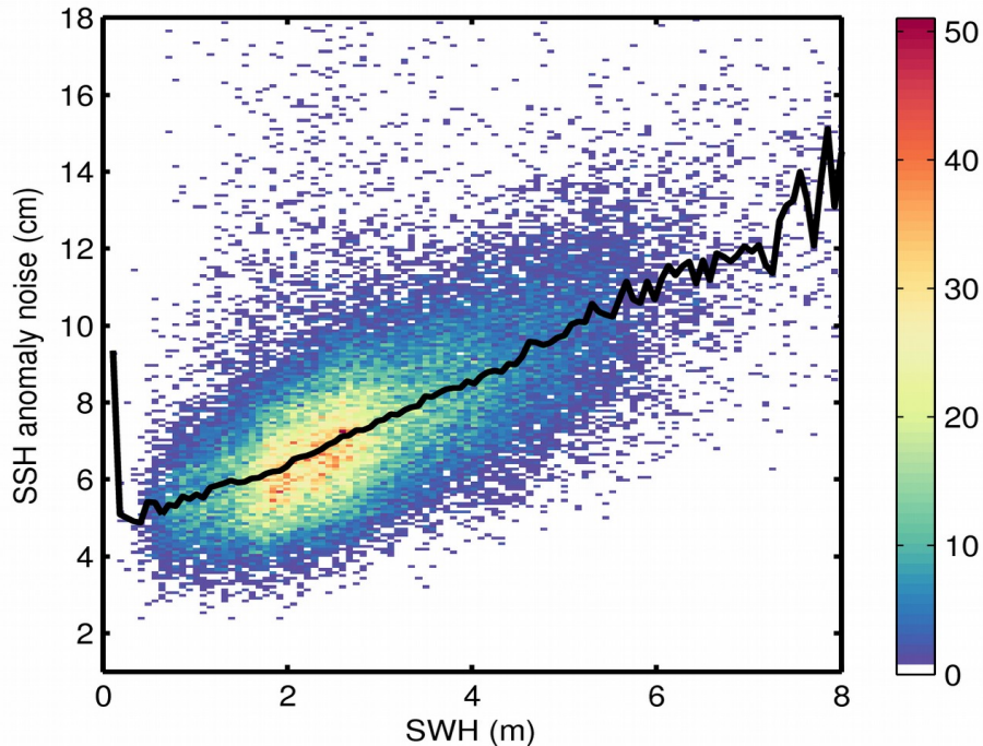
Figure 9. 2D histogram showing flag-valid SSH anomaly noise as a function of SWH for 04/03/2019. The black line denotes the median SSH anomaly noise as a function of SWH.
