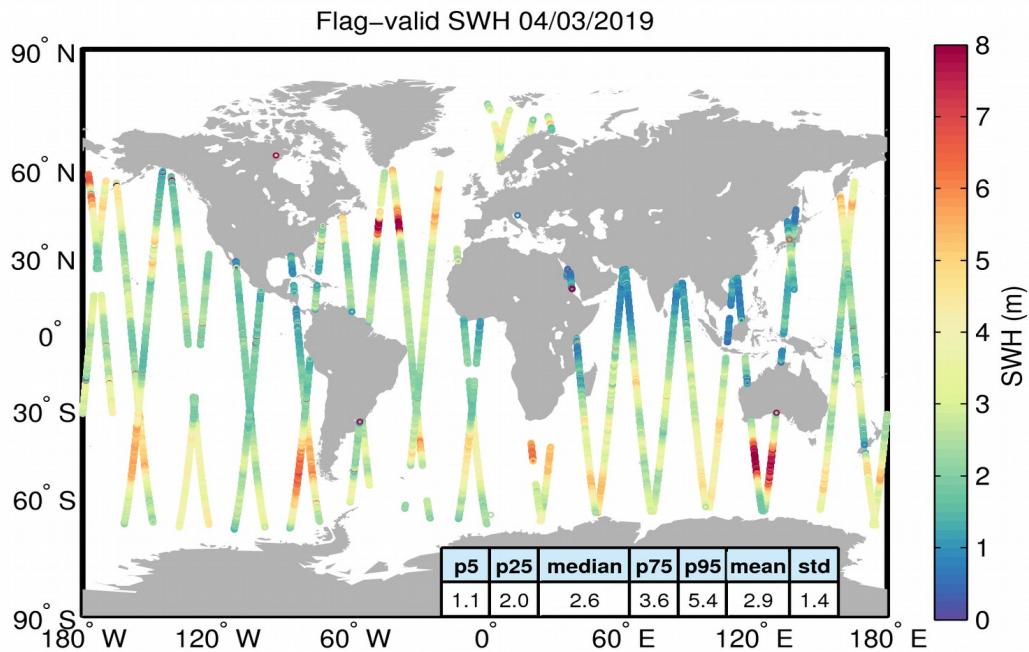
Figure 15. Geographical distribution of flag-valid SWH data over oceans and lakes for 04/03/2019. The statistical values shown in the table refer to the SWH in m and are calculated over all measurements shown in the figure.
