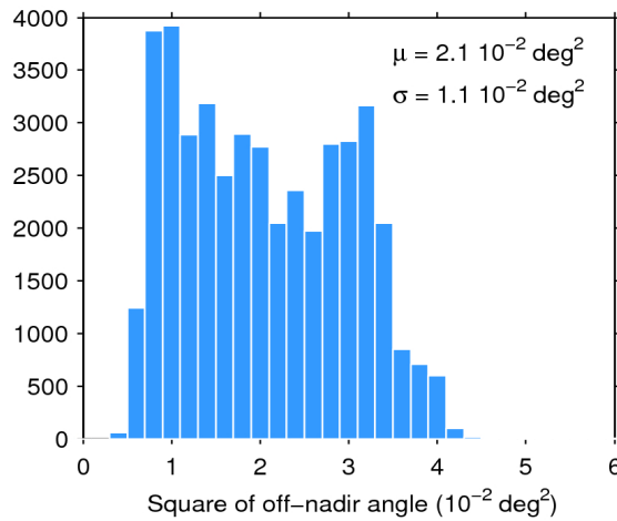
Figure 39. Histogram of flag-valid mispointing over oceans and lakes for 04/03/2019. The mean ( \mu ) and standard deviation ( \sigma ) are also shown. Note that values larger than 6 \cdot 10^{-2} \text{ deg}^2 are excluded from the histogram for the sake of readability but not from the computation of \mu and \sigma .
