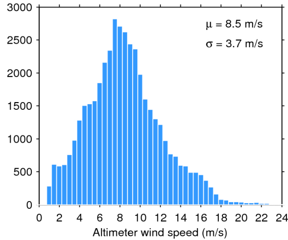
Figure 33. Histogram of flag-valid wind over oceans and lakes for 04/03/2019. The mean ( \mu ) and standard deviation ( \sigma ) are also shown. Note that values larger than 24 m/s are excluded from the histogram for the sake of readability but not from the computation of \mu and \sigma .
