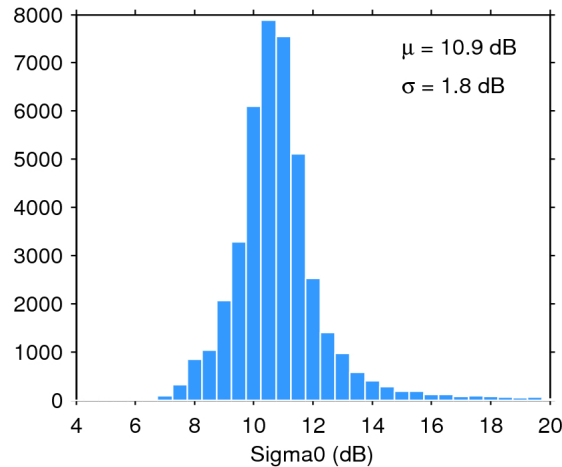
Figure 25. Histogram of flag-valid sigma0 over oceans and lakes for 03/03/2019. The mean ( \mu ) and standard deviation ( \sigma ) are also shown. Note that values outside [4 20] dB are excluded from the histogram for the sake of readability but not from the computation of \mu and \sigma .
