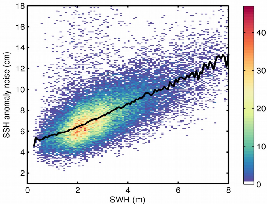
Figure 9. 2D histogram showing flag-valid SSH anomaly noise as a function of SWH for 03/03/2019. The black line denotes the median SSH anomaly noise as a function of SWH.
