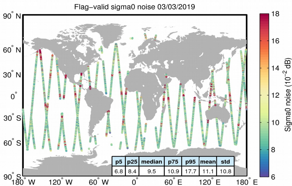
Figure 26. Geographical distribution of flag-valid 20-Hz sigma0 measurement noise over oceans and lakes for 03/03/2019. The statistical values shown in the table refer to the sigma0 noise and are calculated over all measurements shown in the figure.
