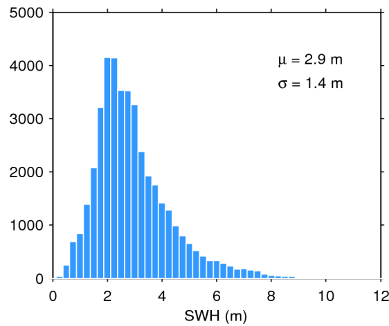
Figure 17. Histogram of flag-valid SWH over oceans and lakes for 03/03/2019. The mean ( \mu ) and standard deviation ( \sigma ) are also shown. Note that values larger than 12 m are excluded from the histogram for the sake of readability but not from the computation of \mu and \sigma .
