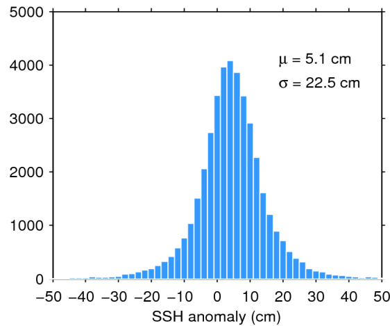
Figure 7. Histogram of flag-valid SSH anomaly over oceans and lakes for 03/03/2019. The mean ( \mu ) and standard deviation ( \sigma ) are also shown. Note that values outside [-50 50] cm are excluded from the histogram for the sake of readability but not from the computation of \mu and \sigma .
