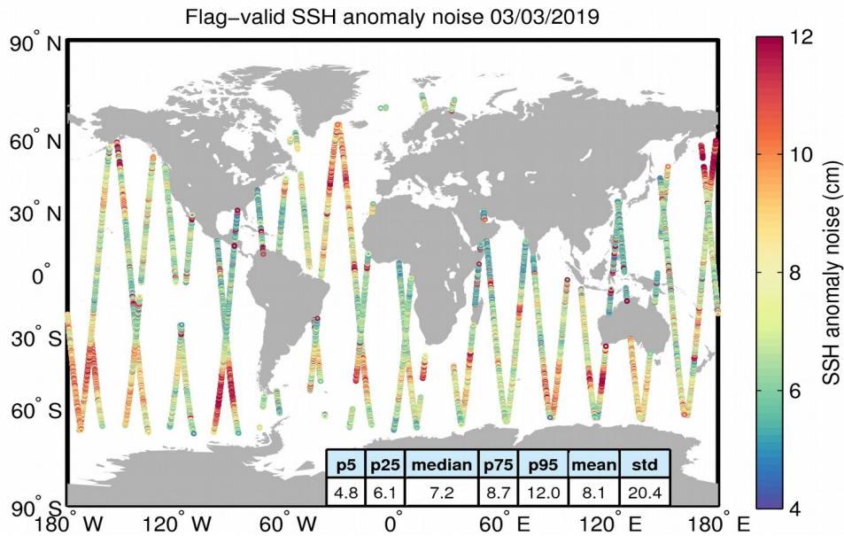
Figure 8. Geographical distribution of flag-valid 20-Hz SSH anomaly measurement noise over oceans and lakes for 03/03/2019. The statistical values shown in the table refer to the SSH anomaly noise and are calculated over all measurements shown in the figure.
