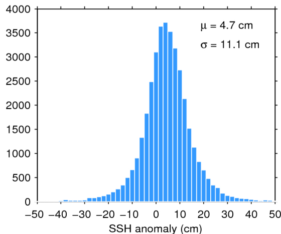
Figure 11. Histogram of science-valid SSH anomaly over oceans and lakes for 03/03/2019. The mean ( \mu ) and standard deviation ( \sigma ) are also shown. Note that values outside [-50 50] cm are excluded from the histogram for the sake of readability but not from the computation of \mu and \sigma .
