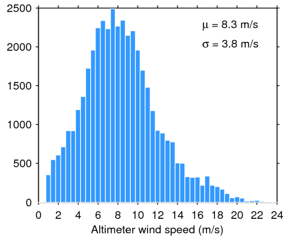
Figure 33. Histogram of flag-valid wind over oceans and lakes for 03/03/2019. The mean ( \mu ) and standard deviation ( \sigma ) are also shown. Note that values larger than 24 m/s are excluded from the histogram for the sake of readability but not from the computation of \mu and \sigma .
