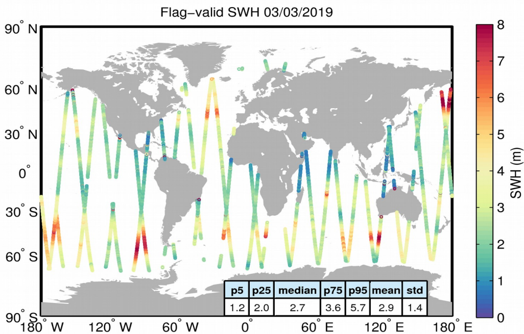
Figure 15. Geographical distribution of flag-valid SWH data over oceans and lakes for 03/03/2019. The statistical values shown in the table refer to the SWH in m and are calculated over all measurements shown in the figure.
