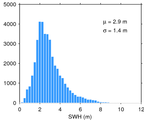
Figure 20. Histogram of science-valid SWH over oceans and lakes for 03/03/2019. The mean ( \mu ) and standard deviation ( \sigma ) are also shown. Note that values larger than 12 m are excluded from the histogram for the sake of readability but not from the computation of \mu and \sigma .
