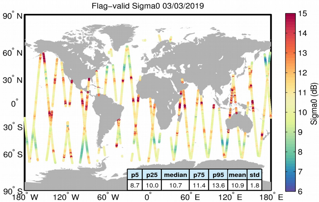
Figure 23. Geographical distribution of flag-valid sigma0 data over oceans and lakes for 03/03/2019. The statistical values shown in the table refer to the sigma0 in dB and are calculated over all measurements shown in the figure.
