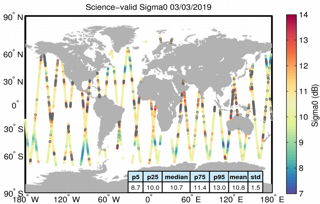
Figure 27. Geographical distribution of science-valid sigma0 data over oceans and lakes for 03/03/2019. The statistical values shown in the table refer to the sigma0 in dB and are calculated over all measurements shown in the figure. Gray circles denote records that have been rejected based on the editing criteria described in Table 4.
