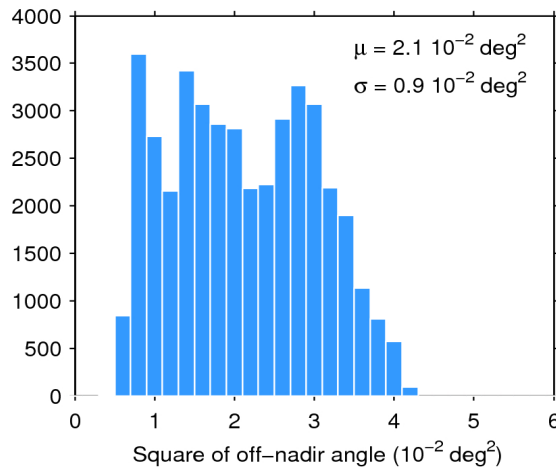
Figure 39. Histogram of flag-valid mispointing over oceans and lakes for 03/03/2019. The mean ( \mu ) and standard deviation ( \sigma ) are also shown. Note that values larger than 6 \cdot 10^{-2} \text{ deg}^2 are excluded from the histogram for the sake of readability but not from the computation of \mu and \sigma .
