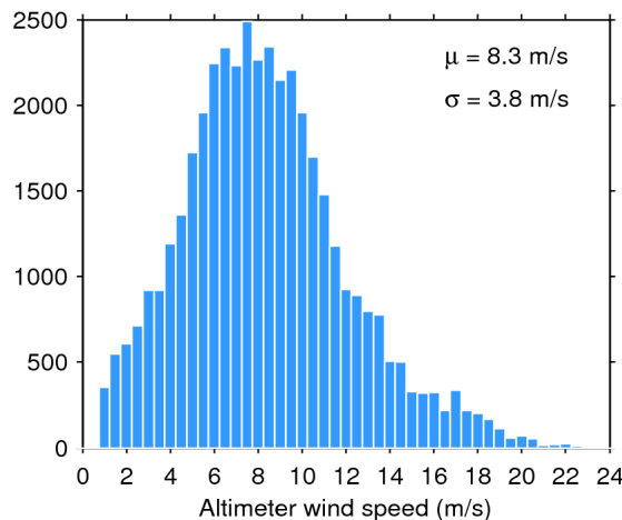
Figure 35. Histogram of science-valid wind over oceans and lakes for 03/03/2019. The mean ( \mu ) and standard deviation ( \sigma ) are also shown. Note that values larger than 24 m/s are excluded from the histogram for the sake of readability but not from the computation of \mu and \sigma .
