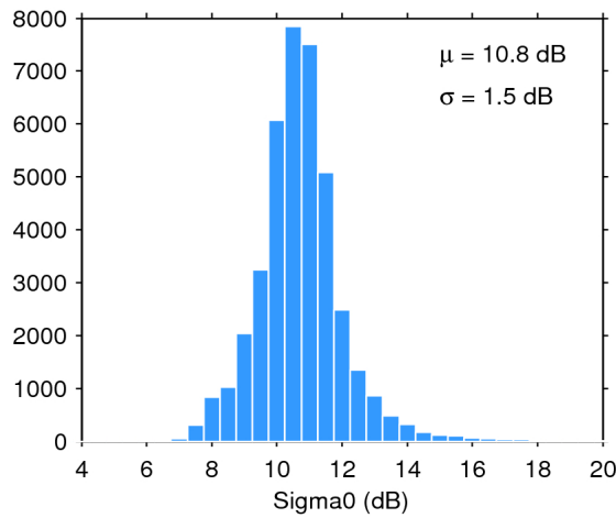
Figure 28. Histogram of science-valid sigma0 over oceans and lakes for 03/03/2019. The mean ( \mu ) and standard deviation ( \sigma ) are also shown. Note that values outside [4 20] dB are excluded from the histogram for the sake of readability but not from the computation of \mu and \sigma .
