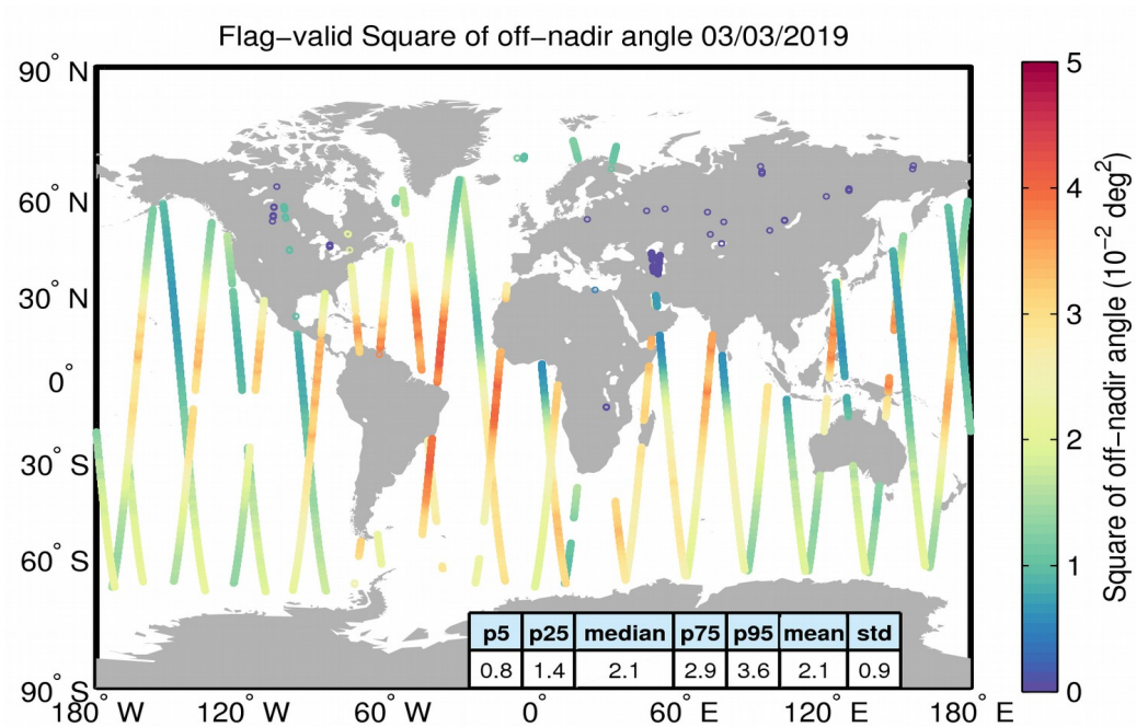
Figure 37. Geographical distribution of flag-valid mispointing data over oceans and lakes for 03/03/2019. The statistical values shown in the table refer to the mispointing in 10^{-2} \text{ deg}^2 and are calculated over all measurements shown in the figure.
