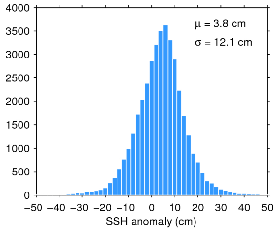
Figure 11. Histogram of science-valid SSH anomaly over oceans and lakes for 02/03/2019. The mean ( \mu ) and standard deviation ( \sigma ) are also shown. Note that values outside [-50 50] cm are excluded from the histogram for the sake of readability but not from the computation of \mu and \sigma .
