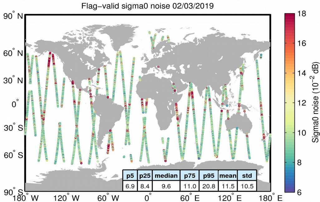
Figure 26. Geographical distribution of flag-valid 20-Hz sigma0 measurement noise over oceans and lakes for 02/03/2019. The statistical values shown in the table refer to the sigma0 noise and are calculated over all measurements shown in the figure.
