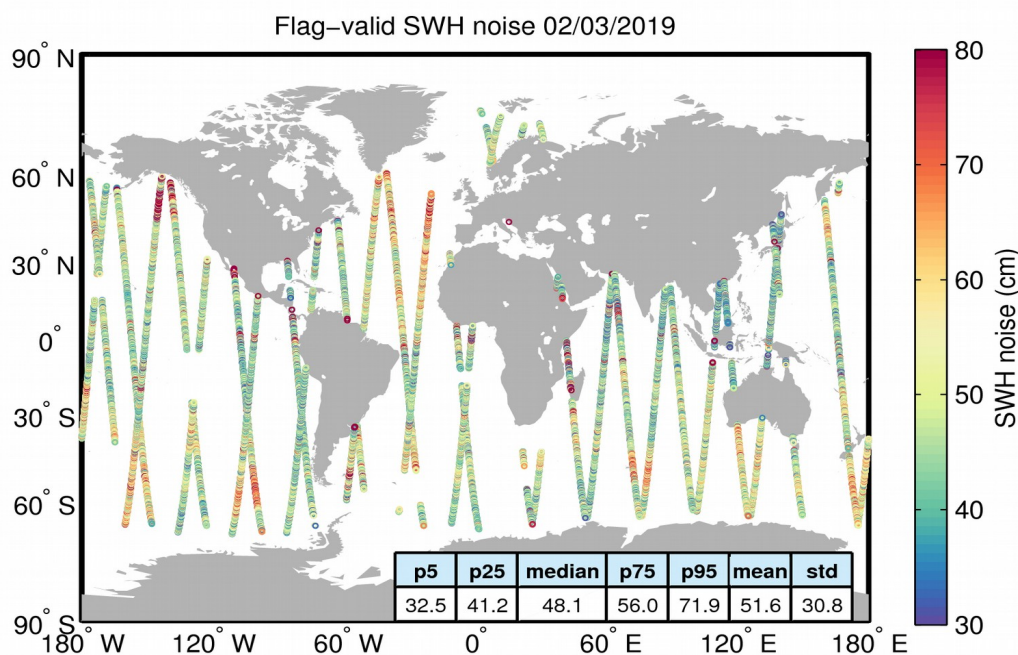
Figure 18. Geographical distribution of flag-valid 20-Hz SWH measurement noise over oceans and lakes for 02/03/2019. The statistical values shown in the table refer to the SWH noise and are calculated over all measurements shown in the figure.
