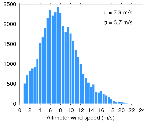
Figure 33. Histogram of flag-valid wind over oceans and lakes for 02/03/2019. The mean ( \mu ) and standard deviation ( \sigma ) are also shown. Note that values larger than 24 m/s are excluded from the histogram for the sake of readability but not from the computation of \mu and \sigma .
