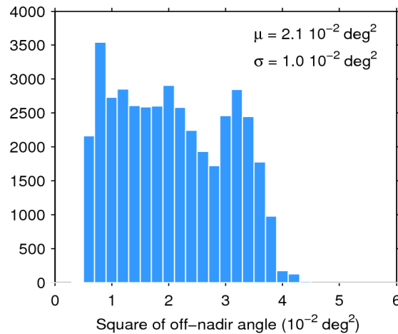
Figure 39. Histogram of flag-valid mispointing over oceans and lakes for 02/03/2019. The mean ( \mu ) and standard deviation ( \sigma ) are also shown. Note that values larger than 6 \cdot 10^{-2} \text{ deg}^2 are excluded from the histogram for the sake of readability but not from the computation of \mu and \sigma .
