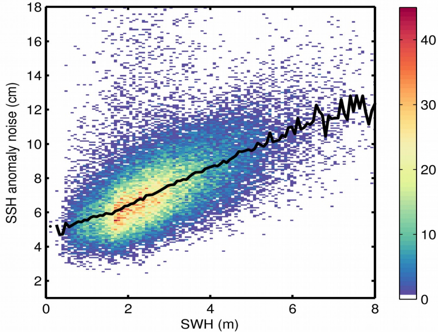
Figure 9. 2D histogram showing flag-valid SSH anomaly noise as a function of SWH for 02/03/2019. The black line denotes the median SSH anomaly noise as a function of SWH.
