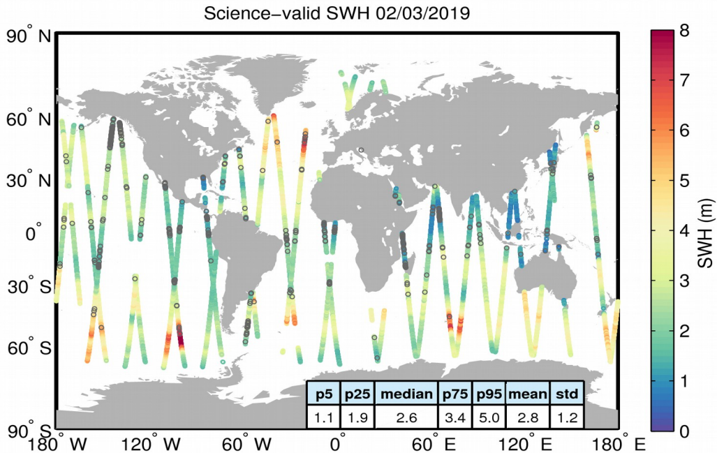
Figure 19. Geographical distribution of science-valid SWH data over oceans and lakes for 02/03/2019. The statistical values shown in the table refer to the SWH in m and are calculated over all measurements shown in the figure. Gray circles denote records that have been rejected based on the editing criteria described in Table 3.
