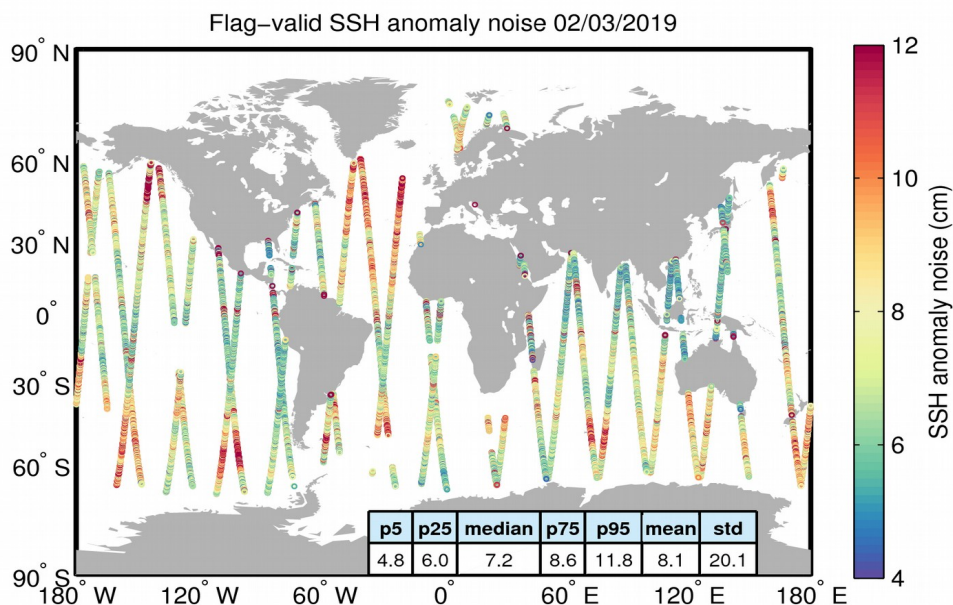
Figure 8. Geographical distribution of flag-valid 20-Hz SSH anomaly measurement noise over oceans and lakes for 02/03/2019. The statistical values shown in the table refer to the SSH anomaly noise and are calculated over all measurements shown in the figure.
