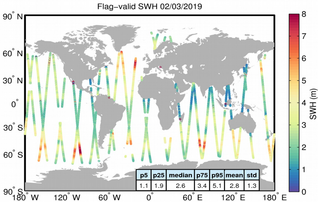
Figure 15. Geographical distribution of flag-valid SWH data over oceans and lakes for 02/03/2019. The statistical values shown in the table refer to the SWH in m and are calculated over all measurements shown in the figure.
