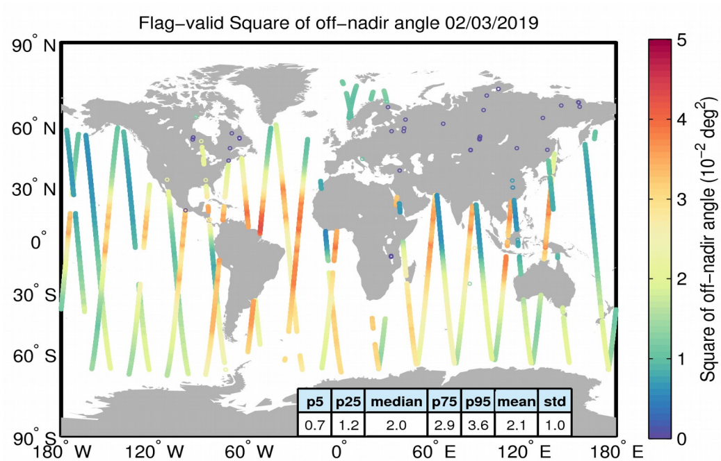
Figure 37. Geographical distribution of flag-valid mispointing data over oceans and lakes for 02/03/2019. The statistical values shown in the table refer to the mispointing in 10^{-2} deg 2 and are calculated over all measurements shown in the figure.
