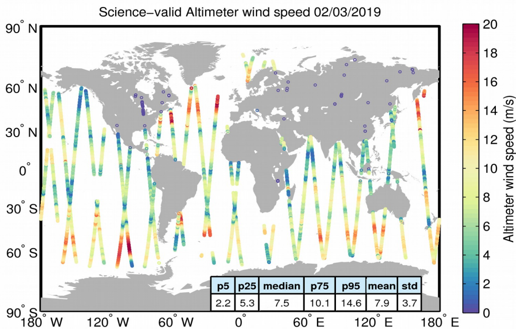
Figure 34. Geographical distribution of science-valid wind data over oceans and lakes for 02/03/2019. The statistical values shown in the table refer to the wind in m/s and are calculated over all measurements shown in the figure. Gray circles denote records that have been rejected based on the editing criteria described in Table 5.
