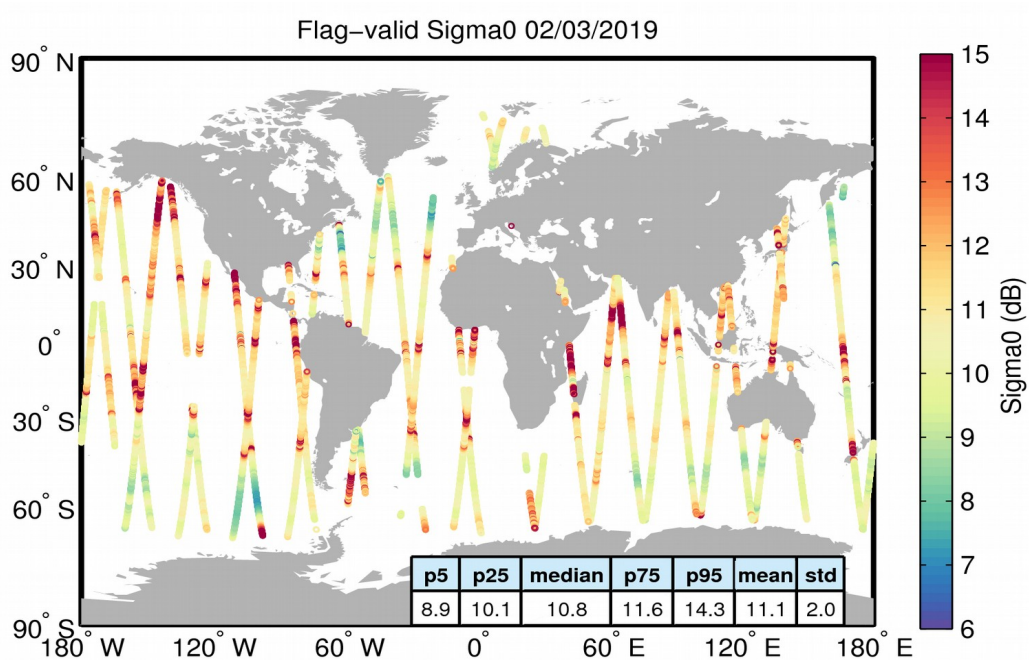
Figure 23. Geographical distribution of flag-valid sigma0 data over oceans and lakes for 02/03/2019. The statistical values shown in the table refer to the sigma0 in dB and are calculated over all measurements shown in the figure.
