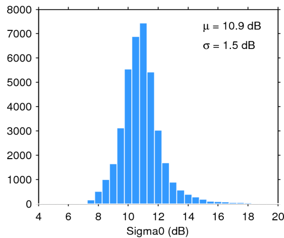
Figure 28. Histogram of science-valid sigma0 over oceans and lakes for 02/03/2019. The mean ( \mu ) and standard deviation ( \sigma ) are also shown. Note that values outside [4 20] dB are excluded from the histogram for the sake of readability but not from the computation of \mu and \sigma .
