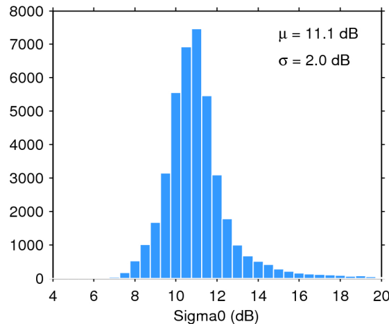
Figure 25. Histogram of flag-valid sigma0 over oceans and lakes for 02/03/2019. The mean ( \mu ) and standard deviation ( \sigma ) are also shown. Note that values outside [4 20] dB are excluded from the histogram for the sake of readability but not from the computation of \mu and \sigma .
