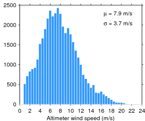
Figure 35. Histogram of science-valid wind over oceans and lakes for 02/03/2019. The mean ( \mu ) and standard deviation ( \sigma ) are also shown. Note that values larger than 24 m/s are excluded from the histogram for the sake of readability but not from the computation of \mu and \sigma .
