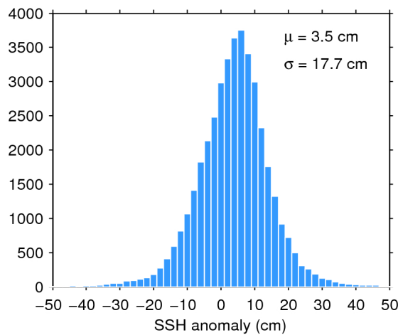
Figure 7. Histogram of flag-valid SSH anomaly over oceans and lakes for 02/03/2019. The mean ( \mu ) and standard deviation ( \sigma ) are also shown. Note that values outside [-50\ 50] cm are excluded from the histogram for the sake of readability but not from the computation of \mu and \sigma .
