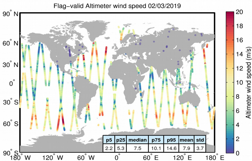
Figure 31. Geographical distribution of flag-valid wind data over oceans and lakes for 02/03/2019. The statistical values shown in the table refer to the wind in m/s and are calculated over all measurements shown in the figure.
