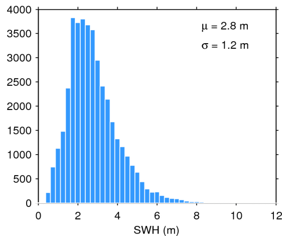
Figure 20. Histogram of science-valid SWH over oceans and lakes for 02/03/2019. The mean ( \mu ) and standard deviation ( \sigma ) are also shown. Note that values larger than 12 m are excluded from the histogram for the sake of readability but not from the computation of \mu and \sigma .
