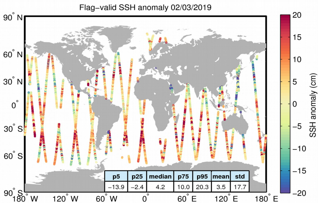
Figure 5. Geographical distribution of flag-valid 1-Hz SSH anomaly data over oceans and lakes for 02/03/2019. The statistical values shown in the table refer to the SSH anomaly in cm and are calculated over all measurements shown in the figure.
