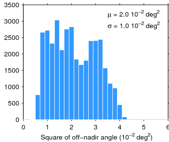
Figure 39. Histogram of flag-valid mispointing over oceans and lakes for 01/03/2019. The mean ( \mu ) and standard deviation ( \sigma ) are also shown. Note that values larger than 6 \cdot 10^{-2} \text{ deg}^2 are excluded from the histogram for the sake of readability but not from the computation of \mu and \sigma .
