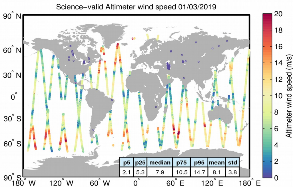
Figure 34. Geographical distribution of science-valid wind data over oceans and lakes for 01/03/2019. The statistical values shown in the table refer to the wind in m/s and are calculated over all measurements shown in the figure. Gray circles denote records that have been rejected based on the editing criteria described in Table 5.
