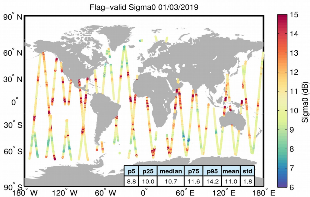
Figure 23. Geographical distribution of flag-valid sigma0 data over oceans and lakes for 01/03/2019. The statistical values shown in the table refer to the sigma0 in dB and are calculated over all measurements shown in the figure.
