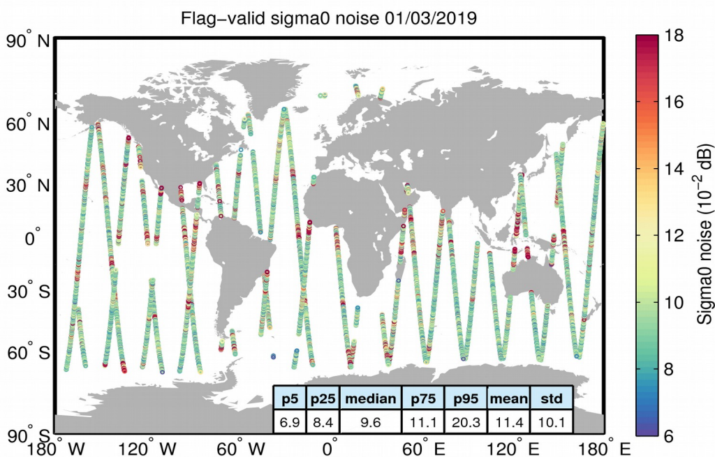
Figure 26. Geographical distribution of flag-valid 20-Hz sigma0 measurement noise over oceans and lakes for 01/03/2019. The statistical values shown in the table refer to the sigma0 noise and are calculated over all measurements shown in the figure.
