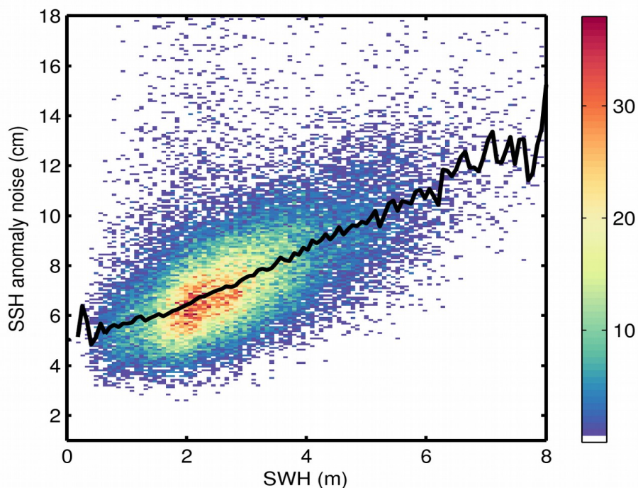
Figure 9. 2D histogram showing flag-valid SSH anomaly noise as a function of SWH for 01/03/2019. The black line denotes the median SSH anomaly noise as a function of SWH.
