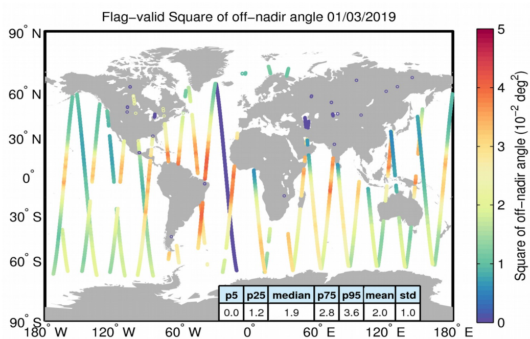
Figure 37. Geographical distribution of flag-valid mispointing data over oceans and lakes for 01/03/2019. The statistical values shown in the table refer to the mispointing in 10^{-2} deg 2 and are calculated over all measurements shown in the figure.
