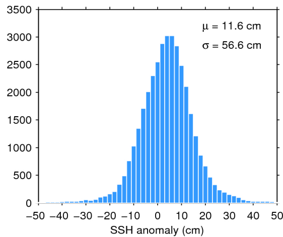
Figure 7. Histogram of flag-valid SSH anomaly over oceans and lakes for 01/03/2019. The mean ( \mu ) and standard deviation ( \sigma ) are also shown. Note that values outside [-50 50] cm are excluded from the histogram for the sake of readability but not from the computation of \mu and \sigma .
