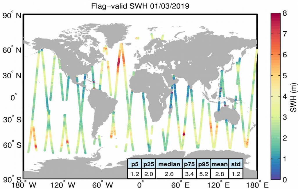
Figure 15. Geographical distribution of flag-valid SWH data over oceans and lakes for 01/03/2019. The statistical values shown in the table refer to the SWH in m and are calculated over all measurements shown in the figure.
