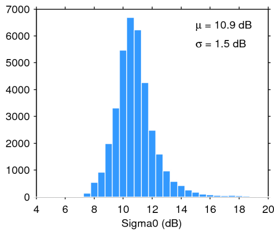
Figure 28. Histogram of science-valid sigma0 over oceans and lakes for 01/03/2019. The mean ( \mu ) and standard deviation ( \sigma ) are also shown. Note that values outside [4 20] dB are excluded from the histogram for the sake of readability but not from the computation of \mu and \sigma .
