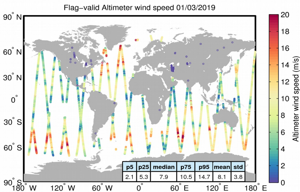
Figure 31. Geographical distribution of flag-valid wind data over oceans and lakes for 01/03/2019. The statistical values shown in the table refer to the wind in m/s and are calculated over all measurements shown in the figure.
