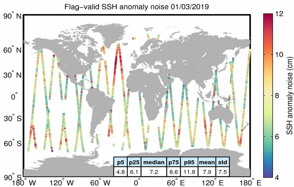
Figure 8. Geographical distribution of flag-valid 20-Hz SSH anomaly measurement noise over oceans and lakes for 01/03/2019. The statistical values shown in the table refer to the SSH anomaly noise and are calculated over all measurements shown in the figure.
