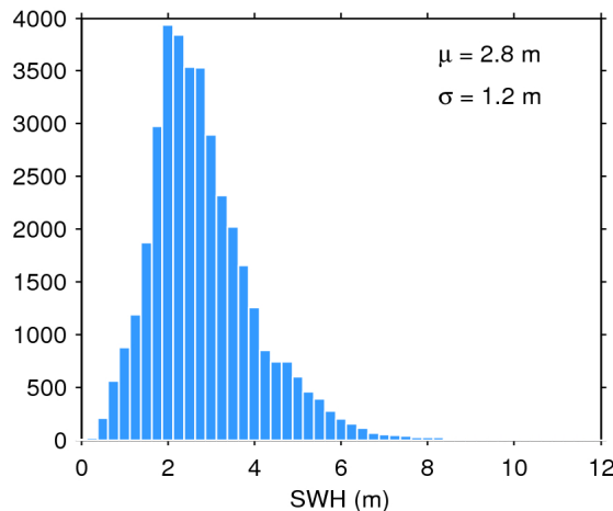
Figure 20. Histogram of science-valid SWH over oceans and lakes for 01/03/2019. The mean ( \mu ) and standard deviation ( \sigma ) are also shown. Note that values larger than 12 m are excluded from the histogram for the sake of readability but not from the computation of \mu and \sigma .
