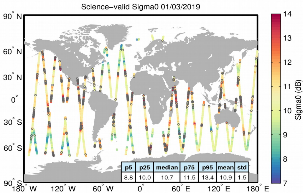
Figure 27. Geographical distribution of science-valid sigma0 data over oceans and lakes for 01/03/2019. The statistical values shown in the table refer to the sigma0 in dB and are calculated over all measurements shown in the figure. Gray circles denote records that have been rejected based on the editing criteria described in Table 4.
