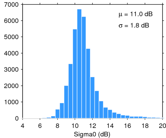
Figure 25. Histogram of flag-valid sigma0 over oceans and lakes for 01/03/2019. The mean ( \mu ) and standard deviation ( \sigma ) are also shown. Note that values outside [4 20] dB are excluded from the histogram for the sake of readability but not from the computation of \mu and \sigma .
