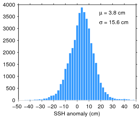
Figure 7. Histogram of flag-valid SSH anomaly over oceans and lakes for 28/02/2019. The mean ( \mu ) and standard deviation ( \sigma ) are also shown. Note that values outside [-50 50] cm are excluded from the histogram for the sake of readability but not from the computation of \mu and \sigma .
