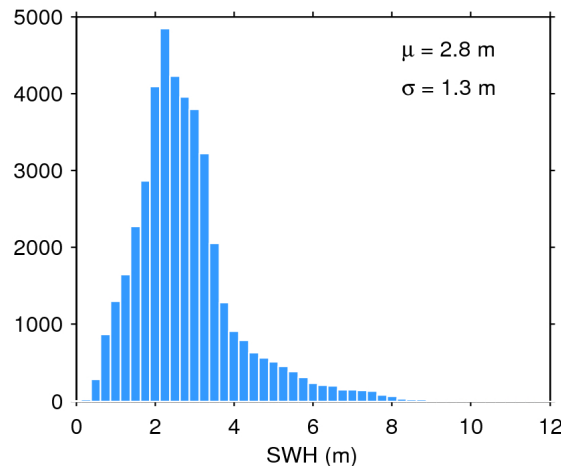
Figure 20. Histogram of science-valid SWH over oceans and lakes for 28/02/2019. The mean ( \mu ) and standard deviation ( \sigma ) are also shown. Note that values larger than 12 m are excluded from the histogram for the sake of readability but not from the computation of \mu and \sigma .
