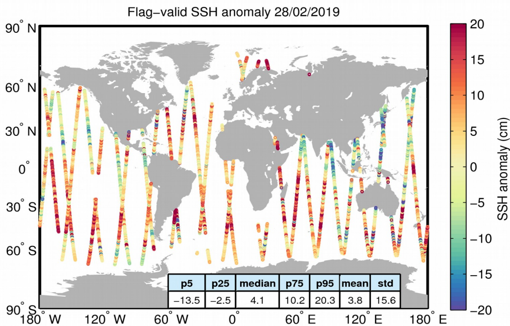
Figure 5. Geographical distribution of flag-valid 1-Hz SSH anomaly data over oceans and lakes for 28/02/2019. The statistical values shown in the table refer to the SSH anomaly in cm and are calculated over all measurements shown in the figure.
