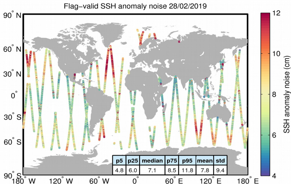
Figure 8. Geographical distribution of flag-valid 20-Hz SSH anomaly measurement noise over oceans and lakes for 28/02/2019. The statistical values shown in the table refer to the SSH anomaly noise and are calculated over all measurements shown in the figure.
