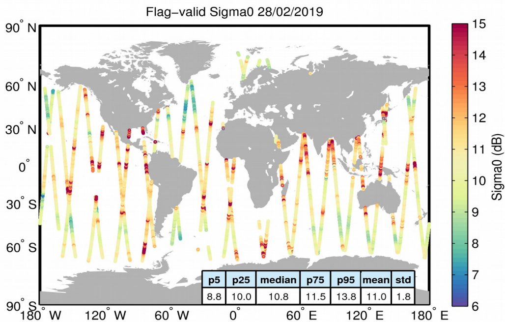
Figure 23. Geographical distribution of flag-valid sigma0 data over oceans and lakes for 28/02/2019. The statistical values shown in the table refer to the sigma0 in dB and are calculated over all measurements shown in the figure.
