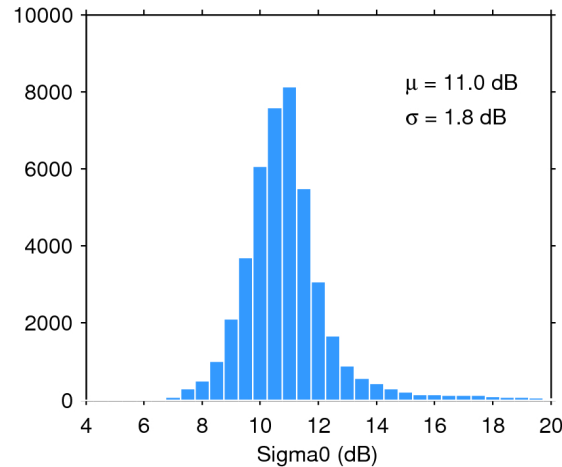
Figure 25. Histogram of flag-valid sigma0 over oceans and lakes for 28/02/2019. The mean ( \mu ) and standard deviation ( \sigma ) are also shown. Note that values outside [4 20] dB are excluded from the histogram for the sake of readability but not from the computation of \mu and \sigma .
