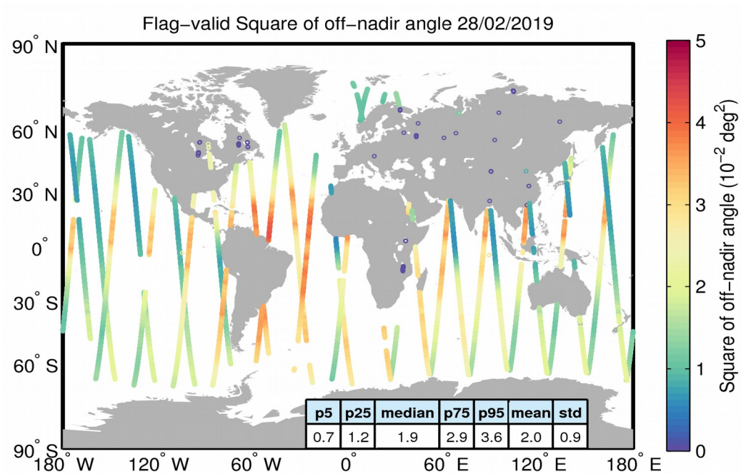
Figure 37. Geographical distribution of flag-valid mispointing data over oceans and lakes for 28/02/2019. The statistical values shown in the table refer to the mispointing in 10^{-2} deg 2 and are calculated over all measurements shown in the figure.
