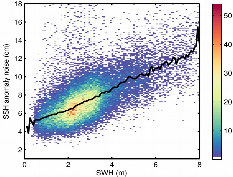
Figure 9. 2D histogram showing flag-valid SSH anomaly noise as a function of SWH for 28/02/2019. The black line denotes the median SSH anomaly noise as a function of SWH.
