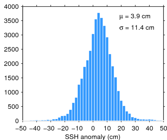
Figure 11. Histogram of science-valid SSH anomaly over oceans and lakes for 28/02/2019. The mean ( \mu ) and standard deviation ( \sigma ) are also shown. Note that values outside [-50 50] cm are excluded from the histogram for the sake of readability but not from the computation of \mu and \sigma .
