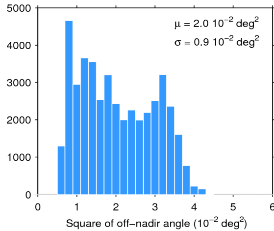
Figure 39. Histogram of flag-valid mispointing over oceans and lakes for 28/02/2019. The mean ( \mu ) and standard deviation ( \sigma ) are also shown. Note that values larger than 6 \cdot 10^{-2} \text{ deg}^2 are excluded from the histogram for the sake of readability but not from the computation of \mu and \sigma .
