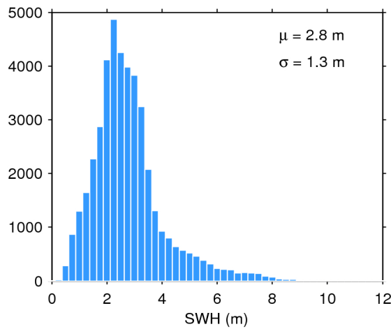
Figure 17. Histogram of flag-valid SWH over oceans and lakes for 28/02/2019. The mean ( \mu ) and standard deviation ( \sigma ) are also shown. Note that values larger than 12 m are excluded from the histogram for the sake of readability but not from the computation of \mu and \sigma .
