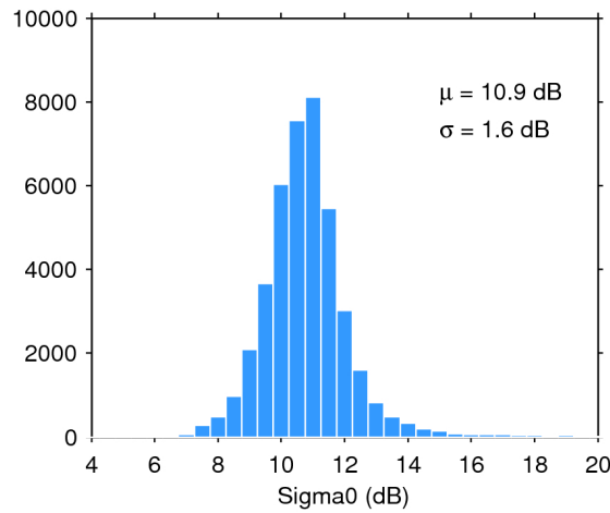
Figure 28. Histogram of science-valid sigma0 over oceans and lakes for 28/02/2019. The mean ( \mu ) and standard deviation ( \sigma ) are also shown. Note that values outside [4 20] dB are excluded from the histogram for the sake of readability but not from the computation of \mu and \sigma .
