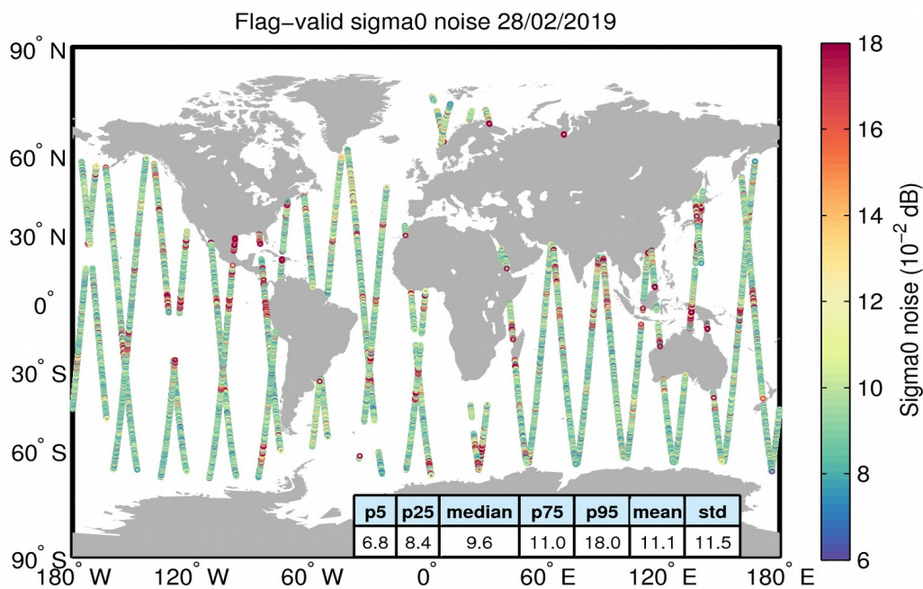
Figure 26. Geographical distribution of flag-valid 20-Hz sigma0 measurement noise over oceans and lakes for 28/02/2019. The statistical values shown in the table refer to the sigma0 noise and are calculated over all measurements shown in the figure.
