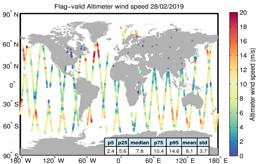
Figure 31. Geographical distribution of flag-valid wind data over oceans and lakes for 28/02/2019. The statistical values shown in the table refer to the wind in m/s and are calculated over all measurements shown in the figure.
