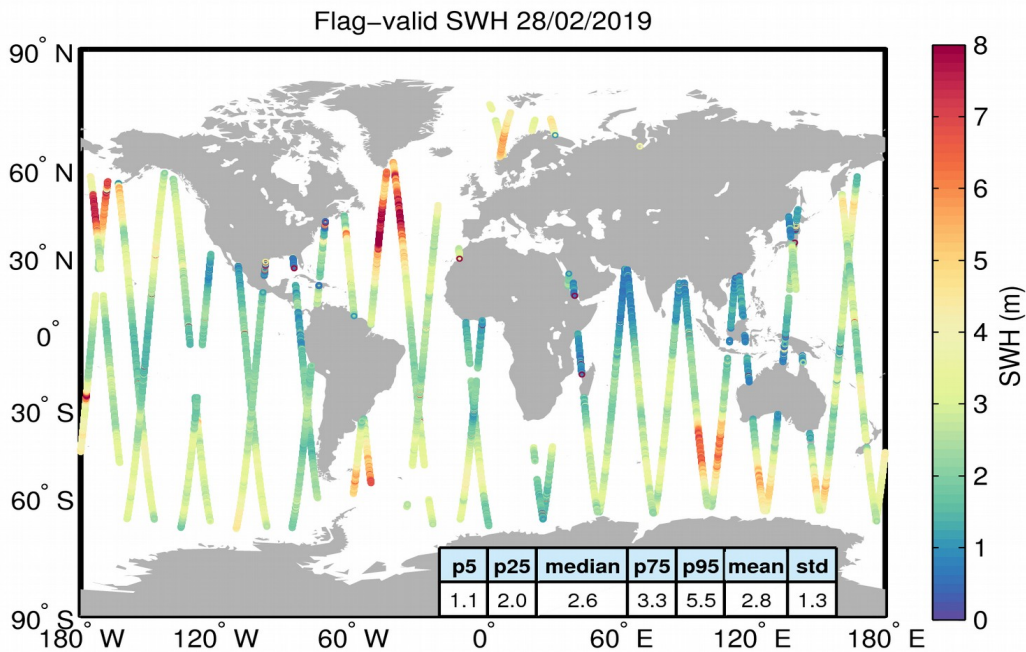
Figure 15. Geographical distribution of flag-valid SWH data over oceans and lakes for 28/02/2019. The statistical values shown in the table refer to the SWH in m and are calculated over all measurements shown in the figure.
