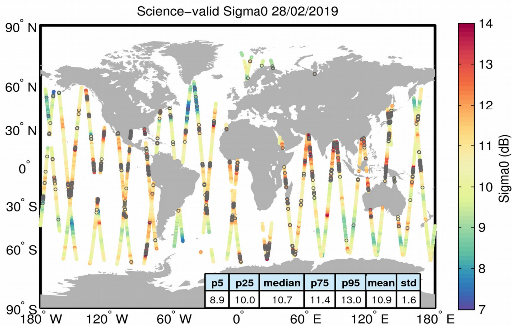
Figure 27. Geographical distribution of science-valid sigma0 data over oceans and lakes for 28/02/2019. The statistical values shown in the table refer to the sigma0 in dB and are calculated over all measurements shown in the figure. Gray circles denote records that have been rejected based on the editing criteria described in Table 4.
