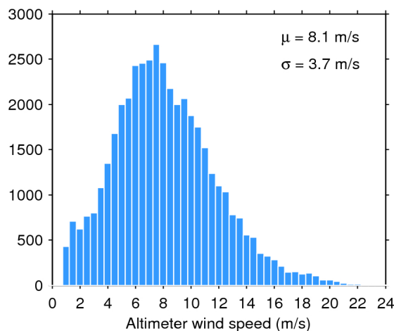
Figure 35. Histogram of science-valid wind over oceans and lakes for 28/02/2019. The mean ( \mu ) and standard deviation ( \sigma ) are also shown. Note that values larger than 24 m/s are excluded from the histogram for the sake of readability but not from the computation of \mu and \sigma .
