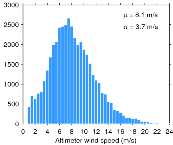
Figure 33. Histogram of flag-valid wind over oceans and lakes for 28/02/2019. The mean ( \mu ) and standard deviation ( \sigma ) are also shown. Note that values larger than 24 m/s are excluded from the histogram for the sake of readability but not from the computation of \mu and \sigma .
