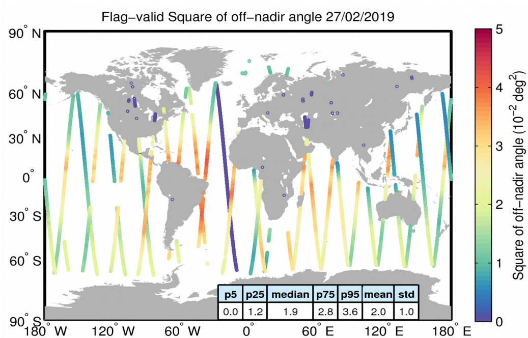
Figure 37. Geographical distribution of flag-valid mispointing data over oceans and lakes for 27/02/2019. The statistical values shown in the table refer to the mispointing in 10^{-2} deg 2 and are calculated over all measurements shown in the figure.
