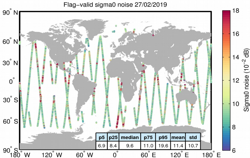
Figure 26. Geographical distribution of flag-valid 20-Hz sigma0 measurement noise over oceans and lakes for 27/02/2019. The statistical values shown in the table refer to the sigma0 noise and are calculated over all measurements shown in the figure.
