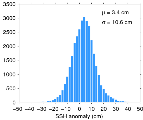
Figure 11. Histogram of science-valid SSH anomaly over oceans and lakes for 27/02/2019. The mean ( \mu ) and standard deviation ( \sigma ) are also shown. Note that values outside [-50 50] cm are excluded from the histogram for the sake of readability but not from the computation of \mu and \sigma .
