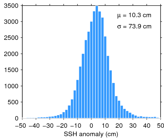
Figure 7. Histogram of flag-valid SSH anomaly over oceans and lakes for 27/02/2019. The mean ( \mu ) and standard deviation ( \sigma ) are also shown. Note that values outside [-50\ 50] cm are excluded from the histogram for the sake of readability but not from the computation of \mu and \sigma .
