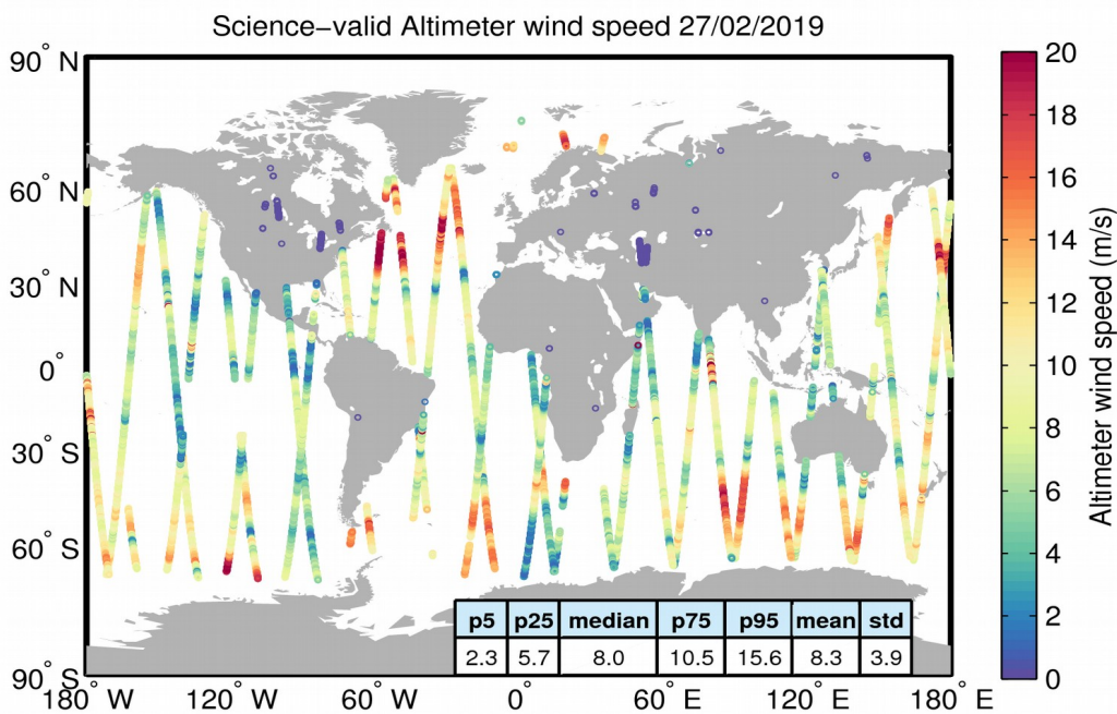
Figure 34. Geographical distribution of science-valid wind data over oceans and lakes for 27/02/2019. The statistical values shown in the table refer to the wind in m/s and are calculated over all measurements shown in the figure. Gray circles denote records that have been rejected based on the editing criteria described in Table 5.
