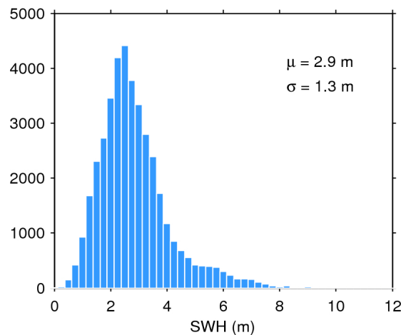
Figure 20. Histogram of science-valid SWH over oceans and lakes for 27/02/2019. The mean ( \mu ) and standard deviation ( \sigma ) are also shown. Note that values larger than 12 m are excluded from the histogram for the sake of readability but not from the computation of \mu and \sigma .
