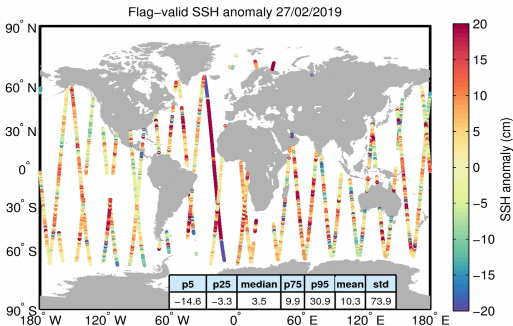
Figure 5. Geographical distribution of flag-valid 1-Hz SSH anomaly data over oceans and lakes for 27/02/2019. The statistical values shown in the table refer to the SSH anomaly in cm and are calculated over all measurements shown in the figure.
