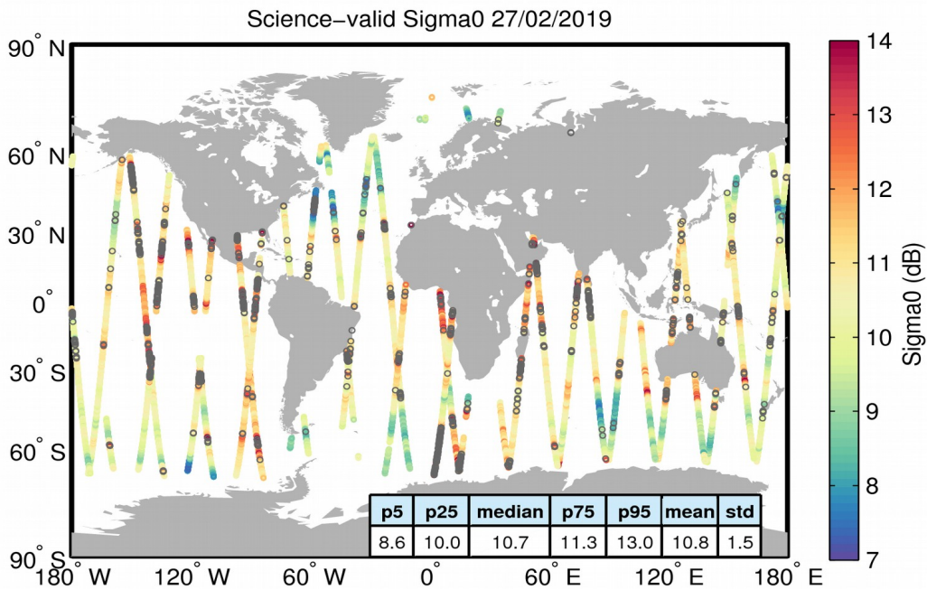
Figure 27. Geographical distribution of science-valid sigma0 data over oceans and lakes for 27/02/2019. The statistical values shown in the table refer to the sigma0 in dB and are calculated over all measurements shown in the figure. Gray circles denote records that have been rejected based on the editing criteria described in Table 4.
