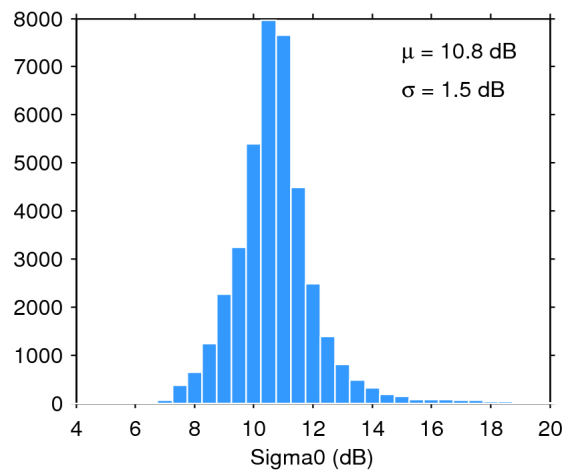
Figure 28. Histogram of science-valid sigma0 over oceans and lakes for 27/02/2019. The mean ( \mu ) and standard deviation ( \sigma ) are also shown. Note that values outside [4 20] dB are excluded from the histogram for the sake of readability but not from the computation of \mu and \sigma .
