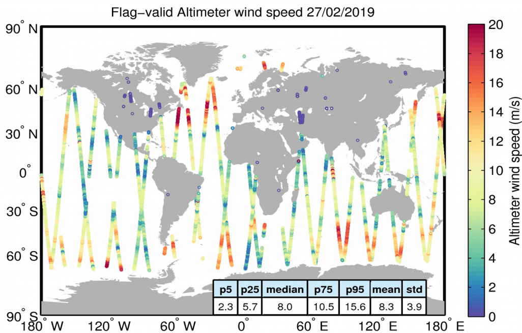
Figure 31. Geographical distribution of flag-valid wind data over oceans and lakes for 27/02/2019. The statistical values shown in the table refer to the wind in m/s and are calculated over all measurements shown in the figure.
