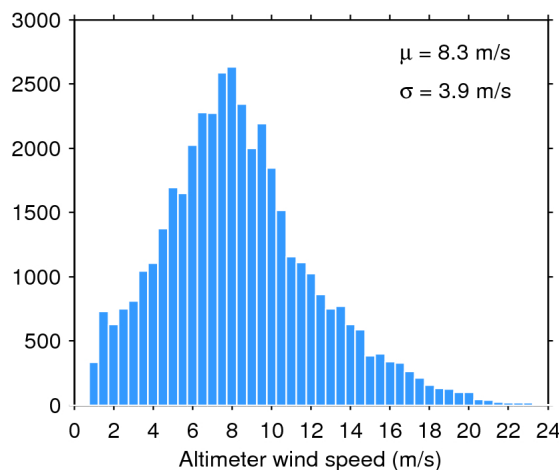
Figure 35. Histogram of science-valid wind over oceans and lakes for 27/02/2019. The mean ( \mu ) and standard deviation ( \sigma ) are also shown. Note that values larger than 24 m/s are excluded from the histogram for the sake of readability but not from the computation of \mu and \sigma .
