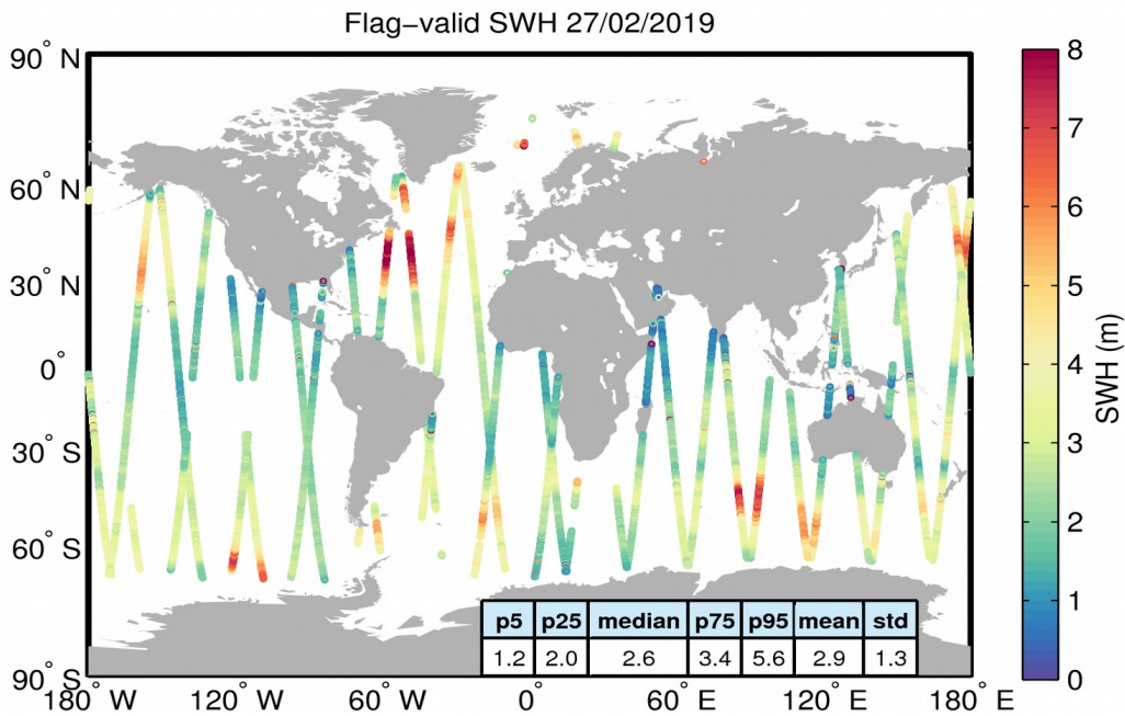
Figure 15. Geographical distribution of flag-valid SWH data over oceans and lakes for 27/02/2019. The statistical values shown in the table refer to the SWH in m and are calculated over all measurements shown in the figure.
