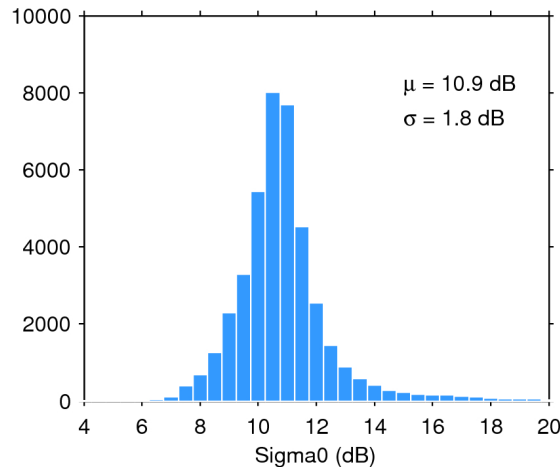
Figure 25. Histogram of flag-valid sigma0 over oceans and lakes for 27/02/2019. The mean ( \mu ) and standard deviation ( \sigma ) are also shown. Note that values outside [4 20] dB are excluded from the histogram for the sake of readability but not from the computation of \mu and \sigma .
