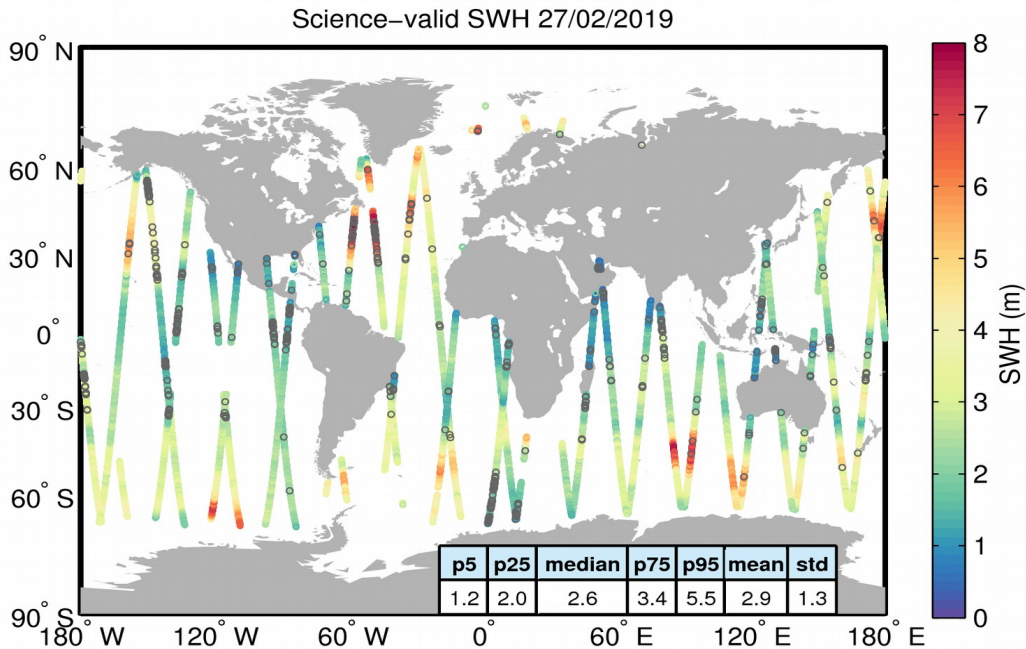
Figure 19. Geographical distribution of science-valid SWH data over oceans and lakes for 27/02/2019. The statistical values shown in the table refer to the SWH in m and are calculated over all measurements shown in the figure. Gray circles denote records that have been rejected based on the editing criteria described in Table 3.
