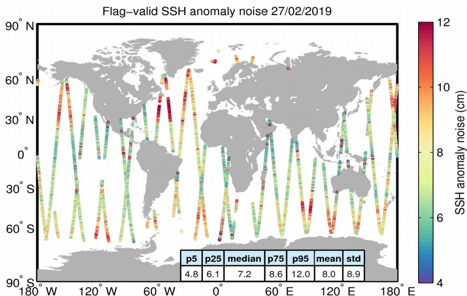
Figure 8. Geographical distribution of flag-valid 20-Hz SSH anomaly measurement noise over oceans and lakes for 27/02/2019. The statistical values shown in the table refer to the SSH anomaly noise and are calculated over all measurements shown in the figure.
