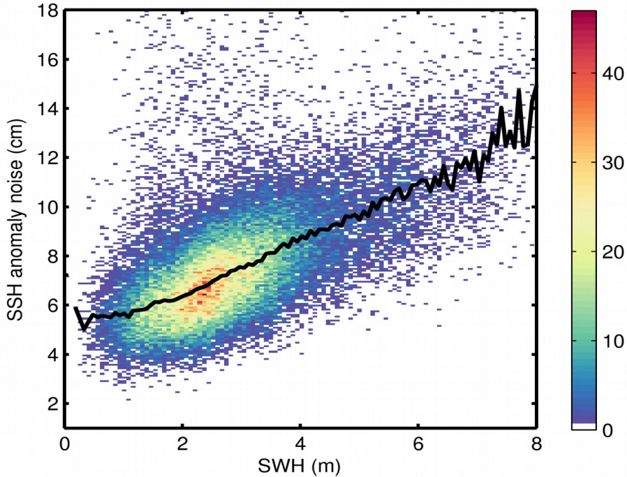
Figure 9. 2D histogram showing flag-valid SSH anomaly noise as a function of SWH for 27/02/2019. The black line denotes the median SSH anomaly noise as a function of SWH.
