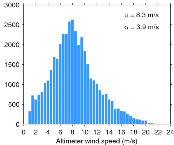
Figure 33. Histogram of flag-valid wind over oceans and lakes for 27/02/2019. The mean ( \mu ) and standard deviation ( \sigma ) are also shown. Note that values larger than 24 m/s are excluded from the histogram for the sake of readability but not from the computation of \mu and \sigma .
