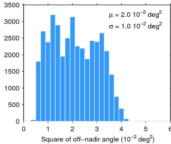
Figure 39. Histogram of flag-valid mispointing over oceans and lakes for 27/02/2019. The mean ( \mu ) and standard deviation ( \sigma ) are also shown. Note that values larger than 6 \cdot 10^{-2} \text{ deg}^2 are excluded from the histogram for the sake of readability but not from the computation of \mu and \sigma .
