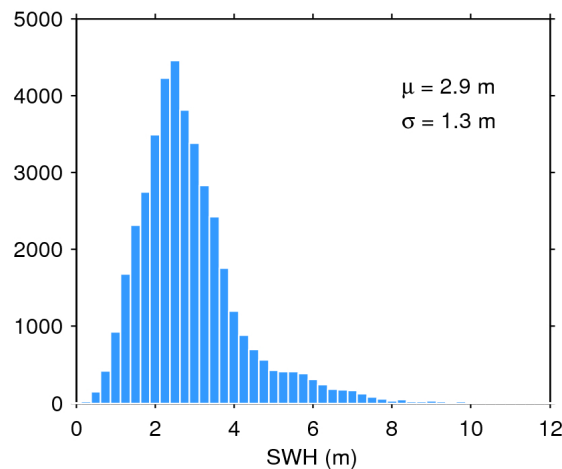
Figure 17. Histogram of flag-valid SWH over oceans and lakes for 27/02/2019. The mean ( \mu ) and standard deviation ( \sigma ) are also shown. Note that values larger than 12 m are excluded from the histogram for the sake of readability but not from the computation of \mu and \sigma .
