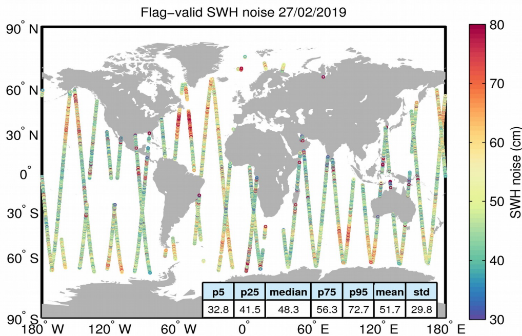
Figure 18. Geographical distribution of flag-valid 20-Hz SWH measurement noise over oceans and lakes for 27/02/2019. The statistical values shown in the figure refer to the SWH noise and are calculated over all measurements shown in the figure.
