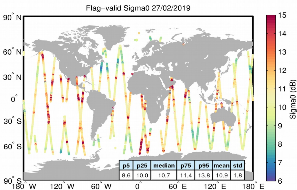
Figure 23. Geographical distribution of flag-valid sigma0 data over oceans and lakes for 27/02/2019. The statistical values shown in the table refer to the sigma0 in dB and are calculated over all measurements shown in the figure.
