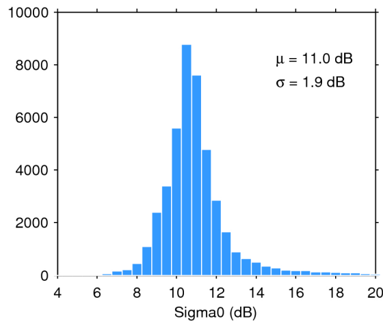
Figure 25. Histogram of flag-valid sigma0 over oceans and lakes for 26/02/2019. The mean ( \mu ) and standard deviation ( \sigma ) are also shown. Note that values outside [4 20] dB are excluded from the histogram for the sake of readability but not from the computation of \mu and \sigma .
