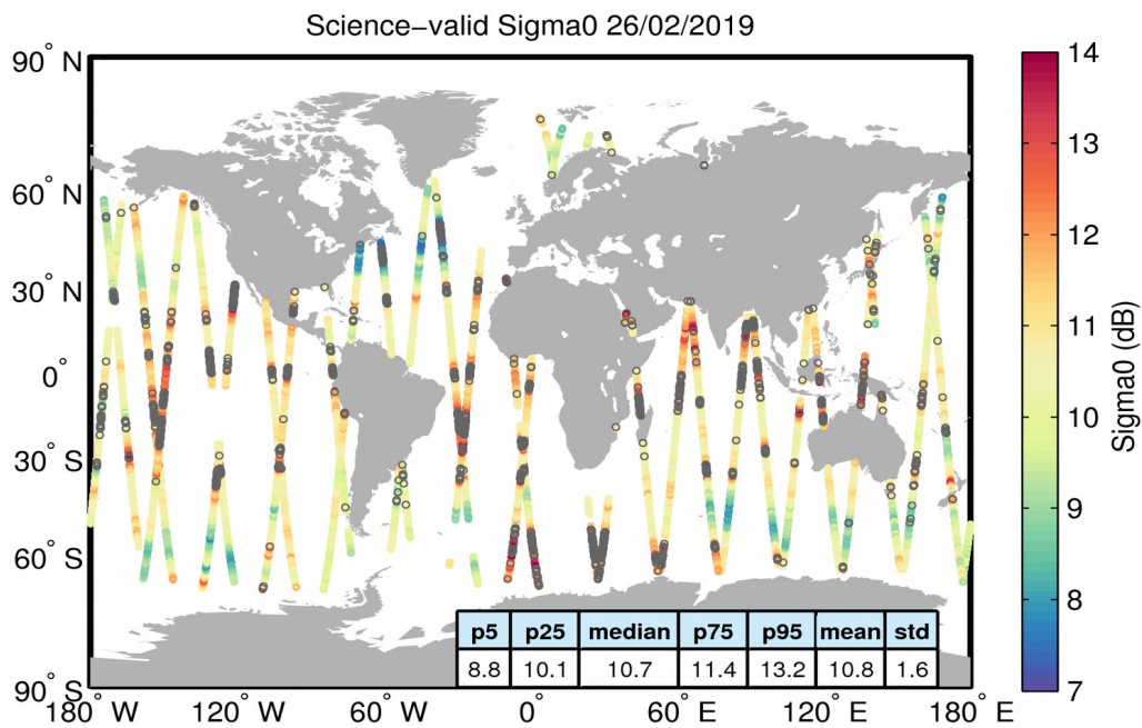
Figure 27. Geographical distribution of science-valid sigma0 data over oceans and lakes for 26/02/2019. The statistical values shown in the table refer to the sigma0 in dB and are calculated over all measurements shown in the figure. Gray circles denote records that have been rejected based on the editing criteria described in Table 4.
