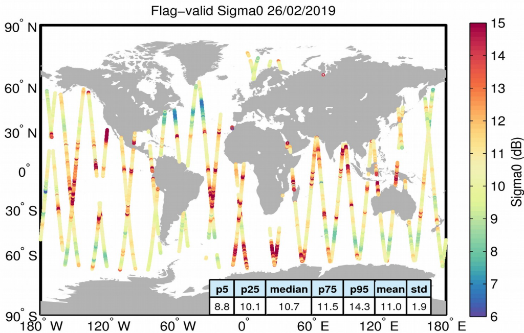
Figure 23. Geographical distribution of flag-valid sigma0 data over oceans and lakes for 26/02/2019. The statistical values shown in the table refer to the sigma0 in dB and are calculated over all measurements shown in the figure.
