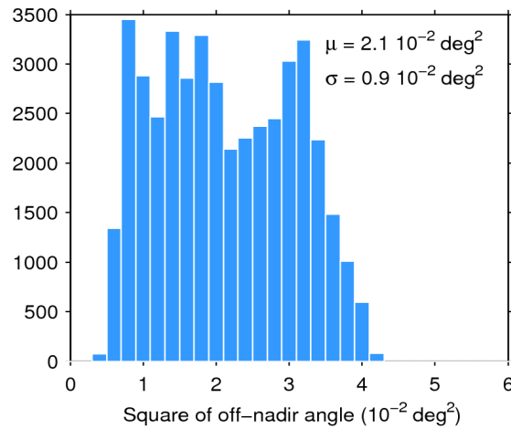
Figure 39. Histogram of flag-valid mispointing over oceans and lakes for 26/02/2019. The mean ( \mu ) and standard deviation ( \sigma ) are also shown. Note that values larger than 6 \cdot 10^{-2} \text{ deg}^2 are excluded from the histogram for the sake of readability but not from the computation of \mu and \sigma .
