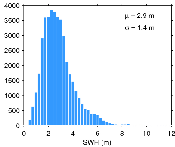
Figure 17. Histogram of flag-valid SWH over oceans and lakes for 26/02/2019. The mean ( \mu ) and standard deviation ( \sigma ) are also shown. Note that values larger than 12 m are excluded from the histogram for the sake of readability but not from the computation of \mu and \sigma .
