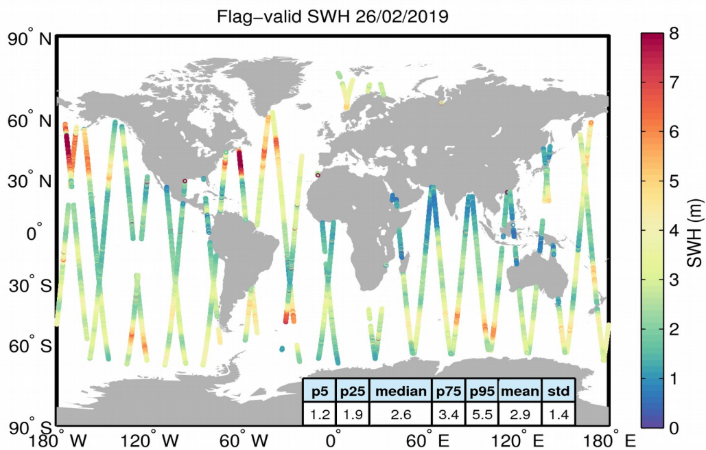
Figure 15. Geographical distribution of flag-valid SWH data over oceans and lakes for 26/02/2019. The statistical values shown in the table refer to the SWH in m and are calculated over all measurements shown in the figure.
