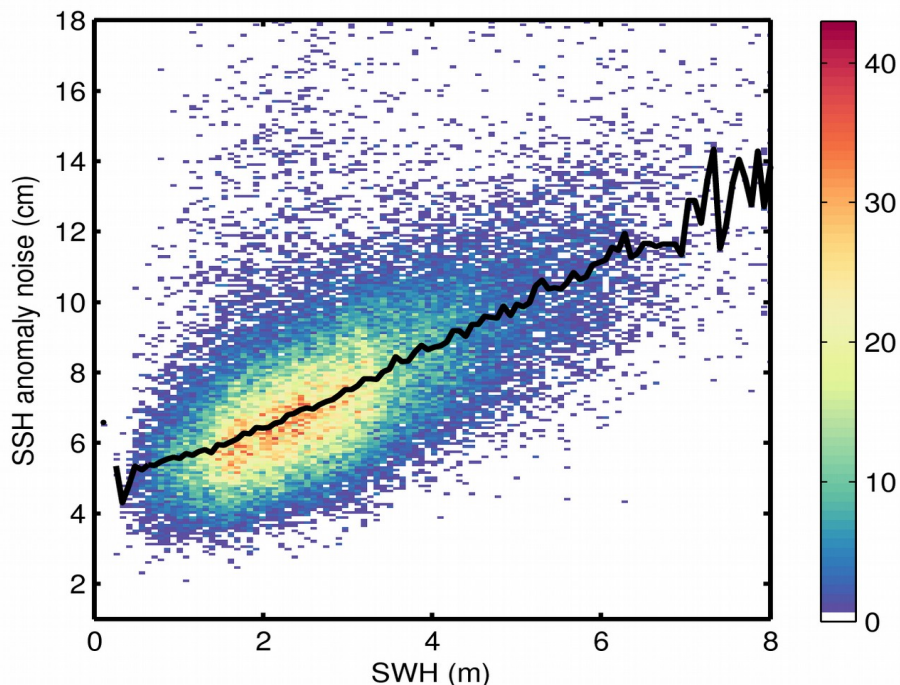
Figure 9. 2D histogram showing flag-valid SSH anomaly noise as a function of SWH for 26/02/2019. The black line denotes the median SSH anomaly noise as a function of SWH.
