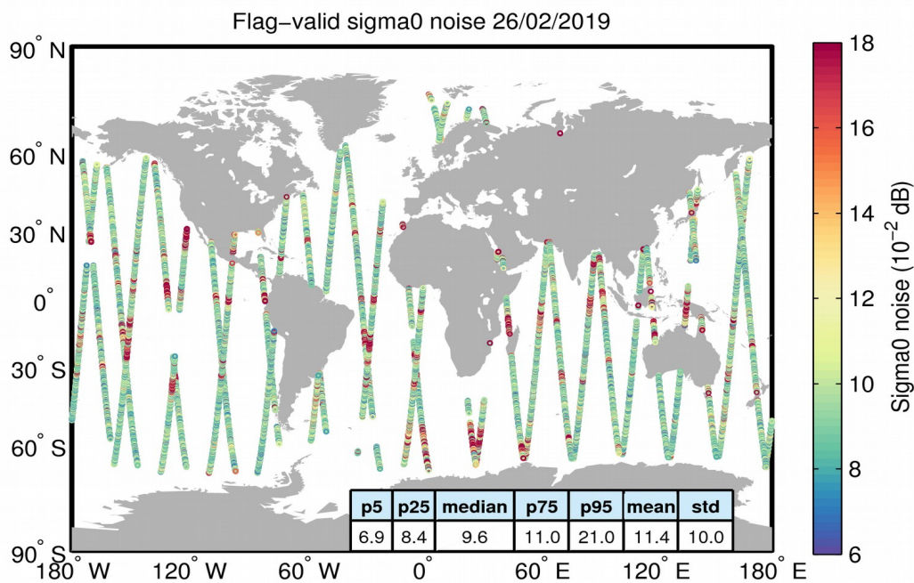
Figure 26. Geographical distribution of flag-valid 20-Hz sigma0 measurement noise over oceans and lakes for 26/02/2019. The statistical values shown in the table refer to the sigma0 noise and are calculated over all measurements shown in the figure.
