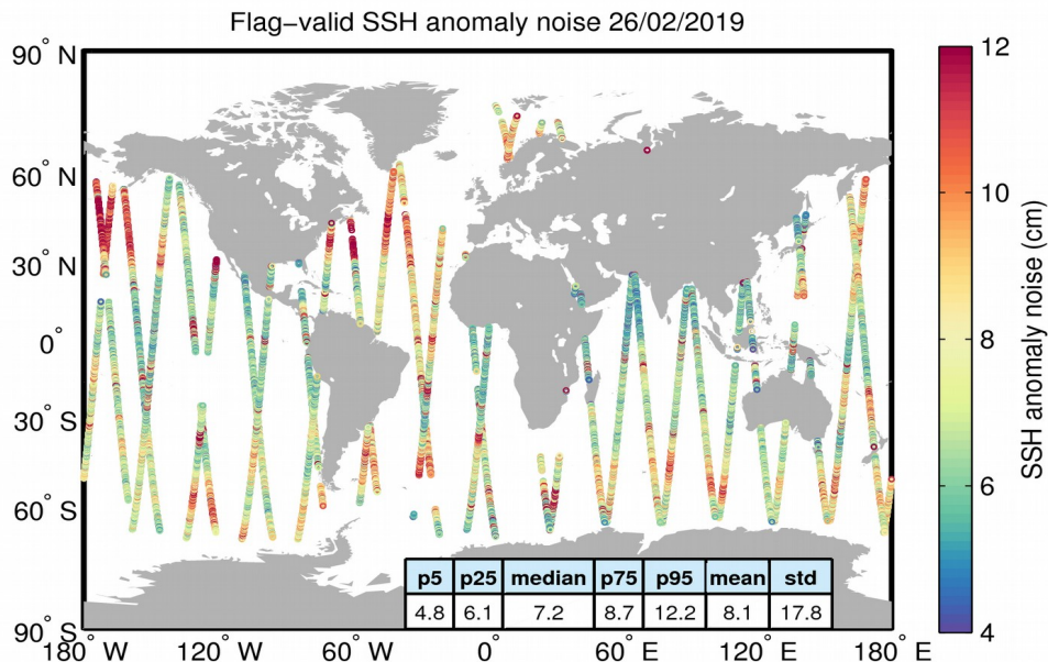
Figure 8. Geographical distribution of flag-valid 20-Hz SSH anomaly measurement noise over oceans and lakes for 26/02/2019. The statistical values shown in the table refer to the SSH anomaly noise and are calculated over all measurements shown in the figure.
