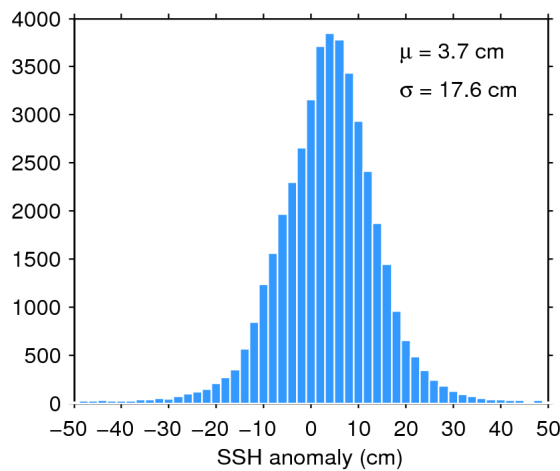
Figure 7. Histogram of flag-valid SSH anomaly over oceans and lakes for 26/02/2019. The mean ( \mu ) and standard deviation ( \sigma ) are also shown. Note that values outside [-50 50] cm are excluded from the histogram for the sake of readability but not from the computation of \mu and \sigma .
