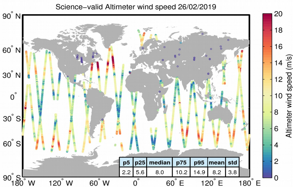
Figure 34. Geographical distribution of science-valid wind data over oceans and lakes for 26/02/2019. The statistical values shown in the table refer to the wind in m/s and are calculated over all measurements shown in the figure. Gray circles denote records that have been rejected based on the editing criteria described in Table 5.
