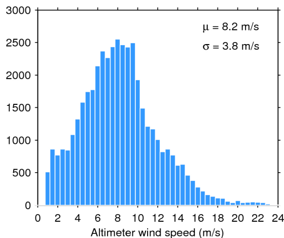
Figure 35. Histogram of science-valid wind over oceans and lakes for 26/02/2019. The mean ( \mu ) and standard deviation ( \sigma ) are also shown. Note that values larger than 24 m/s are excluded from the histogram for the sake of readability but not from the computation of \mu and \sigma .
