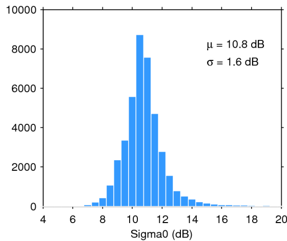
Figure 28. Histogram of science-valid sigma0 over oceans and lakes for 26/02/2019. The mean ( \mu ) and standard deviation ( \sigma ) are also shown. Note that values outside [4 20] dB are excluded from the histogram for the sake of readability but not from the computation of \mu and \sigma .
