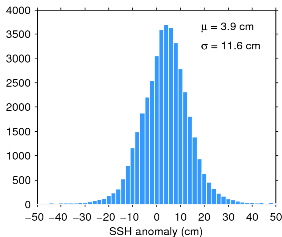
Figure 11. Histogram of science-valid SSH anomaly over oceans and lakes for 26/02/2019. The mean ( \mu ) and standard deviation ( \sigma ) are also shown. Note that values outside [-50 50] cm are excluded from the histogram for the sake of readability but not from the computation of \mu and \sigma .
