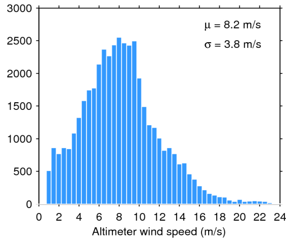
Figure 33. Histogram of flag-valid wind over oceans and lakes for 26/02/2019. The mean ( \mu ) and standard deviation ( \sigma ) are also shown. Note that values larger than 24 m/s are excluded from the histogram for the sake of readability but not from the computation of \mu and \sigma .
