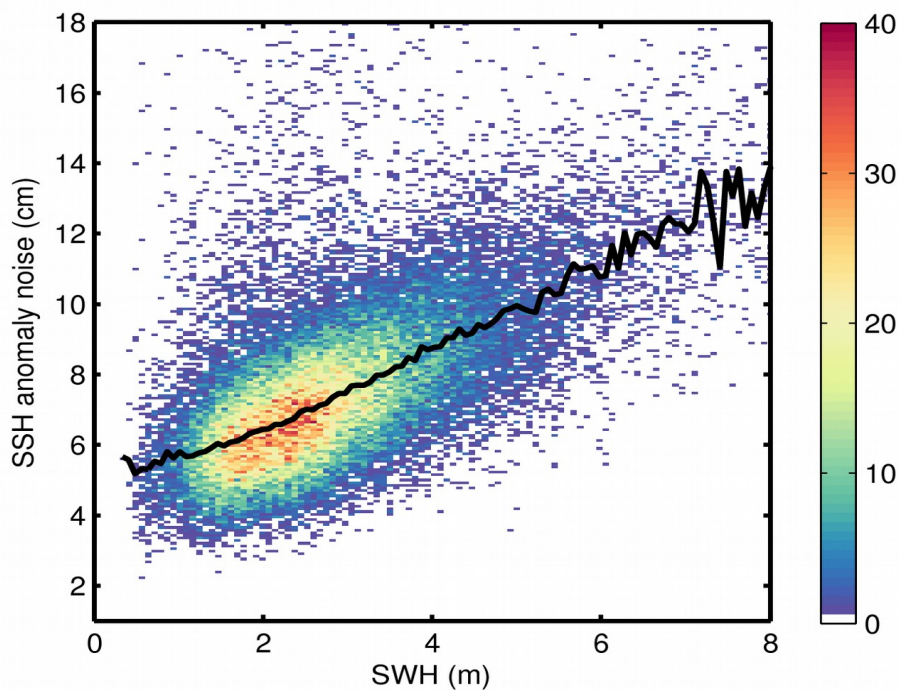
Figure 9. 2D histogram showing flag-valid SSH anomaly noise as a function of SWH for 25/02/2019. The black line denotes the median SSH anomaly noise as a function of SWH.
