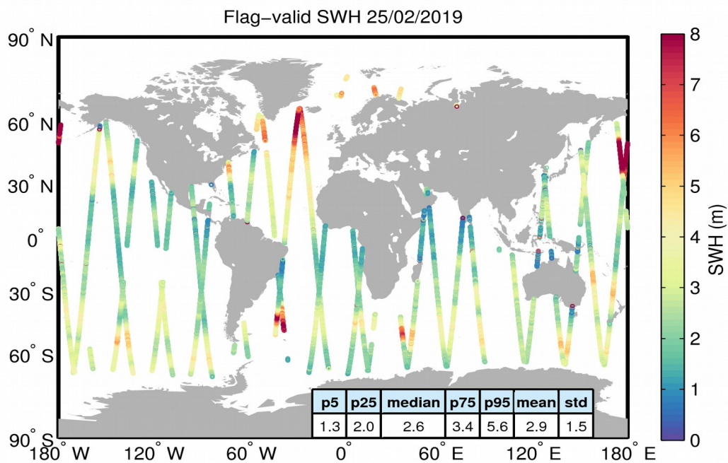
Figure 15. Geographical distribution of flag-valid SWH data over oceans and lakes for 25/02/2019. The statistical values shown in the table refer to the SWH in m and are calculated over all measurements shown in the figure.
