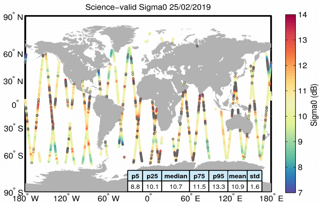
Figure 27. Geographical distribution of science-valid sigma0 data over oceans and lakes for 25/02/2019. The statistical values shown in the table refer to the sigma0 in dB and are calculated over all measurements shown in the figure. Gray circles denote records that have been rejected based on the editing criteria described in Table 4.
