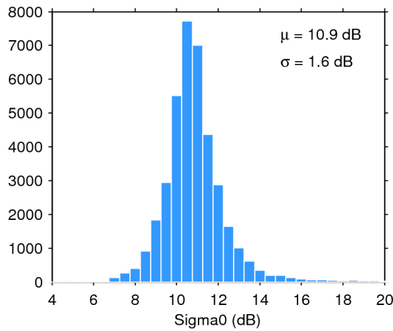
Figure 28. Histogram of science-valid sigma0 over oceans and lakes for 25/02/2019. The mean ( \mu ) and standard deviation ( \sigma ) are also shown. Note that values outside [4 20] dB are excluded from the histogram for the sake of readability but not from the computation of \mu and \sigma .
