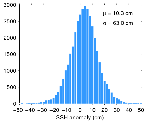
Figure 7. Histogram of flag-valid SSH anomaly over oceans and lakes for 25/02/2019. The mean ( \mu ) and standard deviation ( \sigma ) are also shown. Note that values outside [-50 50] cm are excluded from the histogram for the sake of readability but not from the computation of \mu and \sigma .
