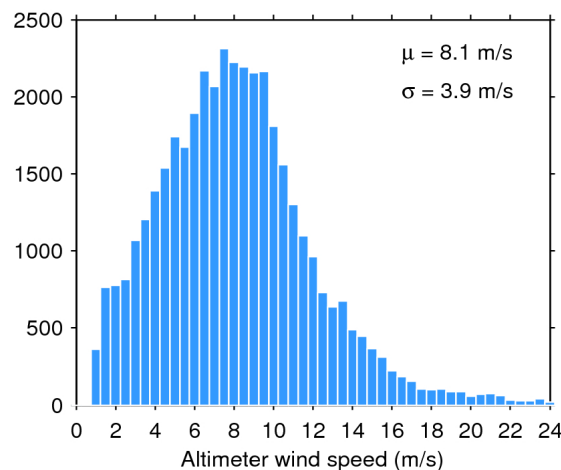
Figure 35. Histogram of science-valid wind over oceans and lakes for 25/02/2019. The mean ( \mu ) and standard deviation ( \sigma ) are also shown. Note that values larger than 24 m/s are excluded from the histogram for the sake of readability but not from the computation of \mu and \sigma .
