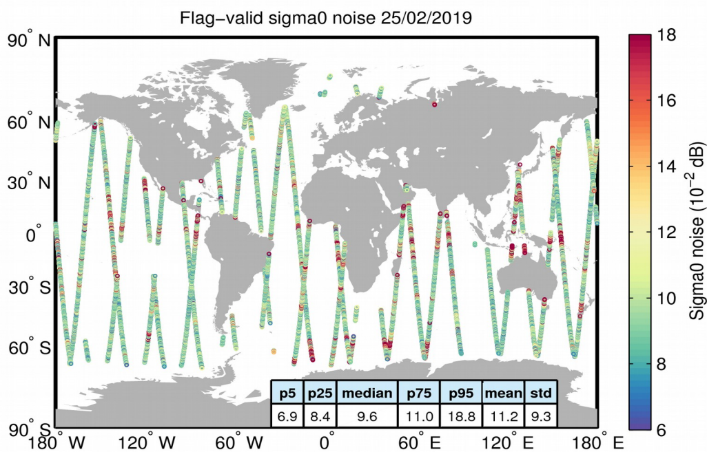
Figure 26. Geographical distribution of flag-valid 20-Hz sigma0 measurement noise over oceans and lakes for 25/02/2019. The statistical values shown in the table refer to the sigma0 noise and are calculated over all measurements shown in the figure.
