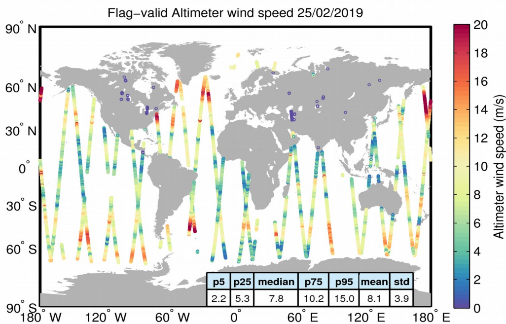
Figure 31. Geographical distribution of flag-valid wind data over oceans and lakes for 25/02/2019. The statistical values shown in the table refer to the wind in m/s and are calculated over all measurements shown in the figure.
