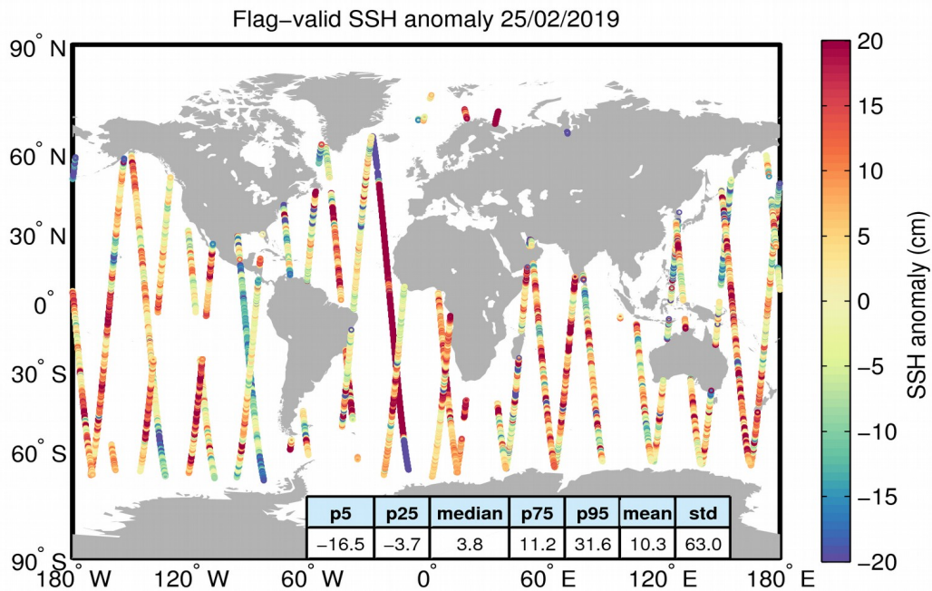
Figure 5. Geographical distribution of flag-valid 1-Hz SSH anomaly data over oceans and lakes for 25/02/2019. The statistical values shown in the table refer to the SSH anomaly in cm and are calculated over all measurements shown in the figure.
