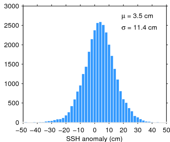
Figure 11. Histogram of science-valid SSH anomaly over oceans and lakes for 25/02/2019. The mean ( \mu ) and standard deviation ( \sigma ) are also shown. Note that values outside [-50 50] cm are excluded from the histogram for the sake of readability but not from the computation of \mu and \sigma .
