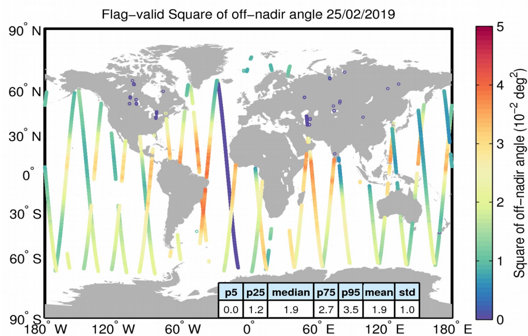
Figure 37. Geographical distribution of flag-valid mispointing data over oceans and lakes for 25/02/2019. The statistical values shown in the table refer to the mispointing in 10^{-2} deg 2 and are calculated over all measurements shown in the figure.
