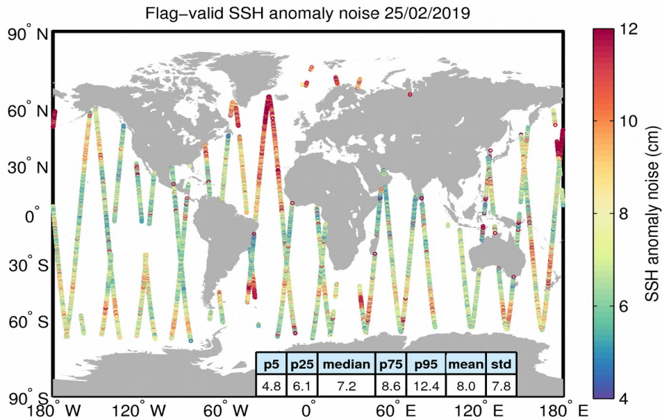
Figure 8. Geographical distribution of flag-valid 20-Hz SSH anomaly measurement noise over oceans and lakes for 25/02/2019. The statistical values shown in the table refer to the SSH anomaly noise and are calculated over all measurements shown in the figure.
