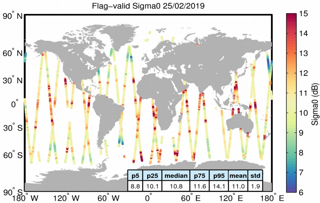
Figure 23. Geographical distribution of flag-valid sigma0 data over oceans and lakes for 25/02/2019. The statistical values shown in the table refer to the sigma0 in dB and are calculated over all measurements shown in the figure.
