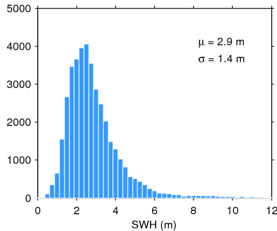
Figure 20. Histogram of science-valid SWH over oceans and lakes for 25/02/2019. The mean ( \mu ) and standard deviation ( \sigma ) are also shown. Note that values larger than 12 m are excluded from the histogram for the sake of readability but not from the computation of \mu and \sigma .
