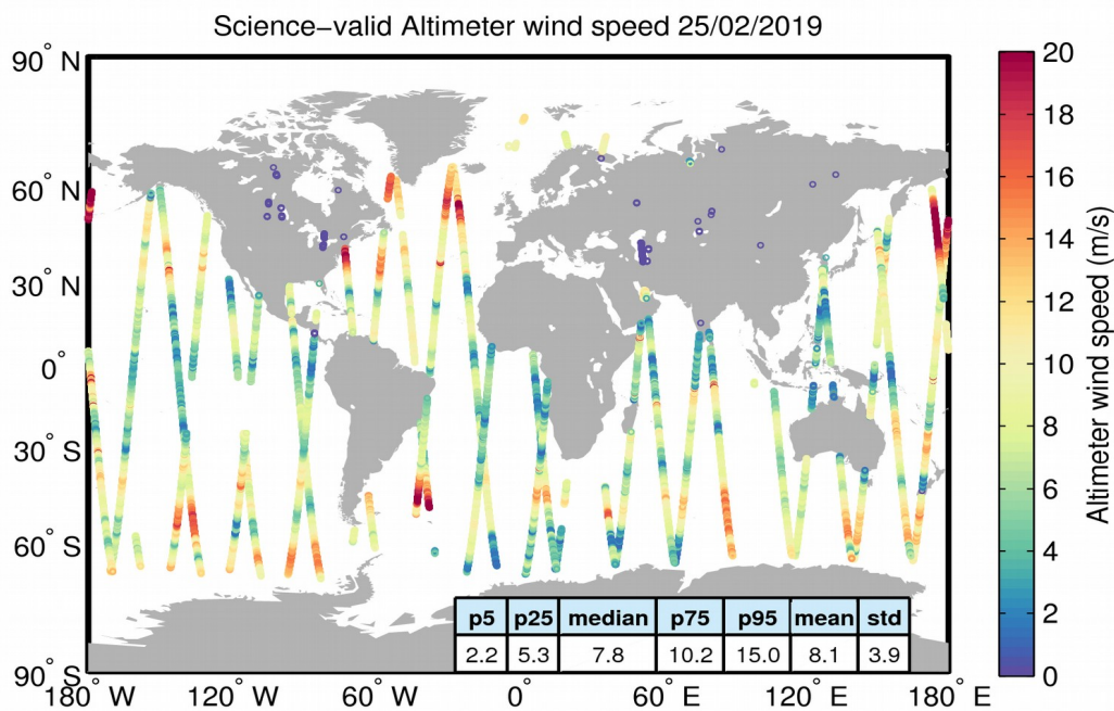
Figure 34. Geographical distribution of science-valid wind data over oceans and lakes for 25/02/2019. The statistical values shown in the table refer to the wind in m/s and are calculated over all measurements shown in the figure. Gray circles denote records that have been rejected based on the editing criteria described in Table 5.
