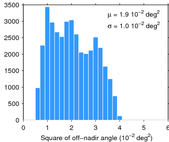
Figure 39. Histogram of flag-valid mispointing over oceans and lakes for 25/02/2019. The mean ( \mu ) and standard deviation ( \sigma ) are also shown. Note that values larger than 6 \cdot 10^{-2} \text{ deg}^2 are excluded from the histogram for the sake of readability but not from the computation of \mu and \sigma .
