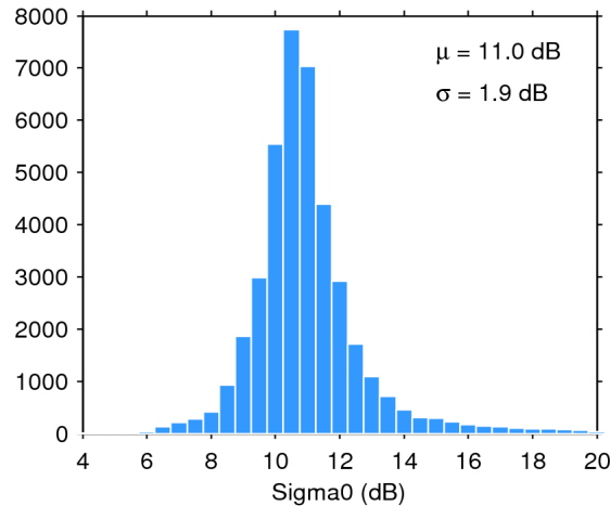
Figure 25. Histogram of flag-valid sigma0 over oceans and lakes for 25/02/2019. The mean ( \mu ) and standard deviation ( \sigma ) are also shown. Note that values outside [4 20] dB are excluded from the histogram for the sake of readability but not from the computation of \mu and \sigma .
