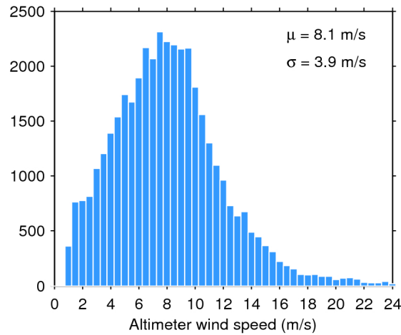
Figure 33. Histogram of flag-valid wind over oceans and lakes for 25/02/2019. The mean ( \mu ) and standard deviation ( \sigma ) are also shown. Note that values larger than 24 m/s are excluded from the histogram for the sake of readability but not from the computation of \mu and \sigma .
