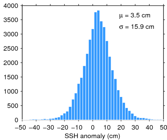
Figure 7. Histogram of flag-valid SSH anomaly over oceans and lakes for 24/02/2019. The mean ( \mu ) and standard deviation ( \sigma ) are also shown. Note that values outside [-50 50] cm are excluded from the histogram for the sake of readability but not from the computation of \mu and \sigma .
