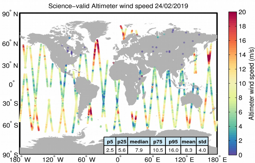
Figure 34. Geographical distribution of science-valid wind data over oceans and lakes for 24/02/2019. The statistical values shown in the table refer to the wind in m/s and are calculated over all measurements shown in the figure. Gray circles denote records that have been rejected based on the editing criteria described in Table 5.
