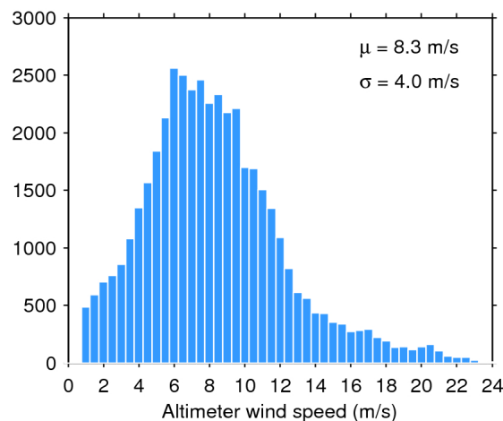
Figure 35. Histogram of science-valid wind over oceans and lakes for 24/02/2019. The mean ( \mu ) and standard deviation ( \sigma ) are also shown. Note that values larger than 24 m/s are excluded from the histogram for the sake of readability but not from the computation of \mu and \sigma .
