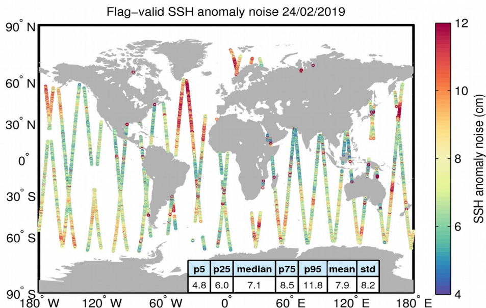
Figure 8. Geographical distribution of flag-valid 20-Hz SSH anomaly measurement noise over oceans and lakes for 24/02/2019. The statistical values shown in the table refer to the SSH anomaly noise and are calculated over all measurements shown in the figure.
