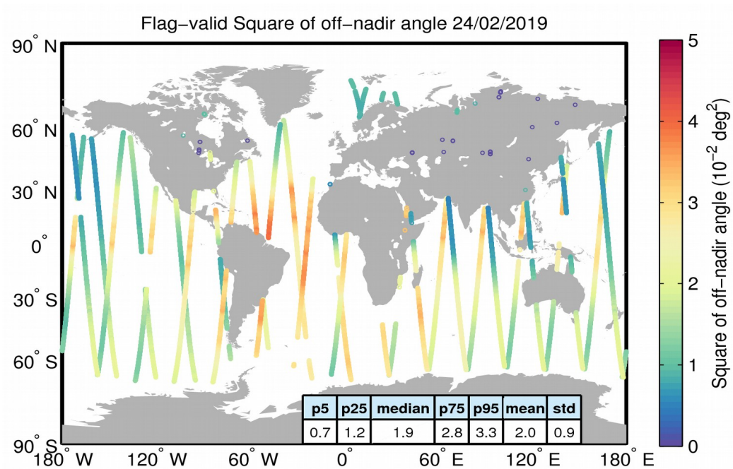
Figure 37. Geographical distribution of flag-valid mispointing data over oceans and lakes for 24/02/2019. The statistical values shown in the table refer to the mispointing in 10^{-2} deg 2 and are calculated over all measurements shown in the figure.
