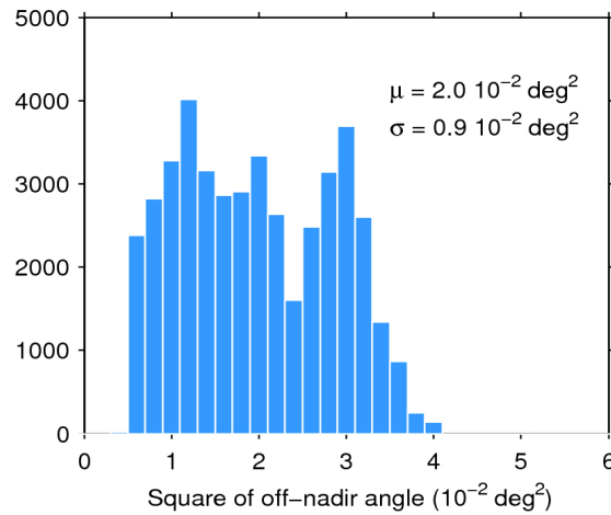
Figure 39. Histogram of flag-valid mispointing over oceans and lakes for 24/02/2019. The mean ( \mu ) and standard deviation ( \sigma ) are also shown. Note that values larger than 6 \cdot 10^{-2} \text{ deg}^2 are excluded from the histogram for the sake of readability but not from the computation of \mu and \sigma .
