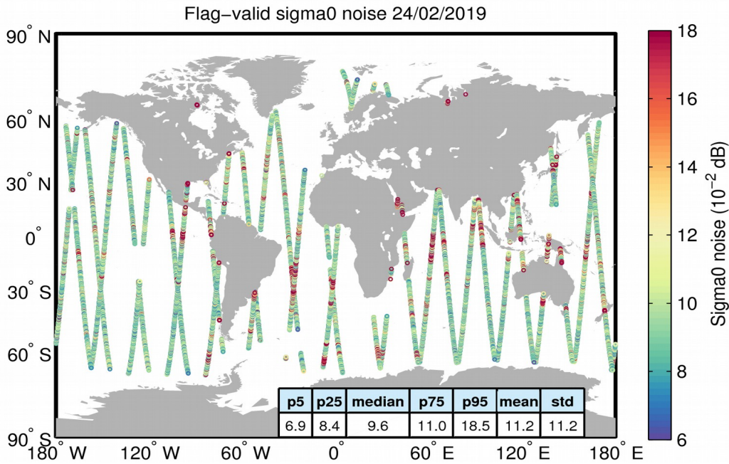
Figure 26. Geographical distribution of flag-valid 20-Hz sigma0 measurement noise over oceans and lakes for 24/02/2019. The statistical values shown in the table refer to the sigma0 noise and are calculated over all measurements shown in the figure.
