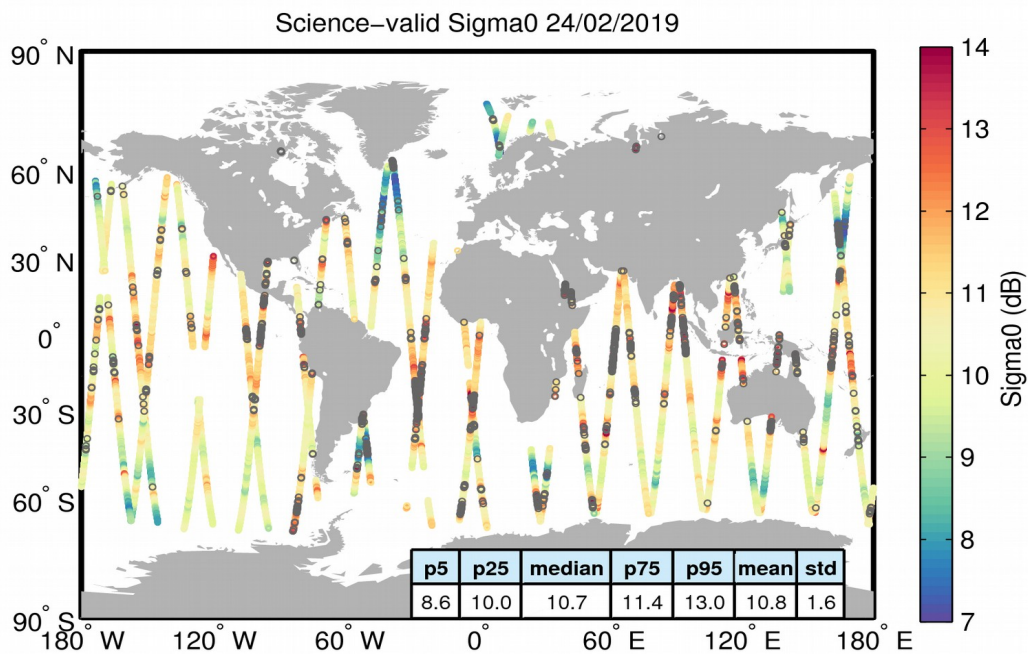
Figure 27. Geographical distribution of science-valid sigma0 data over oceans and lakes for 24/02/2019. The statistical values shown in the table refer to the sigma0 in dB and are calculated over all measurements shown in the figure. Gray circles denote records that have been rejected based on the editing criteria described in Table 4.
