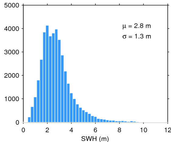
Figure 20. Histogram of science-valid SWH over oceans and lakes for 24/02/2019. The mean ( \mu ) and standard deviation ( \sigma ) are also shown. Note that values larger than 12 m are excluded from the histogram for the sake of readability but not from the computation of \mu and \sigma .
