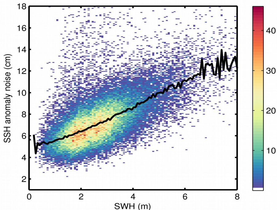
Figure 9. 2D histogram showing flag-valid SSH anomaly noise as a function of SWH for 24/02/2019. The black line denotes the median SSH anomaly noise as a function of SWH.
