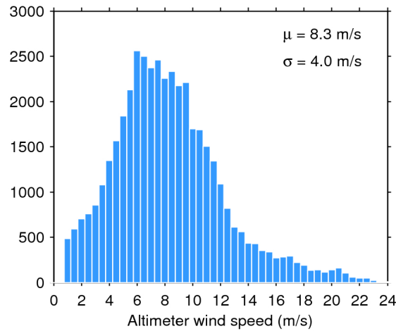
Figure 33. Histogram of flag-valid wind over oceans and lakes for 24/02/2019. The mean ( \mu ) and standard deviation ( \sigma ) are also shown. Note that values larger than 24 m/s are excluded from the histogram for the sake of readability but not from the computation of \mu and \sigma .
