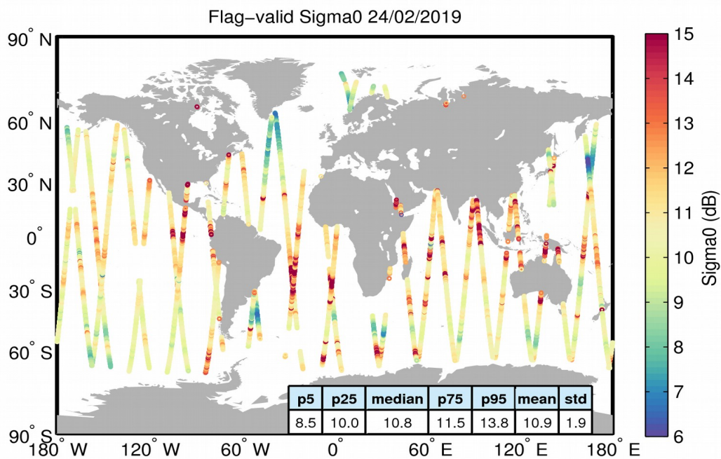
Figure 23. Geographical distribution of flag-valid sigma0 data over oceans and lakes for 24/02/2019. The statistical values shown in the table refer to the sigma0 in dB and are calculated over all measurements shown in the figure.
