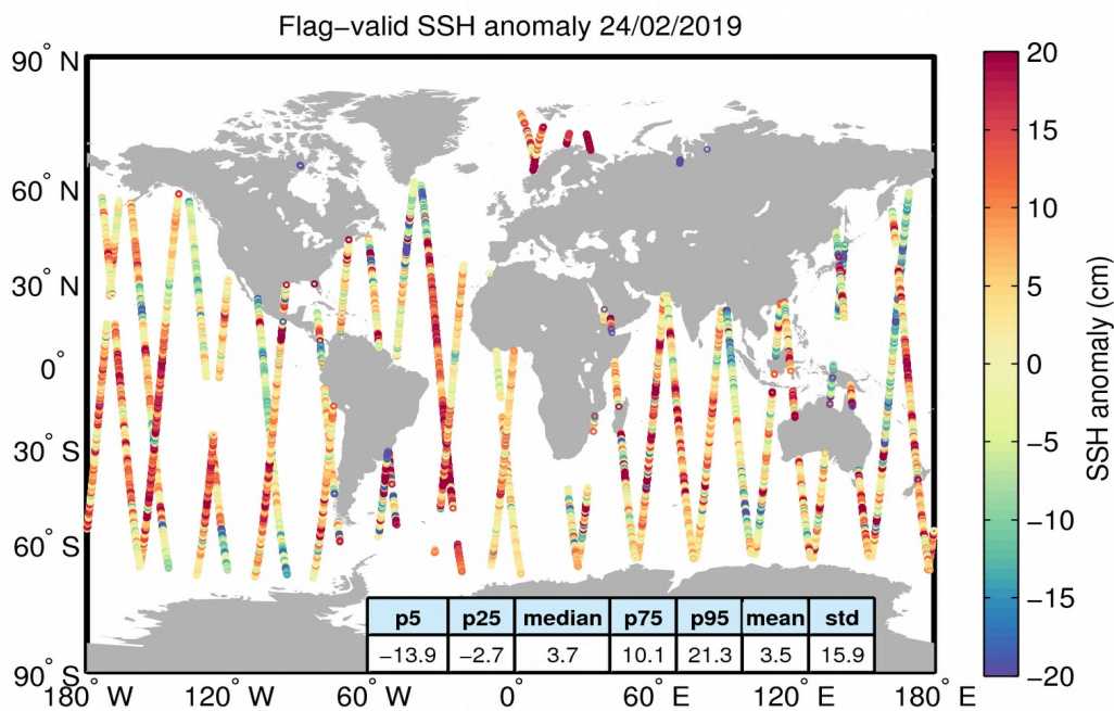
Figure 5. Geographical distribution of flag-valid 1-Hz SSH anomaly data over oceans and lakes for 24/02/2019. The statistical values shown in the table refer to the SSH anomaly in cm and are calculated over all measurements shown in the figure.
