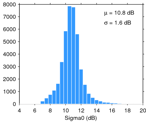
Figure 28. Histogram of science-valid sigma0 over oceans and lakes for 24/02/2019. The mean ( \mu ) and standard deviation ( \sigma ) are also shown. Note that values outside [4 20] dB are excluded from the histogram for the sake of readability but not from the computation of \mu and \sigma .
