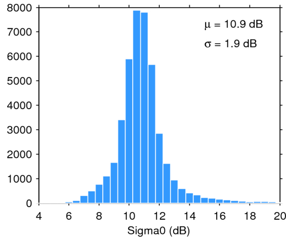
Figure 25. Histogram of flag-valid sigma0 over oceans and lakes for 24/02/2019. The mean ( \mu ) and standard deviation ( \sigma ) are also shown. Note that values outside [4 20] dB are excluded from the histogram for the sake of readability but not from the computation of \mu and \sigma .
