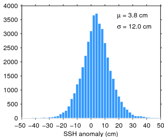
Figure 11. Histogram of science-valid SSH anomaly over oceans and lakes for 24/02/2019. The mean ( \mu ) and standard deviation ( \sigma ) are also shown. Note that values outside [-50 50] cm are excluded from the histogram for the sake of readability but not from the computation of \mu and \sigma .
