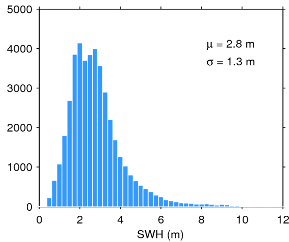
Figure 17. Histogram of flag-valid SWH over oceans and lakes for 24/02/2019. The mean ( \mu ) and standard deviation ( \sigma ) are also shown. Note that values larger than 12 m are excluded from the histogram for the sake of readability but not from the computation of \mu and \sigma .
