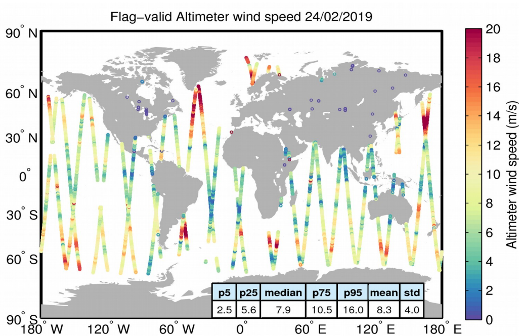
Figure 31. Geographical distribution of flag-valid wind data over oceans and lakes for 24/02/2019. The statistical values shown in the table refer to the wind in m/s and are calculated over all measurements shown in the figure.
