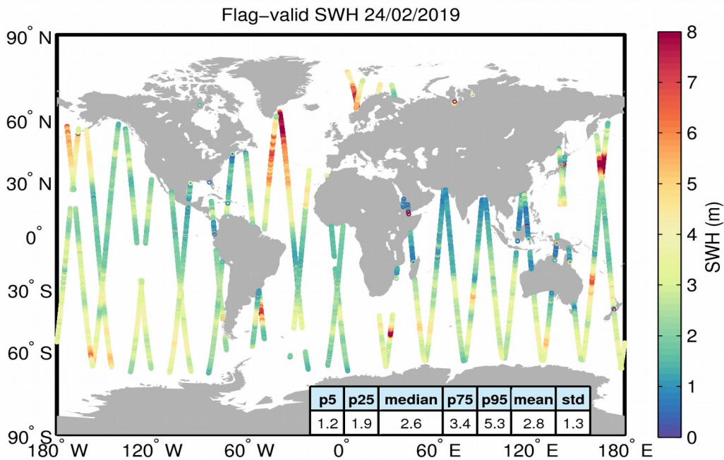
Figure 15. Geographical distribution of flag-valid SWH data over oceans and lakes for 24/02/2019. The statistical values shown in the table refer to the SWH in m and are calculated over all measurements shown in the figure.
