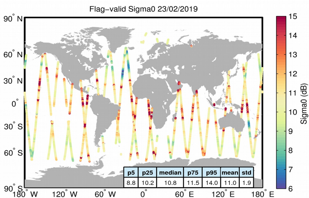
Figure 23. Geographical distribution of flag-valid sigma0 data over oceans and lakes for 23/02/2019. The statistical values shown in the table refer to the sigma0 in dB and are calculated over all measurements shown in the figure.
