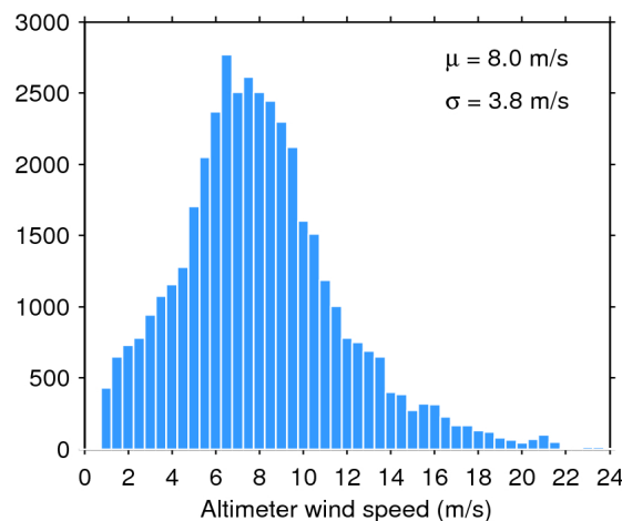
Figure 35. Histogram of science-valid wind over oceans and lakes for 23/02/2019. The mean ( \mu ) and standard deviation ( \sigma ) are also shown. Note that values larger than 24 m/s are excluded from the histogram for the sake of readability but not from the computation of \mu and \sigma .
