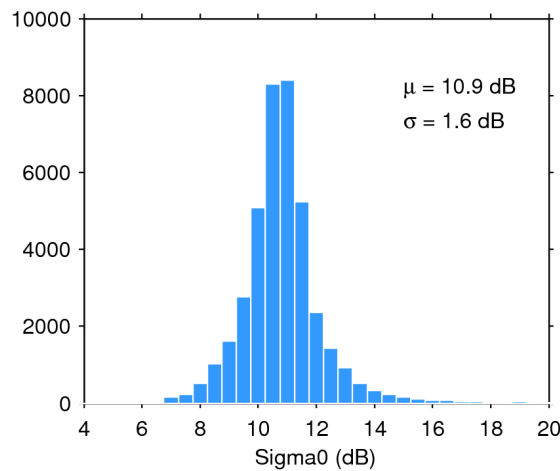
Figure 28. Histogram of science-valid sigma0 over oceans and lakes for 23/02/2019. The mean ( \mu ) and standard deviation ( \sigma ) are also shown. Note that values outside [4 20] dB are excluded from the histogram for the sake of readability but not from the computation of \mu and \sigma .
