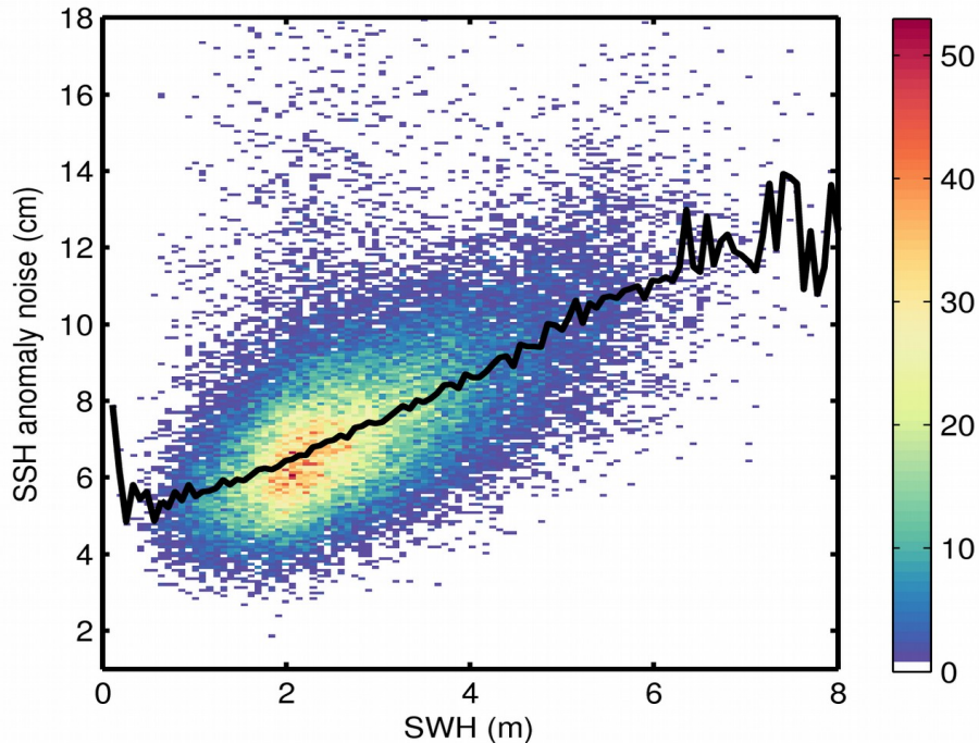
Figure 9. 2D histogram showing flag-valid SSH anomaly noise as a function of SWH for 23/02/2019. The black line denotes the median SSH anomaly noise as a function of SWH.
