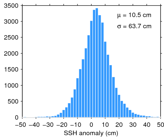
Figure 7. Histogram of flag-valid SSH anomaly over oceans and lakes for 23/02/2019. The mean ( \mu ) and standard deviation ( \sigma ) are also shown. Note that values outside [-50\ 50] cm are excluded from the histogram for the sake of readability but not from the computation of \mu and \sigma .
