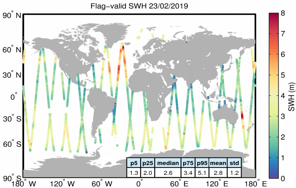
Figure 15. Geographical distribution of flag-valid SWH data over oceans and lakes for 23/02/2019. The statistical values shown in the table refer to the SWH in m and are calculated over all measurements shown in the figure.
