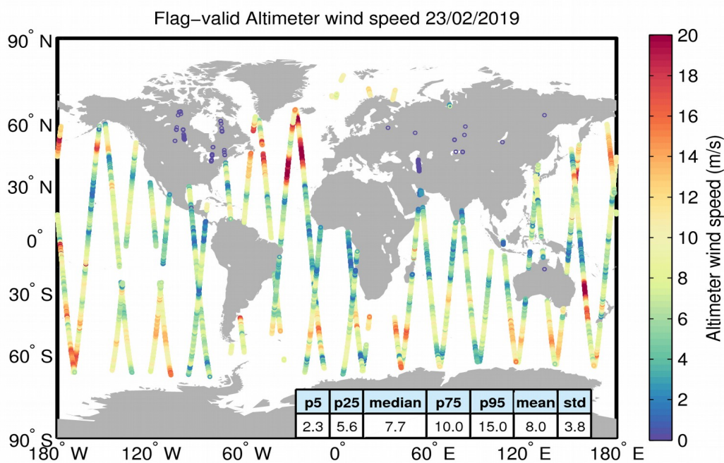
Figure 31. Geographical distribution of flag-valid wind data over oceans and lakes for 23/02/2019. The statistical values shown in the table refer to the wind in m/s and are calculated over all measurements shown in the figure.
