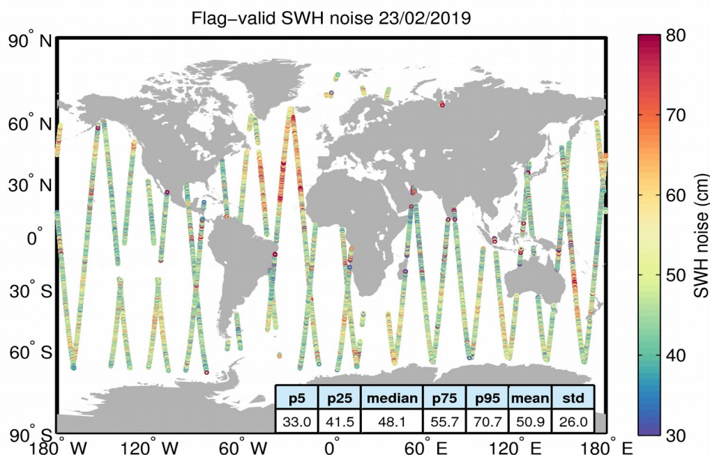
Figure 18. Geographical distribution of flag-valid 20-Hz SWH measurement noise over oceans and lakes for 23/02/2019. The statistical values shown in the figure refer to the SWH noise and are calculated over all measurements shown in the figure.
