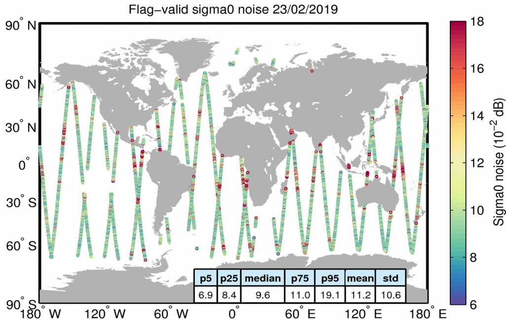
Figure 26. Geographical distribution of flag-valid 20-Hz sigma0 measurement noise over oceans and lakes for 23/02/2019. The statistical values shown in the table refer to the sigma0 noise and are calculated over all measurements shown in the figure.
