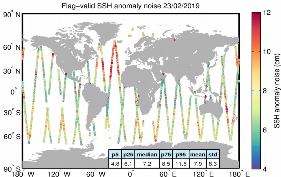
Figure 8. Geographical distribution of flag-valid 20-Hz SSH anomaly measurement noise over oceans and lakes for 23/02/2019. The statistical values shown in the table refer to the SSH anomaly noise and are calculated over all measurements shown in the figure.
