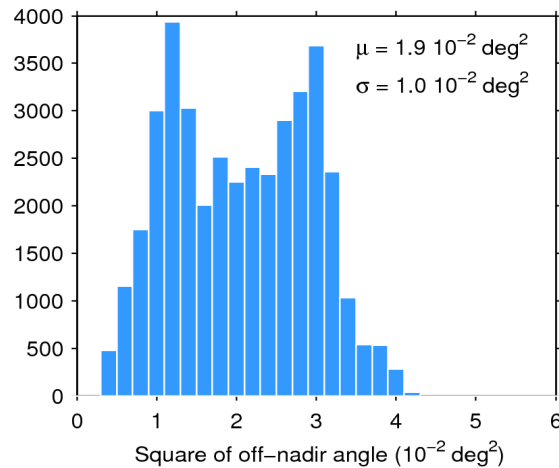
Figure 39. Histogram of flag-valid mispointing over oceans and lakes for 23/02/2019. The mean ( \mu ) and standard deviation ( \sigma ) are also shown. Note that values larger than 6 \cdot 10^{-2} \text{ deg}^2 are excluded from the histogram for the sake of readability but not from the computation of \mu and \sigma .
