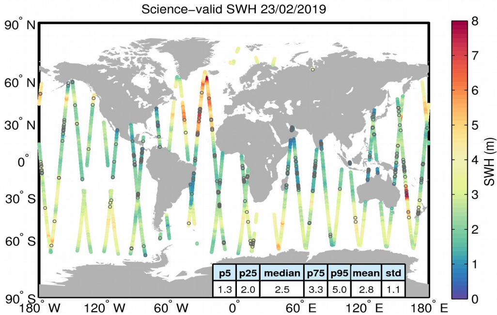
Figure 19. Geographical distribution of science-valid SWH data over oceans and lakes for 23/02/2019. The statistical values shown in the table refer to the SWH in m and are calculated over all measurements shown in the figure. Gray circles denote records that have been rejected based on the editing criteria described in Table 3.
