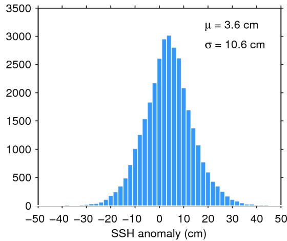
Figure 11. Histogram of science-valid SSH anomaly over oceans and lakes for 23/02/2019. The mean ( \mu ) and standard deviation ( \sigma ) are also shown. Note that values outside [-50 50] cm are excluded from the histogram for the sake of readability but not from the computation of \mu and \sigma .
