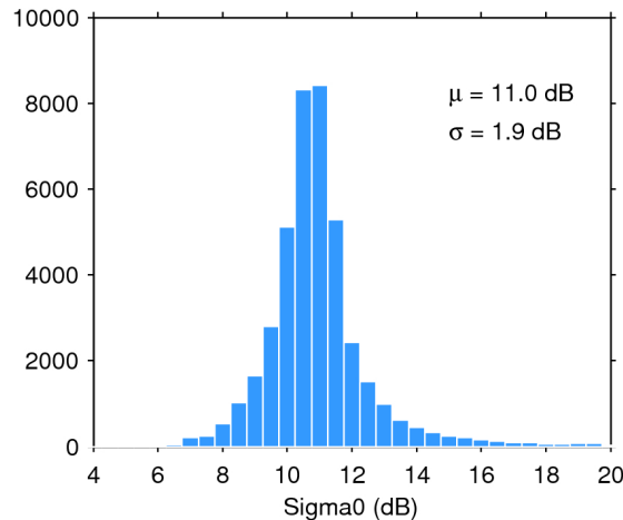
Figure 25. Histogram of flag-valid sigma0 over oceans and lakes for 23/02/2019. The mean ( \mu ) and standard deviation ( \sigma ) are also shown. Note that values outside [4 20] dB are excluded from the histogram for the sake of readability but not from the computation of \mu and \sigma .
