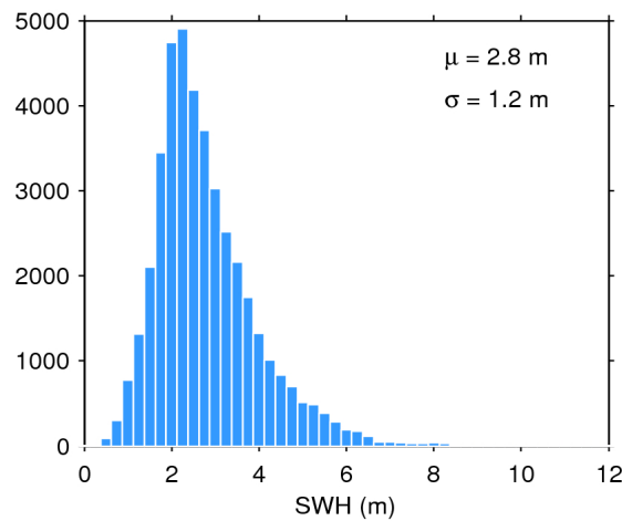
Figure 17. Histogram of flag-valid SWH over oceans and lakes for 23/02/2019. The mean ( \mu ) and standard deviation ( \sigma ) are also shown. Note that values larger than 12 m are excluded from the histogram for the sake of readability but not from the computation of \mu and \sigma .
