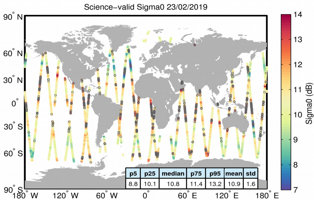
Figure 27. Geographical distribution of science-valid sigma0 data over oceans and lakes for 23/02/2019. The statistical values shown in the table refer to the sigma0 in dB and are calculated over all measurements shown in the figure. Gray circles denote records that have been rejected based on the editing criteria described in Table 4.
