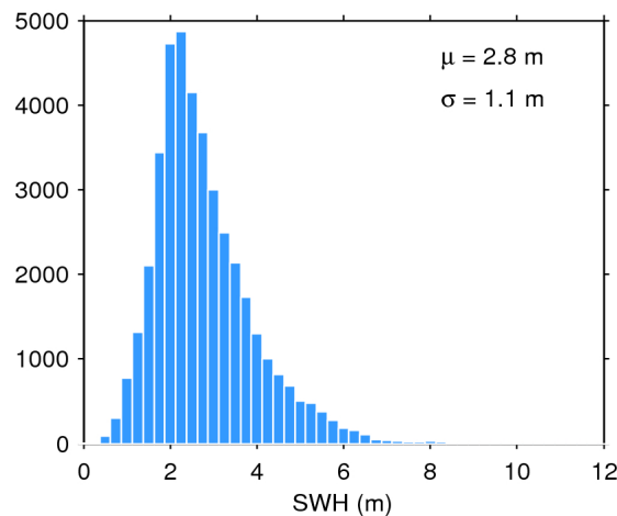
Figure 20. Histogram of science-valid SWH over oceans and lakes for 23/02/2019. The mean ( \mu ) and standard deviation ( \sigma ) are also shown. Note that values larger than 12 m are excluded from the histogram for the sake of readability but not from the computation of \mu and \sigma .
