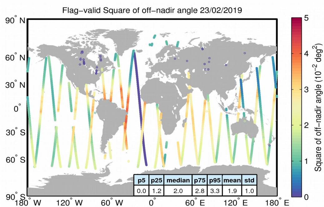
Figure 37. Geographical distribution of flag-valid mispointing data over oceans and lakes for 23/02/2019. The statistical values shown in the table refer to the mispointing in 10^{-2} \text{deg}^2 and are calculated over all measurements shown in the figure.
