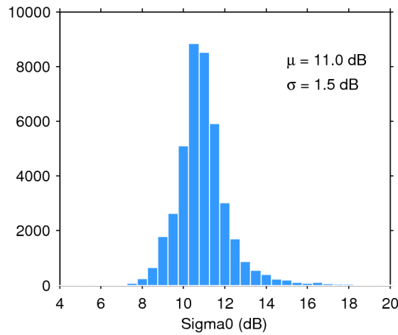
Figure 28. Histogram of science-valid sigma0 over oceans and lakes for 22/02/2019. The mean ( \mu ) and standard deviation ( \sigma ) are also shown. Note that values outside [4 20] dB are excluded from the histogram for the sake of readability but not from the computation of \mu and \sigma .
