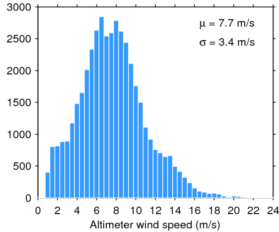
Figure 33. Histogram of flag-valid wind over oceans and lakes for 22/02/2019. The mean ( \mu ) and standard deviation ( \sigma ) are also shown. Note that values larger than 24 m/s are excluded from the histogram for the sake of readability but not from the computation of \mu and \sigma .
