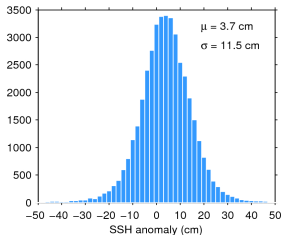
Figure 11. Histogram of science-valid SSH anomaly over oceans and lakes for 22/02/2019. The mean ( \mu ) and standard deviation ( \sigma ) are also shown. Note that values outside [-50 50] cm are excluded from the histogram for the sake of readability but not from the computation of \mu and \sigma .
