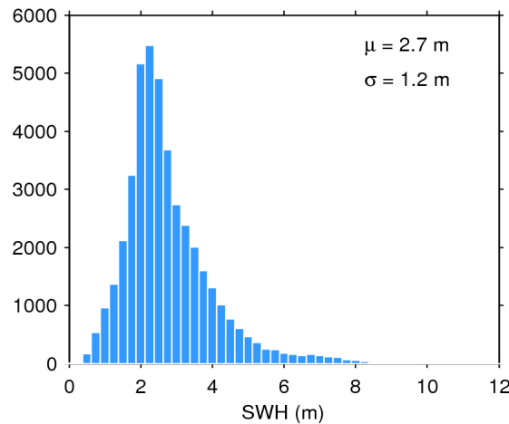
Figure 20. Histogram of science-valid SWH over oceans and lakes for 22/02/2019. The mean ( \mu ) and standard deviation ( \sigma ) are also shown. Note that values larger than 12 m are excluded from the histogram for the sake of readability but not from the computation of \mu and \sigma .
