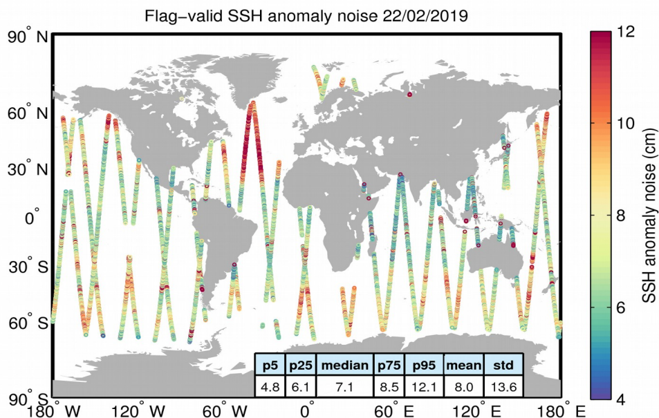
Figure 8. Geographical distribution of flag-valid 20-Hz SSH anomaly measurement noise over oceans and lakes for 22/02/2019. The statistical values shown in the table refer to the SSH anomaly noise and are calculated over all measurements shown in the figure.
