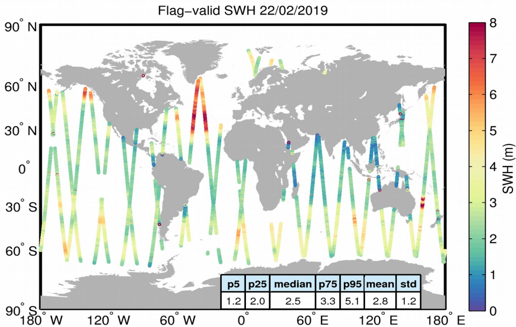
Figure 15. Geographical distribution of flag-valid SWH data over oceans and lakes for 22/02/2019. The statistical values shown in the table refer to the SWH in m and are calculated over all measurements shown in the figure.
