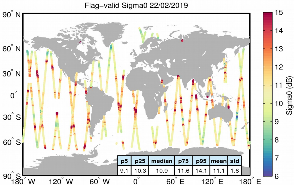
Figure 23. Geographical distribution of flag-valid sigma0 data over oceans and lakes for 22/02/2019. The statistical values shown in the table refer to the sigma0 in dB and are calculated over all measurements shown in the figure.
