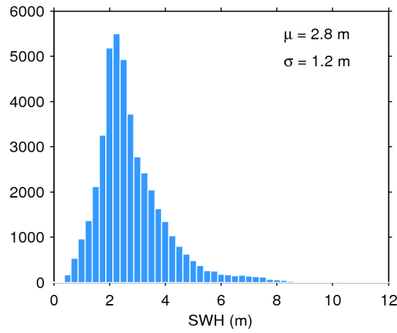
Figure 17. Histogram of flag-valid SWH over oceans and lakes for 22/02/2019. The mean ( \mu ) and standard deviation ( \sigma ) are also shown. Note that values larger than 12 m are excluded from the histogram for the sake of readability but not from the computation of \mu and \sigma .
