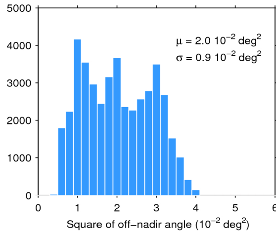
Figure 39. Histogram of flag-valid mispointing over oceans and lakes for 22/02/2019. The mean ( \mu ) and standard deviation ( \sigma ) are also shown. Note that values larger than 6 \cdot 10^{-2} \text{ deg}^2 are excluded from the histogram for the sake of readability but not from the computation of \mu and \sigma .
