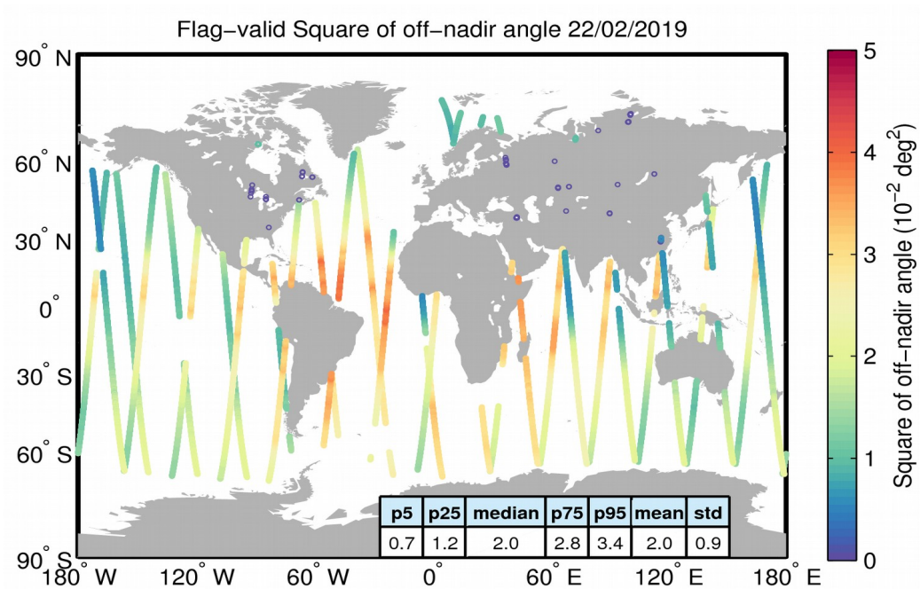
Figure 37. Geographical distribution of flag-valid mispointing data over oceans and lakes for 22/02/2019. The statistical values shown in the table refer to the mispointing in 10^{-2} \text{ deg}^2 and are calculated over all measurements shown in the figure.
