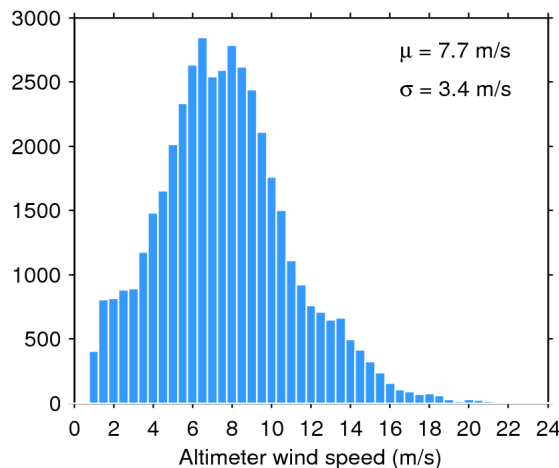
Figure 35. Histogram of science-valid wind over oceans and lakes for 22/02/2019. The mean ( \mu ) and standard deviation ( \sigma ) are also shown. Note that values larger than 24 m/s are excluded from the histogram for the sake of readability but not from the computation of \mu and \sigma .
