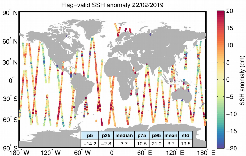
Figure 5. Geographical distribution of flag-valid 1-Hz SSH anomaly data over oceans and lakes for 22/02/2019. The statistical values shown in the table refer to the SSH anomaly in cm and are calculated over all measurements shown in the figure.
