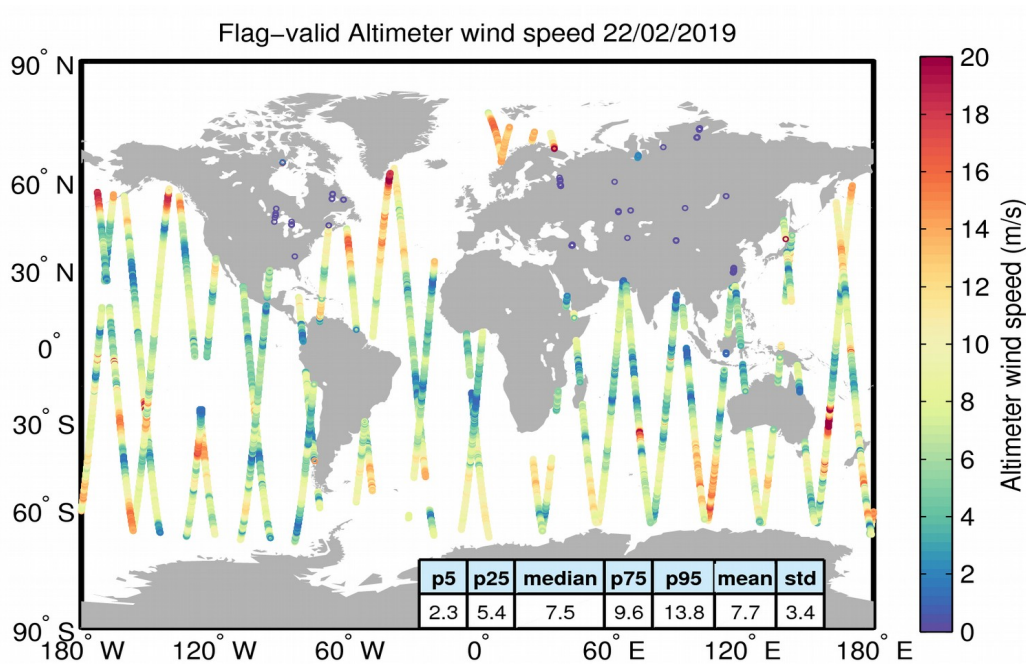
Figure 31. Geographical distribution of flag-valid wind data over oceans and lakes for 22/02/2019. The statistical values shown in the table refer to the wind in m/s and are calculated over all measurements shown in the figure.
