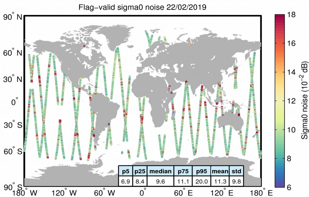
Figure 26. Geographical distribution of flag-valid 20-Hz sigma0 measurement noise over oceans and lakes for 22/02/2019. The statistical values shown in the table refer to the sigma0 noise and are calculated over all measurements shown in the figure.
