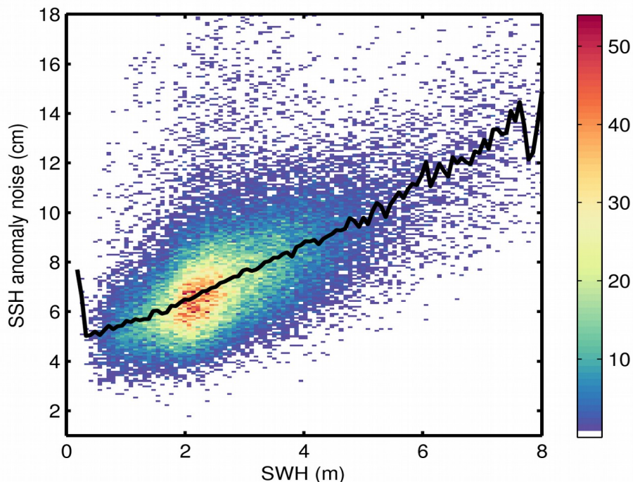
Figure 9. 2D histogram showing flag-valid SSH anomaly noise as a function of SWH for 22/02/2019. The black line denotes the median SSH anomaly noise as a function of SWH.
