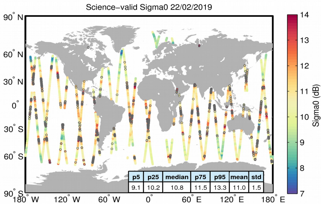
Figure 27. Geographical distribution of science-valid sigma0 data over oceans and lakes for 22/02/2019. The statistical values shown in the table refer to the sigma0 in dB and are calculated over all measurements shown in the figure. Gray circles denote records that have been rejected based on the editing criteria described in Table 4.
