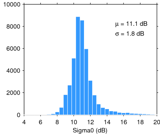
Figure 25. Histogram of flag-valid sigma0 over oceans and lakes for 22/02/2019. The mean ( \mu ) and standard deviation ( \sigma ) are also shown. Note that values outside [4 20] dB are excluded from the histogram for the sake of readability but not from the computation of \mu and \sigma .
