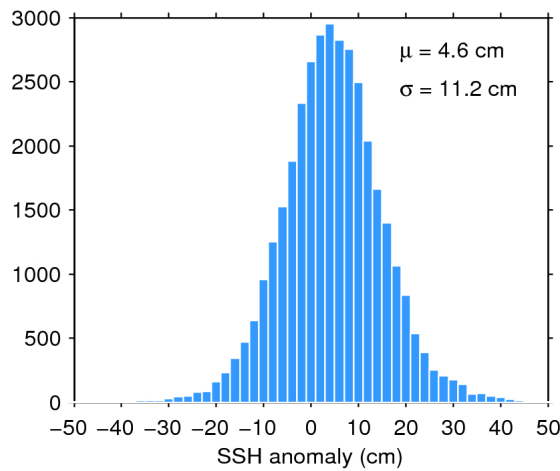
Figure 11. Histogram of science-valid SSH anomaly over oceans and lakes for 21/02/2019. The mean ( \mu ) and standard deviation ( \sigma ) are also shown. Note that values outside [-50 50] cm are excluded from the histogram for the sake of readability but not from the computation of \mu and \sigma .
