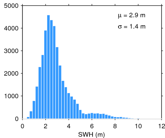
Figure 20. Histogram of science-valid SWH over oceans and lakes for 21/02/2019. The mean ( \mu ) and standard deviation ( \sigma ) are also shown. Note that values larger than 12 m are excluded from the histogram for the sake of readability but not from the computation of \mu and \sigma .
