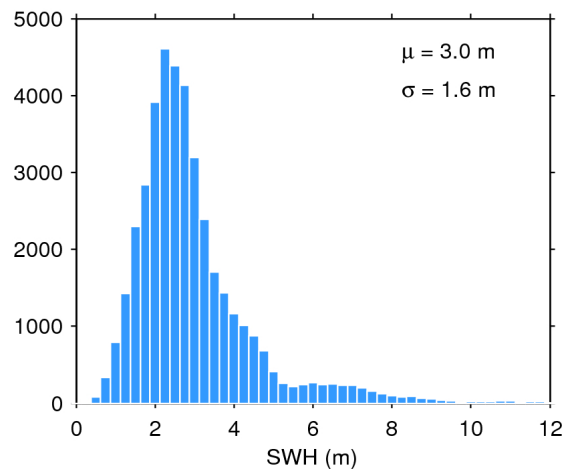
Figure 17. Histogram of flag-valid SWH over oceans and lakes for 21/02/2019. The mean ( \mu ) and standard deviation ( \sigma ) are also shown. Note that values larger than 12 m are excluded from the histogram for the sake of readability but not from the computation of \mu and \sigma .
