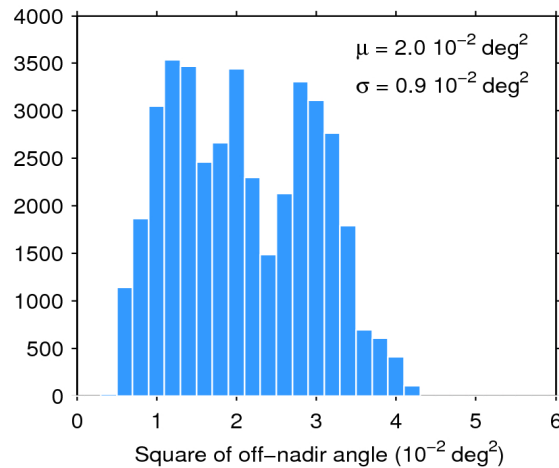
Figure 39. Histogram of flag-valid mispointing over oceans and lakes for 21/02/2019. The mean ( \mu ) and standard deviation ( \sigma ) are also shown. Note that values larger than 6 \cdot 10^{-2} \text{ deg}^2 are excluded from the histogram for the sake of readability but not from the computation of \mu and \sigma .
