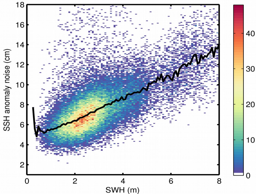
Figure 9. 2D histogram showing flag-valid SSH anomaly noise as a function of SWH for 21/02/2019. The black line denotes the median SSH anomaly noise as a function of SWH.
