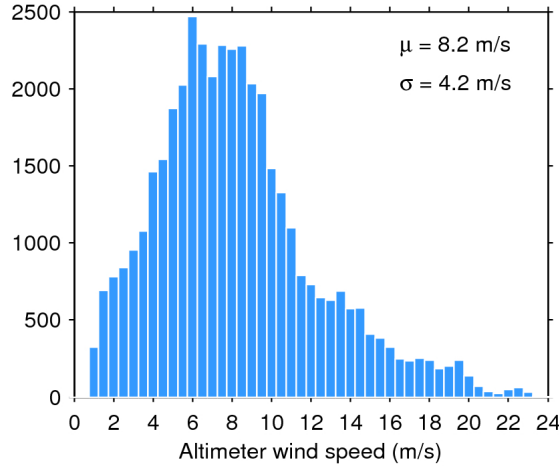
Figure 33. Histogram of flag-valid wind over oceans and lakes for 21/02/2019. The mean ( \mu ) and standard deviation ( \sigma ) are also shown. Note that values larger than 24 m/s are excluded from the histogram for the sake of readability but not from the computation of \mu and \sigma .
