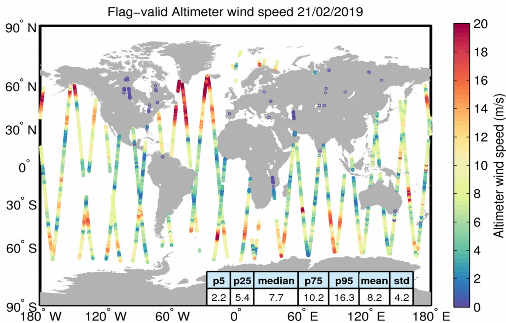
Figure 31. Geographical distribution of flag-valid wind data over oceans and lakes for 21/02/2019. The statistical values shown in the table refer to the wind in m/s and are calculated over all measurements shown in the figure.
