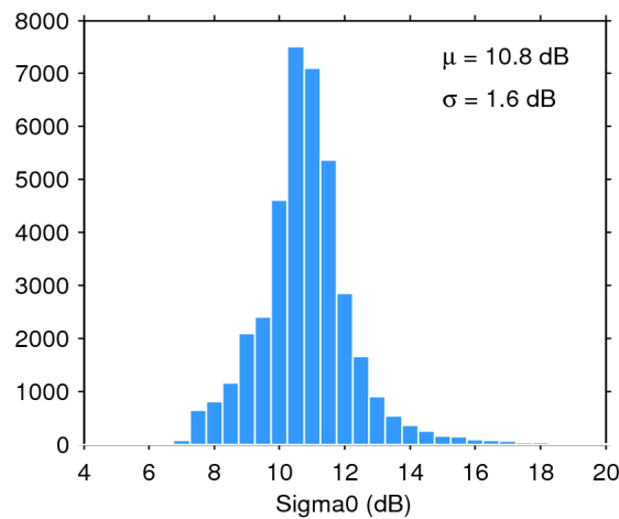
Figure 28. Histogram of science-valid sigma0 over oceans and lakes for 21/02/2019. The mean ( \mu ) and standard deviation ( \sigma ) are also shown. Note that values outside [4 20] dB are excluded from the histogram for the sake of readability but not from the computation of \mu and \sigma .
