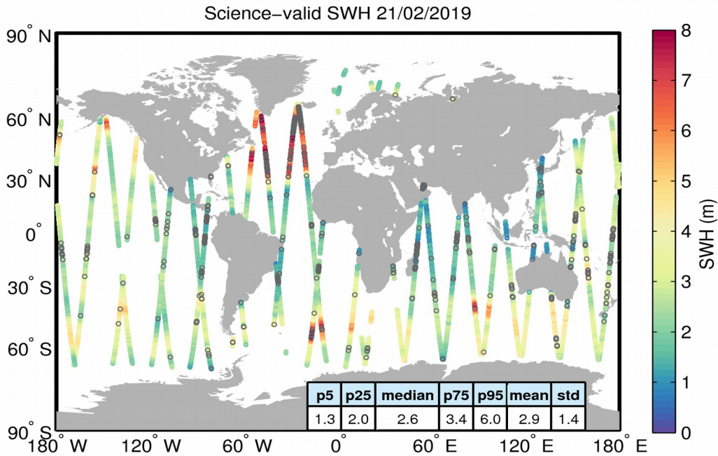
Figure 19. Geographical distribution of science-valid SWH data over oceans and lakes for 21/02/2019. The statistical values shown in the table refer to the SWH in m and are calculated over all measurements shown in the figure. Gray circles denote records that have been rejected based on the editing criteria described in Table 3.
