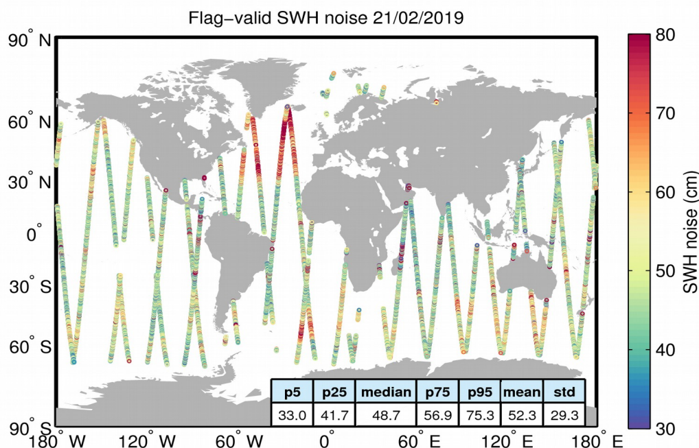
Figure 18. Geographical distribution of flag-valid 20-Hz SWH measurement noise over oceans and lakes for 21/02/2019. The statistical values shown in the figure refer to the SWH noise and are calculated over all measurements shown in the figure.
