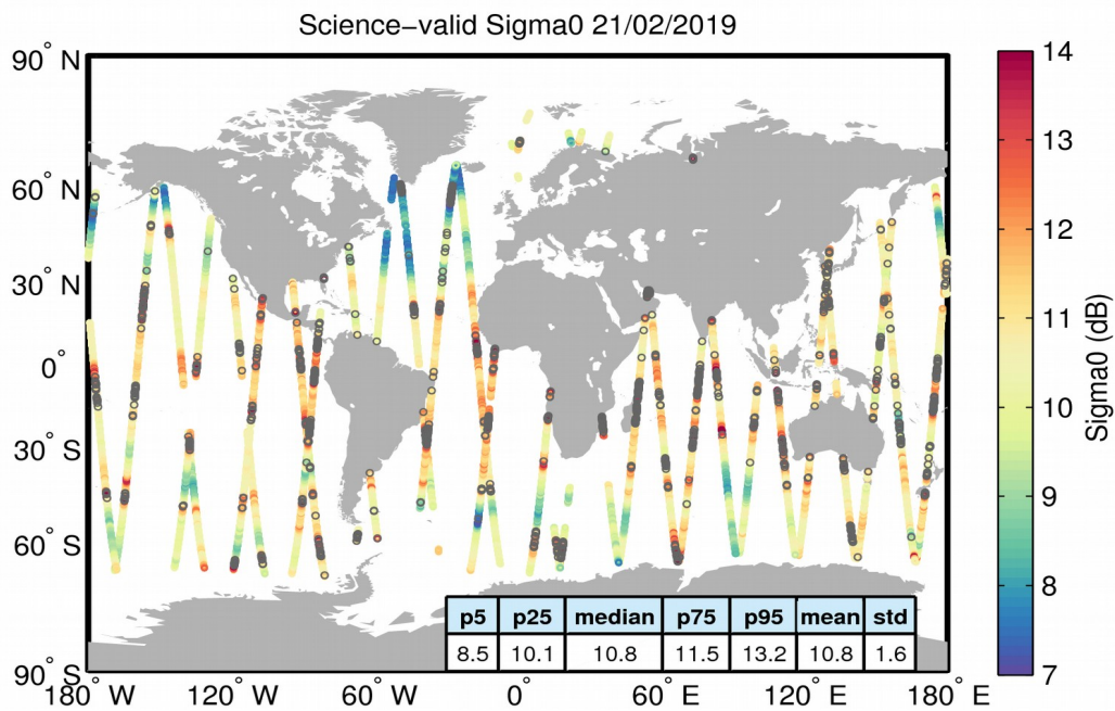
Figure 27. Geographical distribution of science-valid sigma0 data over oceans and lakes for 21/02/2019. The statistical values shown in the table refer to the sigma0 in dB and are calculated over all measurements shown in the figure. Gray circles denote records that have been rejected based on the editing criteria described in Table 4.
