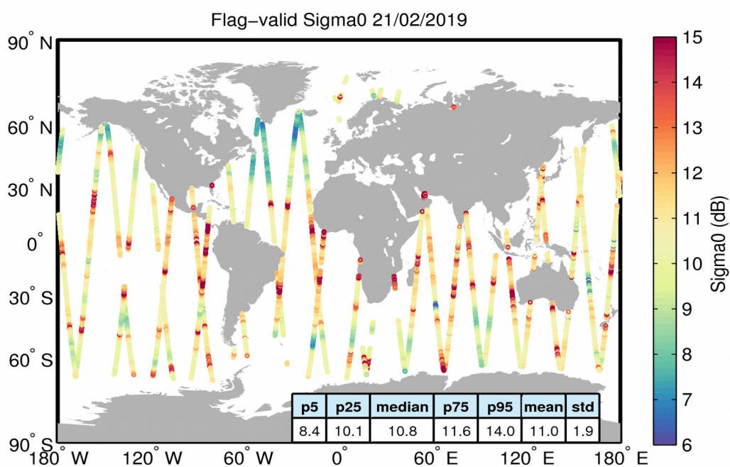
Figure 23. Geographical distribution of flag-valid sigma0 data over oceans and lakes for 21/02/2019. The statistical values shown in the table refer to the sigma0 in dB and are calculated over all measurements shown in the figure.
