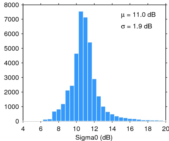
Figure 25. Histogram of flag-valid sigma0 over oceans and lakes for 21/02/2019. The mean ( \mu ) and standard deviation ( \sigma ) are also shown. Note that values outside [4 20] dB are excluded from the histogram for the sake of readability but not from the computation of \mu and \sigma .
