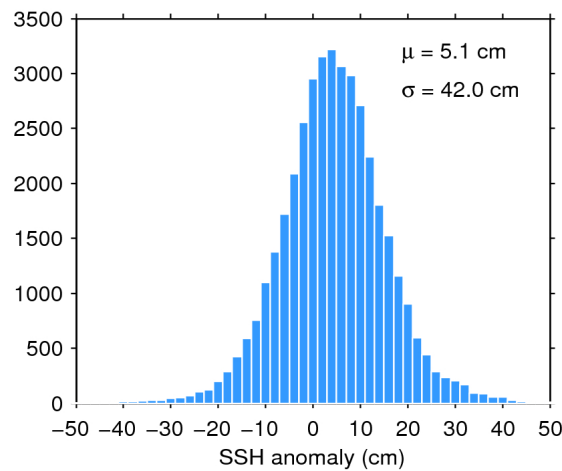
Figure 7. Histogram of flag-valid SSH anomaly over oceans and lakes for 21/02/2019. The mean ( \mu ) and standard deviation ( \sigma ) are also shown. Note that values outside [-50\ 50] cm are excluded from the histogram for the sake of readability but not from the computation of \mu and \sigma .
