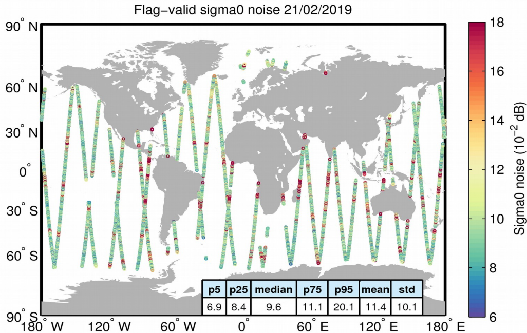
Figure 26. Geographical distribution of flag-valid 20-Hz sigma0 measurement noise over oceans and lakes for 21/02/2019. The statistical values shown in the table refer to the sigma0 noise and are calculated over all measurements shown in the figure.
