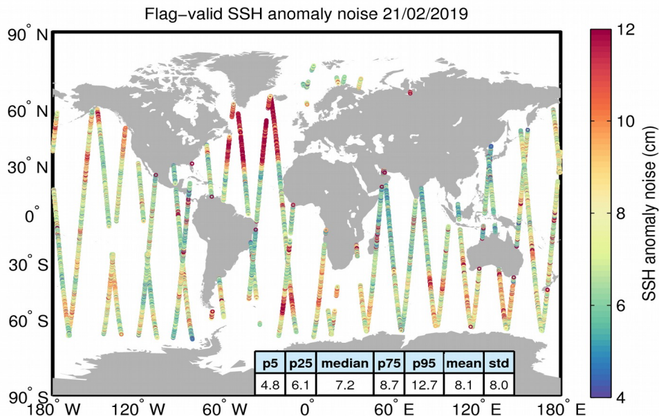
Figure 8. Geographical distribution of flag-valid 20-Hz SSH anomaly measurement noise over oceans and lakes for 21/02/2019. The statistical values shown in the table refer to the SSH anomaly noise and are calculated over all measurements shown in the figure.
