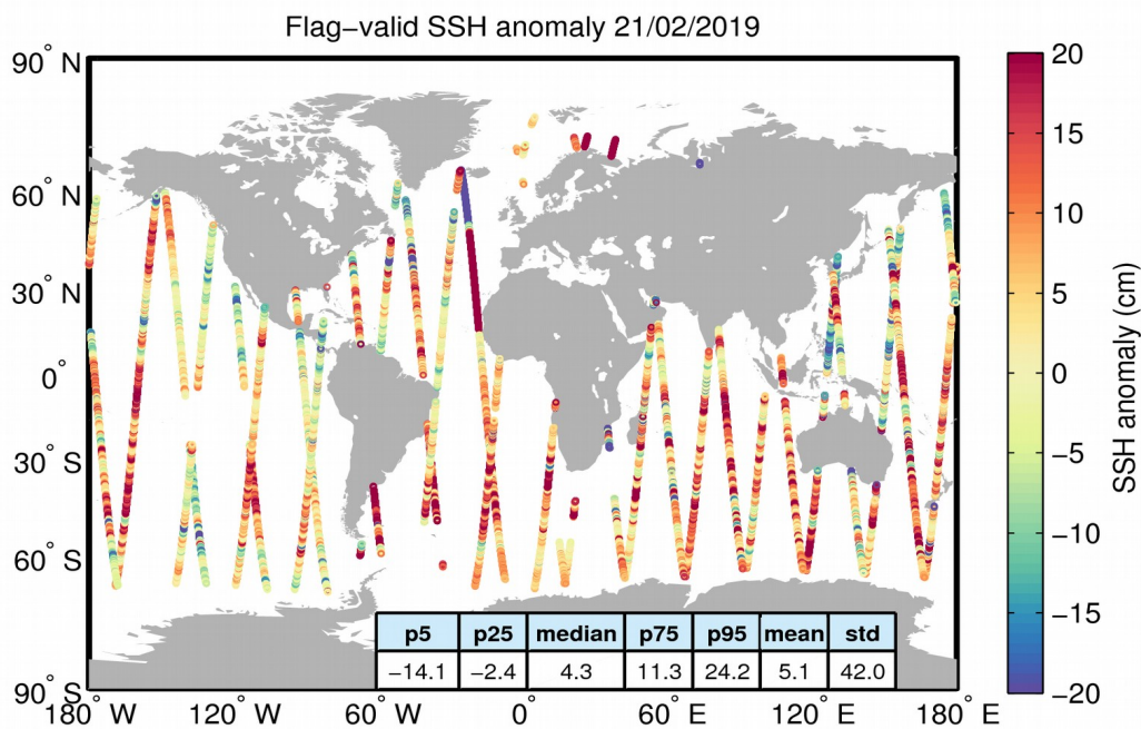
Figure 5. Geographical distribution of flag-valid 1-Hz SSH anomaly data over oceans and lakes for 21/02/2019. The statistical values shown in the table refer to the SSH anomaly in cm and are calculated over all measurements shown in the figure.
