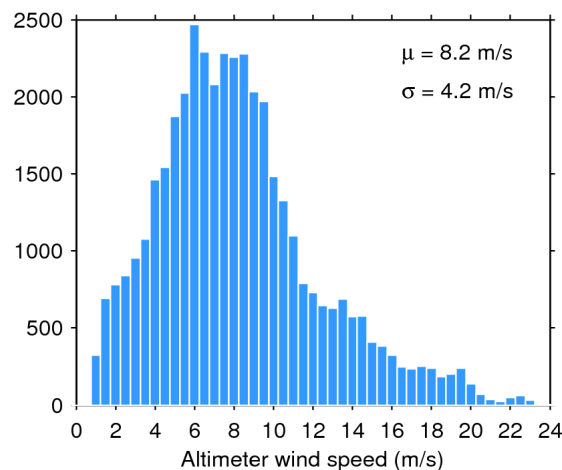
Figure 35. Histogram of science-valid wind over oceans and lakes for 21/02/2019. The mean ( \mu ) and standard deviation ( \sigma ) are also shown. Note that values larger than 24 m/s are excluded from the histogram for the sake of readability but not from the computation of \mu and \sigma .
