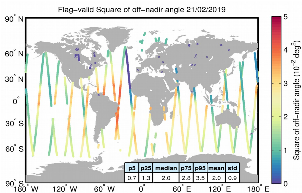
Figure 37. Geographical distribution of flag-valid mispointing data over oceans and lakes for 21/02/2019. The statistical values shown in the table refer to the mispointing in 10^{-2} deg 2 and are calculated over all measurements shown in the figure.
