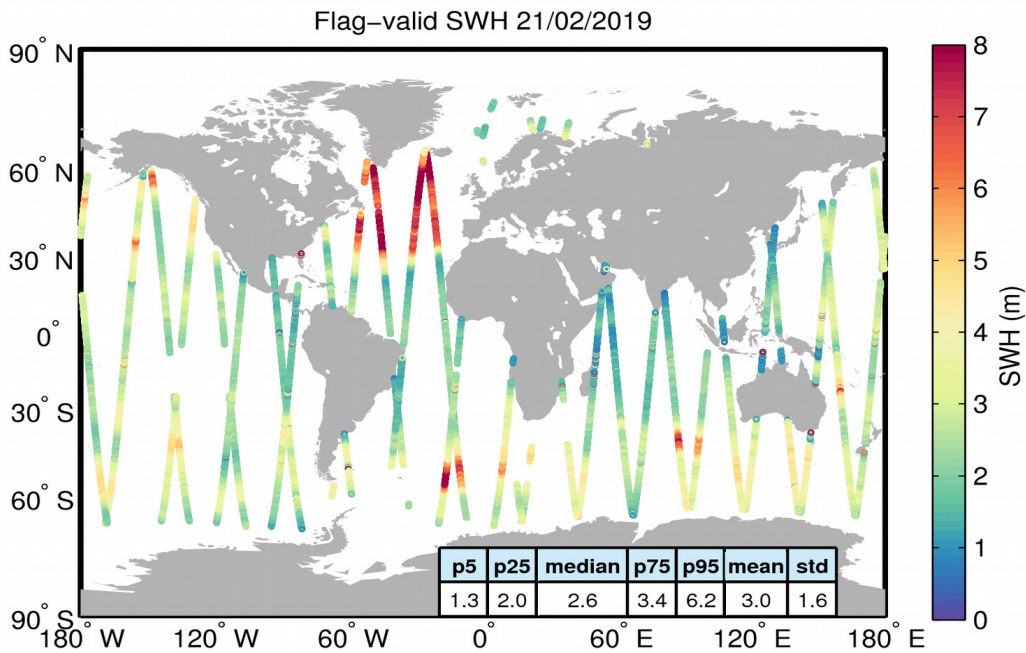
Figure 15. Geographical distribution of flag-valid SWH data over oceans and lakes for 21/02/2019. The statistical values shown in the table refer to the SWH in m and are calculated over all measurements shown in the figure.
