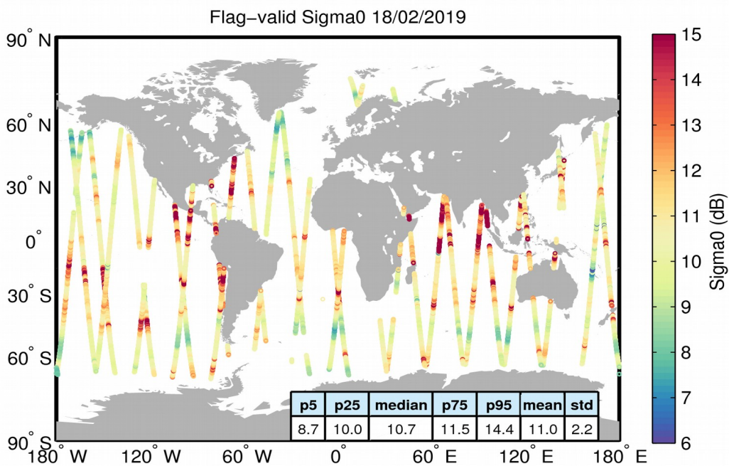
Figure 23. Geographical distribution of flag-valid sigma0 data over oceans and lakes for 18/02/2019. The statistical values shown in the table refer to the sigma0 in dB and are calculated over all measurements shown in the figure.
