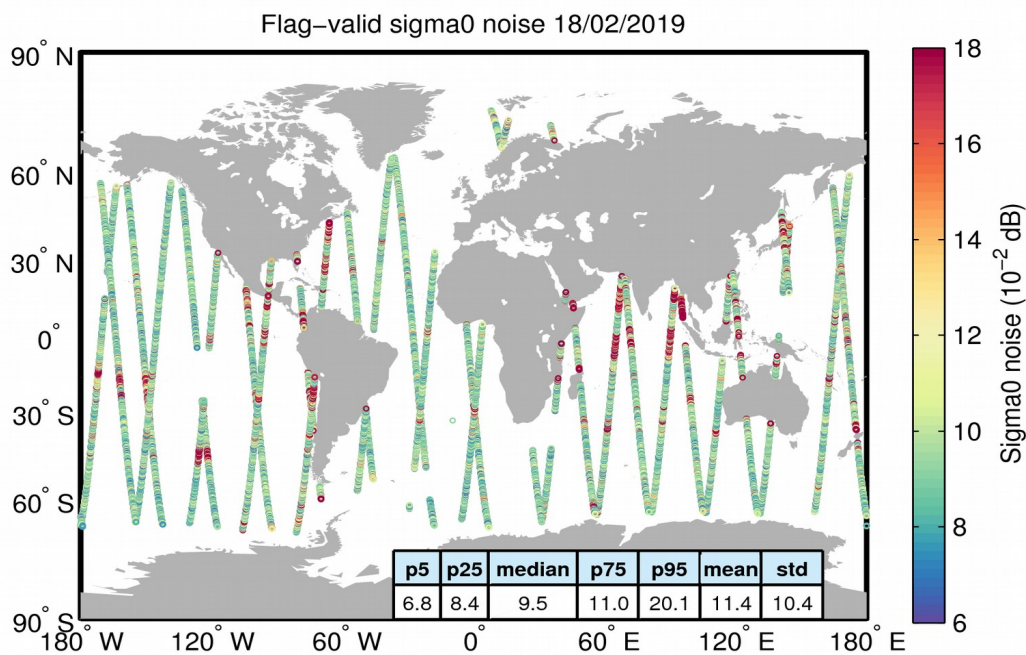
Figure 26. Geographical distribution of flag-valid 20-Hz sigma0 measurement noise over oceans and lakes for 18/02/2019. The statistical values shown in the table refer to the sigma0 noise and are calculated over all measurements shown in the figure.
