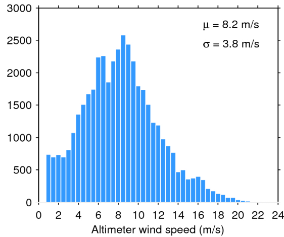
Figure 33. Histogram of flag-valid wind over oceans and lakes for 18/02/2019. The mean ( \mu ) and standard deviation ( \sigma ) are also shown. Note that values larger than 24 m/s are excluded from the histogram for the sake of readability but not from the computation of \mu and \sigma .
