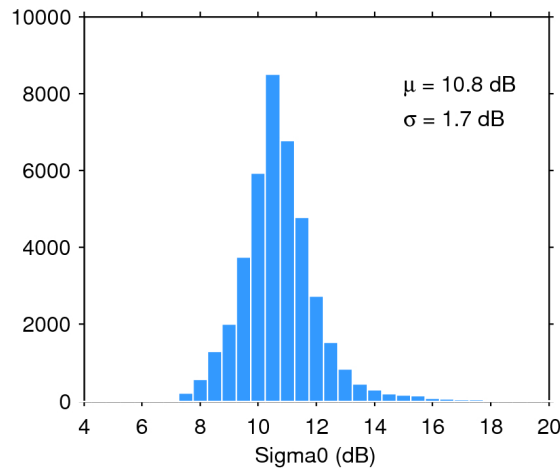
Figure 28. Histogram of science-valid sigma0 over oceans and lakes for 18/02/2019. The mean ( \mu ) and standard deviation ( \sigma ) are also shown. Note that values outside [4 20] dB are excluded from the histogram for the sake of readability but not from the computation of \mu and \sigma .
