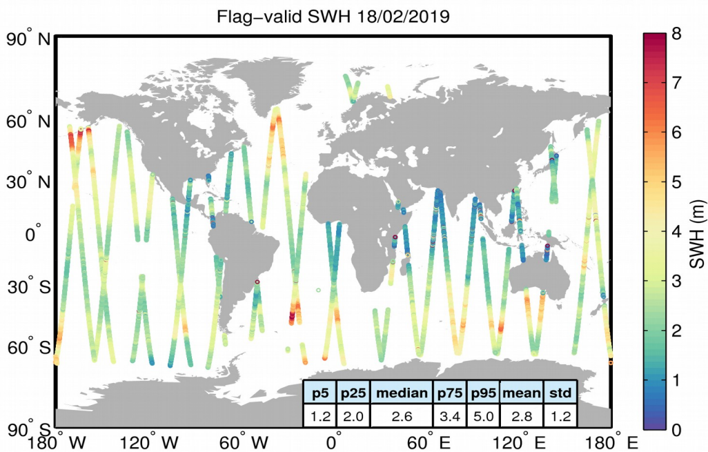
Figure 15. Geographical distribution of flag-valid SWH data over oceans and lakes for 18/02/2019. The statistical values shown in the table refer to the SWH in m and are calculated over all measurements shown in the figure.
