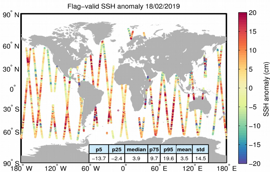
Figure 5. Geographical distribution of flag-valid 1-Hz SSH anomaly data over oceans and lakes for 18/02/2019. The statistical values shown in the table refer to the SSH anomaly in cm and are calculated over all measurements shown in the figure.
