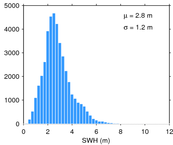
Figure 17. Histogram of flag-valid SWH over oceans and lakes for 18/02/2019. The mean ( \mu ) and standard deviation ( \sigma ) are also shown. Note that values larger than 12 m are excluded from the histogram for the sake of readability but not from the computation of \mu and \sigma .
