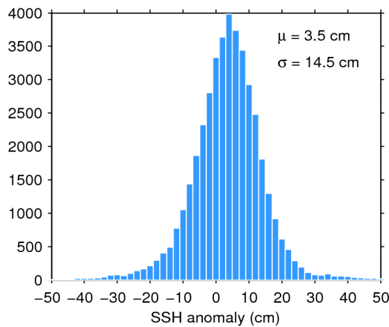
Figure 7. Histogram of flag-valid SSH anomaly over oceans and lakes for 18/02/2019. The mean ( \mu ) and standard deviation ( \sigma ) are also shown. Note that values outside [-50 50] cm are excluded from the histogram for the sake of readability but not from the computation of \mu and \sigma .
