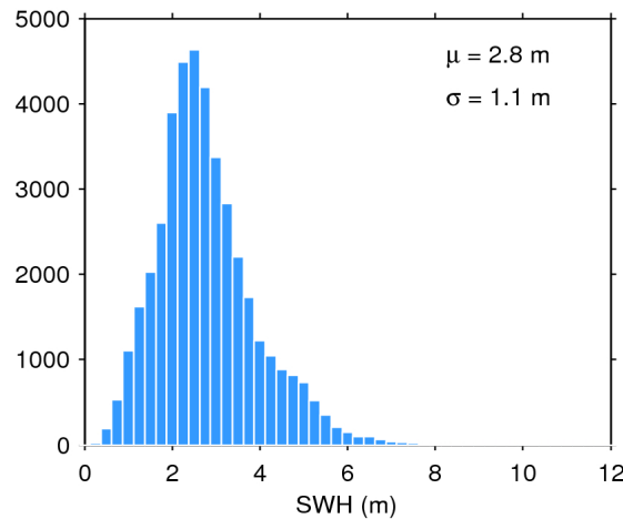
Figure 20. Histogram of science-valid SWH over oceans and lakes for 18/02/2019. The mean ( \mu ) and standard deviation ( \sigma ) are also shown. Note that values larger than 12 m are excluded from the histogram for the sake of readability but not from the computation of \mu and \sigma .
