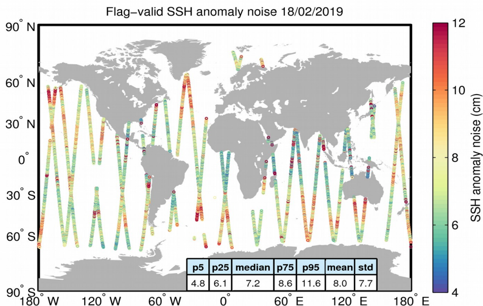
Figure 8. Geographical distribution of flag-valid 20-Hz SSH anomaly measurement noise over oceans and lakes for 18/02/2019. The statistical values shown in the table refer to the SSH anomaly noise and are calculated over all measurements shown in the figure.
