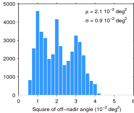
Figure 39. Histogram of flag-valid mispointing over oceans and lakes for 18/02/2019. The mean ( \mu ) and standard deviation ( \sigma ) are also shown. Note that values larger than 6 \cdot 10^{-2} \text{ deg}^2 are excluded from the histogram for the sake of readability but not from the computation of \mu and \sigma .
