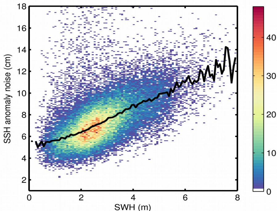
Figure 9. 2D histogram showing flag-valid SSH anomaly noise as a function of SWH for 18/02/2019. The black line denotes the median SSH anomaly noise as a function of SWH.
