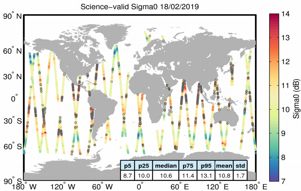
Figure 27. Geographical distribution of science-valid sigma0 data over oceans and lakes for 18/02/2019. The statistical values shown in the table refer to the sigma0 in dB and are calculated over all measurements shown in the figure. Gray circles denote records that have been rejected based on the editing criteria described in Table 4.
