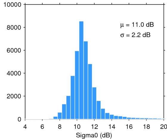
Figure 25. Histogram of flag-valid sigma0 over oceans and lakes for 18/02/2019. The mean ( \mu ) and standard deviation ( \sigma ) are also shown. Note that values outside [4 20] dB are excluded from the histogram for the sake of readability but not from the computation of \mu and \sigma .
