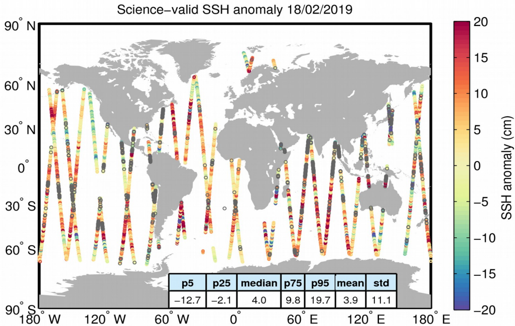
Figure 10. Geographical distribution of science-valid SSH anomaly data over oceans and lakes for 18/02/2019. The statistical values shown in the table refer to the SSH anomaly in cm and are calculated over all measurements shown in the figure. Gray circles denote records that have been rejected based on the editing criteria described in Table 2.
