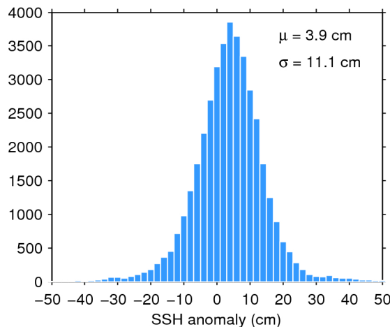
Figure 11. Histogram of science-valid SSH anomaly over oceans and lakes for 18/02/2019. The mean ( \mu ) and standard deviation ( \sigma ) are also shown. Note that values outside [-50 50] cm are excluded from the histogram for the sake of readability but not from the computation of \mu and \sigma .
