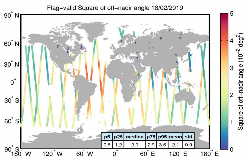
Figure 37. Geographical distribution of flag-valid mispointing data over oceans and lakes for 18/02/2019. The statistical values shown in the table refer to the mispointing in 10^{-2} \text{ deg}^2 and are calculated over all measurements shown in the figure.
