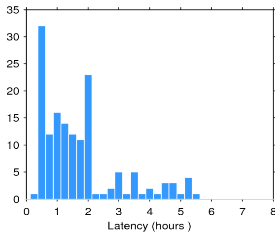
Figure 2. Histogram of the data latency for 18/02/2019. The y-axis denotes the number of files that are made available with a delay of x-hours with respect to the mean time of the records stored in the file.
