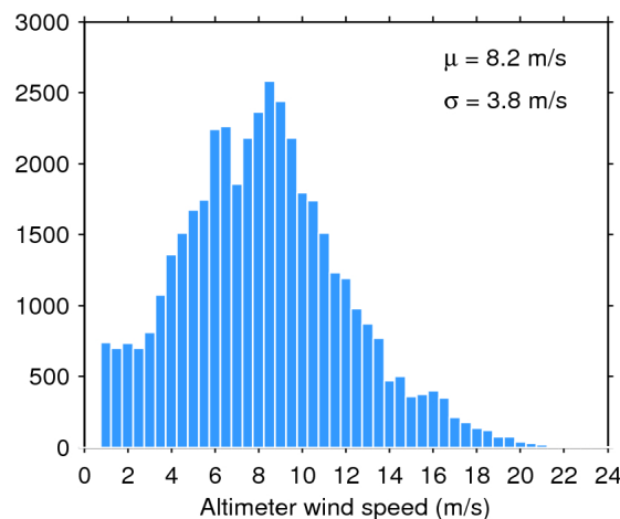
Figure 35. Histogram of science-valid wind over oceans and lakes for 18/02/2019. The mean ( \mu ) and standard deviation ( \sigma ) are also shown. Note that values larger than 24 m/s are excluded from the histogram for the sake of readability but not from the computation of \mu and \sigma .
