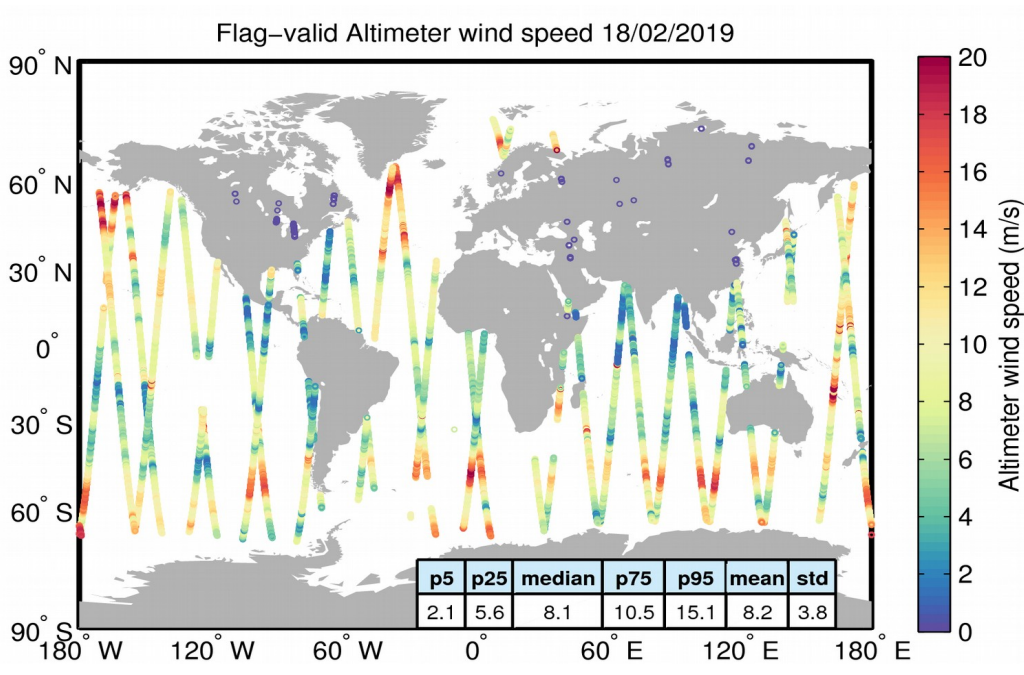
Figure 31. Geographical distribution of flag-valid wind data over oceans and lakes for 18/02/2019. The statistical values shown in the table refer to the wind in m/s and are calculated over all measurements shown in the figure.
