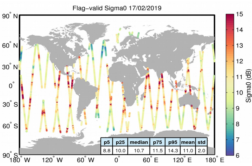
Figure 23. Geographical distribution of flag-valid sigma0 data over oceans and lakes for 17/02/2019. The statistical values shown in the table refer to the sigma0 in dB and are calculated over all measurements shown in the figure.
