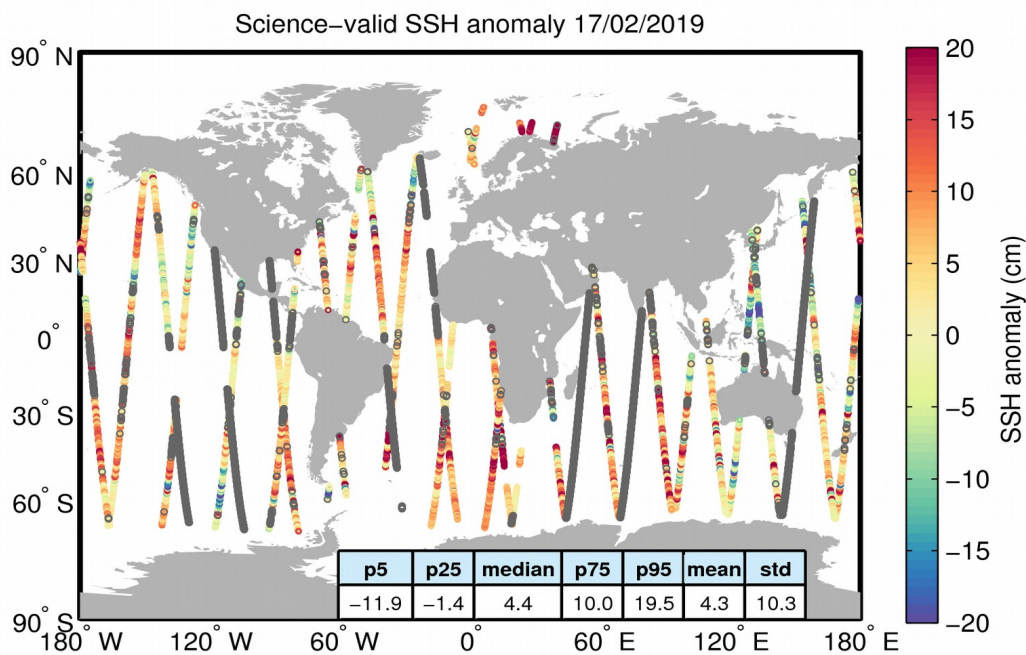
Figure 10. Geographical distribution of science-valid SSH anomaly data over oceans and lakes for 17/02/2019. The statistical values shown in the table refer to the SSH anomaly in cm and are calculated over all measurements shown in the figure. Gray circles denote records that have been rejected based on the editing criteria described in Table 2.
