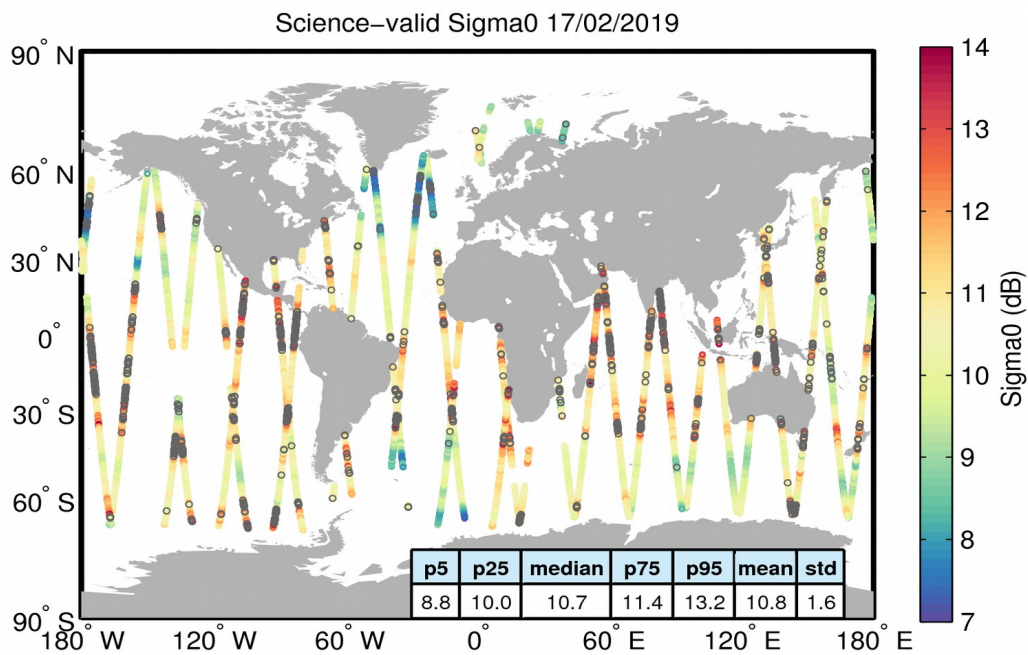
Figure 27. Geographical distribution of science-valid sigma0 data over oceans and lakes for 17/02/2019. The statistical values shown in the table refer to the sigma0 in dB and are calculated over all measurements shown in the figure. Gray circles denote records that have been rejected based on the editing criteria described in Table 4.
