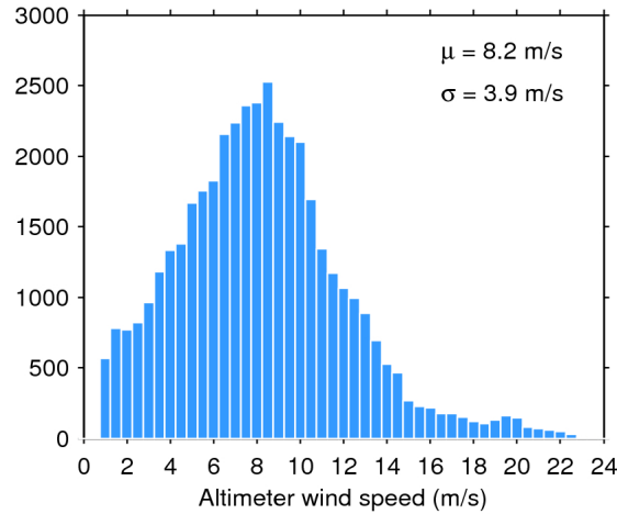
Figure 33. Histogram of flag-valid wind over oceans and lakes for 17/02/2019. The mean ( \mu ) and standard deviation ( \sigma ) are also shown. Note that values larger than 24 m/s are excluded from the histogram for the sake of readability but not from the computation of \mu and \sigma .
