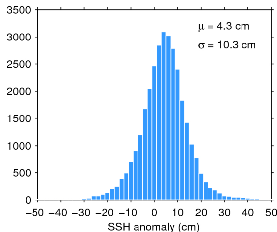
Figure 11. Histogram of science-valid SSH anomaly over oceans and lakes for 17/02/2019. The mean ( \mu ) and standard deviation ( \sigma ) are also shown. Note that values outside [-50 50] cm are excluded from the histogram for the sake of readability but not from the computation of \mu and \sigma .
