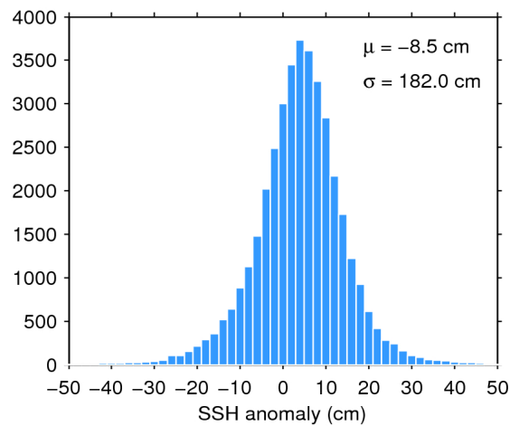
Figure 7. Histogram of flag-valid SSH anomaly over oceans and lakes for 17/02/2019. The mean ( \mu ) and standard deviation ( \sigma ) are also shown. Note that values outside [-50 50] cm are excluded from the histogram for the sake of readability but not from the computation of \mu and \sigma .
