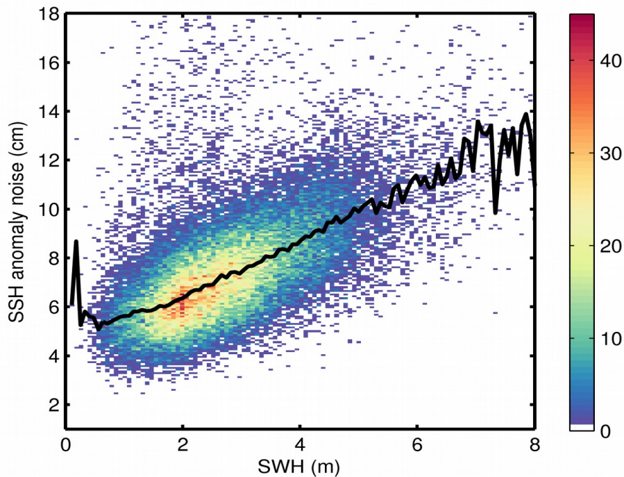
Figure 9. 2D histogram showing flag-valid SSH anomaly noise as a function of SWH for 17/02/2019. The black line denotes the median SSH anomaly noise as a function of SWH.
