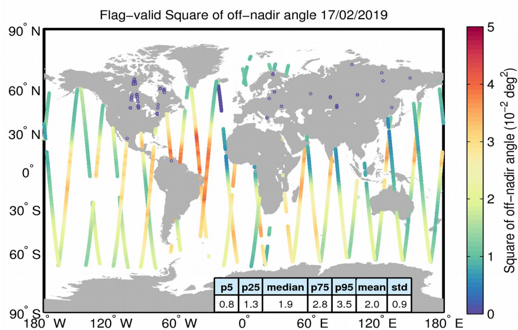
Figure 37. Geographical distribution of flag-valid mispointing data over oceans and lakes for 17/02/2019. The statistical values shown in the table refer to the mispointing in 10^{-2} deg 2 and are calculated over all measurements shown in the figure.
