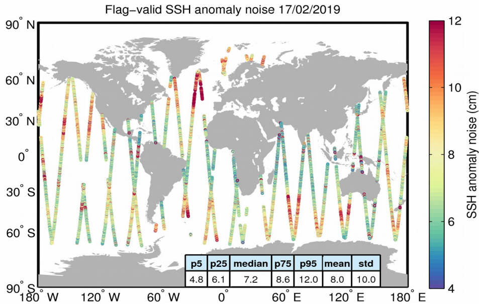
Figure 8. Geographical distribution of flag-valid 20-Hz SSH anomaly measurement noise over oceans and lakes for 17/02/2019. The statistical values shown in the table refer to the SSH anomaly noise and are calculated over all measurements shown in the figure.
