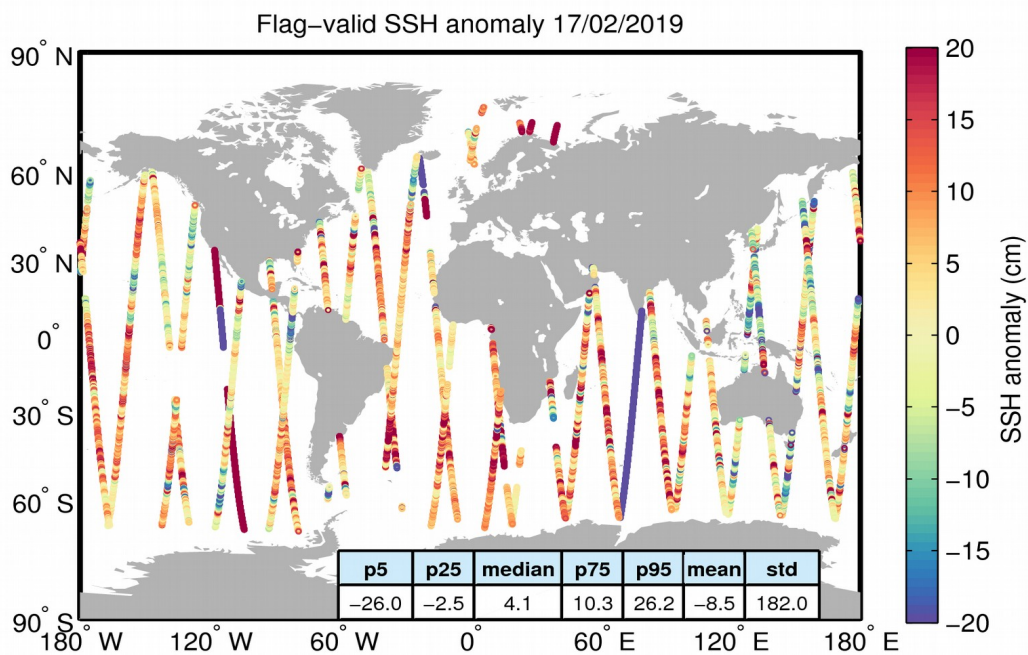
Figure 5. Geographical distribution of flag-valid 1-Hz SSH anomaly data over oceans and lakes for 17/02/2019. The statistical values shown in the table refer to the SSH anomaly in cm and are calculated over all measurements shown in the figure.
