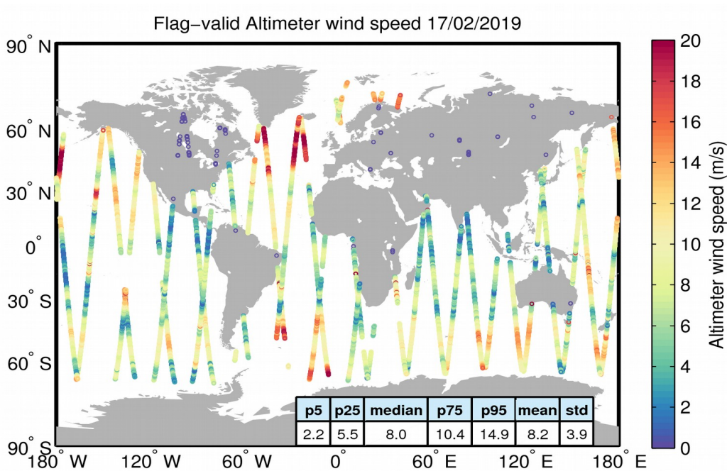
Figure 31. Geographical distribution of flag-valid wind data over oceans and lakes for 17/02/2019. The statistical values shown in the table refer to the wind in m/s and are calculated over all measurements shown in the figure.
