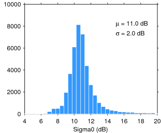
Figure 25. Histogram of flag-valid sigma0 over oceans and lakes for 17/02/2019. The mean ( \mu ) and standard deviation ( \sigma ) are also shown. Note that values outside [4 20] dB are excluded from the histogram for the sake of readability but not from the computation of \mu and \sigma .
