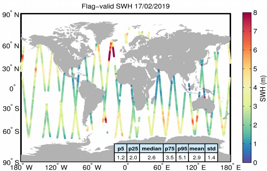
Figure 15. Geographical distribution of flag-valid SWH data over oceans and lakes for 17/02/2019. The statistical values shown in the table refer to the SWH in m and are calculated over all measurements shown in the figure.
