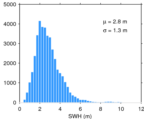
Figure 20. Histogram of science-valid SWH over oceans and lakes for 17/02/2019. The mean ( \mu ) and standard deviation ( \sigma ) are also shown. Note that values larger than 12 m are excluded from the histogram for the sake of readability but not from the computation of \mu and \sigma .
