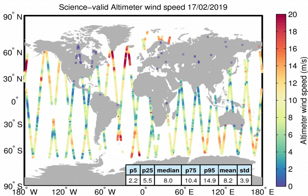
Figure 34. Geographical distribution of science-valid wind data over oceans and lakes for 17/02/2019. The statistical values shown in the table refer to the wind in m/s and are calculated over all measurements shown in the figure. Gray circles denote records that have been rejected based on the editing criteria described in Table 5.
