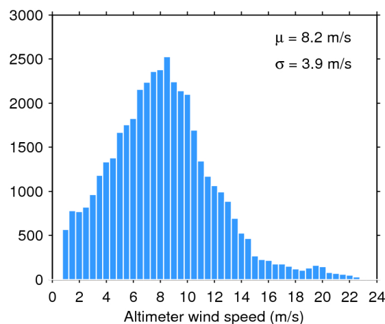
Figure 35. Histogram of science-valid wind over oceans and lakes for 17/02/2019. The mean ( \mu ) and standard deviation ( \sigma ) are also shown. Note that values larger than 24 m/s are excluded from the histogram for the sake of readability but not from the computation of \mu and \sigma .
