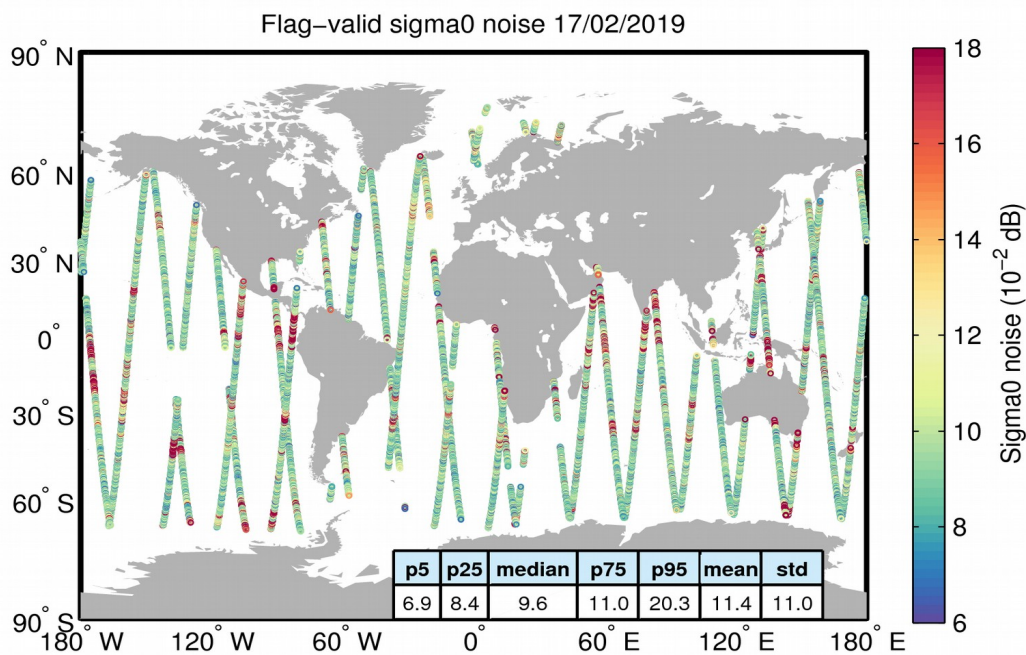
Figure 26. Geographical distribution of flag-valid 20-Hz sigma0 measurement noise over oceans and lakes for 17/02/2019. The statistical values shown in the table refer to the sigma0 noise and are calculated over all measurements shown in the figure.
