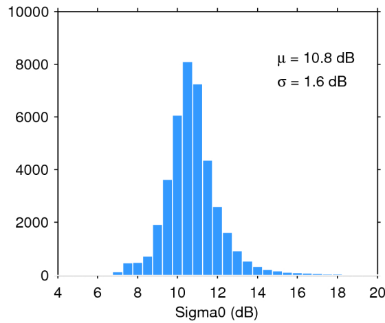
Figure 28. Histogram of science-valid sigma0 over oceans and lakes for 17/02/2019. The mean ( \mu ) and standard deviation ( \sigma ) are also shown. Note that values outside [4 20] dB are excluded from the histogram for the sake of readability but not from the computation of \mu and \sigma .
