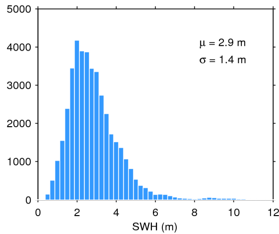
Figure 17. Histogram of flag-valid SWH over oceans and lakes for 17/02/2019. The mean ( \mu ) and standard deviation ( \sigma ) are also shown. Note that values larger than 12 m are excluded from the histogram for the sake of readability but not from the computation of \mu and \sigma .
