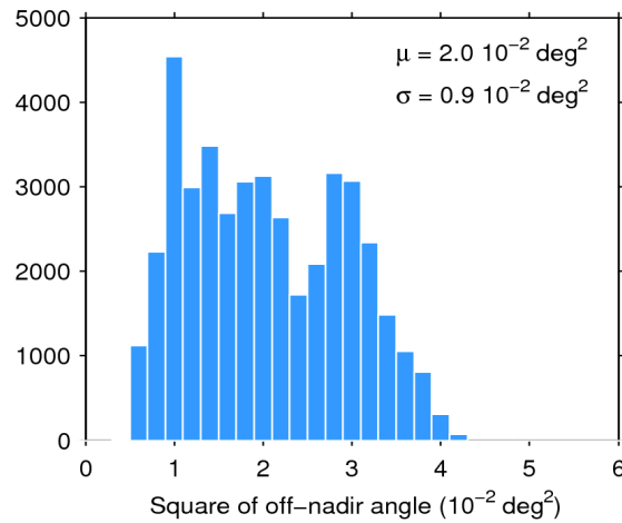
Figure 39. Histogram of flag-valid mispointing over oceans and lakes for 17/02/2019. The mean ( \mu ) and standard deviation ( \sigma ) are also shown. Note that values larger than 6 \cdot 10^{-2} \text{ deg}^2 are excluded from the histogram for the sake of readability but not from the computation of \mu and \sigma .
