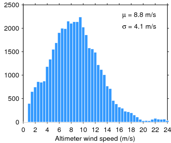
Figure 33. Histogram of flag-valid wind over oceans and lakes for 16/02/2019. The mean ( \mu ) and standard deviation ( \sigma ) are also shown. Note that values larger than 24 m/s are excluded from the histogram for the sake of readability but not from the computation of \mu and \sigma .
