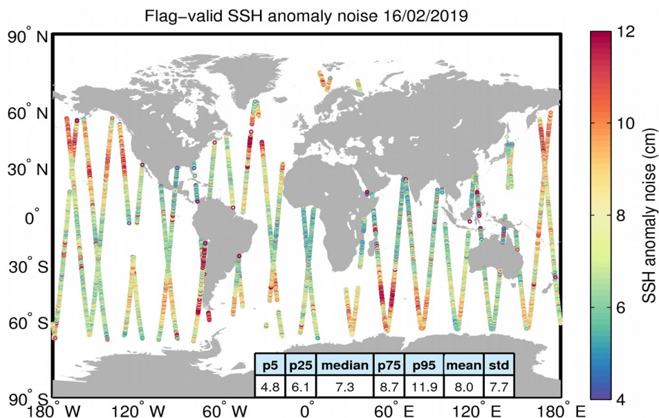
Figure 8. Geographical distribution of flag-valid 20-Hz SSH anomaly measurement noise over oceans and lakes for 16/02/2019. The statistical values shown in the table refer to the SSH anomaly noise and are calculated over all measurements shown in the figure.
