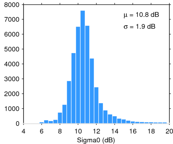
Figure 25. Histogram of flag-valid sigma0 over oceans and lakes for 16/02/2019. The mean ( \mu ) and standard deviation ( \sigma ) are also shown. Note that values outside [4 20] dB are excluded from the histogram for the sake of readability but not from the computation of \mu and \sigma .
