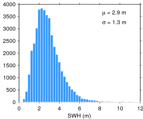
Figure 20. Histogram of science-valid SWH over oceans and lakes for 16/02/2019. The mean ( \mu ) and standard deviation ( \sigma ) are also shown. Note that values larger than 12 m are excluded from the histogram for the sake of readability but not from the computation of \mu and \sigma .
