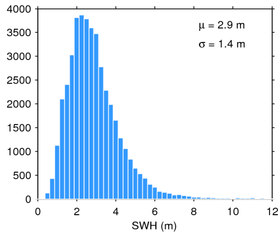
Figure 17. Histogram of flag-valid SWH over oceans and lakes for 16/02/2019. The mean ( \mu ) and standard deviation ( \sigma ) are also shown. Note that values larger than 12 m are excluded from the histogram for the sake of readability but not from the computation of \mu and \sigma .
