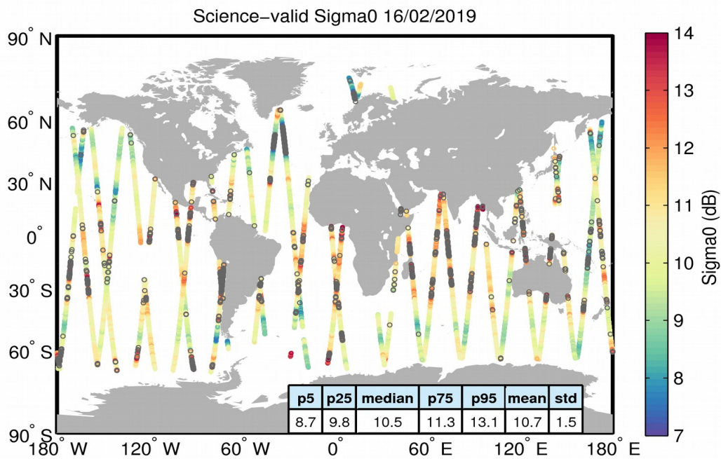
Figure 27. Geographical distribution of science-valid sigma0 data over oceans and lakes for 16/02/2019. The statistical values shown in the table refer to the sigma0 in dB and are calculated over all measurements shown in the figure. Gray circles denote records that have been rejected based on the editing criteria described in Table 4.
