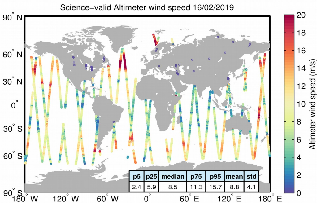
Figure 34. Geographical distribution of science-valid wind data over oceans and lakes for 16/02/2019. The statistical values shown in the table refer to the wind in m/s and are calculated over all measurements shown in the figure. Gray circles denote records that have been rejected based on the editing criteria described in Table 5.
