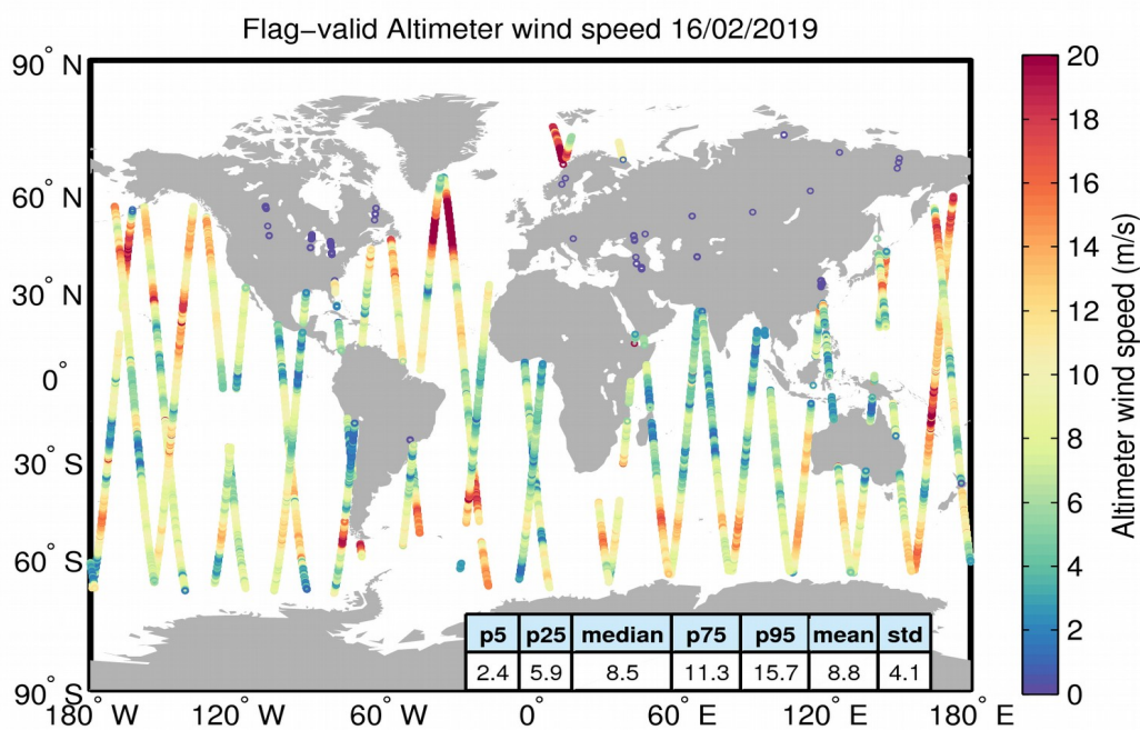
Figure 31. Geographical distribution of flag-valid wind data over oceans and lakes for 16/02/2019. The statistical values shown in the table refer to the wind in m/s and are calculated over all measurements shown in the figure.
