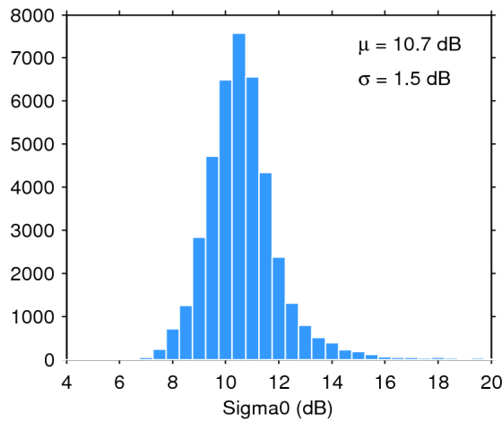
Figure 28. Histogram of science-valid sigma0 over oceans and lakes for 16/02/2019. The mean ( \mu ) and standard deviation ( \sigma ) are also shown. Note that values outside [4 20] dB are excluded from the histogram for the sake of readability but not from the computation of \mu and \sigma .
