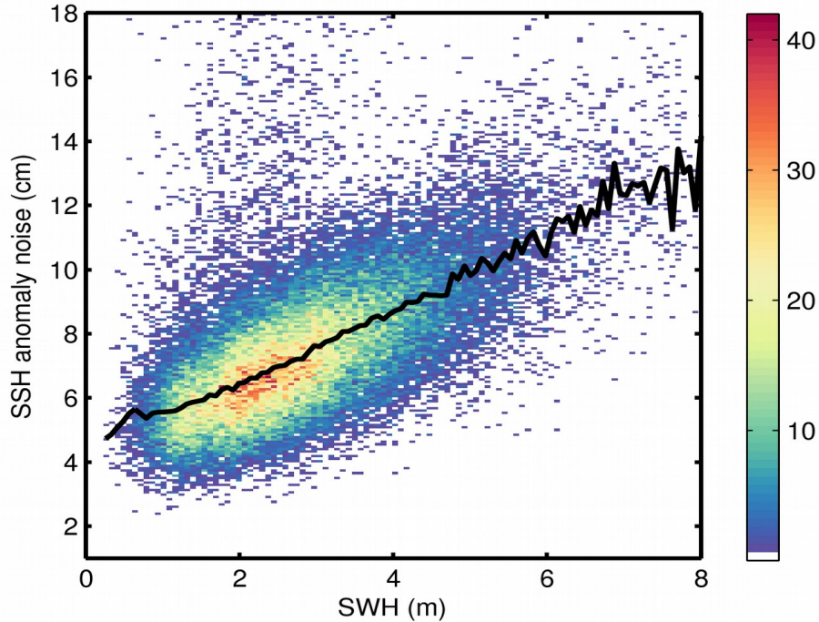
Figure 9. 2D histogram showing flag-valid SSH anomaly noise as a function of SWH for 16/02/2019. The black line denotes the median SSH anomaly noise as a function of SWH.
