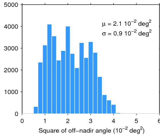
Figure 39. Histogram of flag-valid mispointing over oceans and lakes for 16/02/2019. The mean ( \mu ) and standard deviation ( \sigma ) are also shown. Note that values larger than 6 \cdot 10^{-2} \text{ deg}^2 are excluded from the histogram for the sake of readability but not from the computation of \mu and \sigma .
