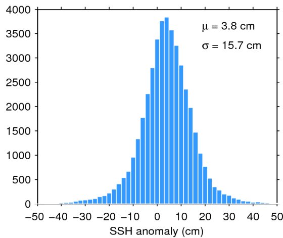
Figure 7. Histogram of flag-valid SSH anomaly over oceans and lakes for 16/02/2019. The mean ( \mu ) and standard deviation ( \sigma ) are also shown. Note that values outside [-50\ 50] cm are excluded from the histogram for the sake of readability but not from the computation of \mu and \sigma .
