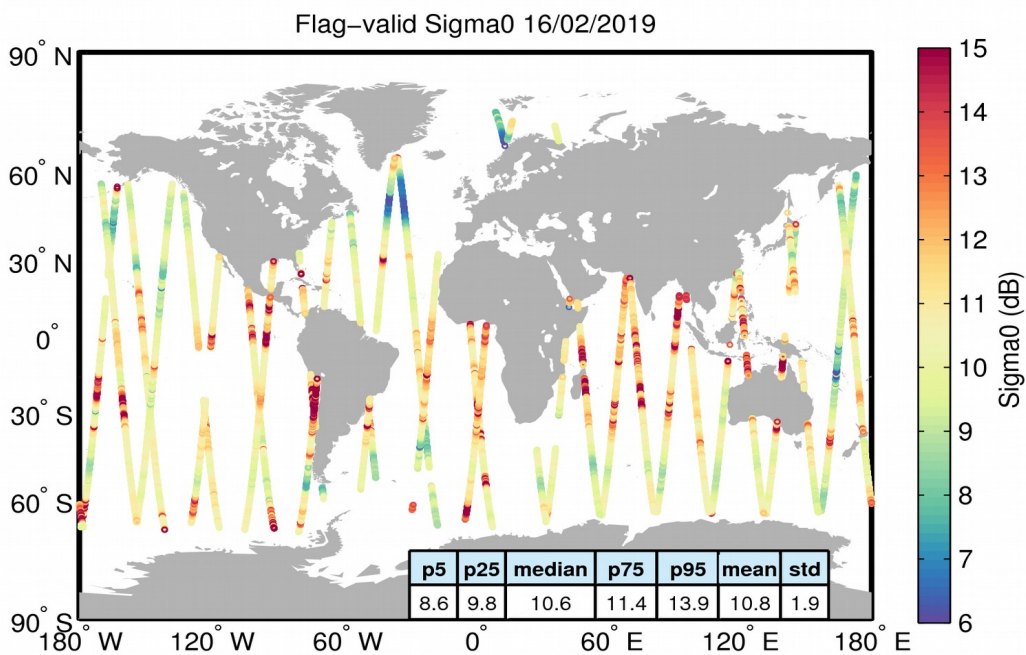
Figure 23. Geographical distribution of flag-valid sigma0 data over oceans and lakes for 16/02/2019. The statistical values shown in the table refer to the sigma0 in dB and are calculated over all measurements shown in the figure.
