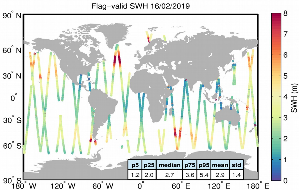
Figure 15. Geographical distribution of flag-valid SWH data over oceans and lakes for 16/02/2019. The statistical values shown in the table refer to the SWH in m and are calculated over all measurements shown in the figure.
