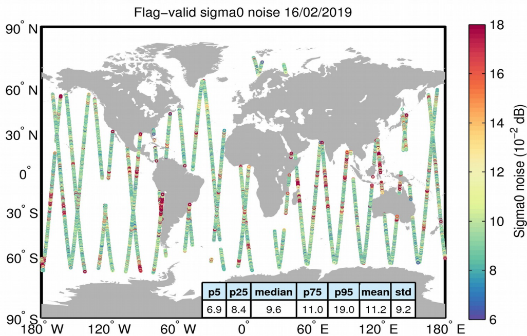
Figure 26. Geographical distribution of flag-valid 20-Hz sigma0 measurement noise over oceans and lakes for 16/02/2019. The statistical values shown in the table refer to the sigma0 noise and are calculated over all measurements shown in the figure.
