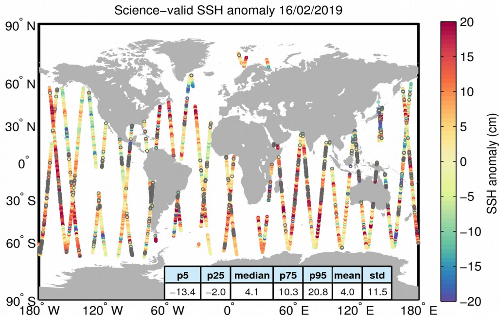
Figure 10. Geographical distribution of science-valid SSH anomaly data over oceans and lakes for 16/02/2019. The statistical values shown in the table refer to the SSH anomaly in cm and are calculated over all measurements shown in the figure. Gray circles denote records that have been rejected based on the editing criteria described in Table 2.
