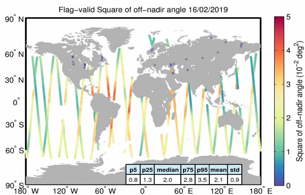
Figure 37. Geographical distribution of flag-valid mispointing data over oceans and lakes for 16/02/2019. The statistical values shown in the table refer to the mispointing in 10^{-2} \text{ deg}^2 and are calculated over all measurements shown in the figure.
