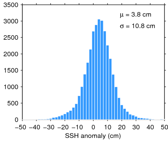
Figure 11. Histogram of science-valid SSH anomaly over oceans and lakes for 15/02/2019. The mean ( \mu ) and standard deviation ( \sigma ) are also shown. Note that values outside [-50 50] cm are excluded from the histogram for the sake of readability but not from the computation of \mu and \sigma .
