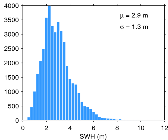
Figure 20. Histogram of science-valid SWH over oceans and lakes for 15/02/2019. The mean ( \mu ) and standard deviation ( \sigma ) are also shown. Note that values larger than 12 m are excluded from the histogram for the sake of readability but not from the computation of \mu and \sigma .
