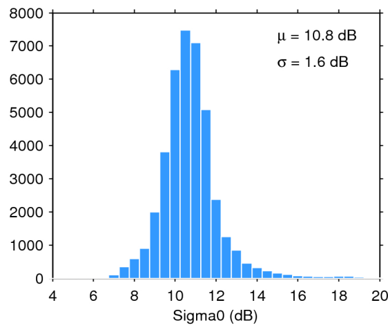
Figure 28. Histogram of science-valid sigma0 over oceans and lakes for 15/02/2019. The mean ( \mu ) and standard deviation ( \sigma ) are also shown. Note that values outside [4 20] dB are excluded from the histogram for the sake of readability but not from the computation of \mu and \sigma .
