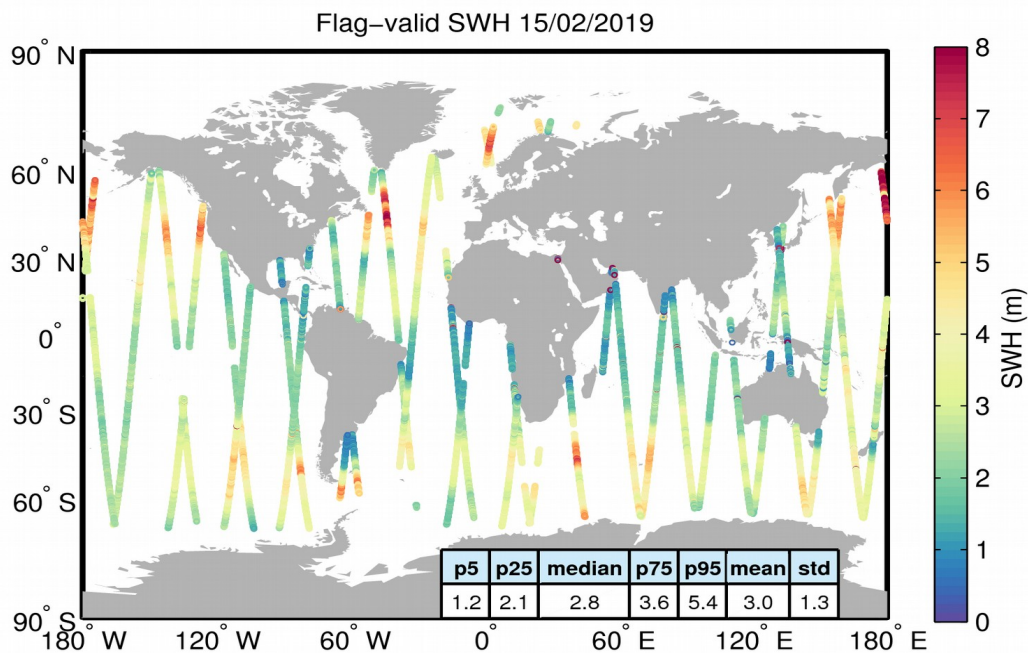
Figure 15. Geographical distribution of flag-valid SWH data over oceans and lakes for 15/02/2019. The statistical values shown in the table refer to the SWH in m and are calculated over all measurements shown in the figure.
