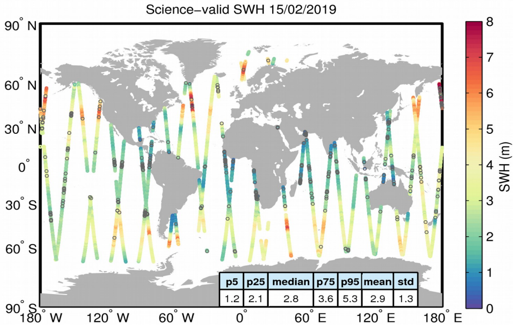
Figure 19. Geographical distribution of science-valid SWH data over oceans and lakes for 15/02/2019. The statistical values shown in the table refer to the SWH in m and are calculated over all measurements shown in the figure. Gray circles denote records that have been rejected based on the editing criteria described in Table 3.
