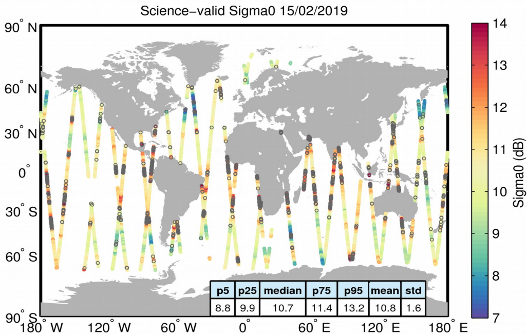
Figure 27. Geographical distribution of science-valid sigma0 data over oceans and lakes for 15/02/2019. The statistical values shown in the table refer to the sigma0 in dB and are calculated over all measurements shown in the figure. Gray circles denote records that have been rejected based on the editing criteria described in Table 4.
