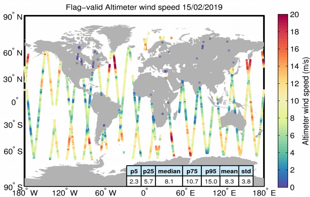
Figure 31. Geographical distribution of flag-valid wind data over oceans and lakes for 15/02/2019. The statistical values shown in the table refer to the wind in m/s and are calculated over all measurements shown in the figure.
