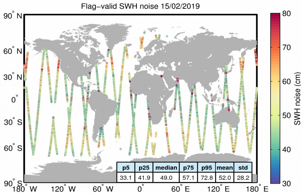
Figure 18. Geographical distribution of flag-valid 20-Hz SWH measurement noise over oceans and lakes for 15/02/2019. The statistical values shown in the figure refer to the SWH noise and are calculated over all measurements shown in the figure.
