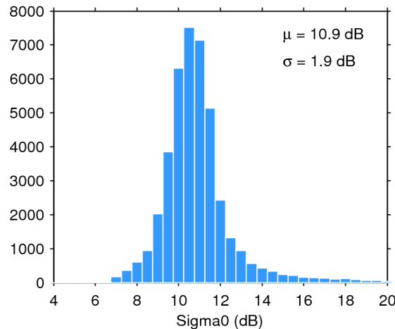
Figure 25. Histogram of flag-valid sigma0 over oceans and lakes for 15/02/2019. The mean ( \mu ) and standard deviation ( \sigma ) are also shown. Note that values outside [4 20] dB are excluded from the histogram for the sake of readability but not from the computation of \mu and \sigma .
