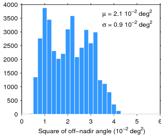
Figure 39. Histogram of flag-valid mispointing over oceans and lakes for 15/02/2019. The mean ( \mu ) and standard deviation ( \sigma ) are also shown. Note that values larger than 6 \cdot 10^{-2} \text{ deg}^2 are excluded from the histogram for the sake of readability but not from the computation of \mu and \sigma .
