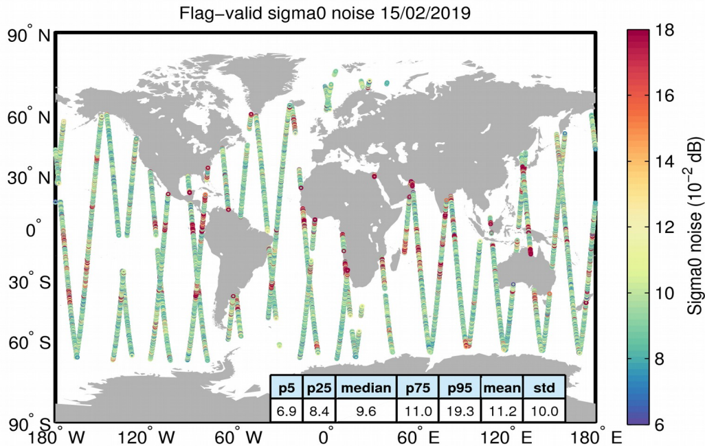
Figure 26. Geographical distribution of flag-valid 20-Hz sigma0 measurement noise over oceans and lakes for 15/02/2019. The statistical values shown in the table refer to the sigma0 noise and are calculated over all measurements shown in the figure.
