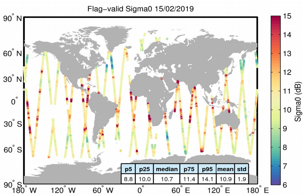
Figure 23. Geographical distribution of flag-valid sigma0 data over oceans and lakes for 15/02/2019. The statistical values shown in the table refer to the sigma0 in dB and are calculated over all measurements shown in the figure.
