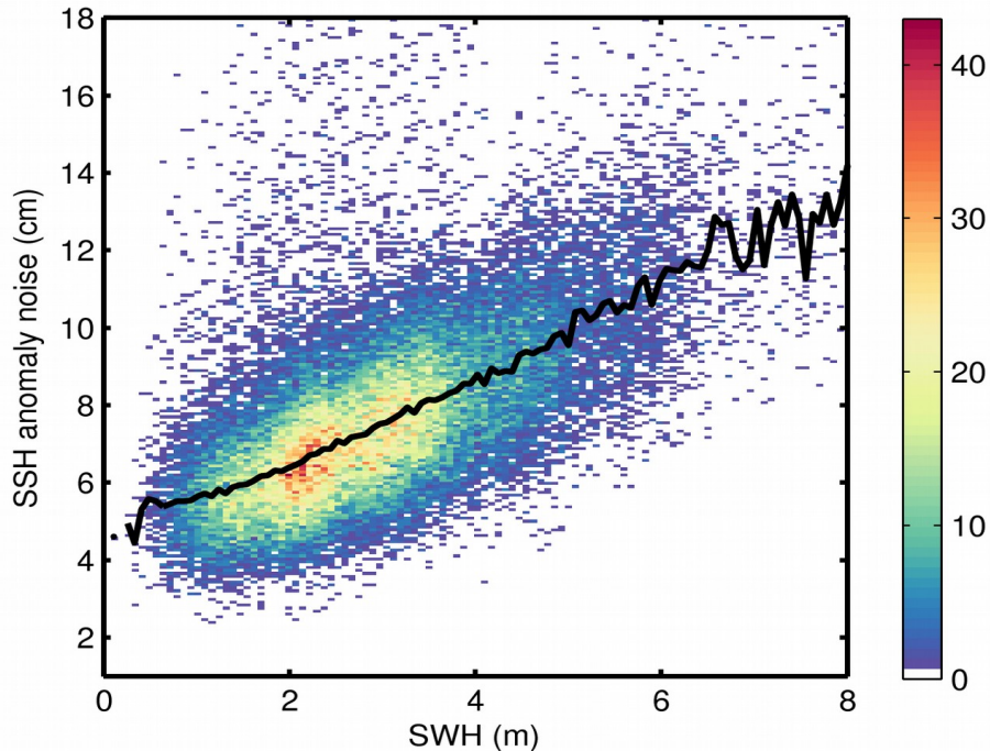
Figure 9. 2D histogram showing flag-valid SSH anomaly noise as a function of SWH for 15/02/2019. The black line denotes the median SSH anomaly noise as a function of SWH.
