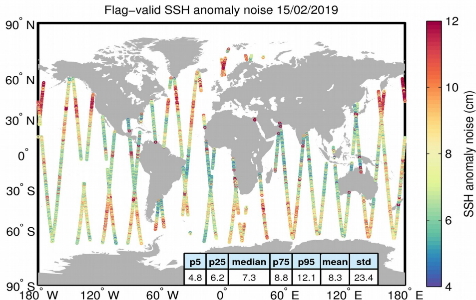
Figure 8. Geographical distribution of flag-valid 20-Hz SSH anomaly measurement noise over oceans and lakes for 15/02/2019. The statistical values shown in the table refer to the SSH anomaly noise and are calculated over all measurements shown in the figure.
