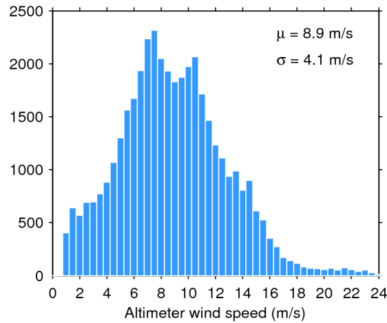
Figure 33. Histogram of flag-valid wind over oceans and lakes for 14/02/2019. The mean ( \mu ) and standard deviation ( \sigma ) are also shown. Note that values larger than 24 m/s are excluded from the histogram for the sake of readability but not from the computation of \mu and \sigma .
