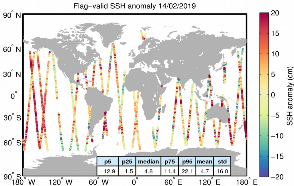
Figure 5. Geographical distribution of flag-valid 1-Hz SSH anomaly data over oceans and lakes for 14/02/2019. The statistical values shown in the table refer to the SSH anomaly in cm and are calculated over all measurements shown in the figure.
