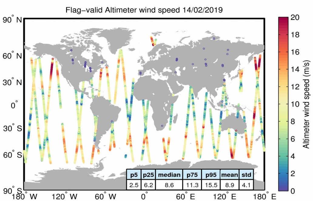
Figure 31. Geographical distribution of flag-valid wind data over oceans and lakes for 14/02/2019. The statistical values shown in the table refer to the wind in m/s and are calculated over all measurements shown in the figure.
