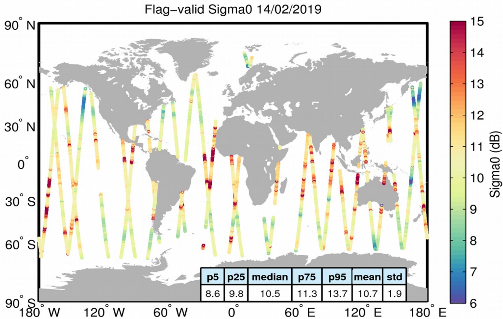
Figure 23. Geographical distribution of flag-valid sigma0 data over oceans and lakes for 14/02/2019. The statistical values shown in the table refer to the sigma0 in dB and are calculated over all measurements shown in the figure.
