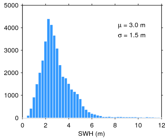
Figure 17. Histogram of flag-valid SWH over oceans and lakes for 14/02/2019. The mean ( \mu ) and standard deviation ( \sigma ) are also shown. Note that values larger than 12 m are excluded from the histogram for the sake of readability but not from the computation of \mu and \sigma .
