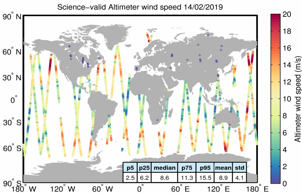
Figure 34. Geographical distribution of science-valid wind data over oceans and lakes for 14/02/2019. The statistical values shown in the table refer to the wind in m/s and are calculated over all measurements shown in the figure. Gray circles denote records that have been rejected based on the editing criteria described in Table 5.
