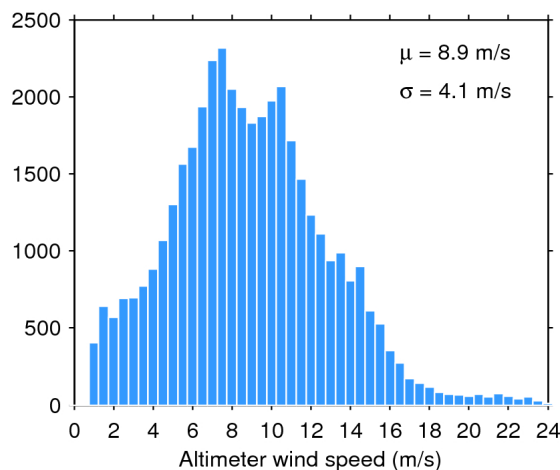
Figure 35. Histogram of science-valid wind over oceans and lakes for 14/02/2019. The mean ( \mu ) and standard deviation ( \sigma ) are also shown. Note that values larger than 24 m/s are excluded from the histogram for the sake of readability but not from the computation of \mu and \sigma .
