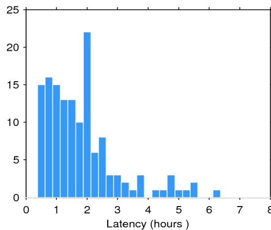
Figure 2. Histogram of the data latency for 14/02/2019. The y-axis denotes the number of files that are made available with a delay of x-hours with respect to the mean time of the records stored in the file.
