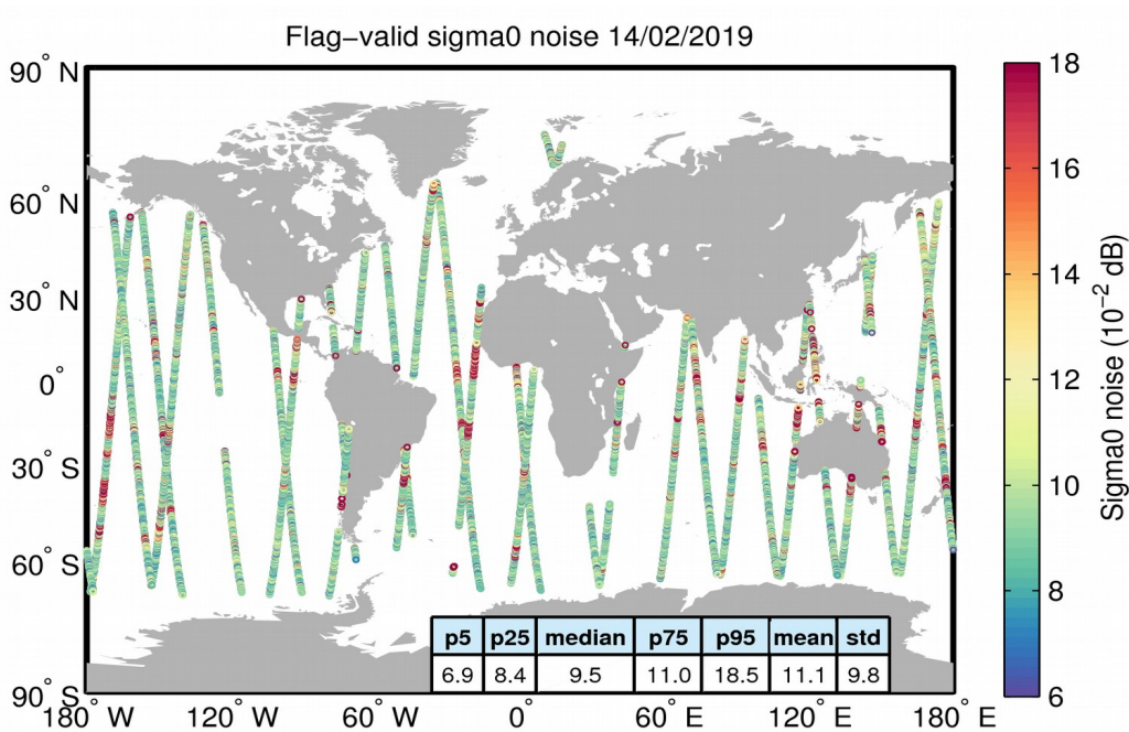
Figure 26. Geographical distribution of flag-valid 20-Hz sigma0 measurement noise over oceans and lakes for 14/02/2019. The statistical values shown in the table refer to the sigma0 noise and are calculated over all measurements shown in the figure.
