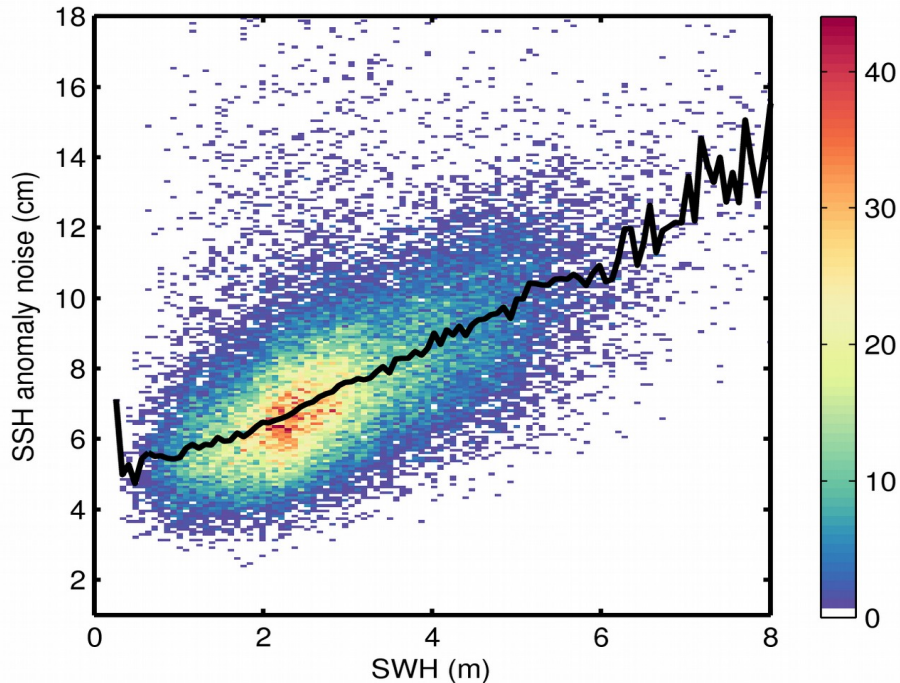
Figure 9. 2D histogram showing flag-valid SSH anomaly noise as a function of SWH for 14/02/2019. The black line denotes the median SSH anomaly noise as a function of SWH.
