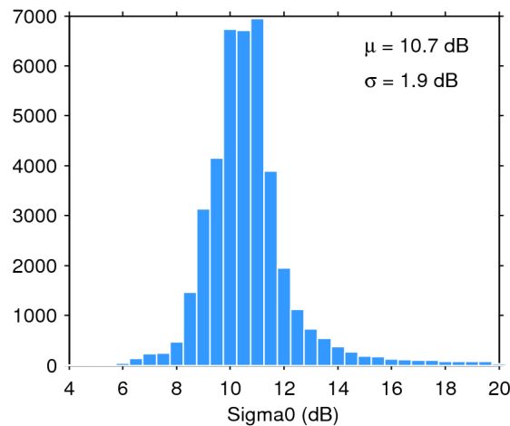
Figure 25. Histogram of flag-valid sigma0 over oceans and lakes for 14/02/2019. The mean ( \mu ) and standard deviation ( \sigma ) are also shown. Note that values outside [4 20] dB are excluded from the histogram for the sake of readability but not from the computation of \mu and \sigma .
