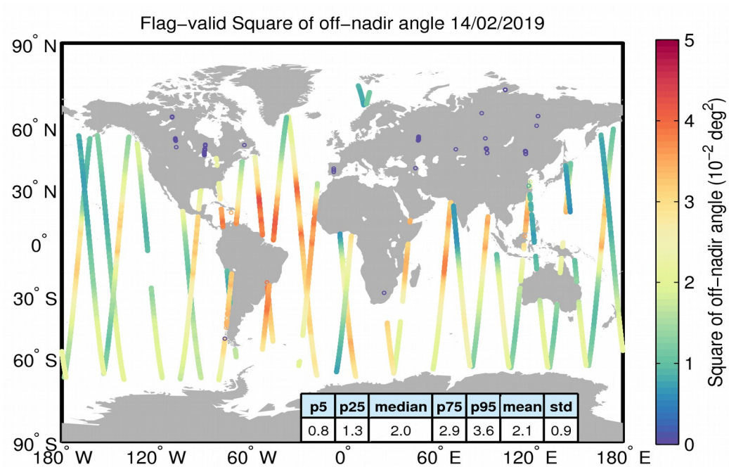
Figure 37. Geographical distribution of flag-valid mispointing data over oceans and lakes for 14/02/2019. The statistical values shown in the table refer to the mispointing in 10^{-2} \text{ deg}^2 and are calculated over all measurements shown in the figure.
