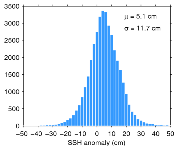
Figure 11. Histogram of science-valid SSH anomaly over oceans and lakes for 14/02/2019. The mean ( \mu ) and standard deviation ( \sigma ) are also shown. Note that values outside [-50 50] cm are excluded from the histogram for the sake of readability but not from the computation of \mu and \sigma .
