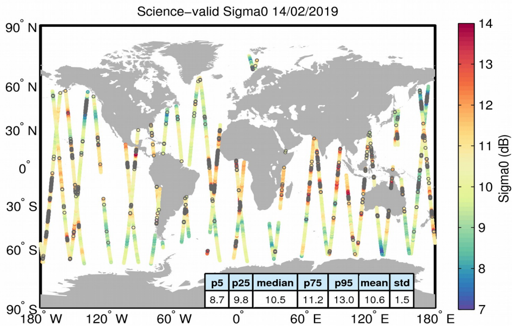
Figure 27. Geographical distribution of science-valid sigma0 data over oceans and lakes for 14/02/2019. The statistical values shown in the table refer to the sigma0 in dB and are calculated over all measurements shown in the figure. Gray circles denote records that have been rejected based on the editing criteria described in Table 4.
