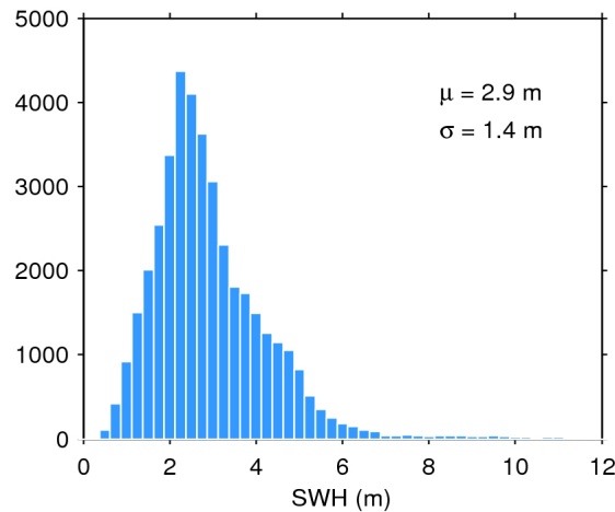
Figure 20. Histogram of science-valid SWH over oceans and lakes for 14/02/2019. The mean ( \mu ) and standard deviation ( \sigma ) are also shown. Note that values larger than 12 m are excluded from the histogram for the sake of readability but not from the computation of \mu and \sigma .
