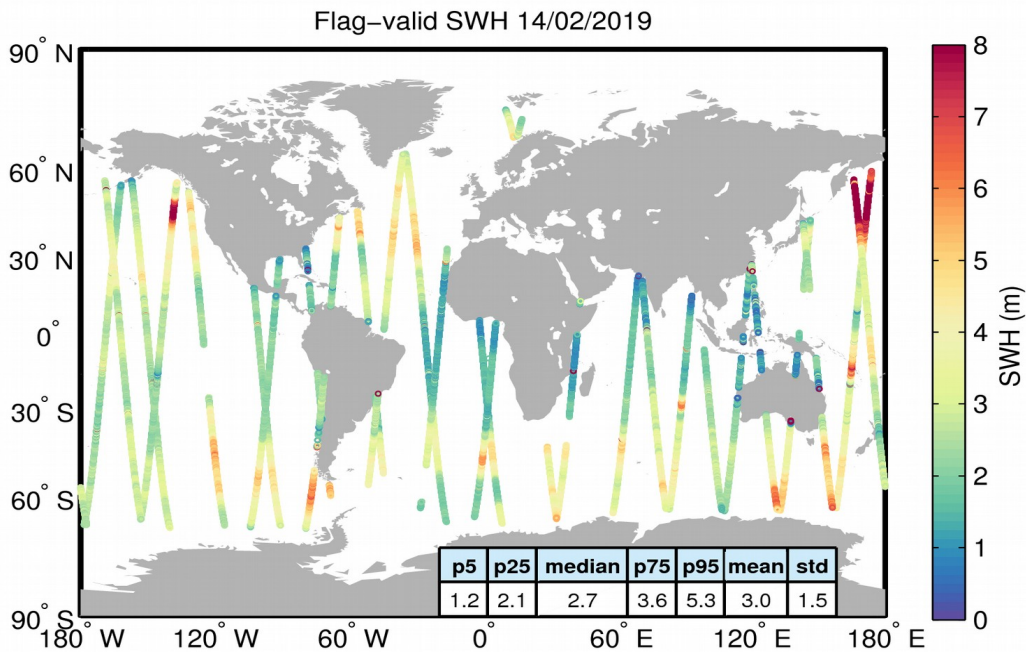
Figure 15. Geographical distribution of flag-valid SWH data over oceans and lakes for 14/02/2019. The statistical values shown in the table refer to the SWH in m and are calculated over all measurements shown in the figure.
