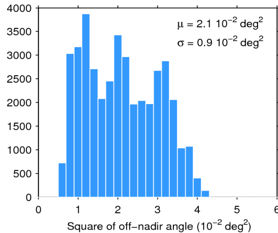
Figure 39. Histogram of flag-valid mispointing over oceans and lakes for 14/02/2019. The mean ( \mu ) and standard deviation ( \sigma ) are also shown. Note that values larger than 6 \cdot 10^{-2} \text{ deg}^2 are excluded from the histogram for the sake of readability but not from the computation of \mu and \sigma .
