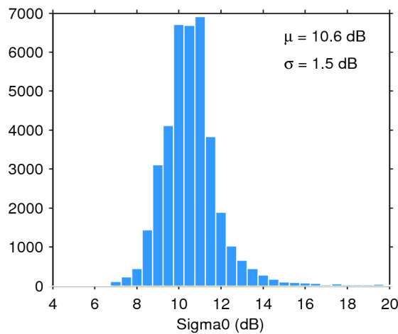
Figure 28. Histogram of science-valid sigma0 over oceans and lakes for 14/02/2019. The mean ( \mu ) and standard deviation ( \sigma ) are also shown. Note that values outside [4 20] dB are excluded from the histogram for the sake of readability but not from the computation of \mu and \sigma .
