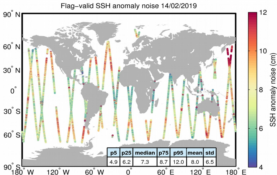
Figure 8. Geographical distribution of flag-valid 20-Hz SSH anomaly measurement noise over oceans and lakes for 14/02/2019. The statistical values shown in the table refer to the SSH anomaly noise and are calculated over all measurements shown in the figure.
