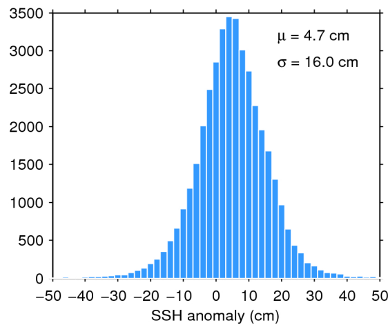
Figure 7. Histogram of flag-valid SSH anomaly over oceans and lakes for 14/02/2019. The mean ( \mu ) and standard deviation ( \sigma ) are also shown. Note that values outside [-50 50] cm are excluded from the histogram for the sake of readability but not from the computation of \mu and \sigma .
