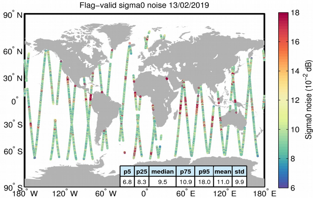
Figure 26. Geographical distribution of flag-valid 20-Hz sigma0 measurement noise over oceans and lakes for 13/02/2019. The statistical values shown in the table refer to the sigma0 noise and are calculated over all measurements shown in the figure.
