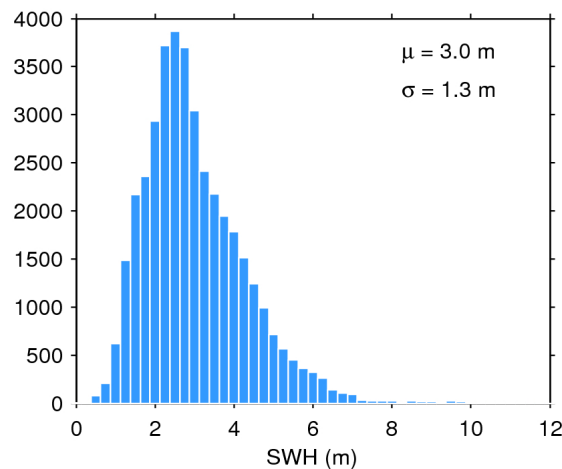
Figure 17. Histogram of flag-valid SWH over oceans and lakes for 13/02/2019. The mean ( \mu ) and standard deviation ( \sigma ) are also shown. Note that values larger than 12 m are excluded from the histogram for the sake of readability but not from the computation of \mu and \sigma .
