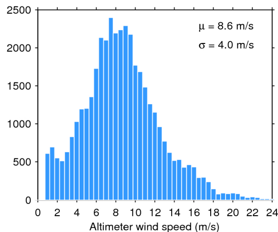
Figure 35. Histogram of science-valid wind over oceans and lakes for 13/02/2019. The mean ( \mu ) and standard deviation ( \sigma ) are also shown. Note that values larger than 24 m/s are excluded from the histogram for the sake of readability but not from the computation of \mu and \sigma .
