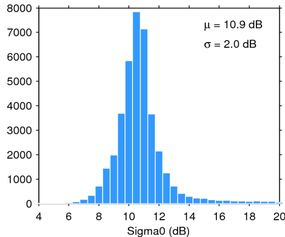
Figure 25. Histogram of flag-valid sigma0 over oceans and lakes for 13/02/2019. The mean ( \mu ) and standard deviation ( \sigma ) are also shown. Note that values outside [4 20] dB are excluded from the histogram for the sake of readability but not from the computation of \mu and \sigma .
