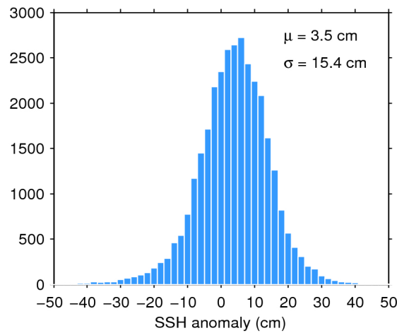
Figure 11. Histogram of science-valid SSH anomaly over oceans and lakes for 13/02/2019. The mean ( \mu ) and standard deviation ( \sigma ) are also shown. Note that values outside [-50 50] cm are excluded from the histogram for the sake of readability but not from the computation of \mu and \sigma .
