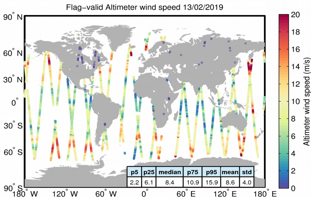
Figure 31. Geographical distribution of flag-valid wind data over oceans and lakes for 13/02/2019. The statistical values shown in the table refer to the wind in m/s and are calculated over all measurements shown in the figure.
