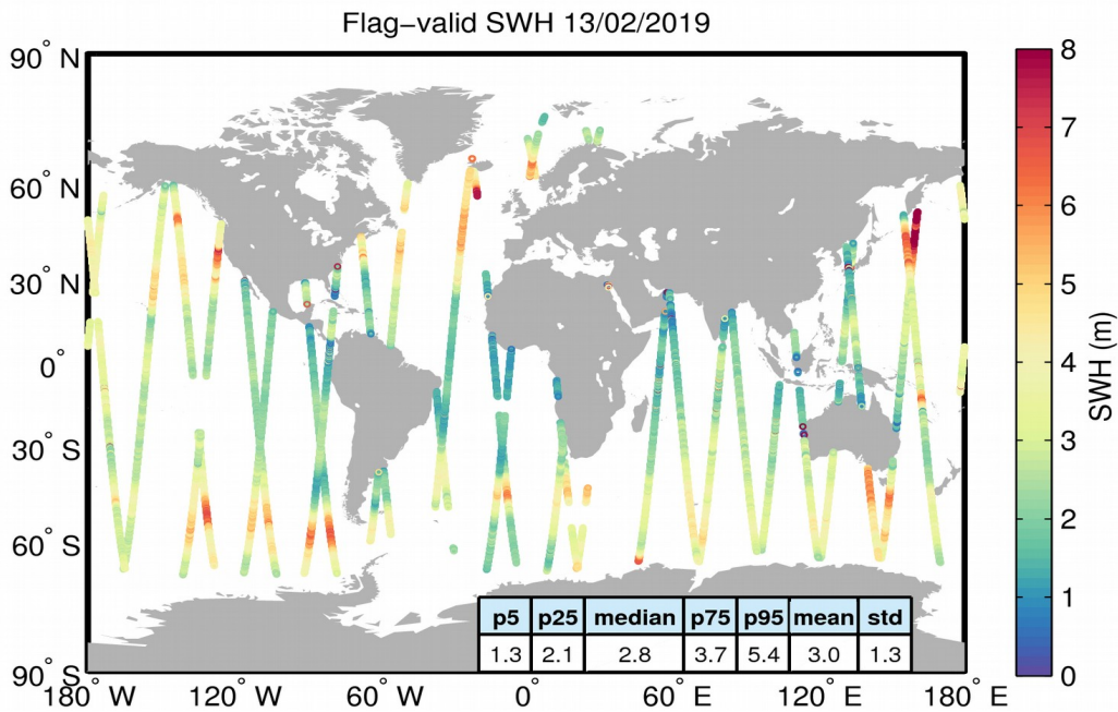
Figure 15. Geographical distribution of flag-valid SWH data over oceans and lakes for 13/02/2019. The statistical values shown in the table refer to the SWH in m and are calculated over all measurements shown in the figure.
