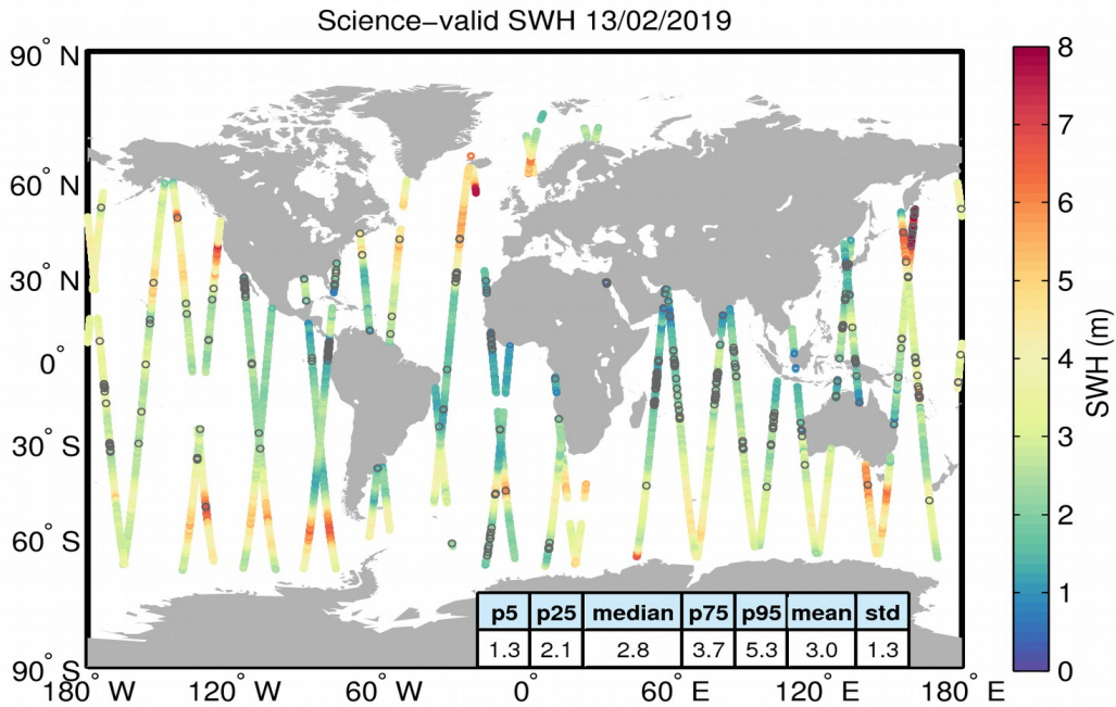
Figure 19. Geographical distribution of science-valid SWH data over oceans and lakes for 13/02/2019. The statistical values shown in the table refer to the SWH in m and are calculated over all measurements shown in the figure. Gray circles denote records that have been rejected based on the editing criteria described in Table 3.
