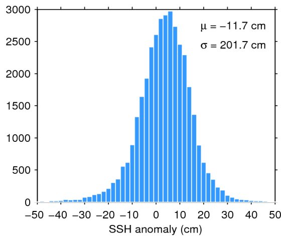
Figure 7. Histogram of flag-valid SSH anomaly over oceans and lakes for 13/02/2019. The mean ( \mu ) and standard deviation ( \sigma ) are also shown. Note that values outside [-50 50] cm are excluded from the histogram for the sake of readability but not from the computation of \mu and \sigma .
