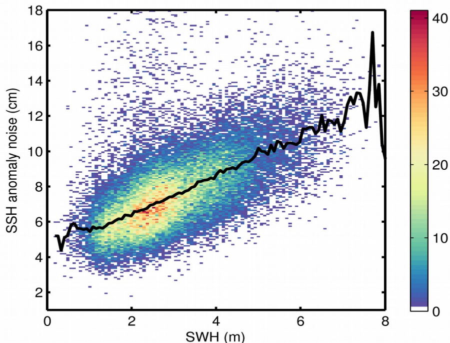
Figure 9. 2D histogram showing flag-valid SSH anomaly noise as a function of SWH for 13/02/2019. The black line denotes the median SSH anomaly noise as a function of SWH.
