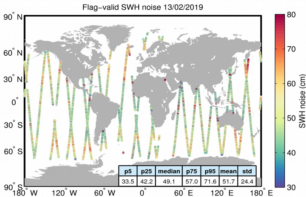
Figure 18. Geographical distribution of flag-valid 20-Hz SWH measurement noise over oceans and lakes for 13/02/2019. The statistical values shown in the figure refer to the SWH noise and are calculated over all measurements shown in the figure.
