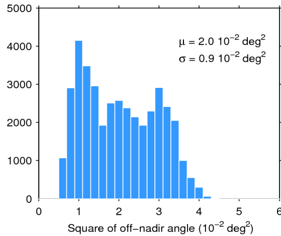
Figure 39. Histogram of flag-valid mispointing over oceans and lakes for 13/02/2019. The mean ( \mu ) and standard deviation ( \sigma ) are also shown. Note that values larger than 6 \cdot 10^{-2} \text{ deg}^2 are excluded from the histogram for the sake of readability but not from the computation of \mu and \sigma .
