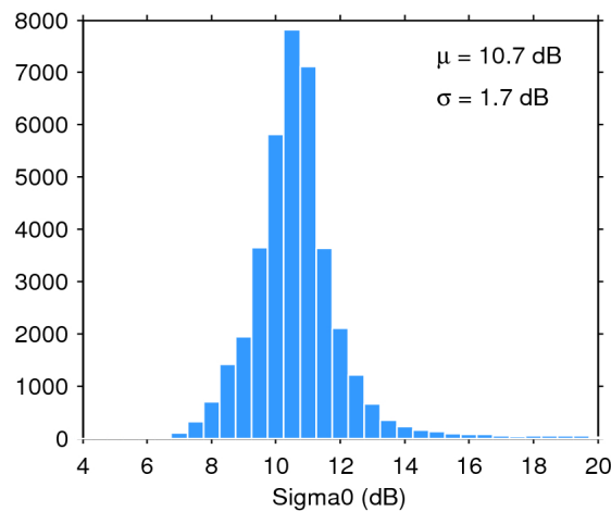
Figure 28. Histogram of science-valid sigma0 over oceans and lakes for 13/02/2019. The mean ( \mu ) and standard deviation ( \sigma ) are also shown. Note that values outside [4 20] dB are excluded from the histogram for the sake of readability but not from the computation of \mu and \sigma .
