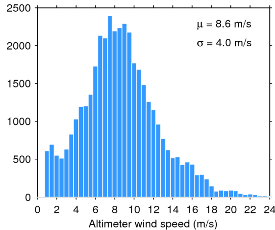
Figure 33. Histogram of flag-valid wind over oceans and lakes for 13/02/2019. The mean ( \mu ) and standard deviation ( \sigma ) are also shown. Note that values larger than 24 m/s are excluded from the histogram for the sake of readability but not from the computation of \mu and \sigma .
