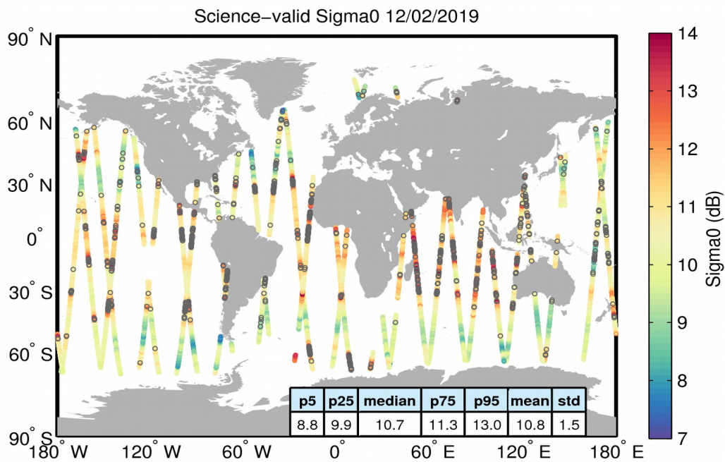
Figure 27. Geographical distribution of science-valid sigma0 data over oceans and lakes for 12/02/2019. The statistical values shown in the table refer to the sigma0 in dB and are calculated over all measurements shown in the figure. Gray circles denote records that have been rejected based on the editing criteria described in Table 4.
