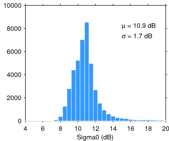
Figure 25. Histogram of flag-valid sigma0 over oceans and lakes for 12/02/2019. The mean ( \mu ) and standard deviation ( \sigma ) are also shown. Note that values outside [4 20] dB are excluded from the histogram for the sake of readability but not from the computation of \mu and \sigma .
