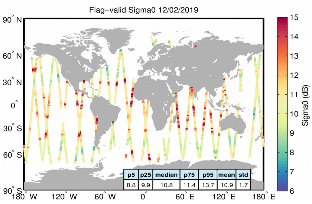
Figure 23. Geographical distribution of flag-valid sigma0 data over oceans and lakes for 12/02/2019. The statistical values shown in the table refer to the sigma0 in dB and are calculated over all measurements shown in the figure.
