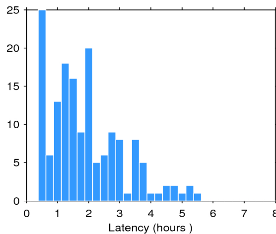
Figure 2. Histogram of the data latency for 12/02/2019. The y-axis denotes the number of files that are made available with a delay of x-hours with respect to the mean time of the records stored in the file.
