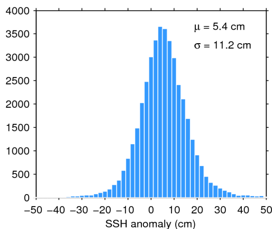
Figure 11. Histogram of science-valid SSH anomaly over oceans and lakes for 12/02/2019. The mean ( \mu ) and standard deviation ( \sigma ) are also shown. Note that values outside [-50 50] cm are excluded from the histogram for the sake of readability but not from the computation of \mu and \sigma .
