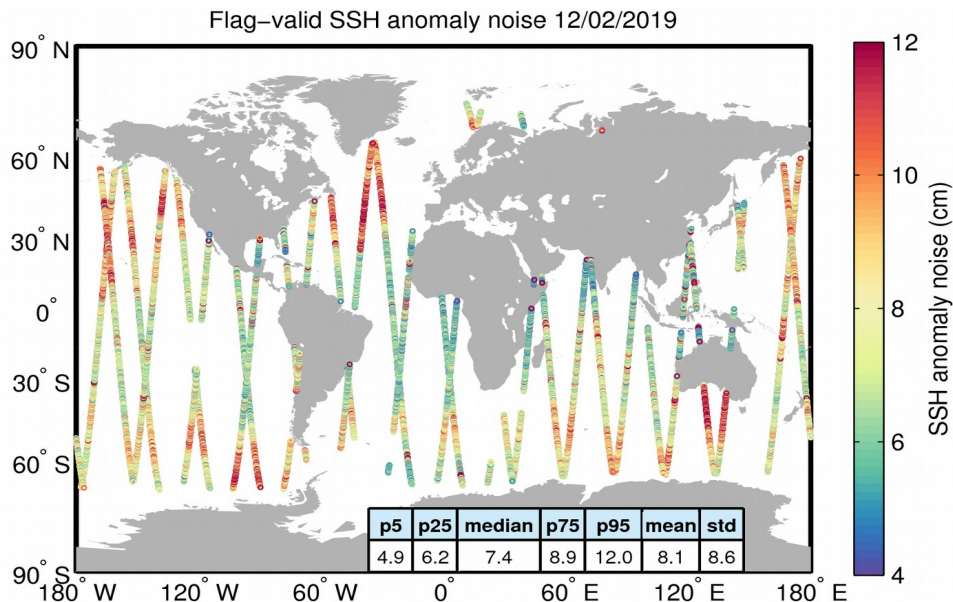
Figure 8. Geographical distribution of flag-valid 20-Hz SSH anomaly measurement noise over oceans and lakes for 12/02/2019. The statistical values shown in the table refer to the SSH anomaly noise and are calculated over all measurements shown in the figure.
