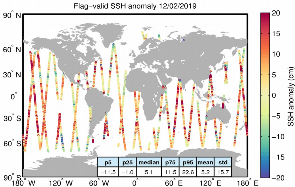
Figure 5. Geographical distribution of flag-valid 1-Hz SSH anomaly data over oceans and lakes for 12/02/2019. The statistical values shown in the table refer to the SSH anomaly in cm and are calculated over all measurements shown in the figure.
