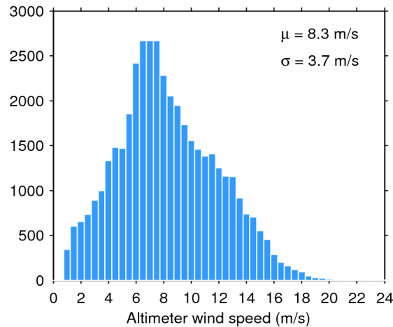
Figure 33. Histogram of flag-valid wind over oceans and lakes for 12/02/2019. The mean ( \mu ) and standard deviation ( \sigma ) are also shown. Note that values larger than 24 m/s are excluded from the histogram for the sake of readability but not from the computation of \mu and \sigma .
