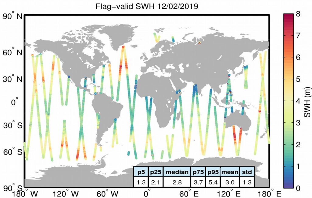
Figure 15. Geographical distribution of flag-valid SWH data over oceans and lakes for 12/02/2019. The statistical values shown in the table refer to the SWH in m and are calculated over all measurements shown in the figure.
