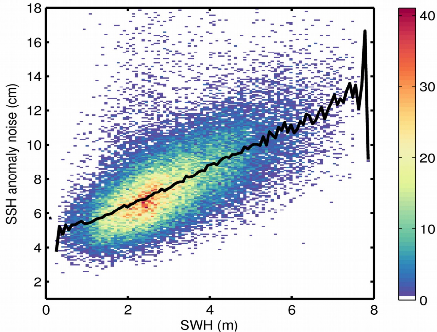
Figure 9. 2D histogram showing flag-valid SSH anomaly noise as a function of SWH for 12/02/2019. The black line denotes the median SSH anomaly noise as a function of SWH.
