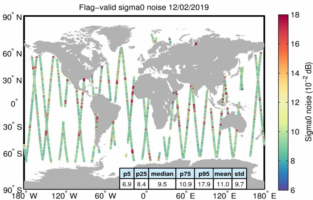
Figure 26. Geographical distribution of flag-valid 20-Hz sigma0 measurement noise over oceans and lakes for 12/02/2019. The statistical values shown in the table refer to the sigma0 noise and are calculated over all measurements shown in the figure.
