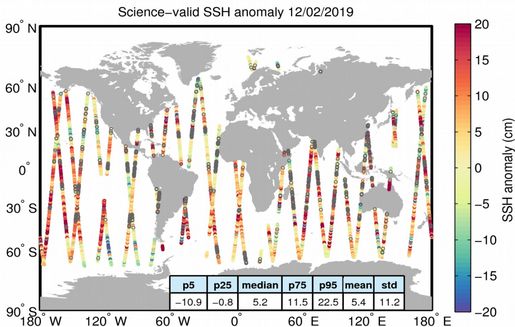
Figure 10. Geographical distribution of science-valid SSH anomaly data over oceans and lakes for 12/02/2019. The statistical values shown in the table refer to the SSH anomaly in cm and are calculated over all measurements shown in the figure. Gray circles denote records that have been rejected based on the editing criteria described in Table 2.
