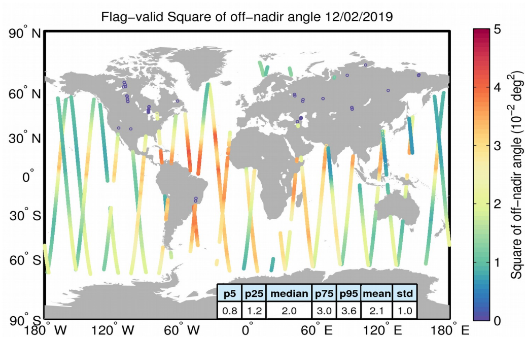
Figure 37. Geographical distribution of flag-valid mispointing data over oceans and lakes for 12/02/2019. The statistical values shown in the table refer to the mispointing in 10^{-2} \text{deg}^2 and are calculated over all measurements shown in the figure.
