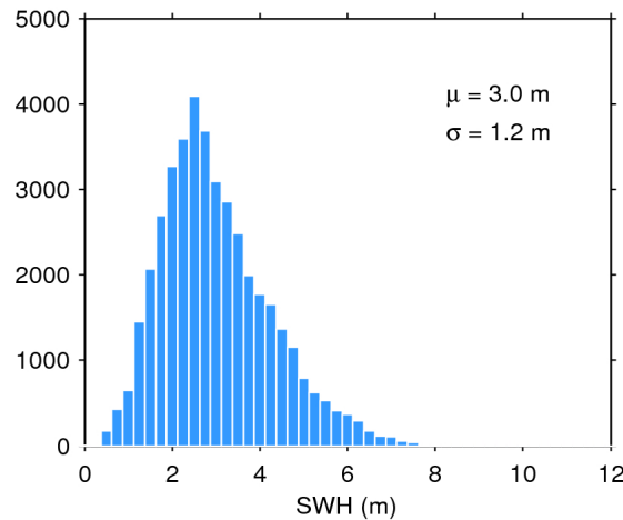
Figure 20. Histogram of science-valid SWH over oceans and lakes for 12/02/2019. The mean ( \mu ) and standard deviation ( \sigma ) are also shown. Note that values larger than 12 m are excluded from the histogram for the sake of readability but not from the computation of \mu and \sigma .
