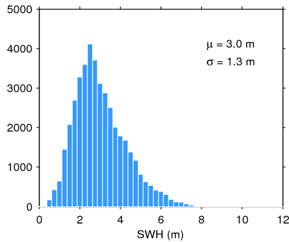
Figure 17. Histogram of flag-valid SWH over oceans and lakes for 12/02/2019. The mean ( \mu ) and standard deviation ( \sigma ) are also shown. Note that values larger than 12 m are excluded from the histogram for the sake of readability but not from the computation of \mu and \sigma .
