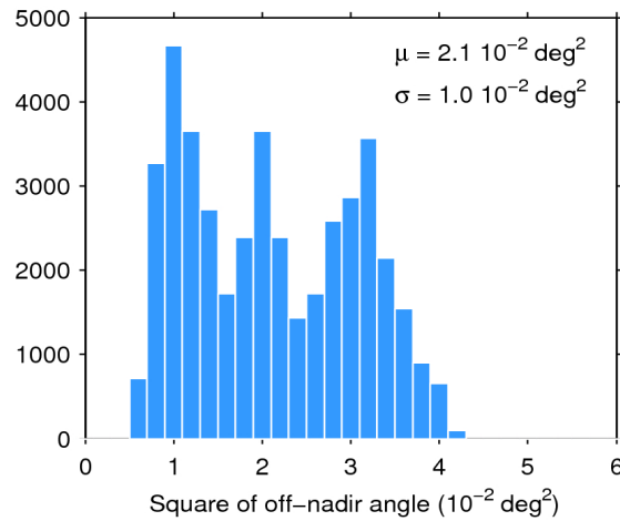
Figure 39. Histogram of flag-valid mispointing over oceans and lakes for 12/02/2019. The mean ( \mu ) and standard deviation ( \sigma ) are also shown. Note that values larger than 6 \cdot 10^{-2} \text{ deg}^2 are excluded from the histogram for the sake of readability but not from the computation of \mu and \sigma .
