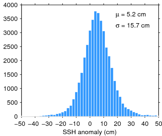
Figure 7. Histogram of flag-valid SSH anomaly over oceans and lakes for 12/02/2019. The mean ( \mu ) and standard deviation ( \sigma ) are also shown. Note that values outside [-50 50] cm are excluded from the histogram for the sake of readability but not from the computation of \mu and \sigma .
