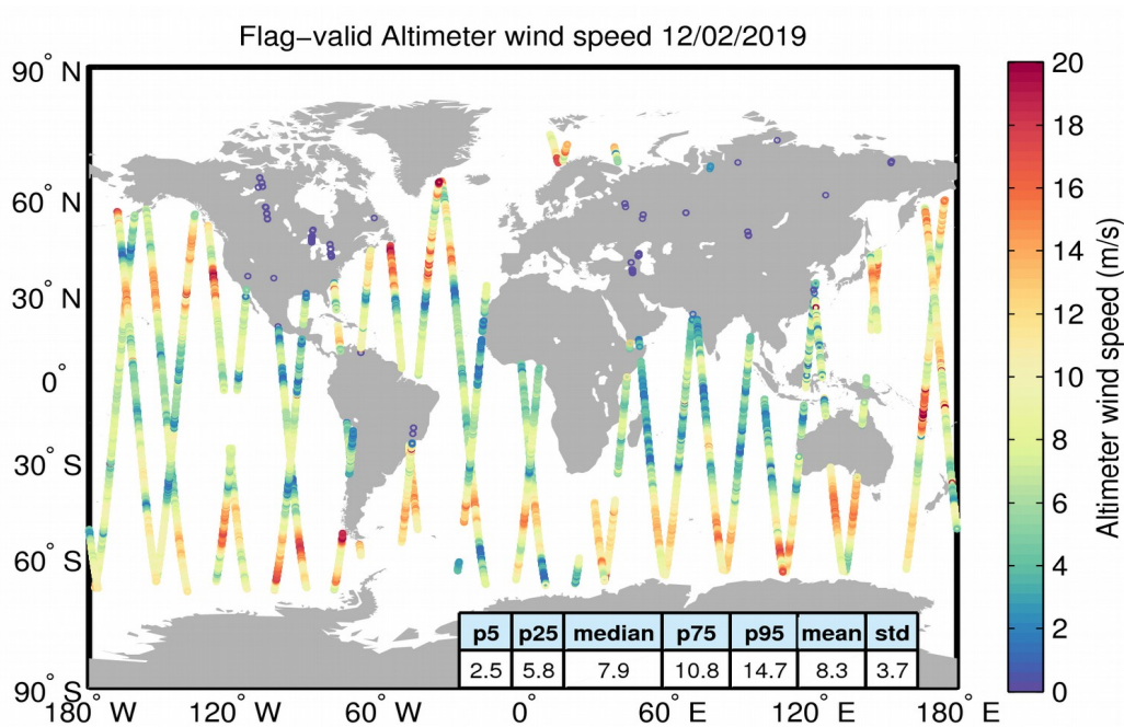
Figure 31. Geographical distribution of flag-valid wind data over oceans and lakes for 12/02/2019. The statistical values shown in the table refer to the wind in m/s and are calculated over all measurements shown in the figure.
