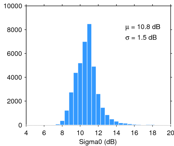
Figure 28. Histogram of science-valid sigma0 over oceans and lakes for 12/02/2019. The mean ( \mu ) and standard deviation ( \sigma ) are also shown. Note that values outside [4 20] dB are excluded from the histogram for the sake of readability but not from the computation of \mu and \sigma .
