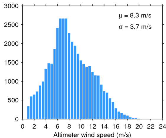
Figure 35. Histogram of science-valid wind over oceans and lakes for 12/02/2019. The mean ( \mu ) and standard deviation ( \sigma ) are also shown. Note that values larger than 24 m/s are excluded from the histogram for the sake of readability but not from the computation of \mu and \sigma .
