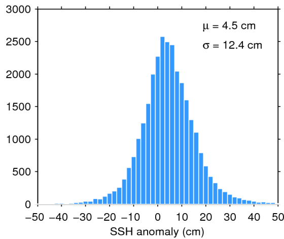
Figure 11. Histogram of science-valid SSH anomaly over oceans and lakes for 11/02/2019. The mean ( \mu ) and standard deviation ( \sigma ) are also shown. Note that values outside [-50 50] cm are excluded from the histogram for the sake of readability but not from the computation of \mu and \sigma .
