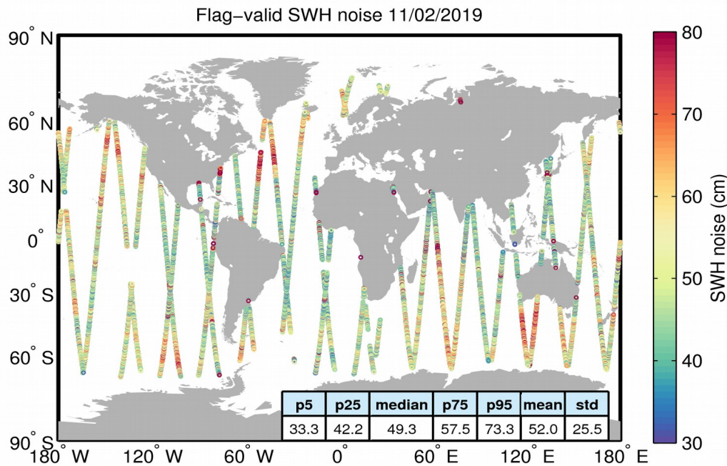
Figure 18. Geographical distribution of flag-valid 20-Hz SWH measurement noise over oceans and lakes for 11/02/2019. The statistical values shown in the figure refer to the SWH noise and are calculated over all measurements shown in the figure.
