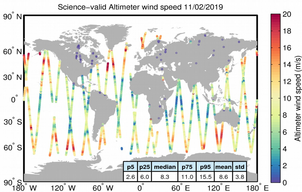
Figure 34. Geographical distribution of science-valid wind data over oceans and lakes for 11/02/2019. The statistical values shown in the table refer to the wind in m/s and are calculated over all measurements shown in the figure. Gray circles denote records that have been rejected based on the editing criteria described in Table 5.
