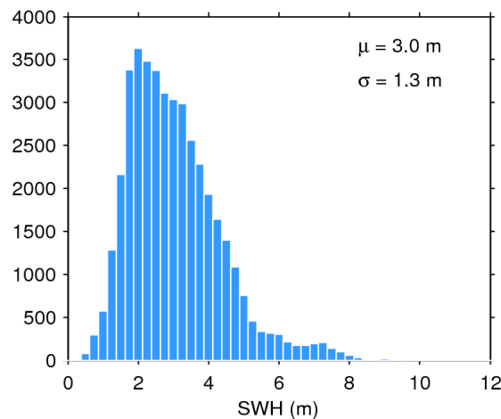
Figure 20. Histogram of science-valid SWH over oceans and lakes for 11/02/2019. The mean ( \mu ) and standard deviation ( \sigma ) are also shown. Note that values larger than 12 m are excluded from the histogram for the sake of readability but not from the computation of \mu and \sigma .
