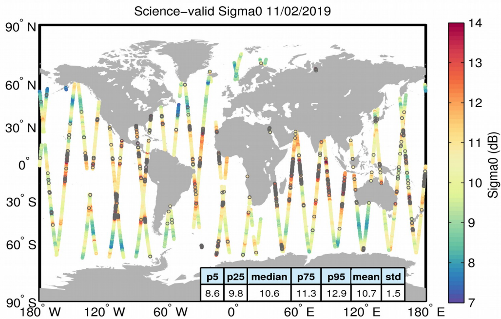
Figure 27. Geographical distribution of science-valid sigma0 data over oceans and lakes for 11/02/2019. The statistical values shown in the table refer to the sigma0 in dB and are calculated over all measurements shown in the figure. Gray circles denote records that have been rejected based on the editing criteria described in Table 4.
