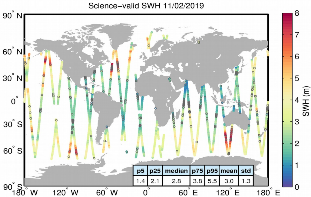
Figure 19. Geographical distribution of science-valid SWH data over oceans and lakes for 11/02/2019. The statistical values shown in the table refer to the SWH in m and are calculated over all measurements shown in the figure. Gray circles denote records that have been rejected based on the editing criteria described in Table 3.
