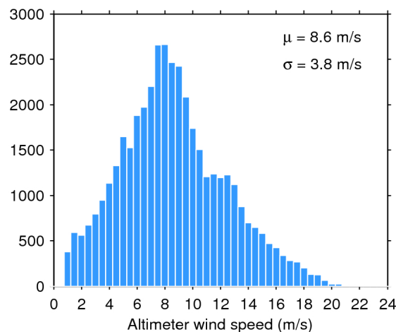
Figure 35. Histogram of science-valid wind over oceans and lakes for 11/02/2019. The mean ( \mu ) and standard deviation ( \sigma ) are also shown. Note that values larger than 24 m/s are excluded from the histogram for the sake of readability but not from the computation of \mu and \sigma .
