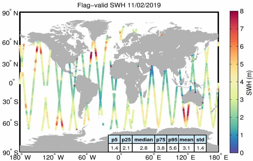
Figure 15. Geographical distribution of flag-valid SWH data over oceans and lakes for 11/02/2019. The statistical values shown in the table refer to the SWH in m and are calculated over all measurements shown in the figure.
