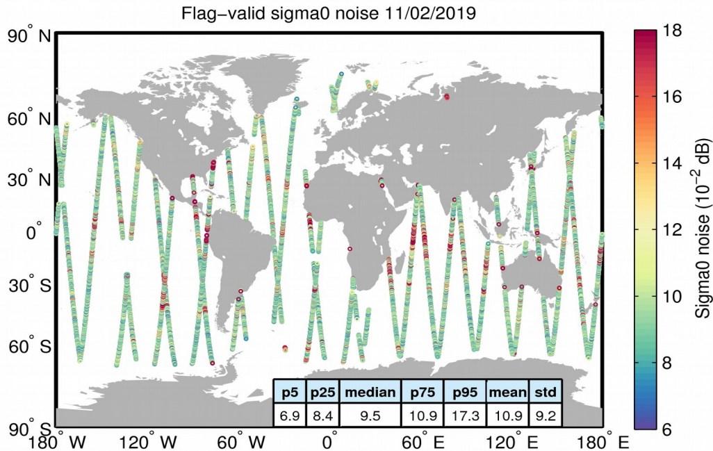
Figure 26. Geographical distribution of flag-valid 20-Hz sigma0 measurement noise over oceans and lakes for 11/02/2019. The statistical values shown in the table refer to the sigma0 noise and are calculated over all measurements shown in the figure.
