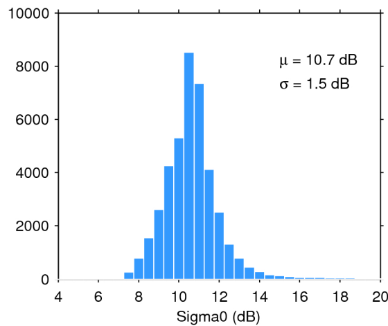
Figure 28. Histogram of science-valid sigma0 over oceans and lakes for 11/02/2019. The mean ( \mu ) and standard deviation ( \sigma ) are also shown. Note that values outside [4 20] dB are excluded from the histogram for the sake of readability but not from the computation of \mu and \sigma .
