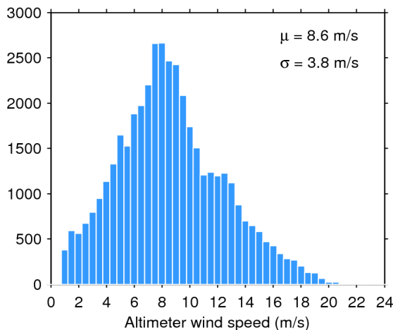
Figure 33. Histogram of flag-valid wind over oceans and lakes for 11/02/2019. The mean ( \mu ) and standard deviation ( \sigma ) are also shown. Note that values larger than 24 m/s are excluded from the histogram for the sake of readability but not from the computation of \mu and \sigma .
