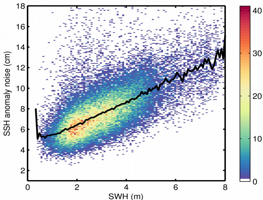
Figure 9. 2D histogram showing flag-valid SSH anomaly noise as a function of SWH for 11/02/2019. The black line denotes the median SSH anomaly noise as a function of SWH.
