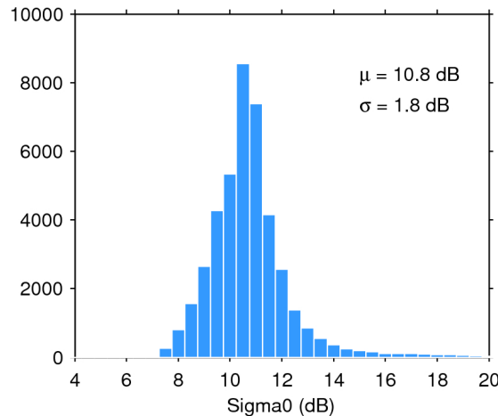
Figure 25. Histogram of flag-valid sigma0 over oceans and lakes for 11/02/2019. The mean ( \mu ) and standard deviation ( \sigma ) are also shown. Note that values outside [4 20] dB are excluded from the histogram for the sake of readability but not from the computation of \mu and \sigma .
