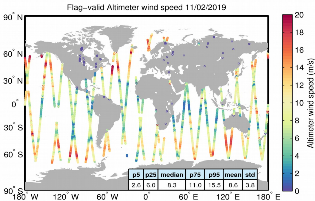
Figure 31. Geographical distribution of flag-valid wind data over oceans and lakes for 11/02/2019. The statistical values shown in the table refer to the wind in m/s and are calculated over all measurements shown in the figure.
