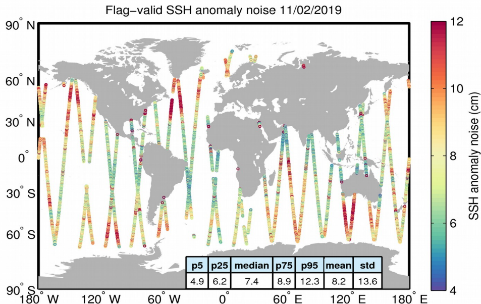
Figure 8. Geographical distribution of flag-valid 20-Hz SSH anomaly measurement noise over oceans and lakes for 11/02/2019. The statistical values shown in the table refer to the SSH anomaly noise and are calculated over all measurements shown in the figure.
