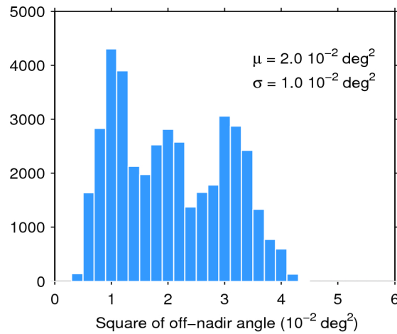
Figure 39. Histogram of flag-valid mispointing over oceans and lakes for 11/02/2019. The mean ( \mu ) and standard deviation ( \sigma ) are also shown. Note that values larger than 6 \cdot 10^{-2} \text{ deg}^2 are excluded from the histogram for the sake of readability but not from the computation of \mu and \sigma .
