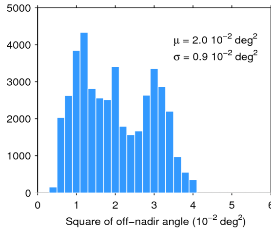
Figure 39. Histogram of flag-valid mispointing over oceans and lakes for 10/02/2019. The mean ( \mu ) and standard deviation ( \sigma ) are also shown. Note that values larger than 6 \cdot 10^{-2} \text{ deg}^2 are excluded from the histogram for the sake of readability but not from the computation of \mu and \sigma .
