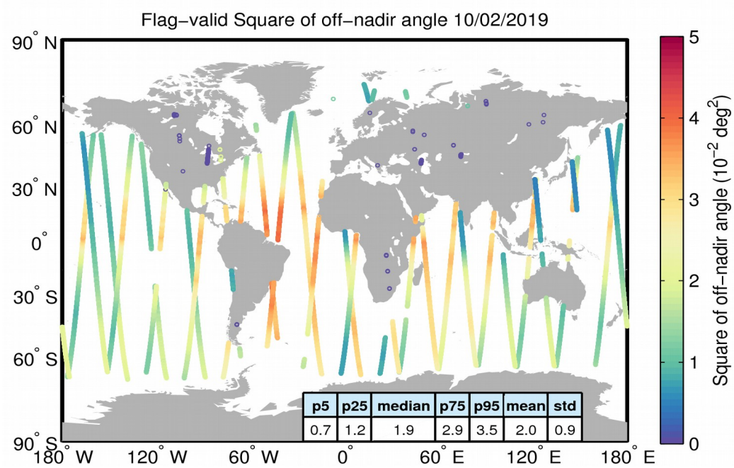
Figure 37. Geographical distribution of flag-valid mispointing data over oceans and lakes for 10/02/2019. The statistical values shown in the table refer to the mispointing in 10^{-2} \text{ deg}^2 and are calculated over all measurements shown in the figure.
