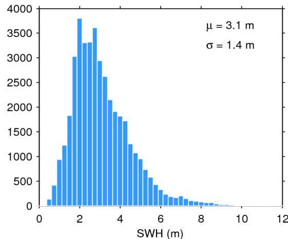
Figure 20. Histogram of science-valid SWH over oceans and lakes for 10/02/2019. The mean ( \mu ) and standard deviation ( \sigma ) are also shown. Note that values larger than 12 m are excluded from the histogram for the sake of readability but not from the computation of \mu and \sigma .
