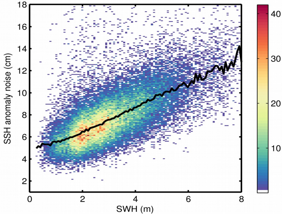
Figure 9. 2D histogram showing flag-valid SSH anomaly noise as a function of SWH for 10/02/2019. The black line denotes the median SSH anomaly noise as a function of SWH.
