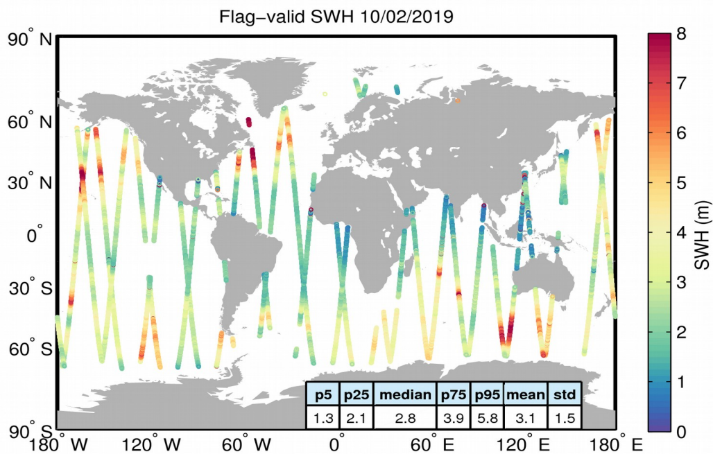
Figure 15. Geographical distribution of flag-valid SWH data over oceans and lakes for 10/02/2019. The statistical values shown in the table refer to the SWH in m and are calculated over all measurements shown in the figure.
