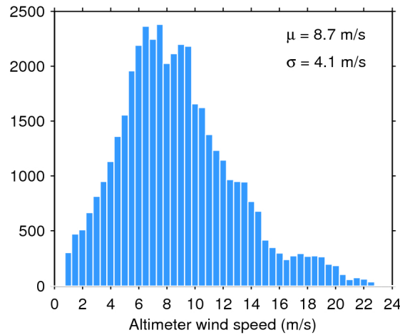
Figure 33. Histogram of flag-valid wind over oceans and lakes for 10/02/2019. The mean ( \mu ) and standard deviation ( \sigma ) are also shown. Note that values larger than 24 m/s are excluded from the histogram for the sake of readability but not from the computation of \mu and \sigma .
