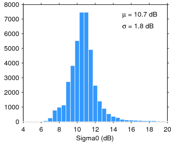
Figure 25. Histogram of flag-valid sigma0 over oceans and lakes for 10/02/2019. The mean ( \mu ) and standard deviation ( \sigma ) are also shown. Note that values outside [4 20] dB are excluded from the histogram for the sake of readability but not from the computation of \mu and \sigma .
