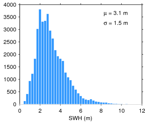
Figure 17. Histogram of flag-valid SWH over oceans and lakes for 10/02/2019. The mean ( \mu ) and standard deviation ( \sigma ) are also shown. Note that values larger than 12 m are excluded from the histogram for the sake of readability but not from the computation of \mu and \sigma .
