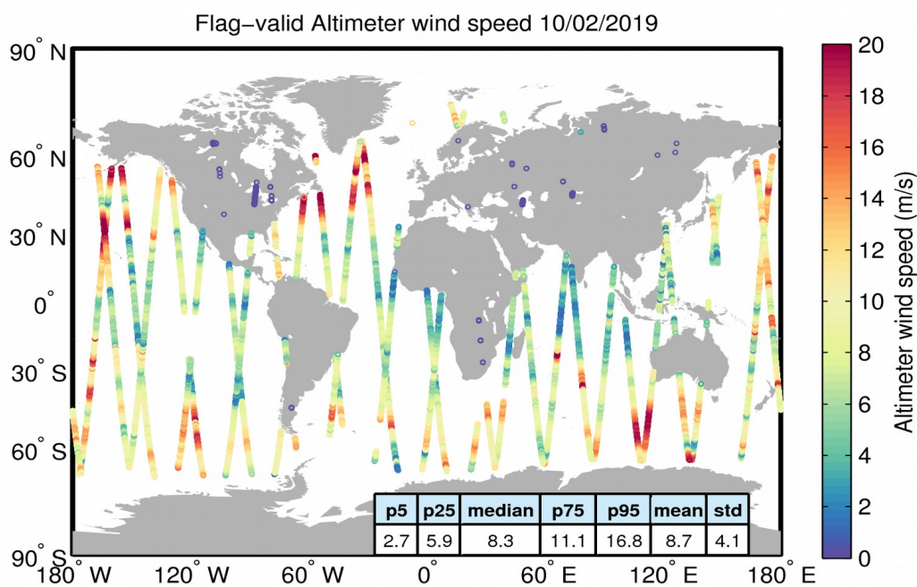
Figure 31. Geographical distribution of flag-valid wind data over oceans and lakes for 10/02/2019. The statistical values shown in the table refer to the wind in m/s and are calculated over all measurements shown in the figure.
