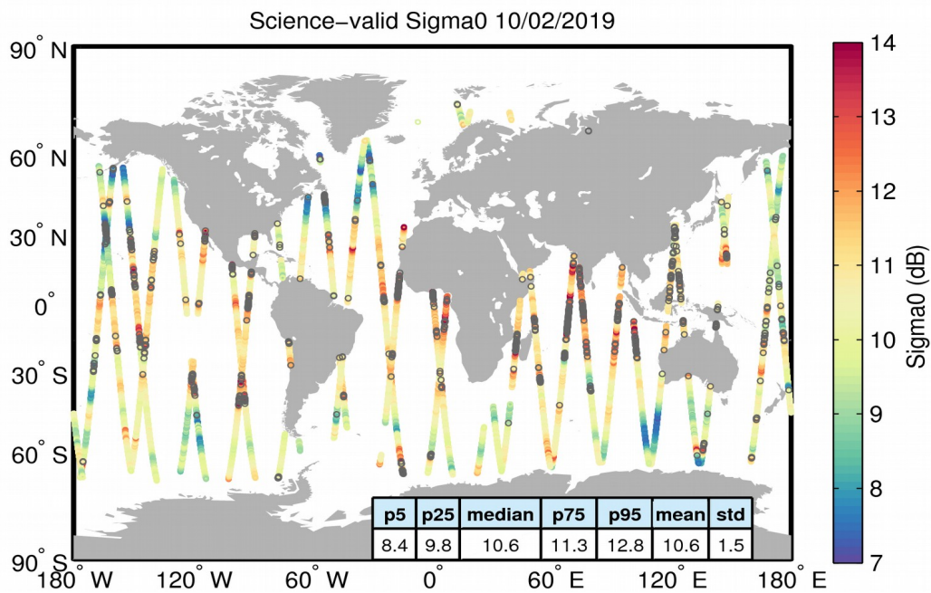
Figure 27. Geographical distribution of science-valid sigma0 data over oceans and lakes for 10/02/2019. The statistical values shown in the table refer to the sigma0 in dB and are calculated over all measurements shown in the figure. Gray circles denote records that have been rejected based on the editing criteria described in Table 4.
