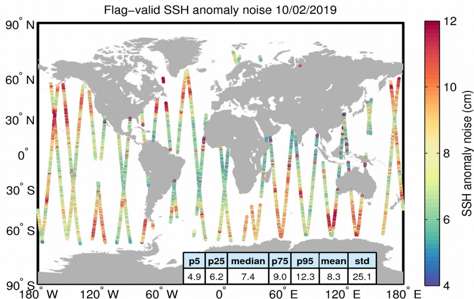
Figure 8. Geographical distribution of flag-valid 20-Hz SSH anomaly measurement noise over oceans and lakes for 10/02/2019. The statistical values shown in the table refer to the SSH anomaly noise and are calculated over all measurements shown in the figure.
