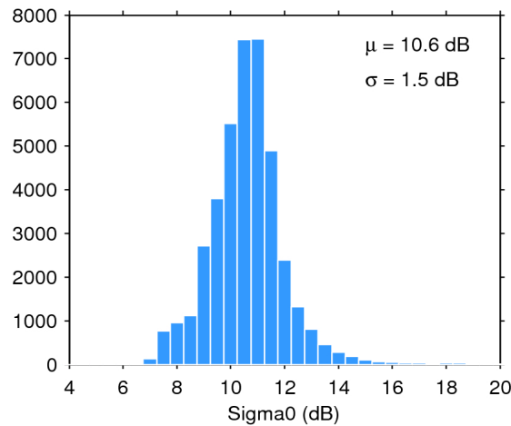
Figure 28. Histogram of science-valid sigma0 over oceans and lakes for 10/02/2019. The mean ( \mu ) and standard deviation ( \sigma ) are also shown. Note that values outside [4 20] dB are excluded from the histogram for the sake of readability but not from the computation of \mu and \sigma .
