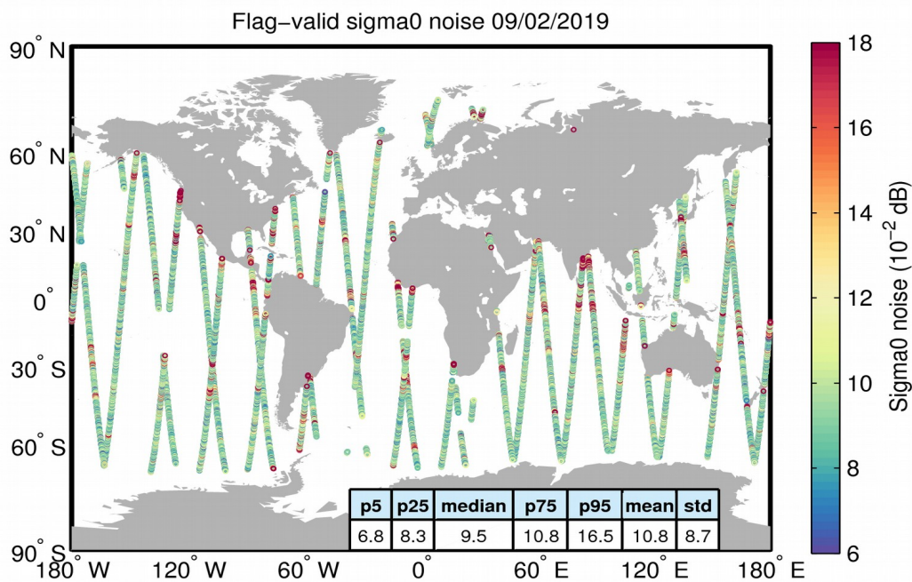
Figure 26. Geographical distribution of flag-valid 20-Hz sigma0 measurement noise over oceans and lakes for 09/02/2019. The statistical values shown in the table refer to the sigma0 noise and are calculated over all measurements shown in the figure.
