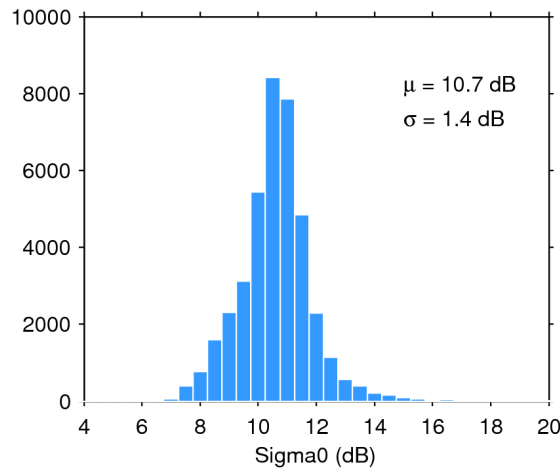
Figure 28. Histogram of science-valid sigma0 over oceans and lakes for 09/02/2019. The mean ( \mu ) and standard deviation ( \sigma ) are also shown. Note that values outside [4 20] dB are excluded from the histogram for the sake of readability but not from the computation of \mu and \sigma .
