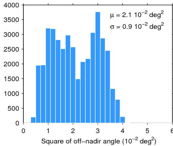
Figure 39. Histogram of flag-valid mispointing over oceans and lakes for 09/02/2019. The mean ( \mu ) and standard deviation ( \sigma ) are also shown. Note that values larger than 6 \cdot 10^{-2} \text{ deg}^2 are excluded from the histogram for the sake of readability but not from the computation of \mu and \sigma .
