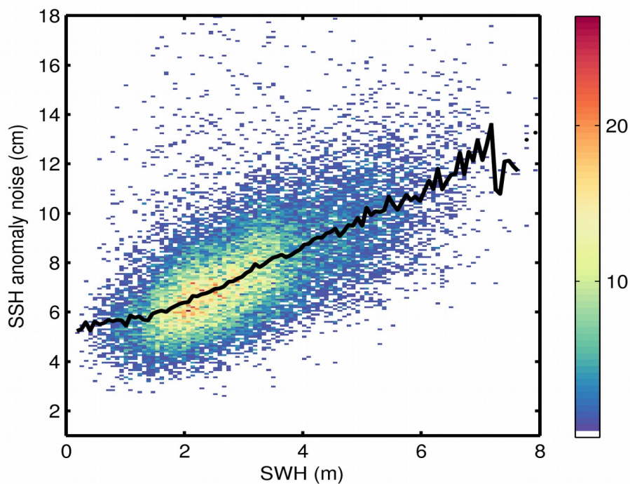
Figure 9. 2D histogram showing flag-valid SSH anomaly noise as a function of SWH for 09/02/2019. The black line denotes the median SSH anomaly noise as a function of SWH.
