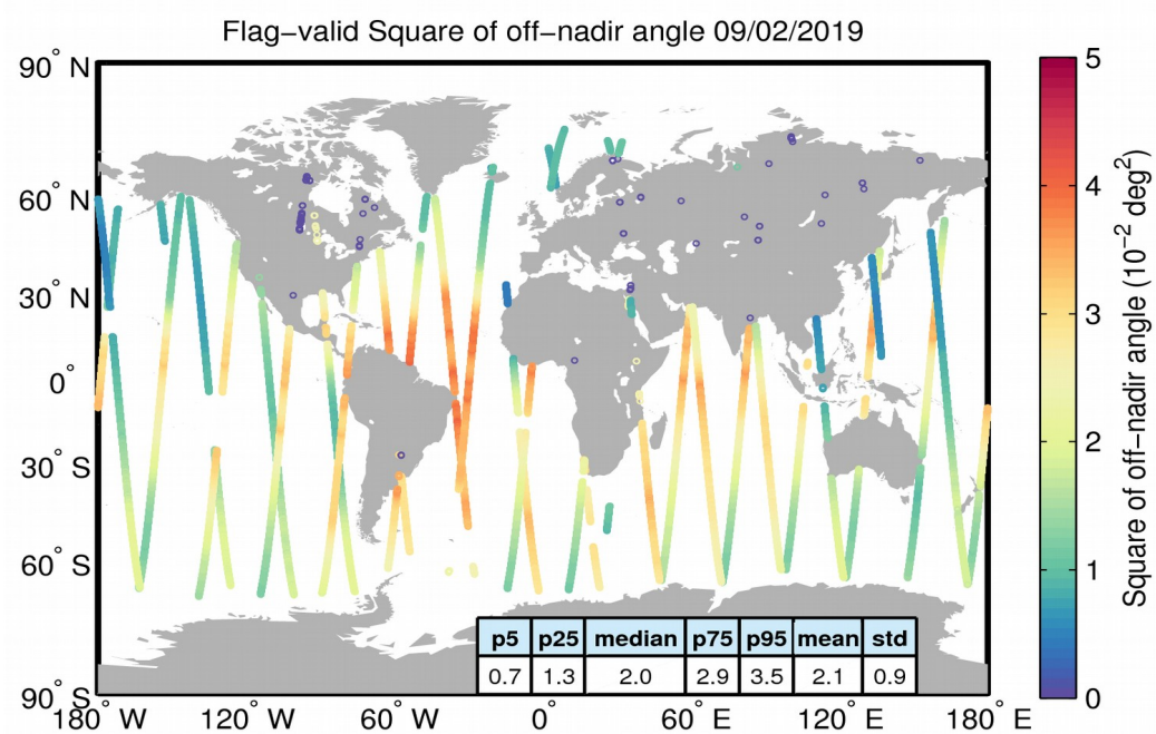
Figure 37. Geographical distribution of flag-valid mispointing data over oceans and lakes for 09/02/2019. The statistical values shown in the table refer to the mispointing in 10^{-2} \text{deg}^2 and are calculated over all measurements shown in the figure.
