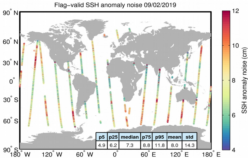
Figure 8. Geographical distribution of flag-valid 20-Hz SSH anomaly measurement noise over oceans and lakes for 09/02/2019. The statistical values shown in the table refer to the SSH anomaly noise and are calculated over all measurements shown in the figure.
