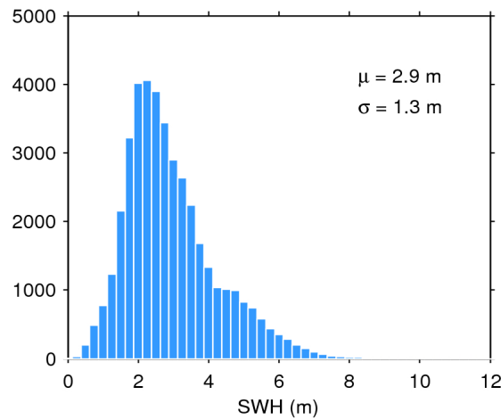
Figure 17. Histogram of flag-valid SWH over oceans and lakes for 09/02/2019. The mean ( \mu ) and standard deviation ( \sigma ) are also shown. Note that values larger than 12 m are excluded from the histogram for the sake of readability but not from the computation of \mu and \sigma .
