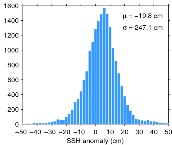
Figure 7. Histogram of flag-valid SSH anomaly over oceans and lakes for 09/02/2019. The mean ( \mu ) and standard deviation ( \sigma ) are also shown. Note that values outside [-50 50] cm are excluded from the histogram for the sake of readability but not from the computation of \mu and \sigma .
