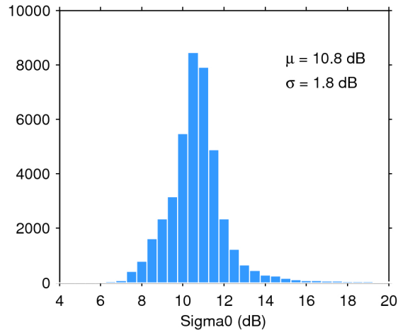
Figure 25. Histogram of flag-valid sigma0 over oceans and lakes for 09/02/2019. The mean ( \mu ) and standard deviation ( \sigma ) are also shown. Note that values outside [4 20] dB are excluded from the histogram for the sake of readability but not from the computation of \mu and \sigma .
