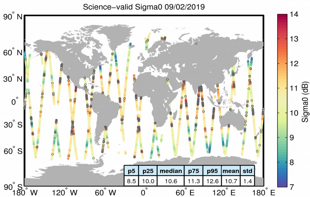
Figure 27. Geographical distribution of science-valid sigma0 data over oceans and lakes for 09/02/2019. The statistical values shown in the table refer to the sigma0 in dB and are calculated over all measurements shown in the figure. Gray circles denote records that have been rejected based on the editing criteria described in Table 4.
