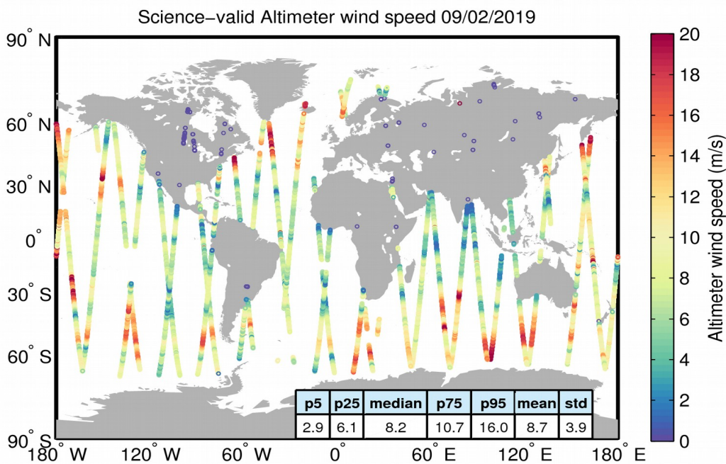
Figure 34. Geographical distribution of science-valid wind data over oceans and lakes for 09/02/2019. The statistical values shown in the table refer to the wind in m/s and are calculated over all measurements shown in the figure. Gray circles denote records that have been rejected based on the editing criteria described in Table 5.
