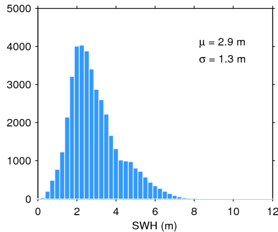
Figure 20. Histogram of science-valid SWH over oceans and lakes for 09/02/2019. The mean ( \mu ) and standard deviation ( \sigma ) are also shown. Note that values larger than 12 m are excluded from the histogram for the sake of readability but not from the computation of \mu and \sigma .
