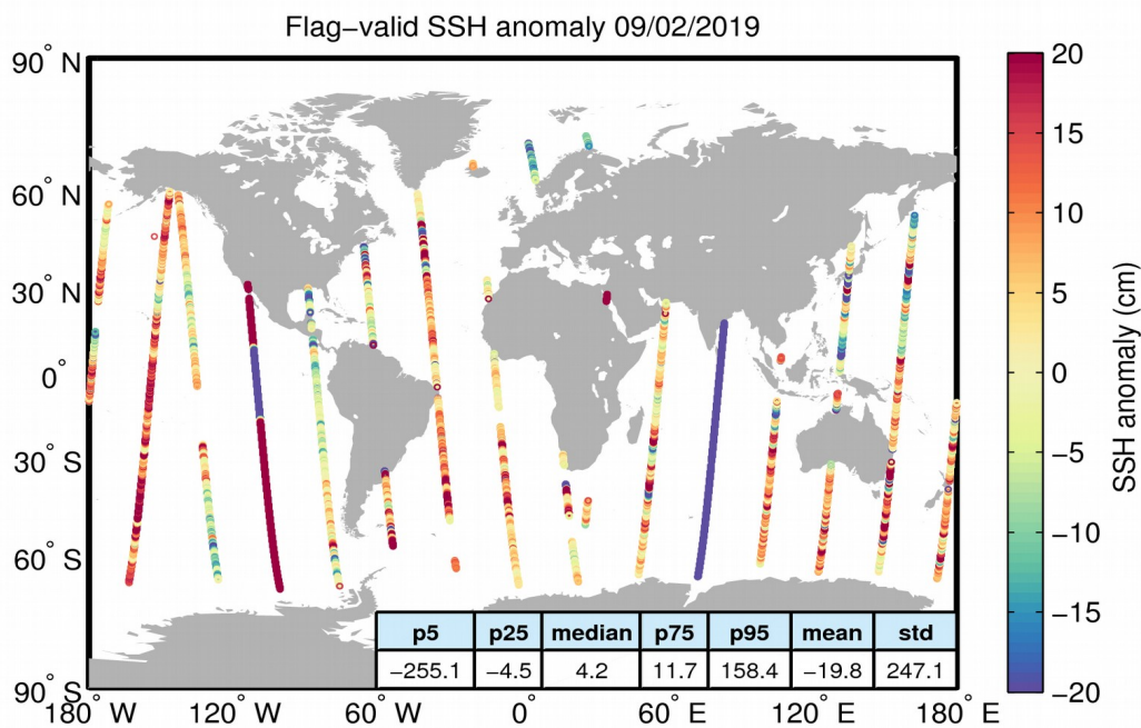
Figure 5. Geographical distribution of flag-valid 1-Hz SSH anomaly data over oceans and lakes for 09/02/2019. The statistical values shown in the table refer to the SSH anomaly in cm and are calculated over all measurements shown in the figure.
