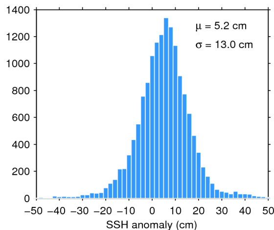
Figure 11. Histogram of science-valid SSH anomaly over oceans and lakes for 09/02/2019. The mean ( \mu ) and standard deviation ( \sigma ) are also shown. Note that values outside [-50 50] cm are excluded from the histogram for the sake of readability but not from the computation of \mu and \sigma .
