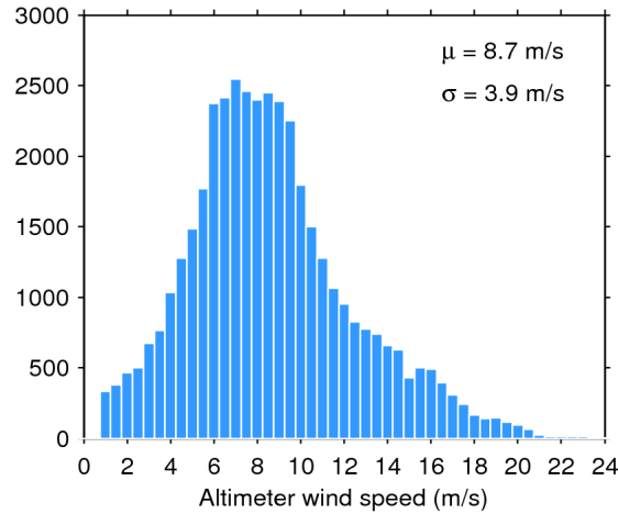
Figure 33. Histogram of flag-valid wind over oceans and lakes for 09/02/2019. The mean ( \mu ) and standard deviation ( \sigma ) are also shown. Note that values larger than 24 m/s are excluded from the histogram for the sake of readability but not from the computation of \mu and \sigma .
