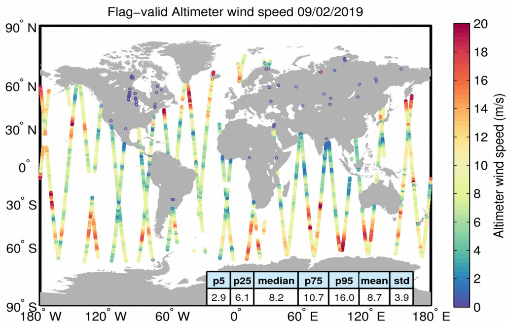
Figure 31. Geographical distribution of flag-valid wind data over oceans and lakes for 09/02/2019. The statistical values shown in the table refer to the wind in m/s and are calculated over all measurements shown in the figure.
