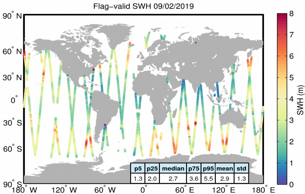
Figure 15. Geographical distribution of flag-valid SWH data over oceans and lakes for 09/02/2019. The statistical values shown in the table refer to the SWH in m and are calculated over all measurements shown in the figure.
