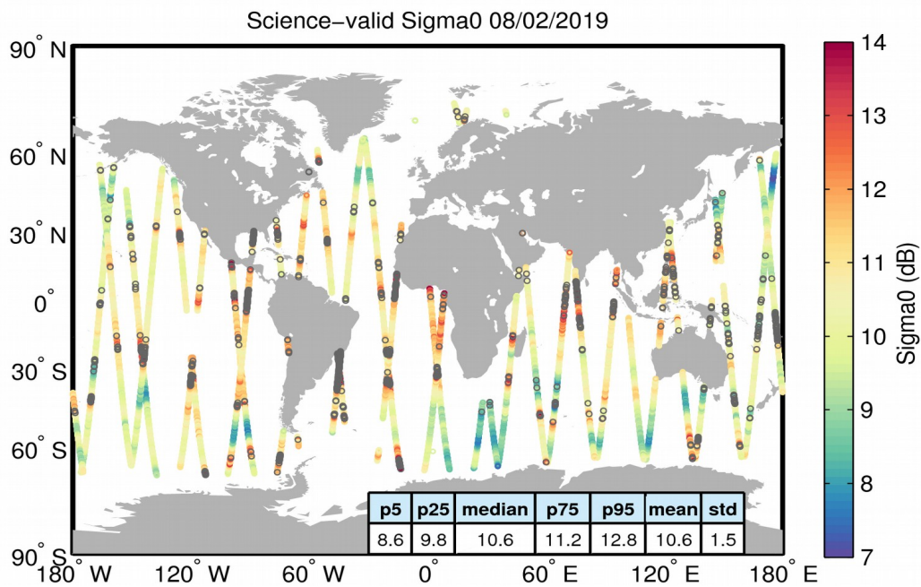
Figure 27. Geographical distribution of science-valid sigma0 data over oceans and lakes for 08/02/2019. The statistical values shown in the table refer to the sigma0 in dB and are calculated over all measurements shown in the figure. Gray circles denote records that have been rejected based on the editing criteria described in Table 4.
