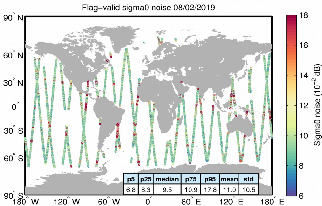
Figure 26. Geographical distribution of flag-valid 20-Hz sigma0 measurement noise over oceans and lakes for 08/02/2019. The statistical values shown in the table refer to the sigma0 noise and are calculated over all measurements shown in the figure.
