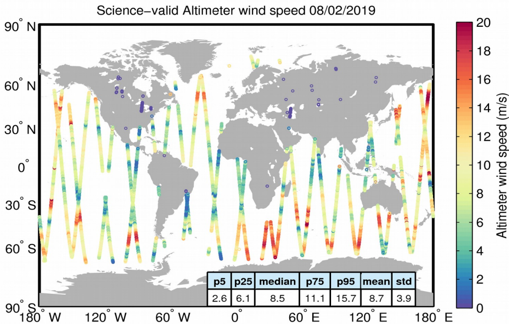
Figure 34. Geographical distribution of science-valid wind data over oceans and lakes for 08/02/2019. The statistical values shown in the table refer to the wind in m/s and are calculated over all measurements shown in the figure. Gray circles denote records that have been rejected based on the editing criteria described in Table 5.
