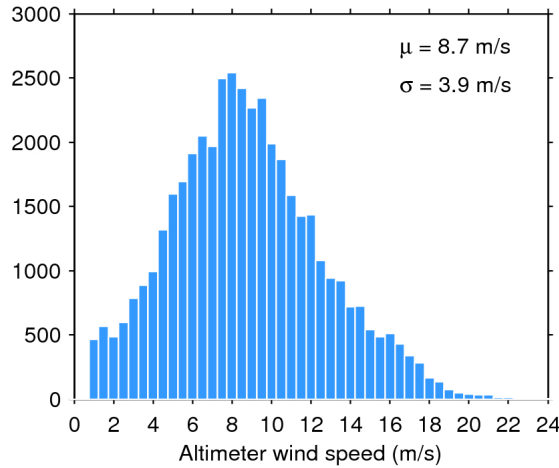
Figure 33. Histogram of flag-valid wind over oceans and lakes for 08/02/2019. The mean ( \mu ) and standard deviation ( \sigma ) are also shown. Note that values larger than 24 m/s are excluded from the histogram for the sake of readability but not from the computation of \mu and \sigma .
