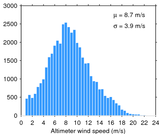
Figure 35. Histogram of science-valid wind over oceans and lakes for 08/02/2019. The mean ( \mu ) and standard deviation ( \sigma ) are also shown. Note that values larger than 24 m/s are excluded from the histogram for the sake of readability but not from the computation of \mu and \sigma .
