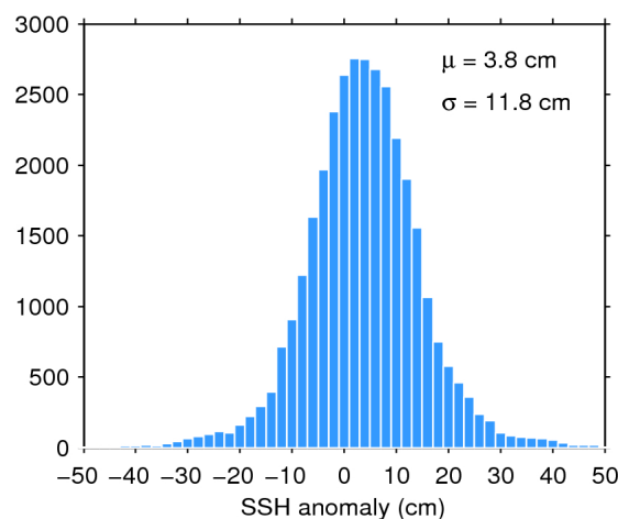
Figure 11. Histogram of science-valid SSH anomaly over oceans and lakes for 08/02/2019. The mean ( \mu ) and standard deviation ( \sigma ) are also shown. Note that values outside [-50 50] cm are excluded from the histogram for the sake of readability but not from the computation of \mu and \sigma .
