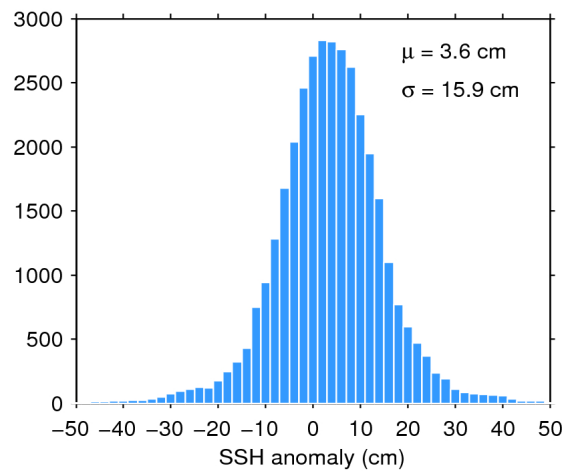
Figure 7. Histogram of flag-valid SSH anomaly over oceans and lakes for 08/02/2019. The mean ( \mu ) and standard deviation ( \sigma ) are also shown. Note that values outside [-50\ 50] cm are excluded from the histogram for the sake of readability but not from the computation of \mu and \sigma .
