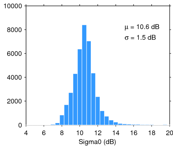
Figure 28. Histogram of science-valid sigma0 over oceans and lakes for 08/02/2019. The mean ( \mu ) and standard deviation ( \sigma ) are also shown. Note that values outside [4 20] dB are excluded from the histogram for the sake of readability but not from the computation of \mu and \sigma .
