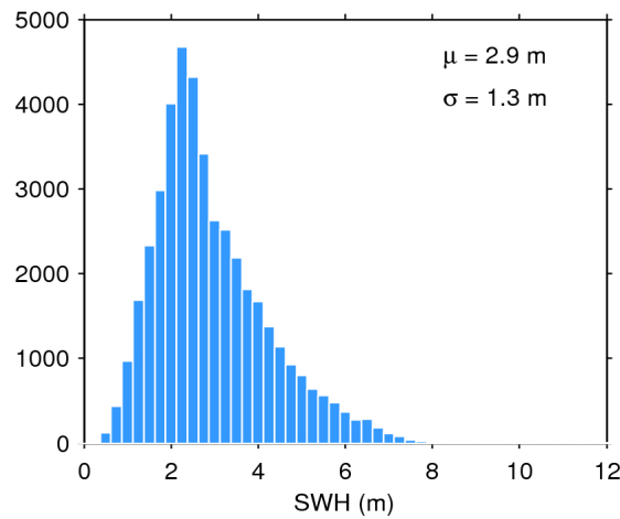
Figure 17. Histogram of flag-valid SWH over oceans and lakes for 08/02/2019. The mean ( \mu ) and standard deviation ( \sigma ) are also shown. Note that values larger than 12 m are excluded from the histogram for the sake of readability but not from the computation of \mu and \sigma .
