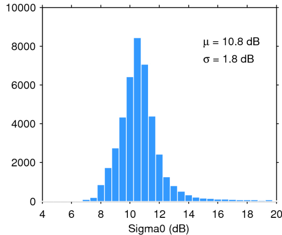
Figure 25. Histogram of flag-valid sigma0 over oceans and lakes for 08/02/2019. The mean ( \mu ) and standard deviation ( \sigma ) are also shown. Note that values outside [4 20] dB are excluded from the histogram for the sake of readability but not from the computation of \mu and \sigma .
