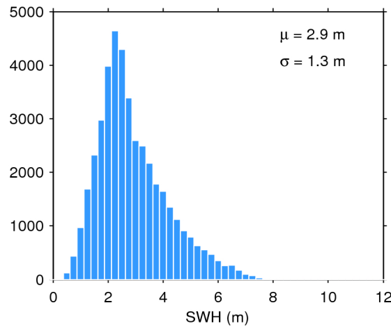
Figure 20. Histogram of science-valid SWH over oceans and lakes for 08/02/2019. The mean ( \mu ) and standard deviation ( \sigma ) are also shown. Note that values larger than 12 m are excluded from the histogram for the sake of readability but not from the computation of \mu and \sigma .
