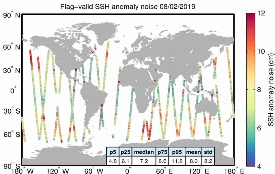
Figure 8. Geographical distribution of flag-valid 20-Hz SSH anomaly measurement noise over oceans and lakes for 08/02/2019. The statistical values shown in the table refer to the SSH anomaly noise and are calculated over all measurements shown in the figure.
