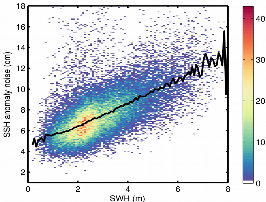
Figure 9. 2D histogram showing flag-valid SSH anomaly noise as a function of SWH for 08/02/2019. The black line denotes the median SSH anomaly noise as a function of SWH.
