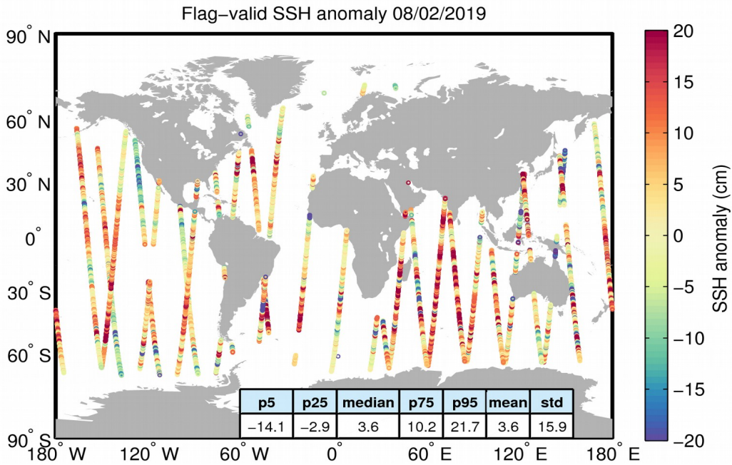
Figure 5. Geographical distribution of flag-valid 1-Hz SSH anomaly data over oceans and lakes for 08/02/2019. The statistical values shown in the table refer to the SSH anomaly in cm and are calculated over all measurements shown in the figure.
