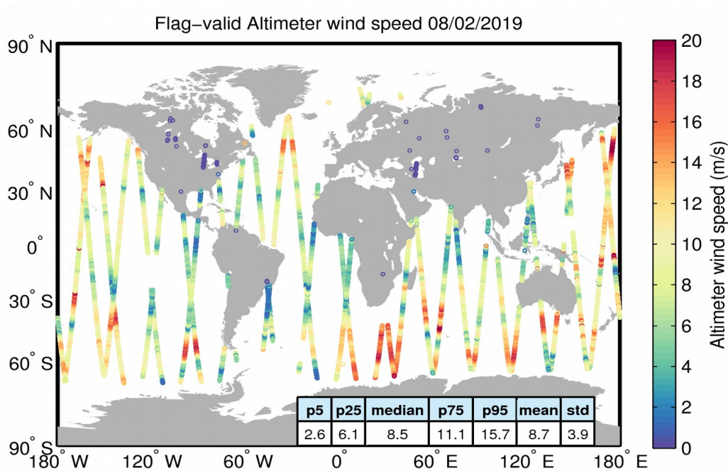
Figure 31. Geographical distribution of flag-valid wind data over oceans and lakes for 08/02/2019. The statistical values shown in the table refer to the wind in m/s and are calculated over all measurements shown in the figure.
