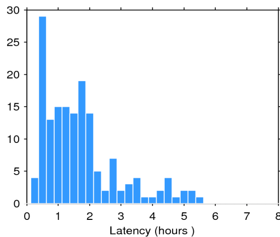
Figure 2. Histogram of the data latency for 08/02/2019. The y-axis denotes the number of files that are made available with a delay of x-hours with respect to the mean time of the records stored in the file.
