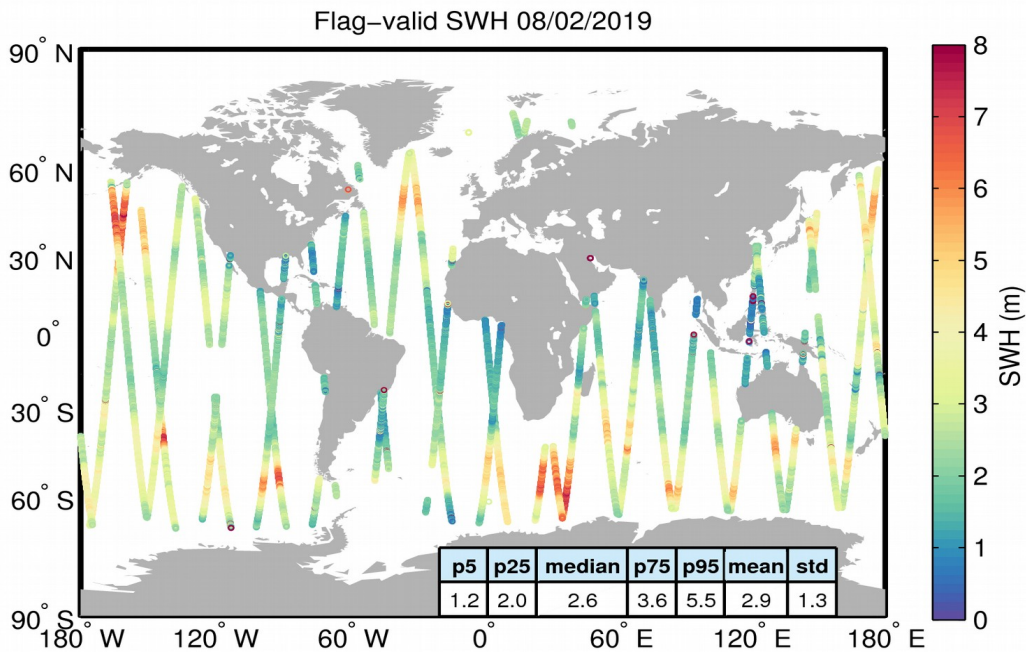
Figure 15. Geographical distribution of flag-valid SWH data over oceans and lakes for 08/02/2019. The statistical values shown in the table refer to the SWH in m and are calculated over all measurements shown in the figure.
