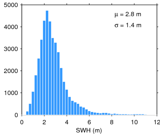
Figure 20. Histogram of science-valid SWH over oceans and lakes for 06/02/2019. The mean ( \mu ) and standard deviation ( \sigma ) are also shown. Note that values larger than 12 m are excluded from the histogram for the sake of readability but not from the computation of \mu and \sigma .
