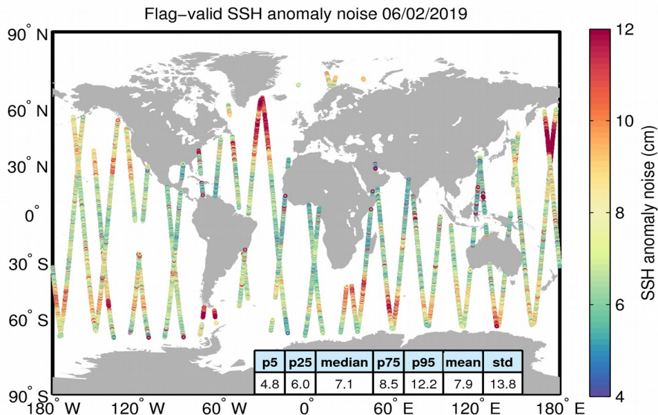
Figure 8. Geographical distribution of flag-valid 20-Hz SSH anomaly measurement noise over oceans and lakes for 06/02/2019. The statistical values shown in the table refer to the SSH anomaly noise and are calculated over all measurements shown in the figure.
