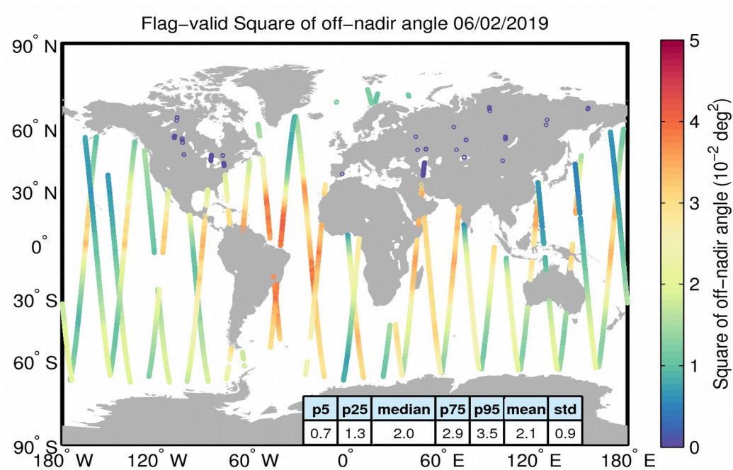
Figure 37. Geographical distribution of flag-valid mispointing data over oceans and lakes for 06/02/2019. The statistical values shown in the table refer to the mispointing in 10^{-2} \text{ deg}^2 and are calculated over all measurements shown in the figure.
