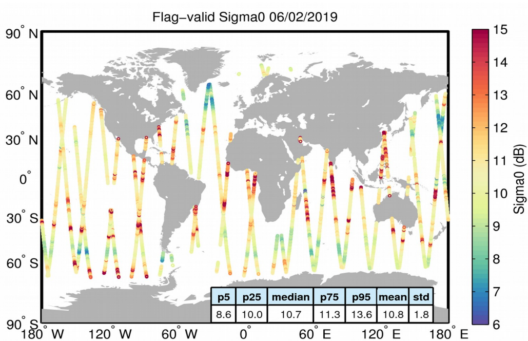
Figure 23. Geographical distribution of flag-valid sigma0 data over oceans and lakes for 06/02/2019. The statistical values shown in the table refer to the sigma0 in dB and are calculated over all measurements shown in the figure.
