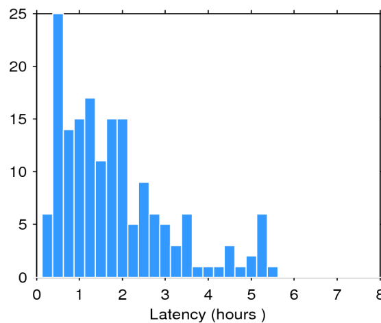
Figure 2. Histogram of the data latency for 06/02/2019. The y-axis denotes the number of files that are made available with a delay of x-hours with respect to the mean time of the records stored in the file.
