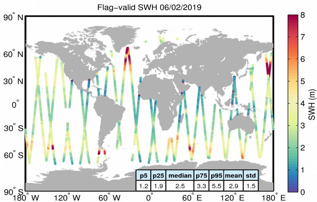
Figure 15. Geographical distribution of flag-valid SWH data over oceans and lakes for 06/02/2019. The statistical values shown in the table refer to the SWH in m and are calculated over all measurements shown in the figure.
