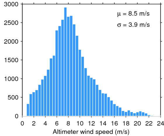
Figure 33. Histogram of flag-valid wind over oceans and lakes for 06/02/2019. The mean ( \mu ) and standard deviation ( \sigma ) are also shown. Note that values larger than 24 m/s are excluded from the histogram for the sake of readability but not from the computation of \mu and \sigma .
