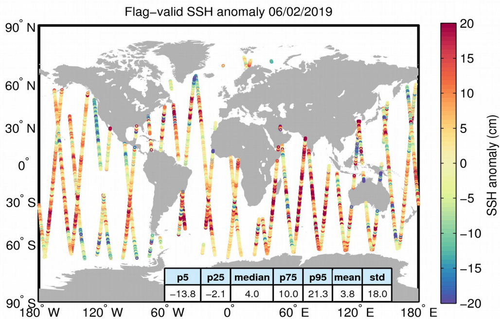
Figure 5. Geographical distribution of flag-valid 1-Hz SSH anomaly data over oceans and lakes for 06/02/2019. The statistical values shown in the table refer to the SSH anomaly in cm and are calculated over all measurements shown in the figure.
