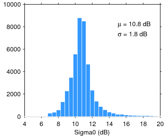
Figure 25. Histogram of flag-valid sigma0 over oceans and lakes for 06/02/2019. The mean ( \mu ) and standard deviation ( \sigma ) are also shown. Note that values outside [4 20] dB are excluded from the histogram for the sake of readability but not from the computation of \mu and \sigma .
