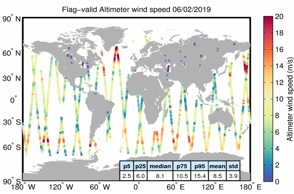
Figure 31. Geographical distribution of flag-valid wind data over oceans and lakes for 06/02/2019. The statistical values shown in the table refer to the wind in m/s and are calculated over all measurements shown in the figure.
