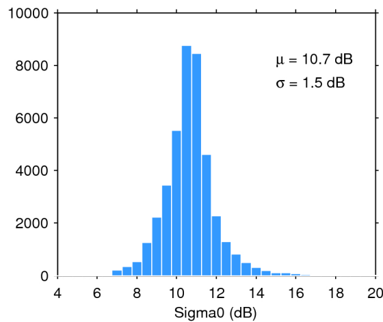
Figure 28. Histogram of science-valid sigma0 over oceans and lakes for 06/02/2019. The mean ( \mu ) and standard deviation ( \sigma ) are also shown. Note that values outside [4 20] dB are excluded from the histogram for the sake of readability but not from the computation of \mu and \sigma .
