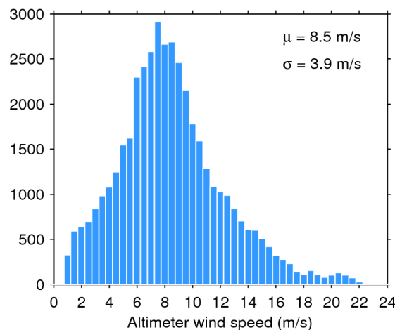
Figure 35. Histogram of science-valid wind over oceans and lakes for 06/02/2019. The mean ( \mu ) and standard deviation ( \sigma ) are also shown. Note that values larger than 24 m/s are excluded from the histogram for the sake of readability but not from the computation of \mu and \sigma .
