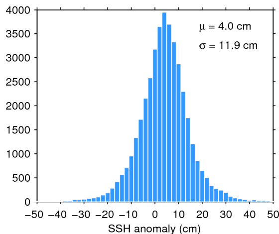
Figure 11. Histogram of science-valid SSH anomaly over oceans and lakes for 06/02/2019. The mean ( \mu ) and standard deviation ( \sigma ) are also shown. Note that values outside [-50 50] cm are excluded from the histogram for the sake of readability but not from the computation of \mu and \sigma .
