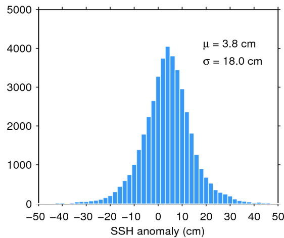
Figure 7. Histogram of flag-valid SSH anomaly over oceans and lakes for 06/02/2019. The mean ( \mu ) and standard deviation ( \sigma ) are also shown. Note that values outside [-50\ 50] cm are excluded from the histogram for the sake of readability but not from the computation of \mu and \sigma .
