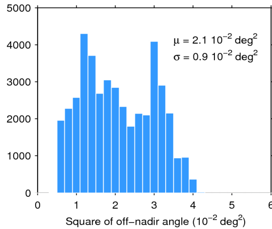
Figure 39. Histogram of flag-valid mispointing over oceans and lakes for 06/02/2019. The mean ( \mu ) and standard deviation ( \sigma ) are also shown. Note that values larger than 6 \cdot 10^{-2} \text{ deg}^2 are excluded from the histogram for the sake of readability but not from the computation of \mu and \sigma .
