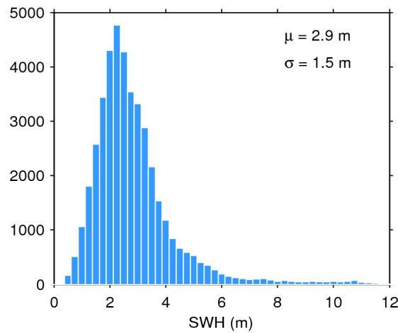
Figure 17. Histogram of flag-valid SWH over oceans and lakes for 06/02/2019. The mean ( \mu ) and standard deviation ( \sigma ) are also shown. Note that values larger than 12 m are excluded from the histogram for the sake of readability but not from the computation of \mu and \sigma .
