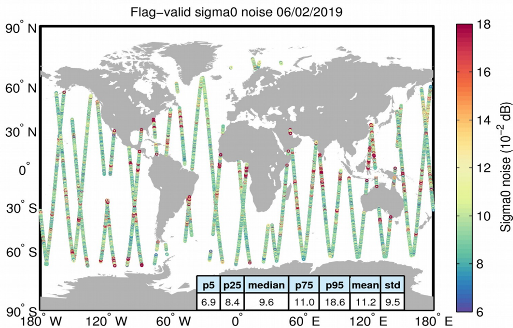
Figure 26. Geographical distribution of flag-valid 20-Hz sigma0 measurement noise over oceans and lakes for 06/02/2019. The statistical values shown in the table refer to the sigma0 noise and are calculated over all measurements shown in the figure.
