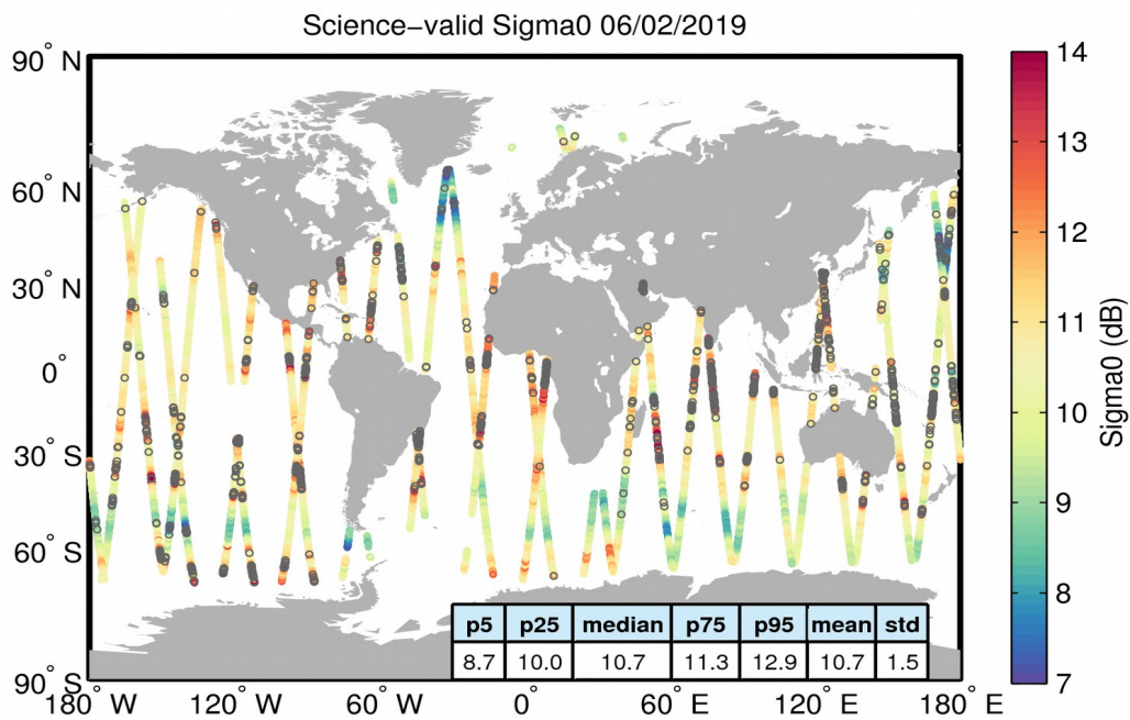
Figure 27. Geographical distribution of science-valid sigma0 data over oceans and lakes for 06/02/2019. The statistical values shown in the table refer to the sigma0 in dB and are calculated over all measurements shown in the figure. Gray circles denote records that have been rejected based on the editing criteria described in Table 4.
