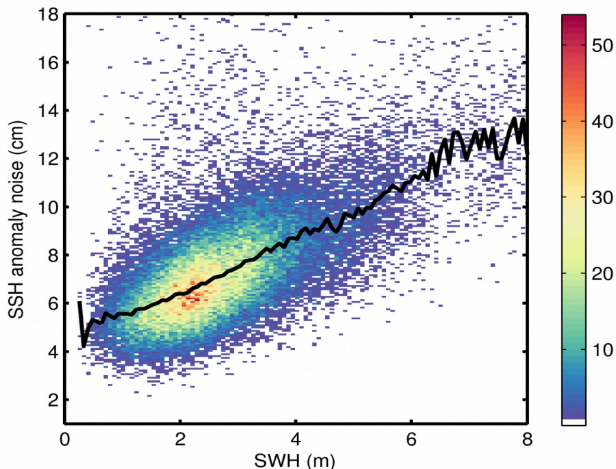
Figure 9. 2D histogram showing flag-valid SSH anomaly noise as a function of SWH for 06/02/2019. The black line denotes the median SSH anomaly noise as a function of SWH.
