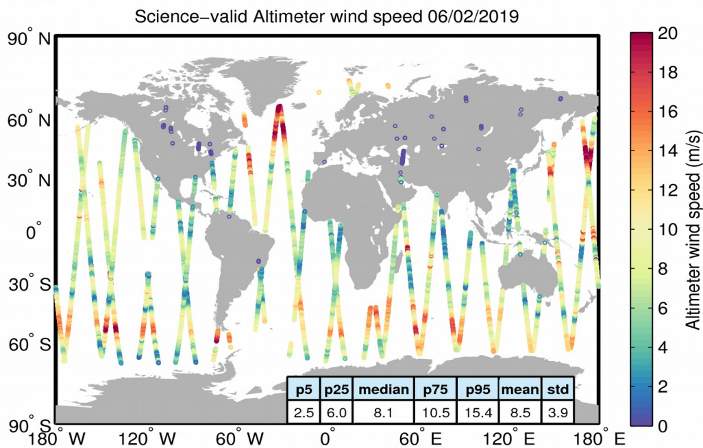
Figure 34. Geographical distribution of science-valid wind data over oceans and lakes for 06/02/2019. The statistical values shown in the table refer to the wind in m/s and are calculated over all measurements shown in the figure. Gray circles denote records that have been rejected based on the editing criteria described in Table 5.
