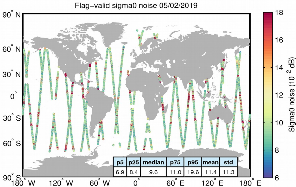
Figure 26. Geographical distribution of flag-valid 20-Hz sigma0 measurement noise over oceans and lakes for 05/02/2019. The statistical values shown in the table refer to the sigma0 noise and are calculated over all measurements shown in the figure.
