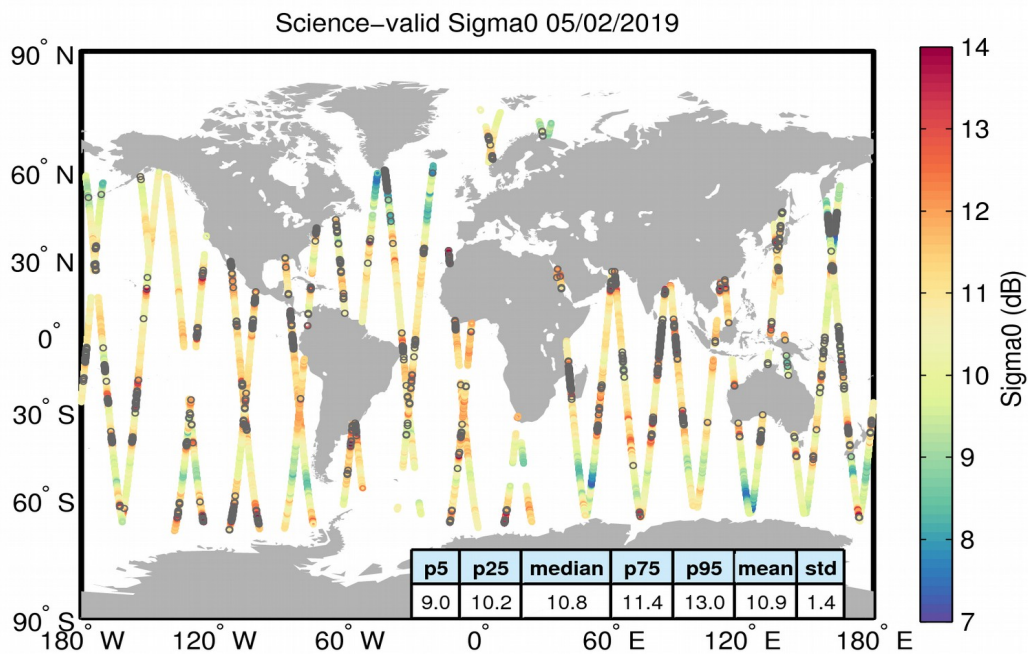
Figure 27. Geographical distribution of science-valid sigma0 data over oceans and lakes for 05/02/2019. The statistical values shown in the table refer to the sigma0 in dB and are calculated over all measurements shown in the figure. Gray circles denote records that have been rejected based on the editing criteria described in Table 4.
