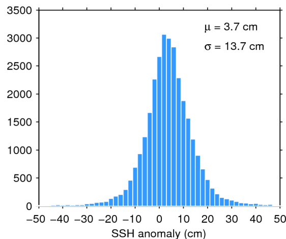
Figure 11. Histogram of science-valid SSH anomaly over oceans and lakes for 05/02/2019. The mean ( \mu ) and standard deviation ( \sigma ) are also shown. Note that values outside [-50 50] cm are excluded from the histogram for the sake of readability but not from the computation of \mu and \sigma .
