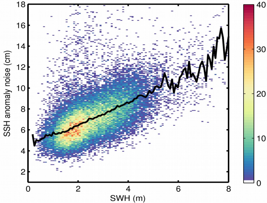
Figure 9. 2D histogram showing flag-valid SSH anomaly noise as a function of SWH for 05/02/2019. The black line denotes the median SSH anomaly noise as a function of SWH.
