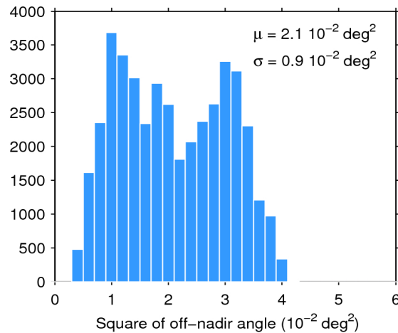
Figure 39. Histogram of flag-valid mispointing over oceans and lakes for 05/02/2019. The mean ( \mu ) and standard deviation ( \sigma ) are also shown. Note that values larger than 6 \cdot 10^{-2} \text{ deg}^2 are excluded from the histogram for the sake of readability but not from the computation of \mu and \sigma .
