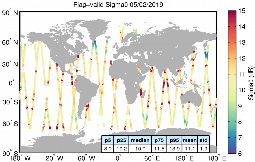
Figure 23. Geographical distribution of flag-valid sigma0 data over oceans and lakes for 05/02/2019. The statistical values shown in the table refer to the sigma0 in dB and are calculated over all measurements shown in the figure.
