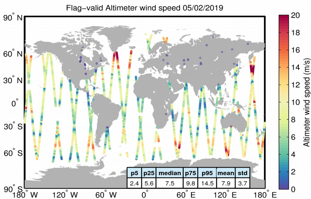
Figure 31. Geographical distribution of flag-valid wind data over oceans and lakes for 05/02/2019. The statistical values shown in the table refer to the wind in m/s and are calculated over all measurements shown in the figure.
