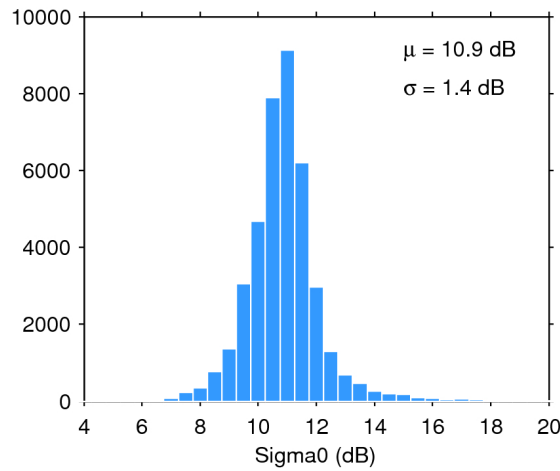
Figure 28. Histogram of science-valid sigma0 over oceans and lakes for 05/02/2019. The mean ( \mu ) and standard deviation ( \sigma ) are also shown. Note that values outside [4 20] dB are excluded from the histogram for the sake of readability but not from the computation of \mu and \sigma .
