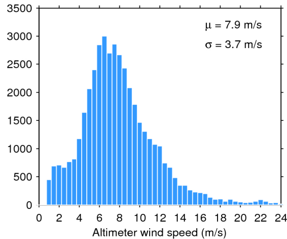
Figure 33. Histogram of flag-valid wind over oceans and lakes for 05/02/2019. The mean ( \mu ) and standard deviation ( \sigma ) are also shown. Note that values larger than 24 m/s are excluded from the histogram for the sake of readability but not from the computation of \mu and \sigma .
