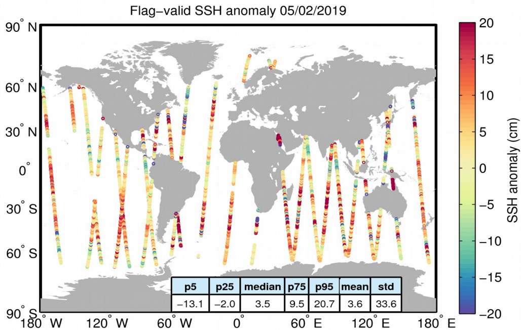
Figure 5. Geographical distribution of flag-valid 1-Hz SSH anomaly data over oceans and lakes for 05/02/2019. The statistical values shown in the table refer to the SSH anomaly in cm and are calculated over all measurements shown in the figure.
