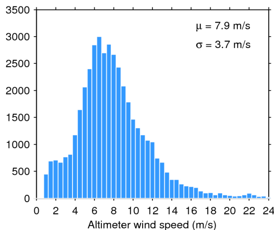
Figure 35. Histogram of science-valid wind over oceans and lakes for 05/02/2019. The mean ( \mu ) and standard deviation ( \sigma ) are also shown. Note that values larger than 24 m/s are excluded from the histogram for the sake of readability but not from the computation of \mu and \sigma .
