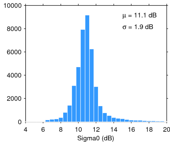
Figure 25. Histogram of flag-valid sigma0 over oceans and lakes for 05/02/2019. The mean ( \mu ) and standard deviation ( \sigma ) are also shown. Note that values outside [4 20] dB are excluded from the histogram for the sake of readability but not from the computation of \mu and \sigma .
