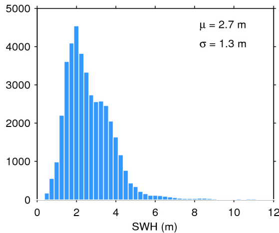
Figure 20. Histogram of science-valid SWH over oceans and lakes for 05/02/2019. The mean ( \mu ) and standard deviation ( \sigma ) are also shown. Note that values larger than 12 m are excluded from the histogram for the sake of readability but not from the computation of \mu and \sigma .
