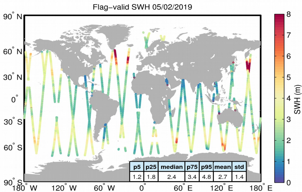
Figure 15. Geographical distribution of flag-valid SWH data over oceans and lakes for 05/02/2019. The statistical values shown in the table refer to the SWH in m and are calculated over all measurements shown in the figure.
