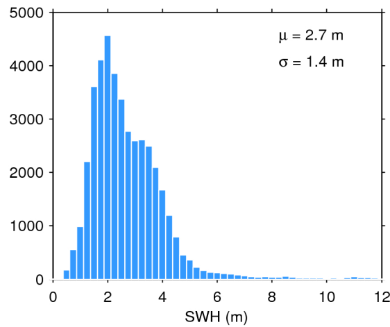
Figure 17. Histogram of flag-valid SWH over oceans and lakes for 05/02/2019. The mean ( \mu ) and standard deviation ( \sigma ) are also shown. Note that values larger than 12 m are excluded from the histogram for the sake of readability but not from the computation of \mu and \sigma .
