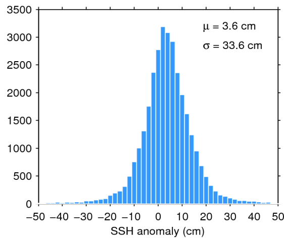
Figure 7. Histogram of flag-valid SSH anomaly over oceans and lakes for 05/02/2019. The mean ( \mu ) and standard deviation ( \sigma ) are also shown. Note that values outside [-50 50] cm are excluded from the histogram for the sake of readability but not from the computation of \mu and \sigma .
