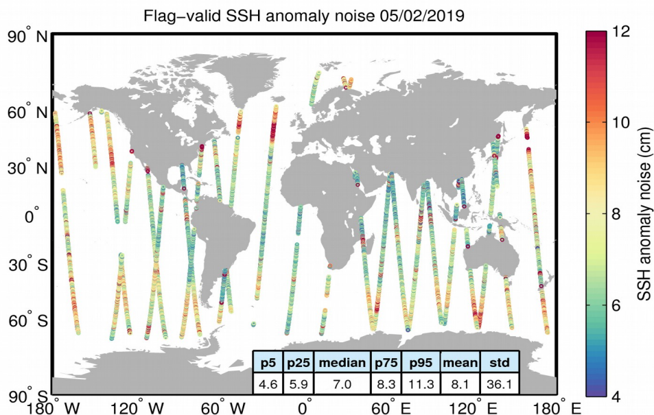
Figure 8. Geographical distribution of flag-valid 20-Hz SSH anomaly measurement noise over oceans and lakes for 05/02/2019. The statistical values shown in the table refer to the SSH anomaly noise and are calculated over all measurements shown in the figure.
