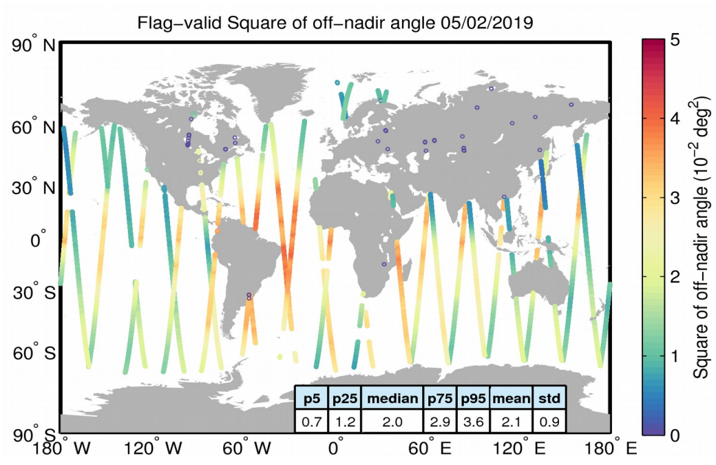
Figure 37. Geographical distribution of flag-valid mispointing data over oceans and lakes for 05/02/2019. The statistical values shown in the table refer to the mispointing in 10^{-2} \text{ deg}^2 and are calculated over all measurements shown in the figure.
