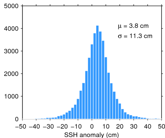
Figure 11. Histogram of science-valid SSH anomaly over oceans and lakes for 04/02/2019. The mean ( \mu ) and standard deviation ( \sigma ) are also shown. Note that values outside [-50 50] cm are excluded from the histogram for the sake of readability but not from the computation of \mu and \sigma .
