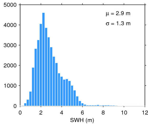
Figure 17. Histogram of flag-valid SWH over oceans and lakes for 04/02/2019. The mean ( \mu ) and standard deviation ( \sigma ) are also shown. Note that values larger than 12 m are excluded from the histogram for the sake of readability but not from the computation of \mu and \sigma .
