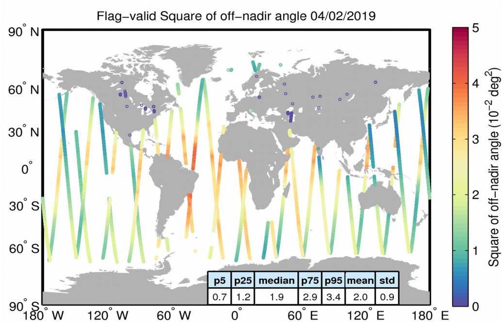
Figure 37. Geographical distribution of flag-valid mispointing data over oceans and lakes for 04/02/2019. The statistical values shown in the table refer to the mispointing in 10^{-2} deg 2 and are calculated over all measurements shown in the figure.
