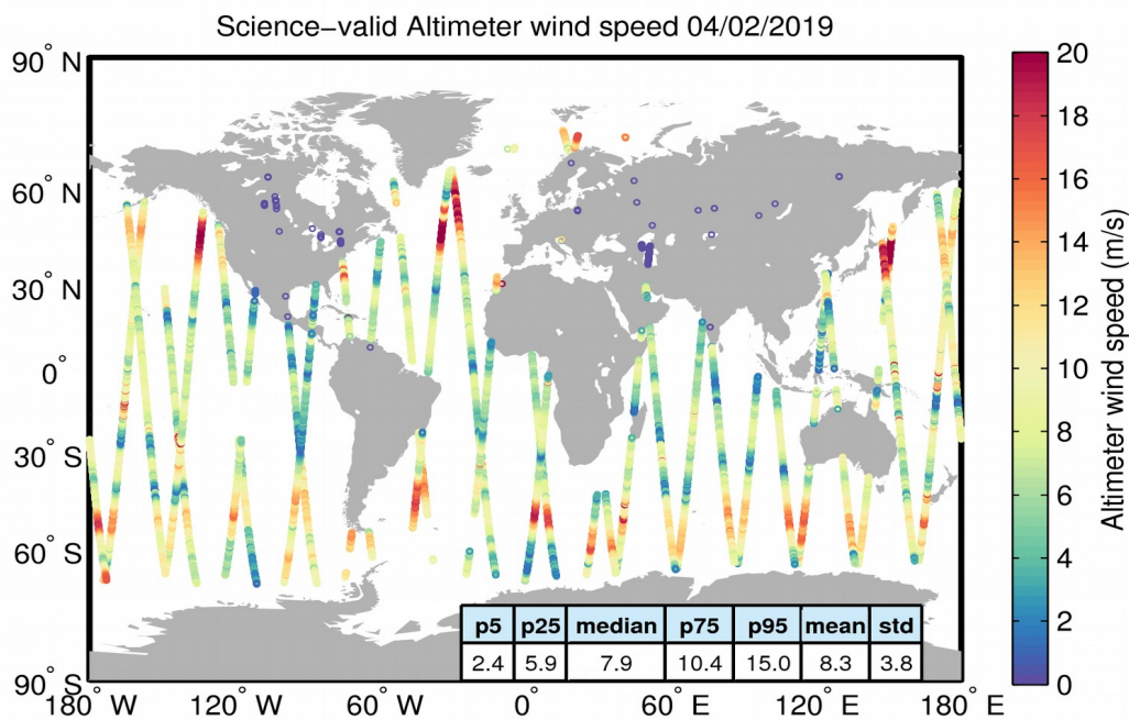
Figure 34. Geographical distribution of science-valid wind data over oceans and lakes for 04/02/2019. The statistical values shown in the table refer to the wind in m/s and are calculated over all measurements shown in the figure. Gray circles denote records that have been rejected based on the editing criteria described in Table 5.
