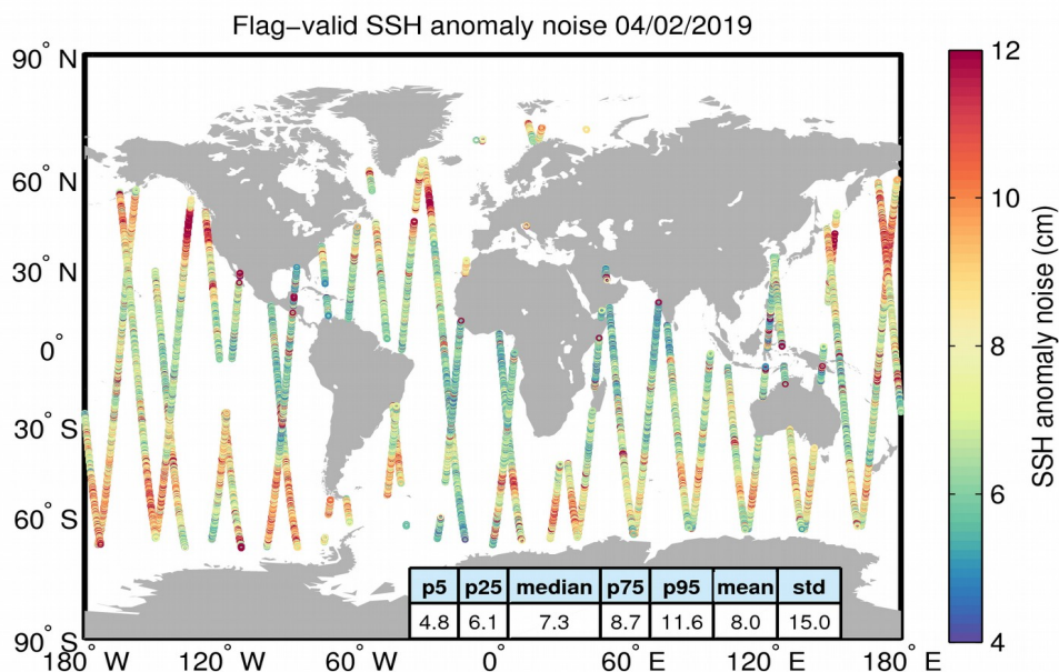
Figure 8. Geographical distribution of flag-valid 20-Hz SSH anomaly measurement noise over oceans and lakes for 04/02/2019. The statistical values shown in the table refer to the SSH anomaly noise and are calculated over all measurements shown in the figure.
