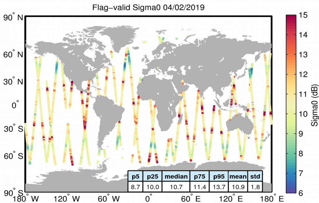
Figure 23. Geographical distribution of flag-valid sigma0 data over oceans and lakes for 04/02/2019. The statistical values shown in the table refer to the sigma0 in dB and are calculated over all measurements shown in the figure.
