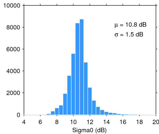
Figure 28. Histogram of science-valid sigma0 over oceans and lakes for 04/02/2019. The mean ( \mu ) and standard deviation ( \sigma ) are also shown. Note that values outside [4 20] dB are excluded from the histogram for the sake of readability but not from the computation of \mu and \sigma .
