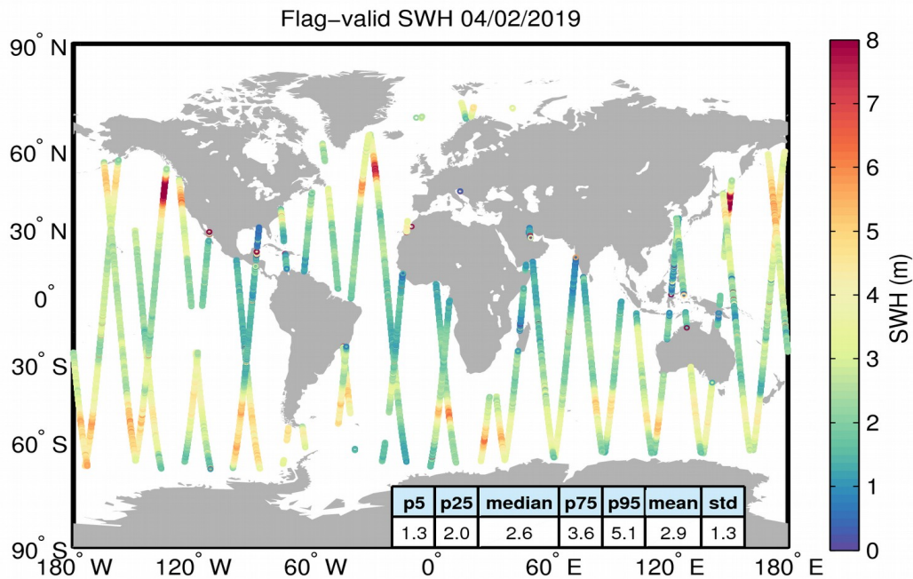
Figure 15. Geographical distribution of flag-valid SWH data over oceans and lakes for 04/02/2019. The statistical values shown in the table refer to the SWH in m and are calculated over all measurements shown in the figure.
