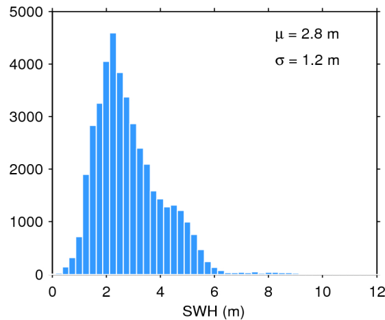
Figure 20. Histogram of science-valid SWH over oceans and lakes for 04/02/2019. The mean ( \mu ) and standard deviation ( \sigma ) are also shown. Note that values larger than 12 m are excluded from the histogram for the sake of readability but not from the computation of \mu and \sigma .
