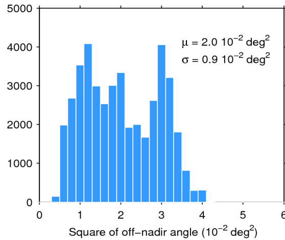
Figure 39. Histogram of flag-valid mispointing over oceans and lakes for 04/02/2019. The mean ( \mu ) and standard deviation ( \sigma ) are also shown. Note that values larger than 6 \cdot 10^{-2} \text{ deg}^2 are excluded from the histogram for the sake of readability but not from the computation of \mu and \sigma .
