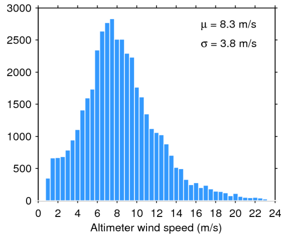
Figure 33. Histogram of flag-valid wind over oceans and lakes for 04/02/2019. The mean ( \mu ) and standard deviation ( \sigma ) are also shown. Note that values larger than 24 m/s are excluded from the histogram for the sake of readability but not from the computation of \mu and \sigma .
