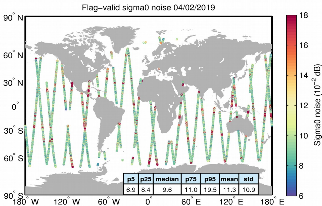
Figure 26. Geographical distribution of flag-valid 20-Hz sigma0 measurement noise over oceans and lakes for 04/02/2019. The statistical values shown in the table refer to the sigma0 noise and are calculated over all measurements shown in the figure.
