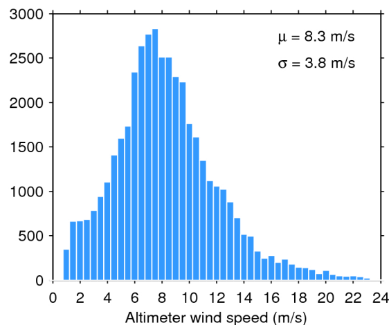
Figure 35. Histogram of science-valid wind over oceans and lakes for 04/02/2019. The mean ( \mu ) and standard deviation ( \sigma ) are also shown. Note that values larger than 24 m/s are excluded from the histogram for the sake of readability but not from the computation of \mu and \sigma .
