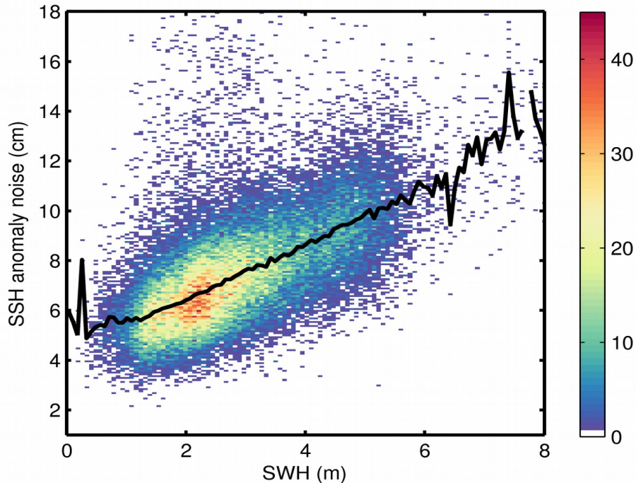
Figure 9. 2D histogram showing flag-valid SSH anomaly noise as a function of SWH for 04/02/2019. The black line denotes the median SSH anomaly noise as a function of SWH.
