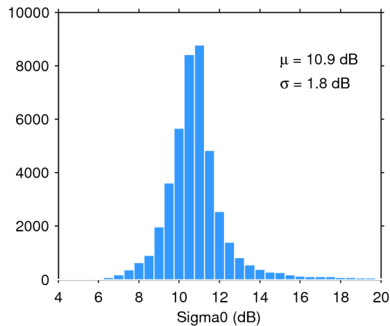
Figure 25. Histogram of flag-valid sigma0 over oceans and lakes for 04/02/2019. The mean ( \mu ) and standard deviation ( \sigma ) are also shown. Note that values outside [4 20] dB are excluded from the histogram for the sake of readability but not from the computation of \mu and \sigma .
