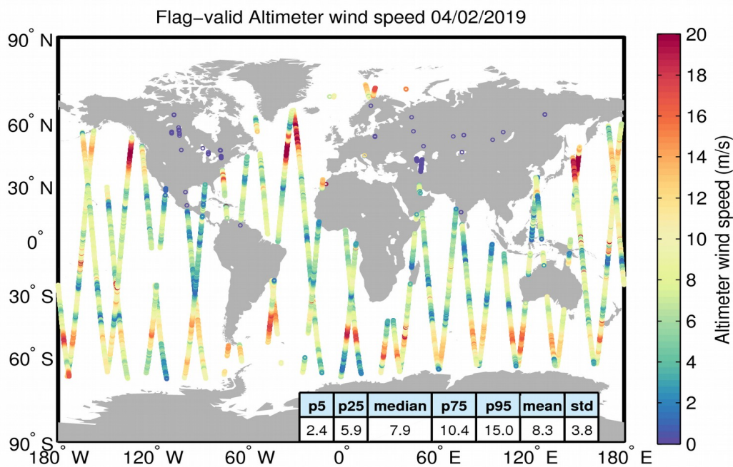
Figure 31. Geographical distribution of flag-valid wind data over oceans and lakes for 04/02/2019. The statistical values shown in the table refer to the wind in m/s and are calculated over all measurements shown in the figure.
