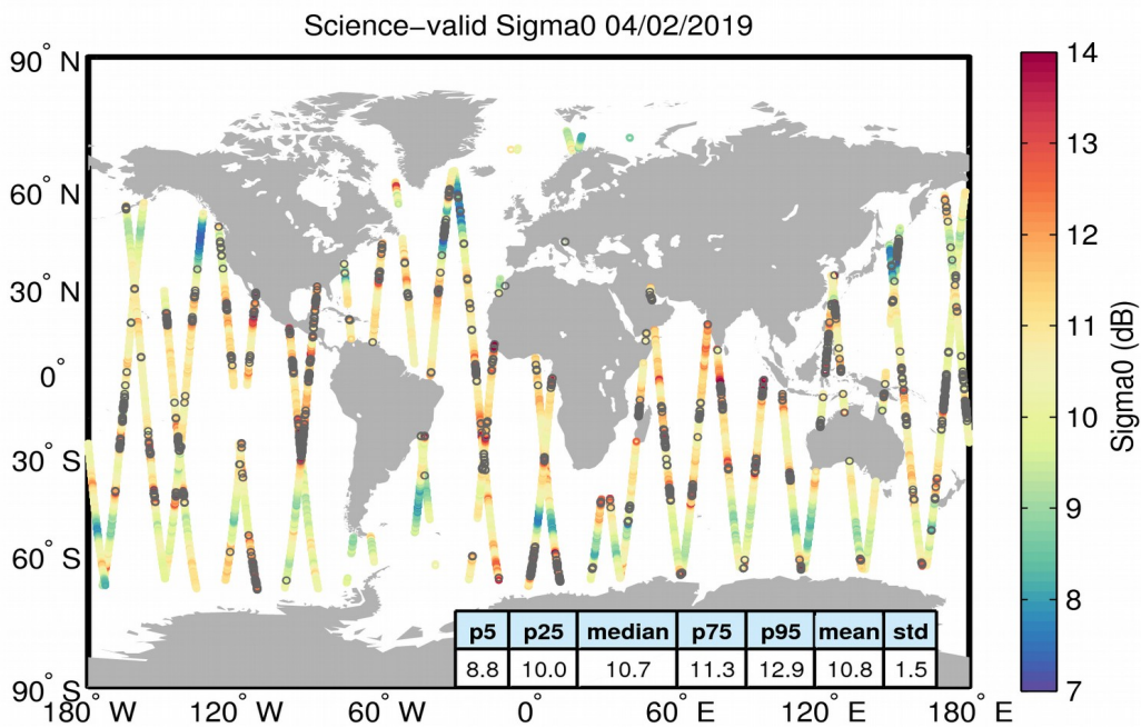
Figure 27. Geographical distribution of science-valid sigma0 data over oceans and lakes for 04/02/2019. The statistical values shown in the table refer to the sigma0 in dB and are calculated over all measurements shown in the figure. Gray circles denote records that have been rejected based on the editing criteria described in Table 4.
