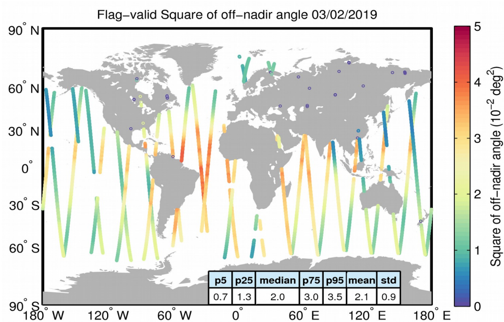
Figure 37. Geographical distribution of flag-valid mispointing data over oceans and lakes for 03/02/2019. The statistical values shown in the table refer to the mispointing in 10^{-2} deg 2 and are calculated over all measurements shown in the figure.
