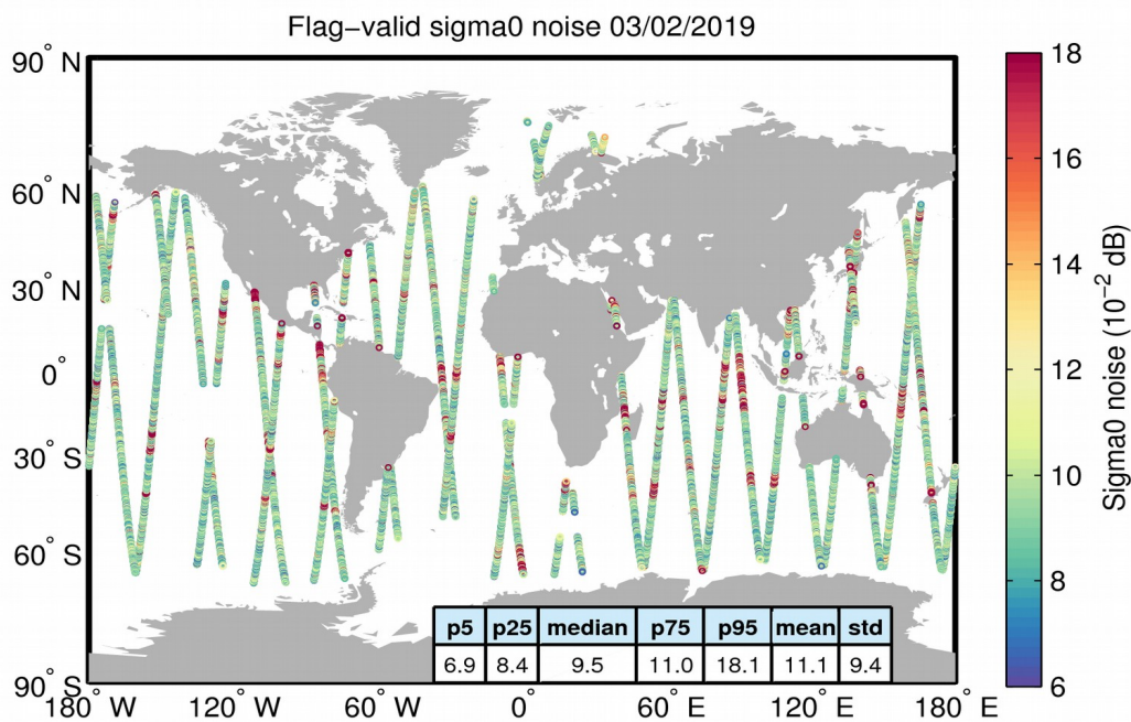
Figure 26. Geographical distribution of flag-valid 20-Hz sigma0 measurement noise over oceans and lakes for 03/02/2019. The statistical values shown in the table refer to the sigma0 noise and are calculated over all measurements shown in the figure.
