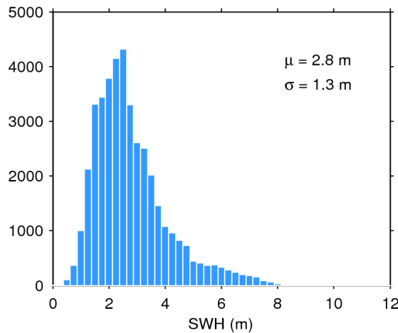
Figure 20. Histogram of science-valid SWH over oceans and lakes for 03/02/2019. The mean ( \mu ) and standard deviation ( \sigma ) are also shown. Note that values larger than 12 m are excluded from the histogram for the sake of readability but not from the computation of \mu and \sigma .
