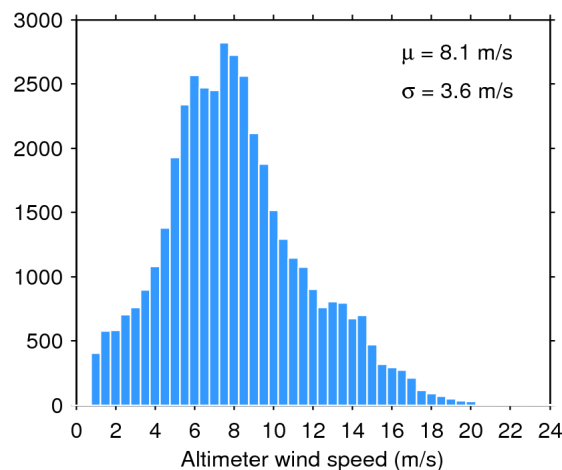
Figure 35. Histogram of science-valid wind over oceans and lakes for 03/02/2019. The mean ( \mu ) and standard deviation ( \sigma ) are also shown. Note that values larger than 24 m/s are excluded from the histogram for the sake of readability but not from the computation of \mu and \sigma .
