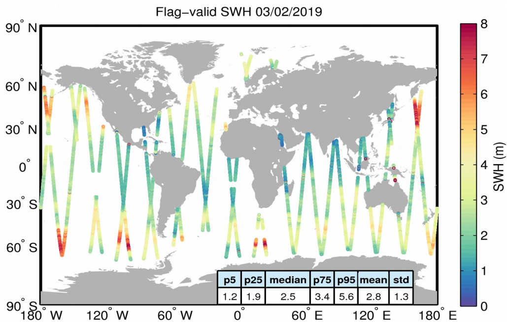
Figure 15. Geographical distribution of flag-valid SWH data over oceans and lakes for 03/02/2019. The statistical values shown in the table refer to the SWH in m and are calculated over all measurements shown in the figure.
