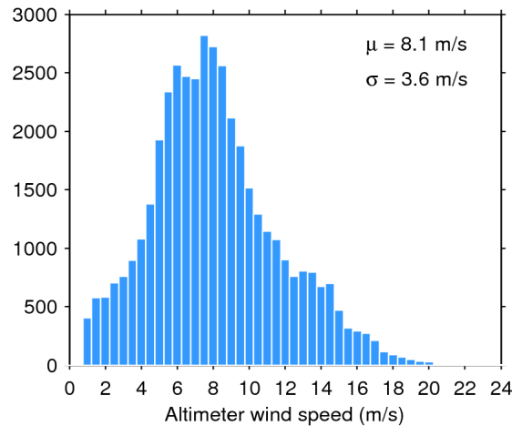
Figure 33. Histogram of flag-valid wind over oceans and lakes for 03/02/2019. The mean ( \mu ) and standard deviation ( \sigma ) are also shown. Note that values larger than 24 m/s are excluded from the histogram for the sake of readability but not from the computation of \mu and \sigma .
