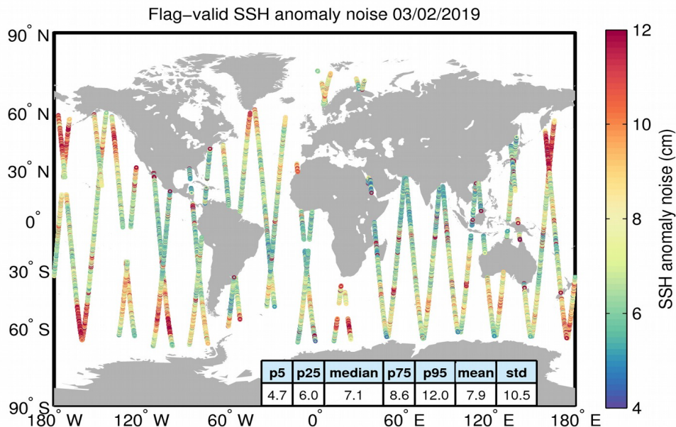
Figure 8. Geographical distribution of flag-valid 20-Hz SSH anomaly measurement noise over oceans and lakes for 03/02/2019. The statistical values shown in the table refer to the SSH anomaly noise and are calculated over all measurements shown in the figure.
