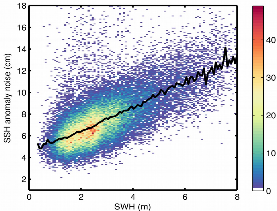
Figure 9. 2D histogram showing flag-valid SSH anomaly noise as a function of SWH for 03/02/2019. The black line denotes the median SSH anomaly noise as a function of SWH.
