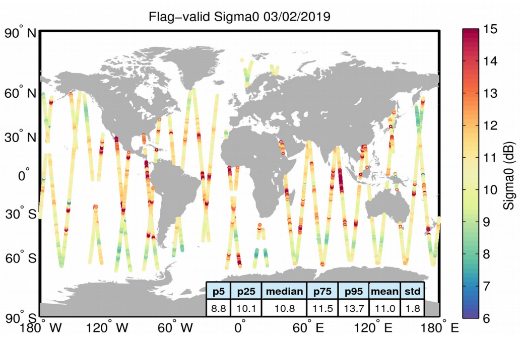
Figure 23. Geographical distribution of flag-valid sigma0 data over oceans and lakes for 03/02/2019. The statistical values shown in the table refer to the sigma0 in dB and are calculated over all measurements shown in the figure.
