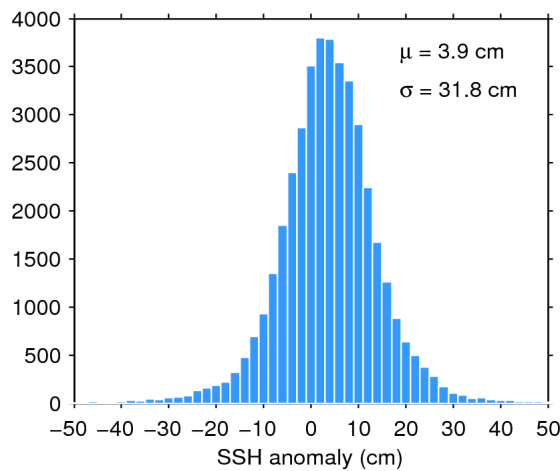
Figure 7. Histogram of flag-valid SSH anomaly over oceans and lakes for 03/02/2019. The mean ( \mu ) and standard deviation ( \sigma ) are also shown. Note that values outside [-50\ 50] cm are excluded from the histogram for the sake of readability but not from the computation of \mu and \sigma .
