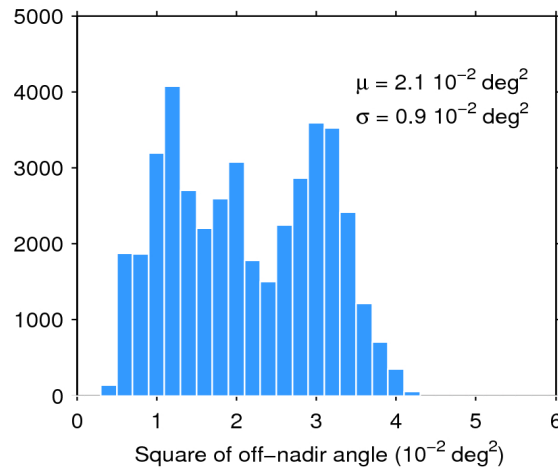
Figure 39. Histogram of flag-valid mispointing over oceans and lakes for 03/02/2019. The mean ( \mu ) and standard deviation ( \sigma ) are also shown. Note that values larger than 6 \cdot 10^{-2} \text{ deg}^2 are excluded from the histogram for the sake of readability but not from the computation of \mu and \sigma .
