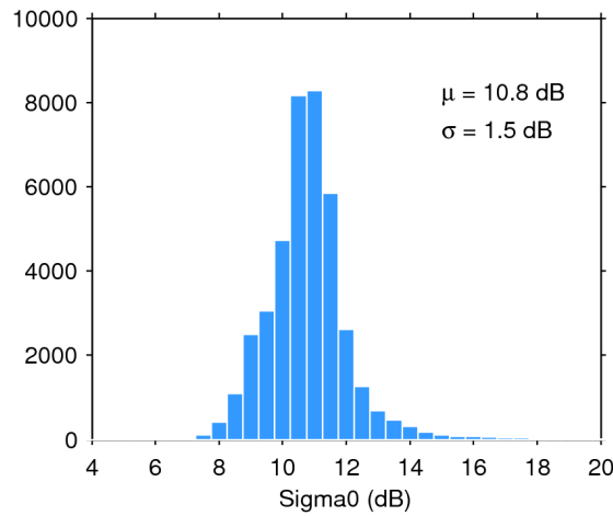
Figure 28. Histogram of science-valid sigma0 over oceans and lakes for 03/02/2019. The mean ( \mu ) and standard deviation ( \sigma ) are also shown. Note that values outside [4 20] dB are excluded from the histogram for the sake of readability but not from the computation of \mu and \sigma .
