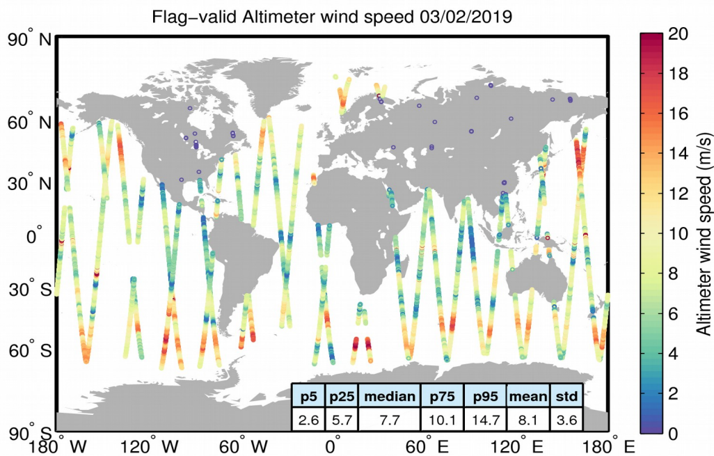
Figure 31. Geographical distribution of flag-valid wind data over oceans and lakes for 03/02/2019. The statistical values shown in the table refer to the wind in m/s and are calculated over all measurements shown in the figure.
