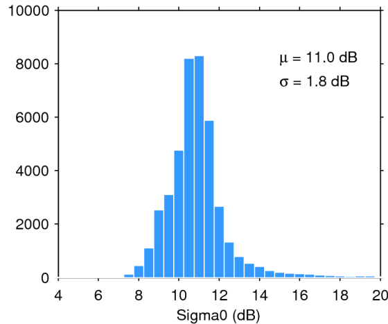
Figure 25. Histogram of flag-valid sigma0 over oceans and lakes for 03/02/2019. The mean ( \mu ) and standard deviation ( \sigma ) are also shown. Note that values outside [4 20] dB are excluded from the histogram for the sake of readability but not from the computation of \mu and \sigma .
