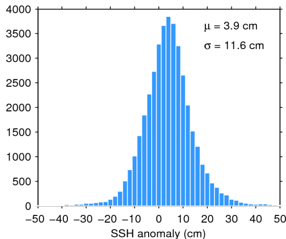
Figure 11. Histogram of science-valid SSH anomaly over oceans and lakes for 01/02/2019. The mean ( \mu ) and standard deviation ( \sigma ) are also shown. Note that values outside [-50 50] cm are excluded from the histogram for the sake of readability but not from the computation of \mu and \sigma .
