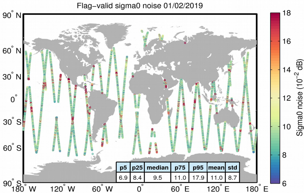
Figure 26. Geographical distribution of flag-valid 20-Hz sigma0 measurement noise over oceans and lakes for 01/02/2019. The statistical values shown in the table refer to the sigma0 noise and are calculated over all measurements shown in the figure.
