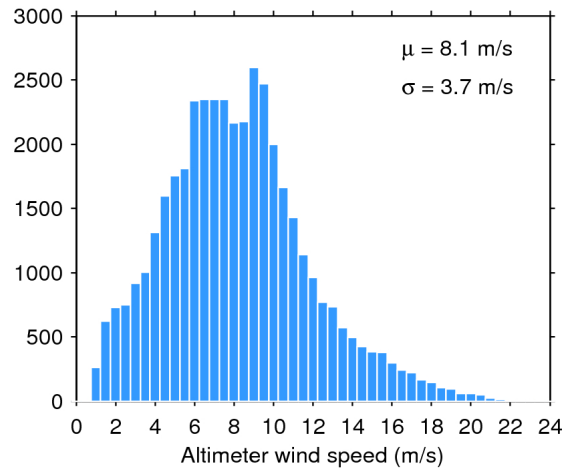
Figure 33. Histogram of flag-valid wind over oceans and lakes for 01/02/2019. The mean ( \mu ) and standard deviation ( \sigma ) are also shown. Note that values larger than 24 m/s are excluded from the histogram for the sake of readability but not from the computation of \mu and \sigma .
