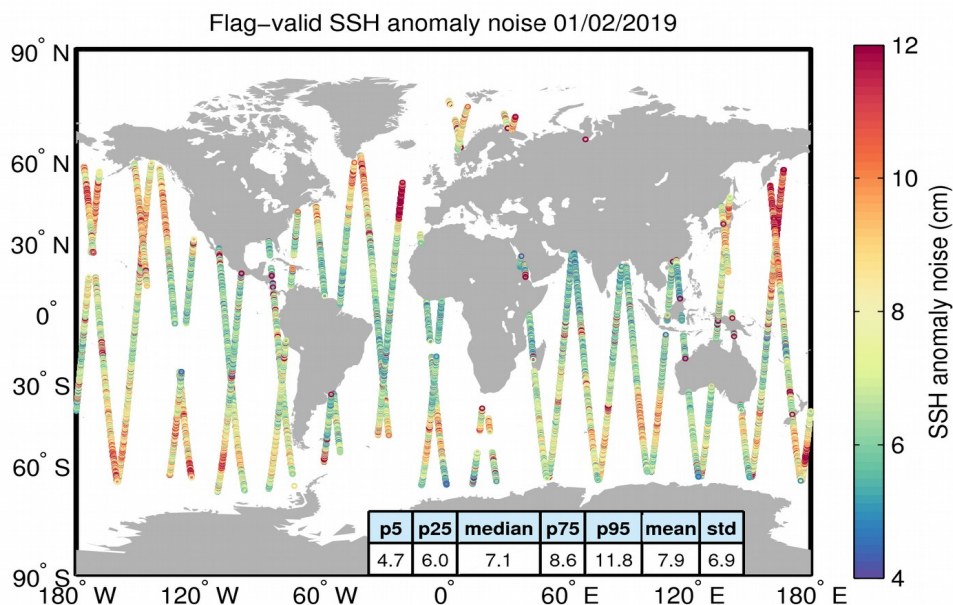
Figure 8. Geographical distribution of flag-valid 20-Hz SSH anomaly measurement noise over oceans and lakes for 01/02/2019. The statistical values shown in the table refer to the SSH anomaly noise and are calculated over all measurements shown in the figure.
