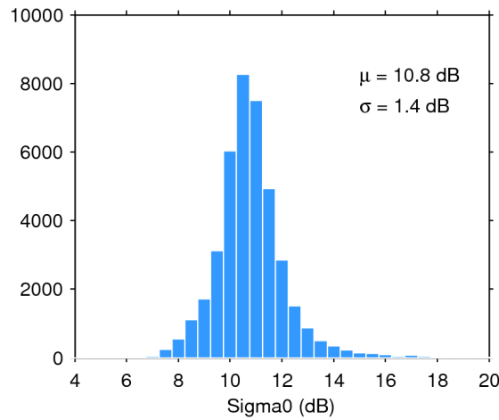
Figure 28. Histogram of science-valid sigma0 over oceans and lakes for 01/02/2019. The mean ( \mu ) and standard deviation ( \sigma ) are also shown. Note that values outside [4 20] dB are excluded from the histogram for the sake of readability but not from the computation of \mu and \sigma .
