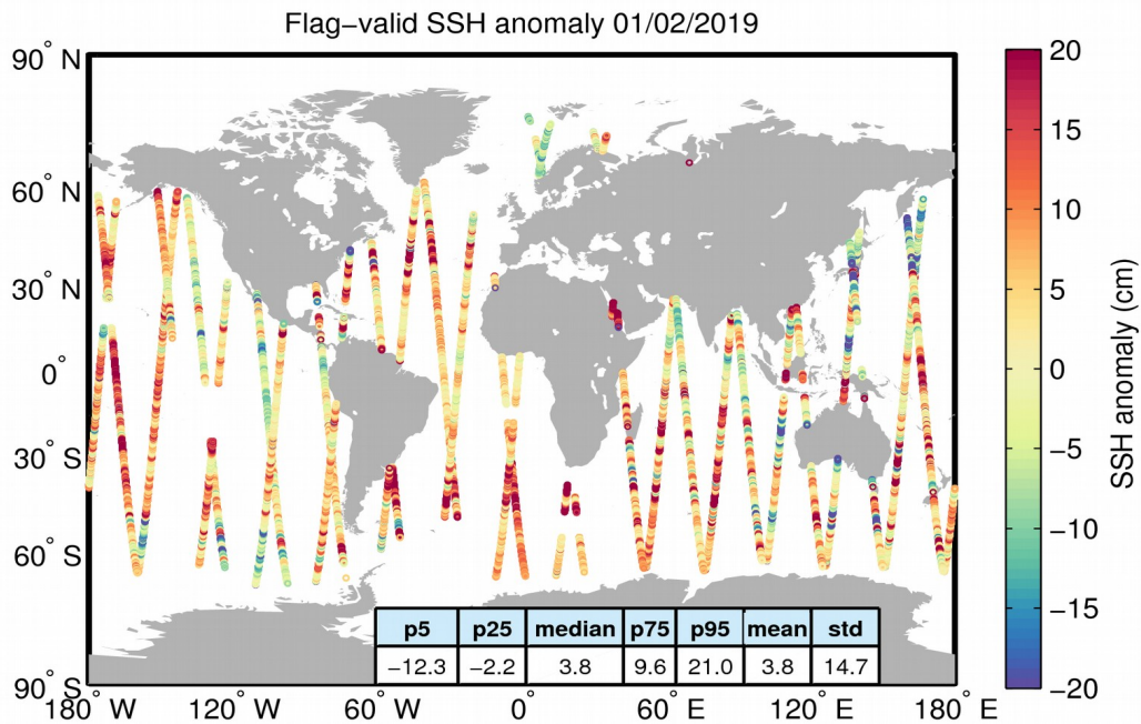
Figure 5. Geographical distribution of flag-valid 1-Hz SSH anomaly data over oceans and lakes for 01/02/2019. The statistical values shown in the table refer to the SSH anomaly in cm and are calculated over all measurements shown in the figure.
