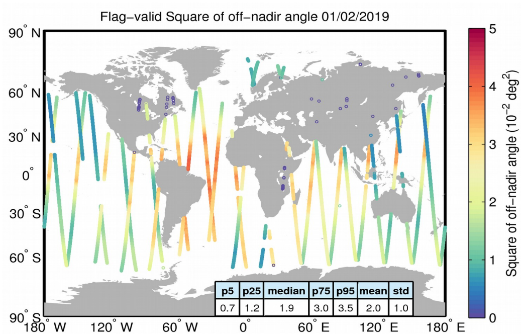
Figure 37. Geographical distribution of flag-valid mispointing data over oceans and lakes for 01/02/2019. The statistical values shown in the table refer to the mispointing in 10^{-2} \text{ deg}^2 and are calculated over all measurements shown in the figure.
