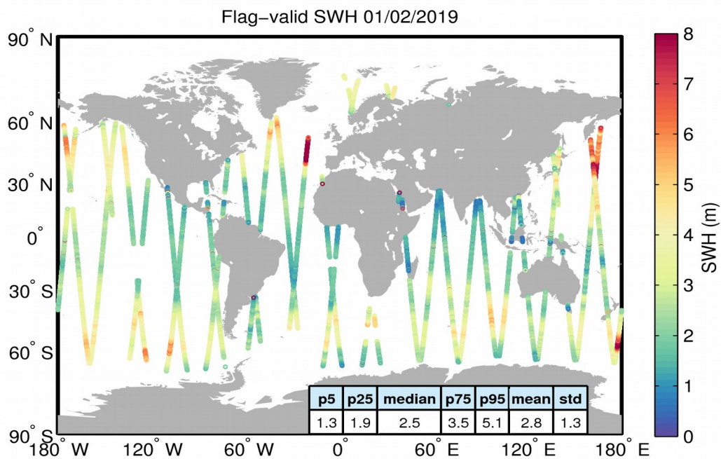
Figure 15. Geographical distribution of flag-valid SWH data over oceans and lakes for 01/02/2019. The statistical values shown in the table refer to the SWH in m and are calculated over all measurements shown in the figure.
