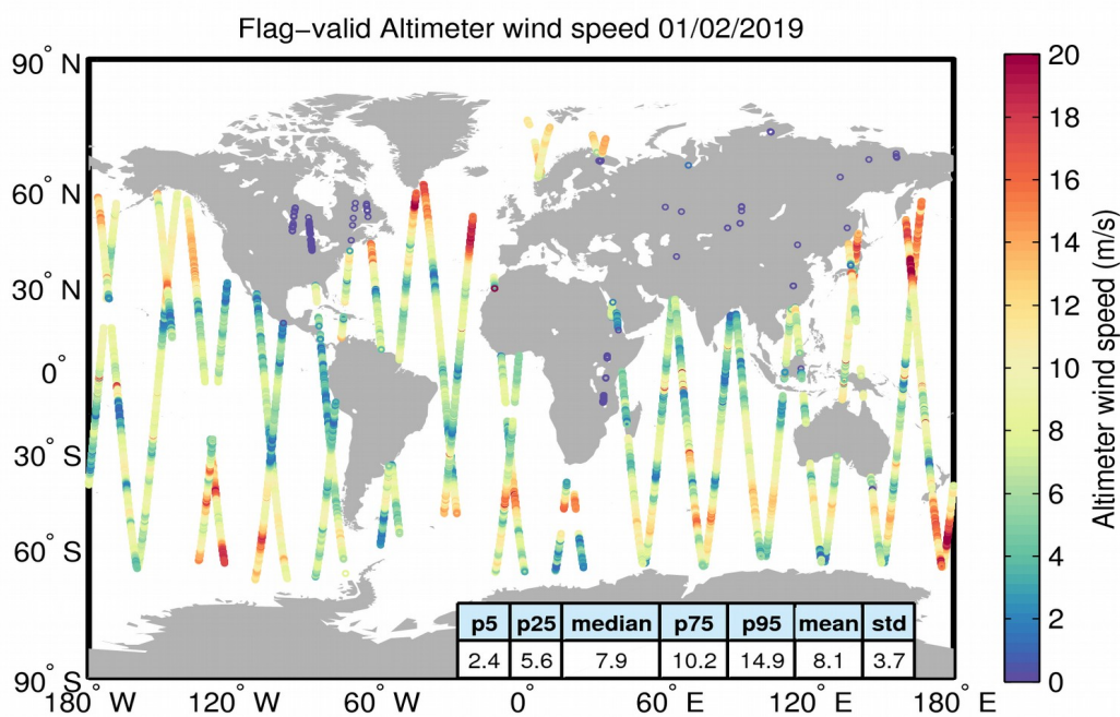
Figure 31. Geographical distribution of flag-valid wind data over oceans and lakes for 01/02/2019. The statistical values shown in the table refer to the wind in m/s and are calculated over all measurements shown in the figure.
