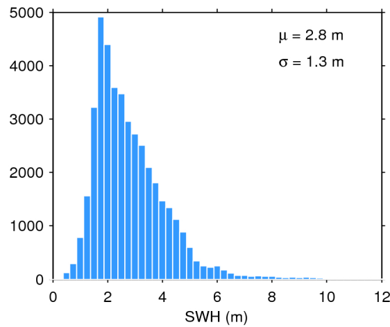
Figure 17. Histogram of flag-valid SWH over oceans and lakes for 01/02/2019. The mean ( \mu ) and standard deviation ( \sigma ) are also shown. Note that values larger than 12 m are excluded from the histogram for the sake of readability but not from the computation of \mu and \sigma .
