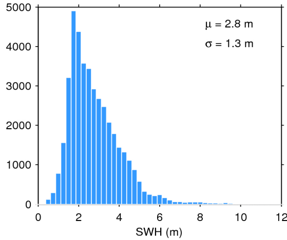
Figure 20. Histogram of science-valid SWH over oceans and lakes for 01/02/2019. The mean ( \mu ) and standard deviation ( \sigma ) are also shown. Note that values larger than 12 m are excluded from the histogram for the sake of readability but not from the computation of \mu and \sigma .
