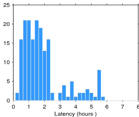
Figure 2. Histogram of the data latency for 01/02/2019. The y-axis denotes the number of files that are made available with a delay of x-hours with respect to the mean time of the records stored in the file.
