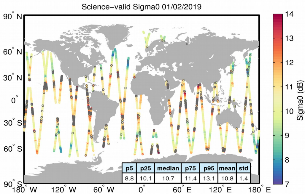
Figure 27. Geographical distribution of science-valid sigma0 data over oceans and lakes for 01/02/2019. The statistical values shown in the table refer to the sigma0 in dB and are calculated over all measurements shown in the figure. Gray circles denote records that have been rejected based on the editing criteria described in Table 4.
