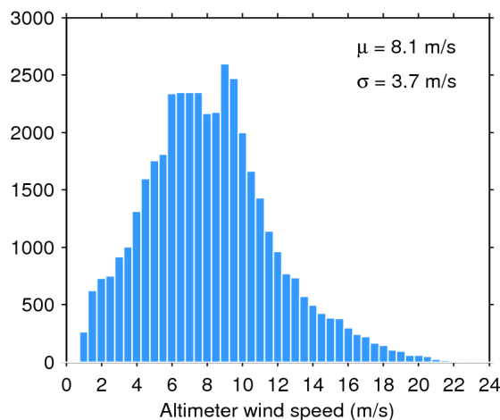
Figure 35. Histogram of science-valid wind over oceans and lakes for 01/02/2019. The mean ( \mu ) and standard deviation ( \sigma ) are also shown. Note that values larger than 24 m/s are excluded from the histogram for the sake of readability but not from the computation of \mu and \sigma .
