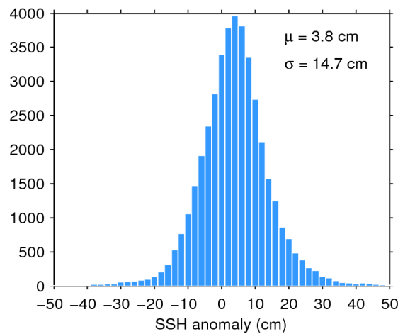
Figure 7. Histogram of flag-valid SSH anomaly over oceans and lakes for 01/02/2019. The mean ( \mu ) and standard deviation ( \sigma ) are also shown. Note that values outside [-50\ 50] cm are excluded from the histogram for the sake of readability but not from the computation of \mu and \sigma .
