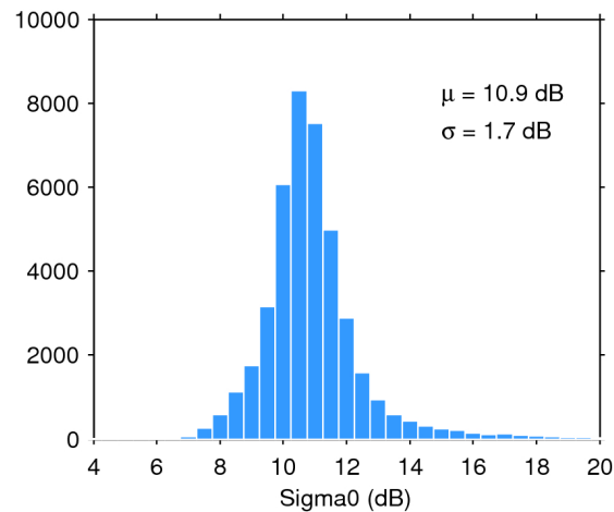
Figure 25. Histogram of flag-valid sigma0 over oceans and lakes for 01/02/2019. The mean ( \mu ) and standard deviation ( \sigma ) are also shown. Note that values outside [4 20] dB are excluded from the histogram for the sake of readability but not from the computation of \mu and \sigma .
