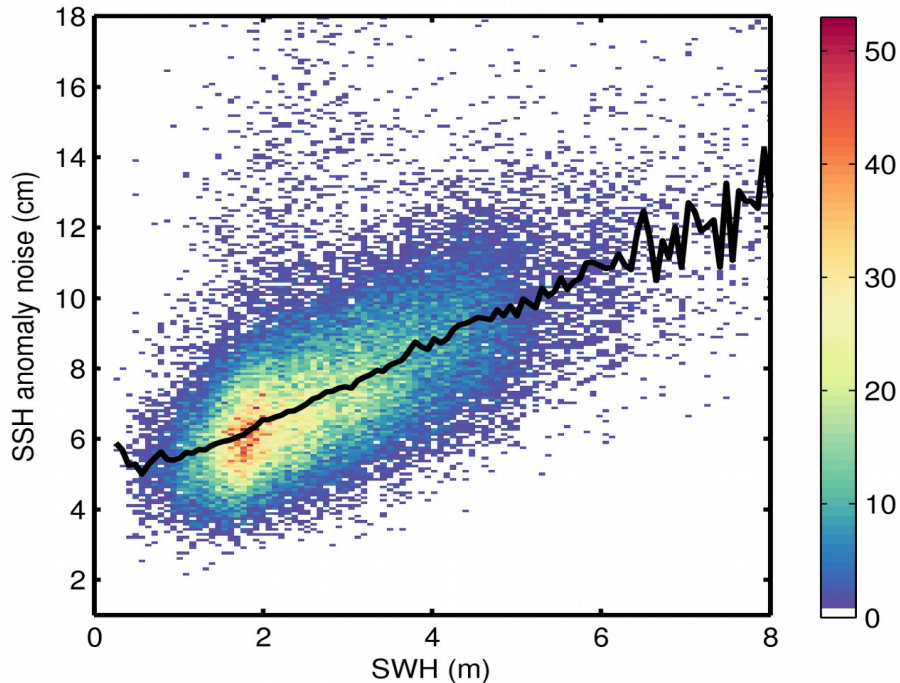
Figure 9. 2D histogram showing flag-valid SSH anomaly noise as a function of SWH for 01/02/2019. The black line denotes the median SSH anomaly noise as a function of SWH.
