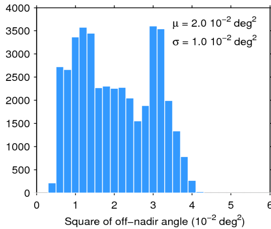
Figure 39. Histogram of flag-valid mispointing over oceans and lakes for 01/02/2019. The mean ( \mu ) and standard deviation ( \sigma ) are also shown. Note that values larger than 6 \cdot 10^{-2} \text{ deg}^2 are excluded from the histogram for the sake of readability but not from the computation of \mu and \sigma .
