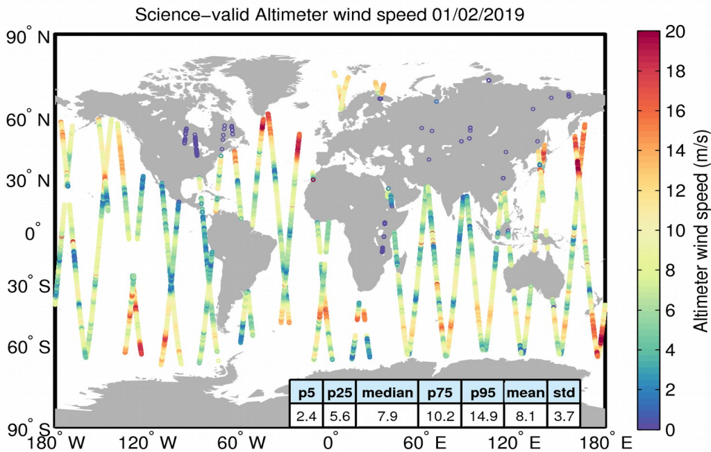
Figure 34. Geographical distribution of science-valid wind data over oceans and lakes for 01/02/2019. The statistical values shown in the table refer to the wind in m/s and are calculated over all measurements shown in the figure. Gray circles denote records that have been rejected based on the editing criteria described in Table 5.
