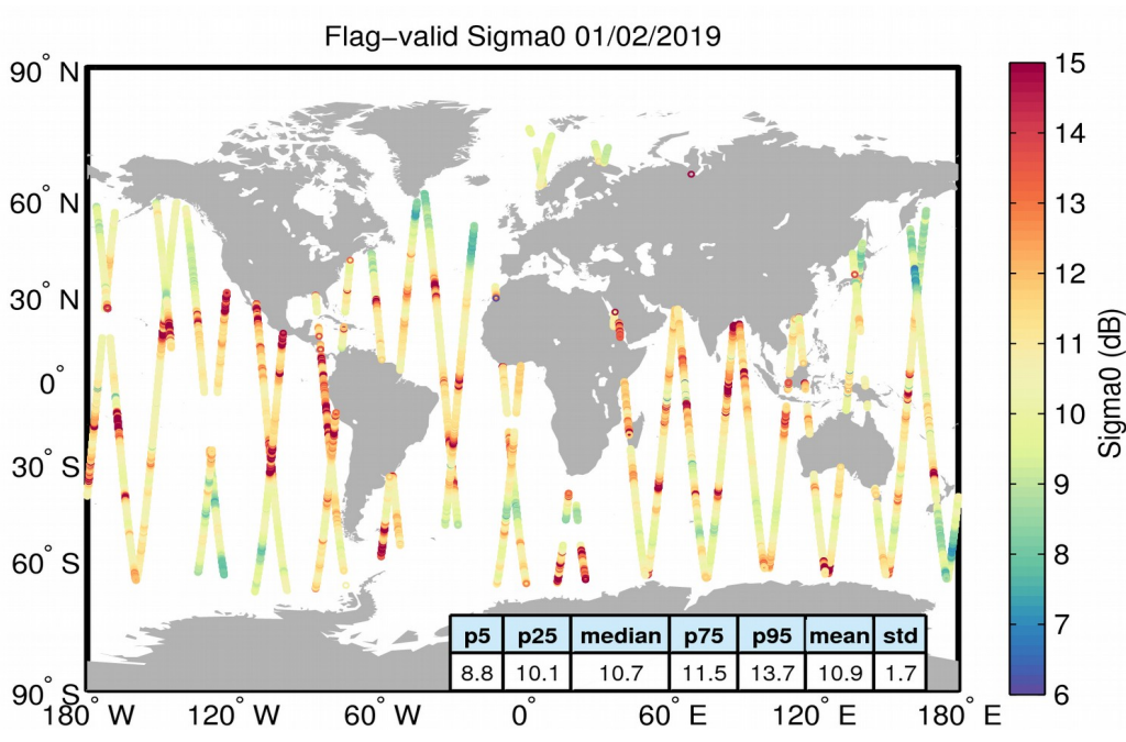
Figure 23. Geographical distribution of flag-valid sigma0 data over oceans and lakes for 01/02/2019. The statistical values shown in the table refer to the sigma0 in dB and are calculated over all measurements shown in the figure.
